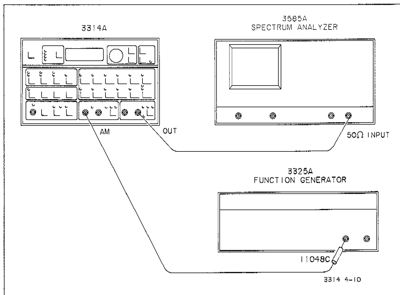
Figure 4-10. AM Harmonics
