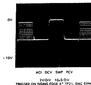
TP 18, MULTIPLEXED DAC OUTPUT (10.00Vp-p to 0.00Vp-p with invert function asserted)
