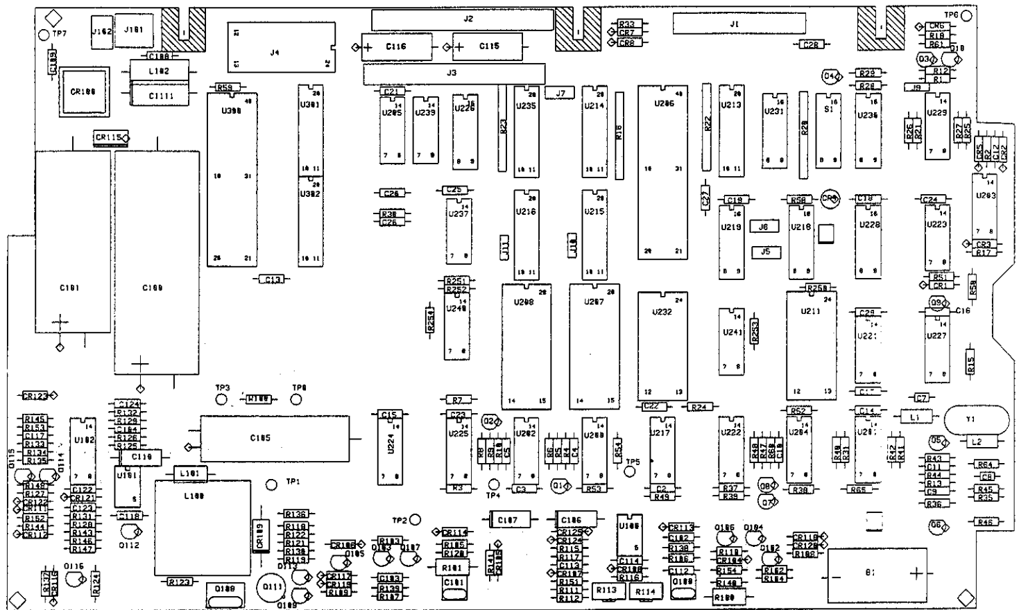
A3(Board Rev C) 03314-66503
