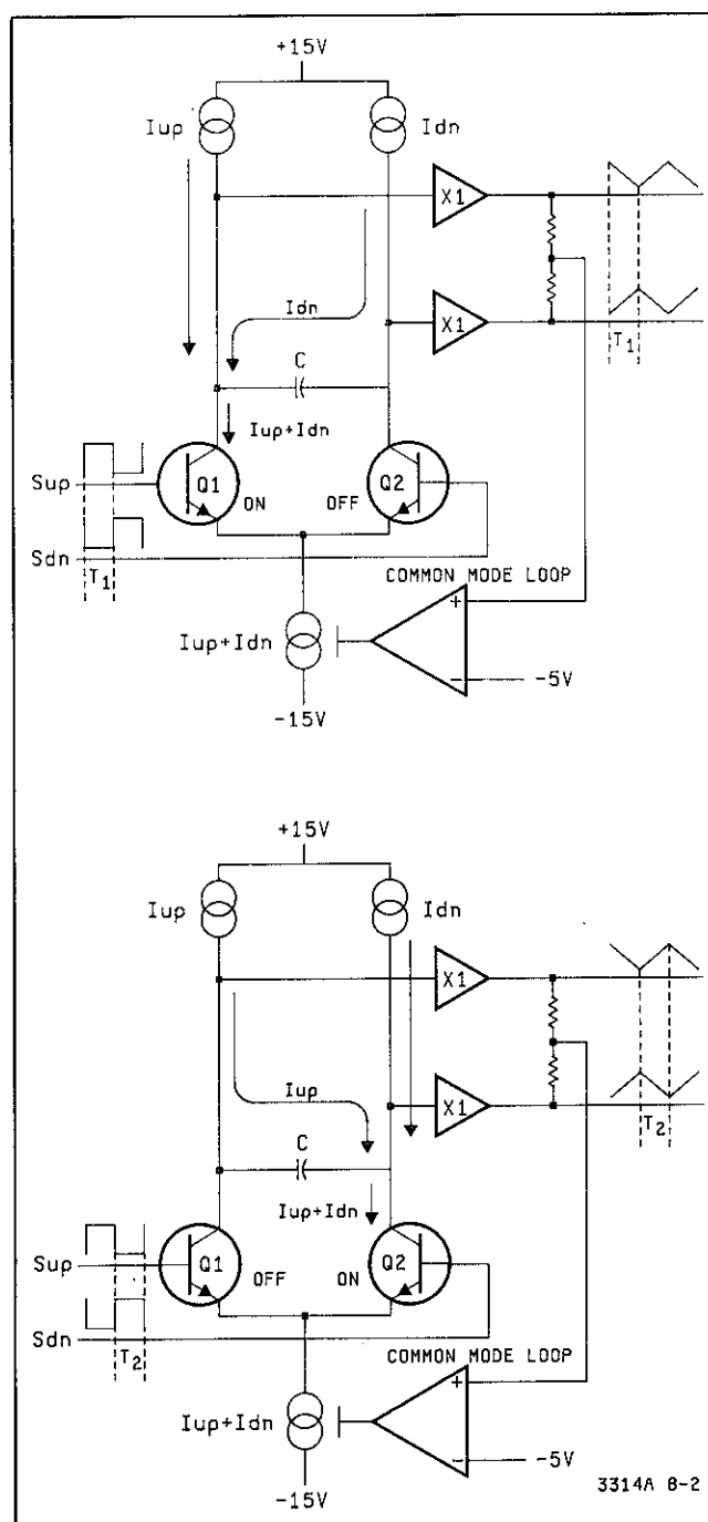
Figure 8-2. Basic Differential Integrator
