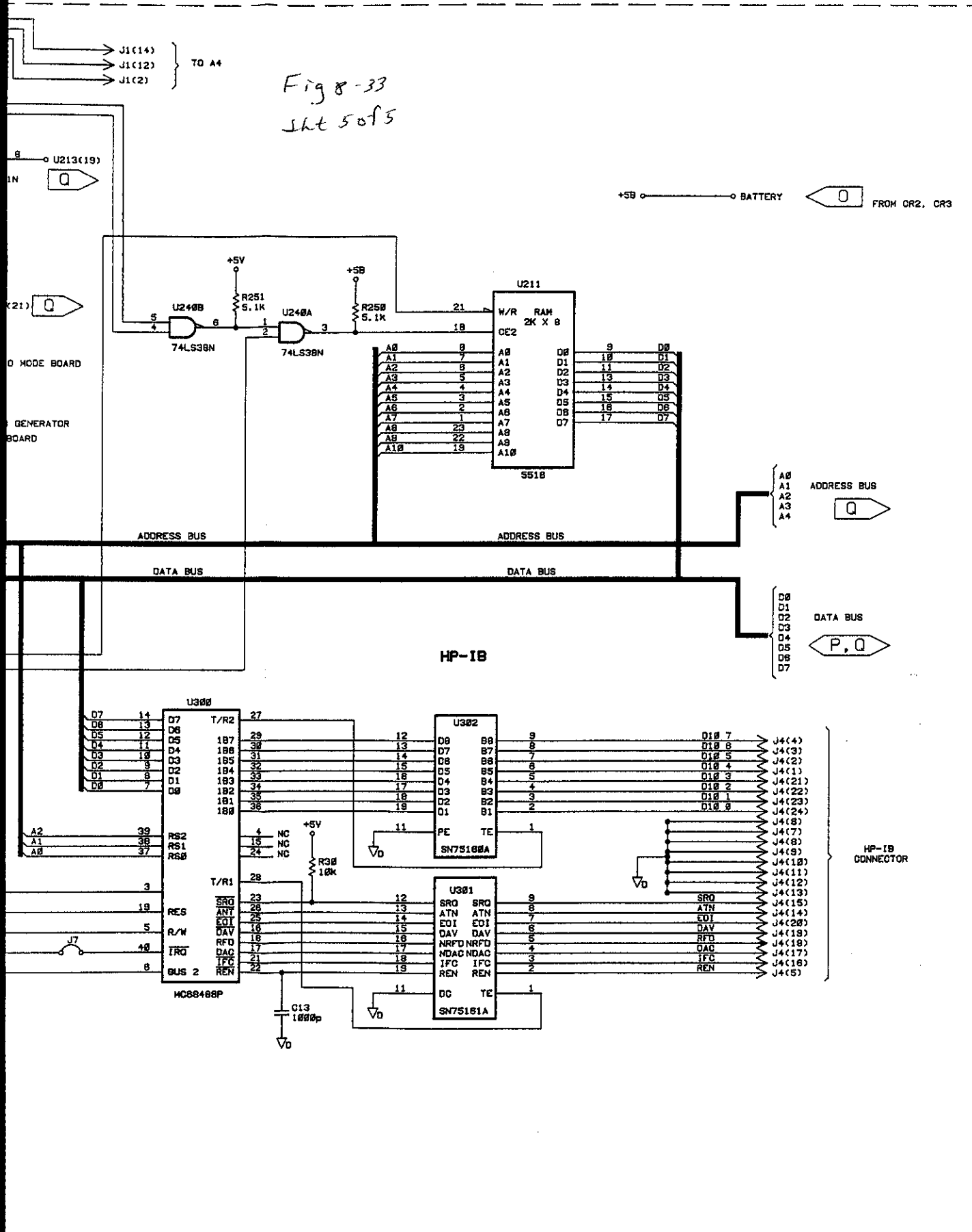
Figure 8-33. Processor, Memory and HP-IB Revised 10/86 8-73/8-74
