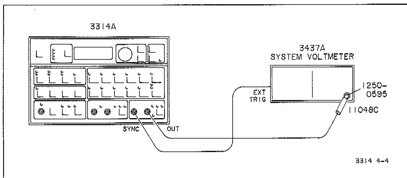
Figure 4-4. Triangle Linearity
