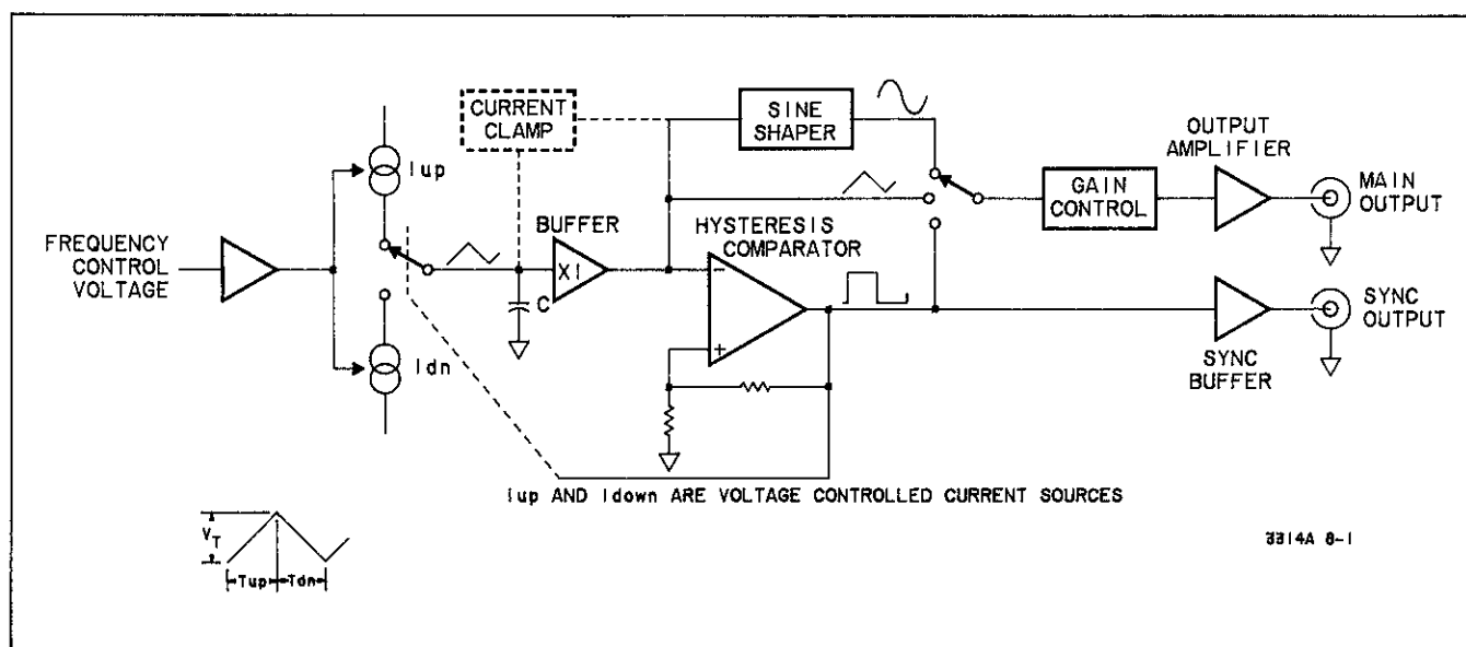
Figure 8-1. Basic Function Generator Block Diagram
