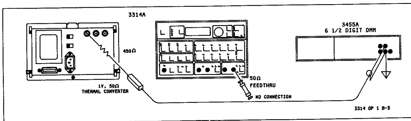
Figure 4-19. Sine Power Flatness Connections
