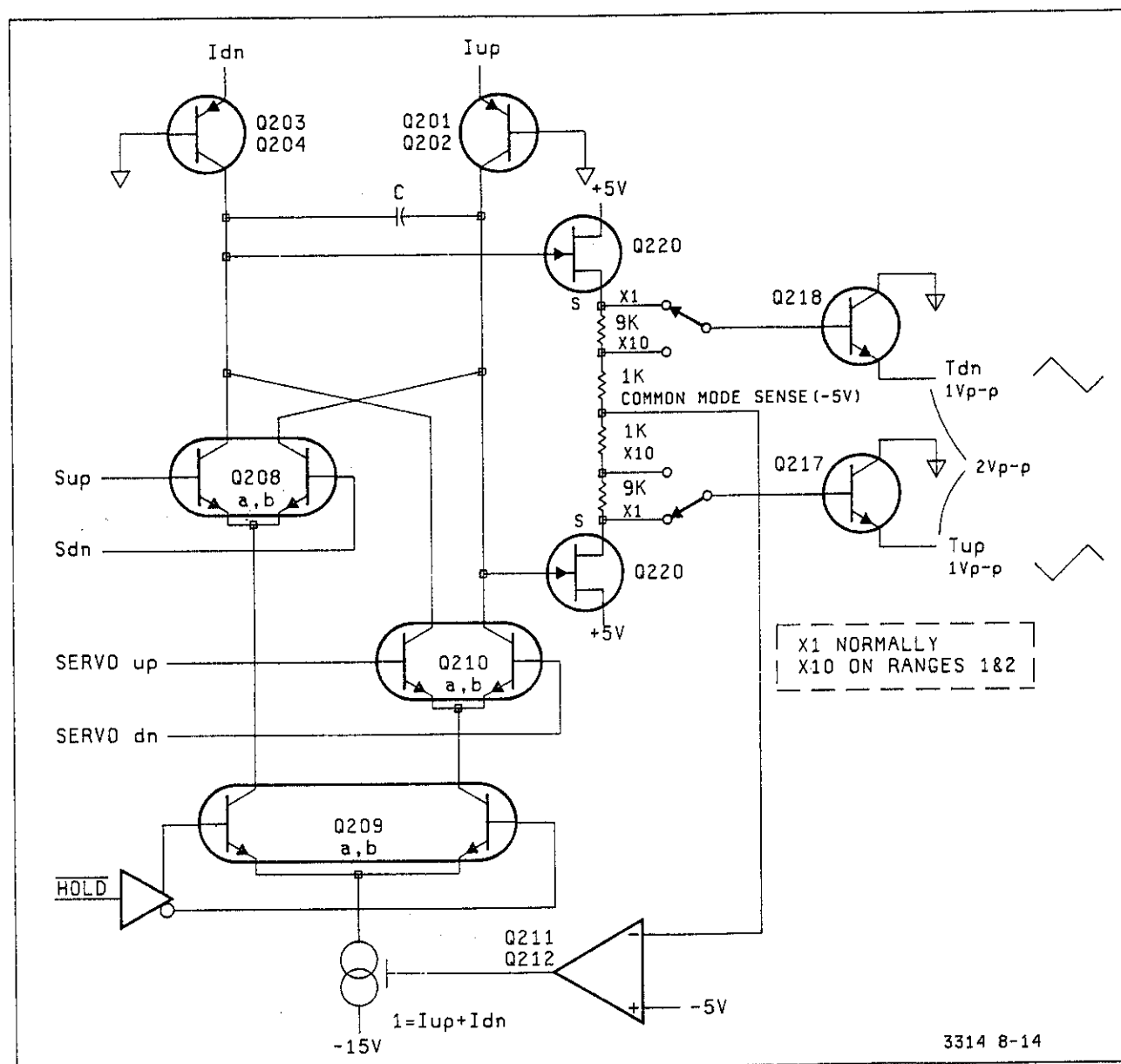
Figure 8-14. Integrator Block Diagram
