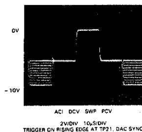
TP 18, MULTIPLEXED DAC OUTPUT (10.00Vp-p to 0.00Vp-p)
