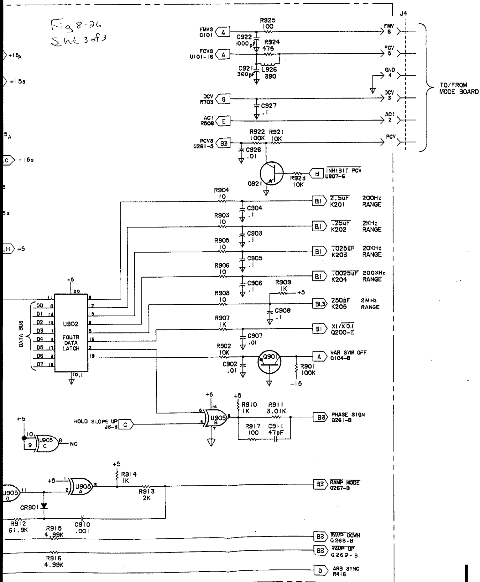
Figure 8-26. Misc Interface Revised 10/86 8-59/8-60
