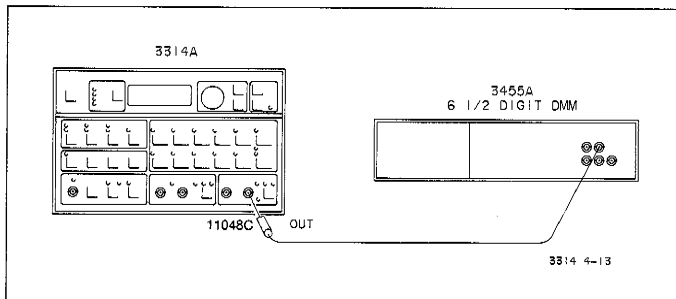
Figure 4-13. Amplitude Accuracy
