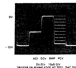
TP 19, MULTIPLEXED DAC OUTPUT (Phase)
