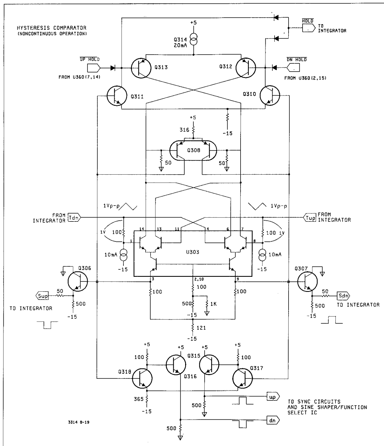
Figure 8-19. Comparator Block Diagram (Non-Continuous Operation)
