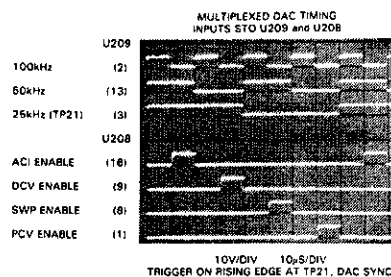
TP 18, MULTIPLEXED DAC OUTPUT AT POWER ON
