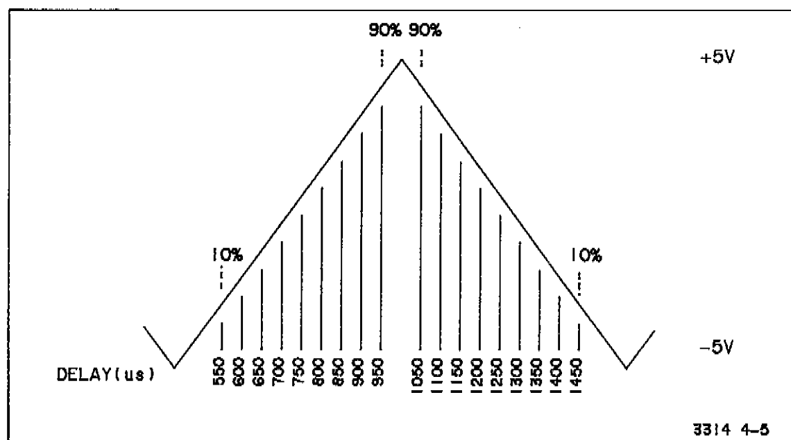
Figure 4-5. Triangle Linearity
