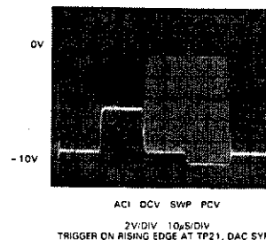
TP 19, MULTIPLEXED DAC OUTPUT DURING SWEEPS
