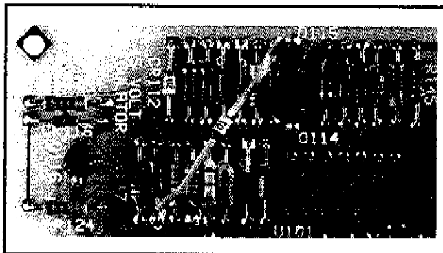
Figure 2-4. A3CR123 Installation
