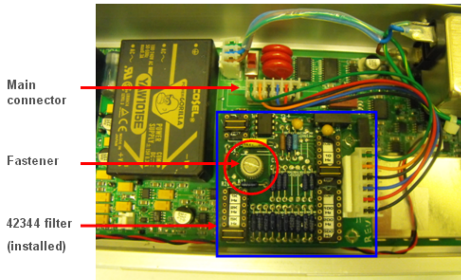
Picture 4. Screwing 42344 Filter into 2775B Signal Conditioner
