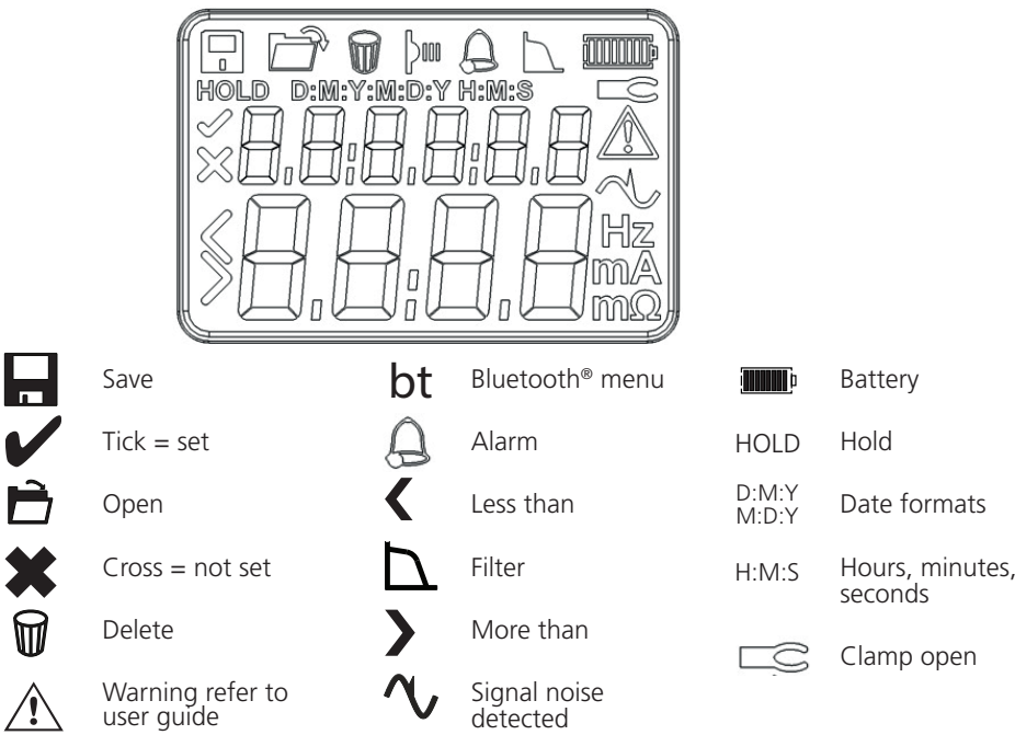
Figure 4: DET14C / DET24C Instrument Display View
