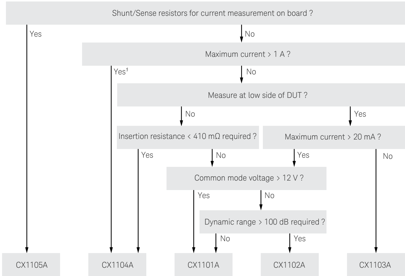
Quick Selection Chart of Current Sensors
