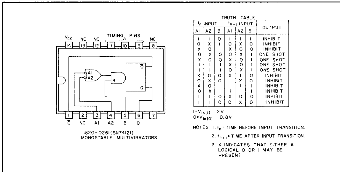
Figure 4-11. Monostable Multivibrator 1820-0261
