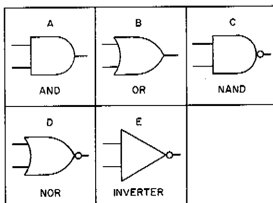
Figure 4-2. Gate Symbols
