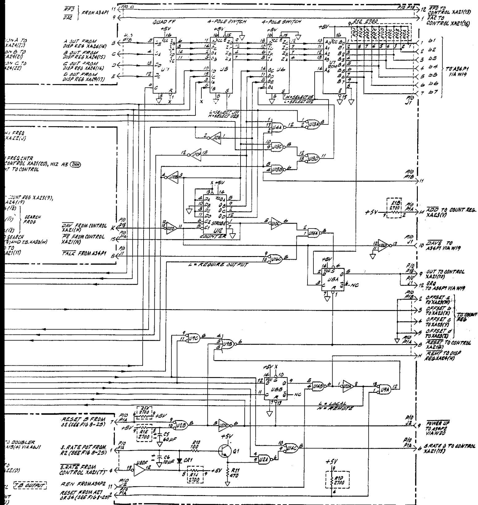
Figure 8-26. A19 Interface B Assembly (Part of Option 011)
