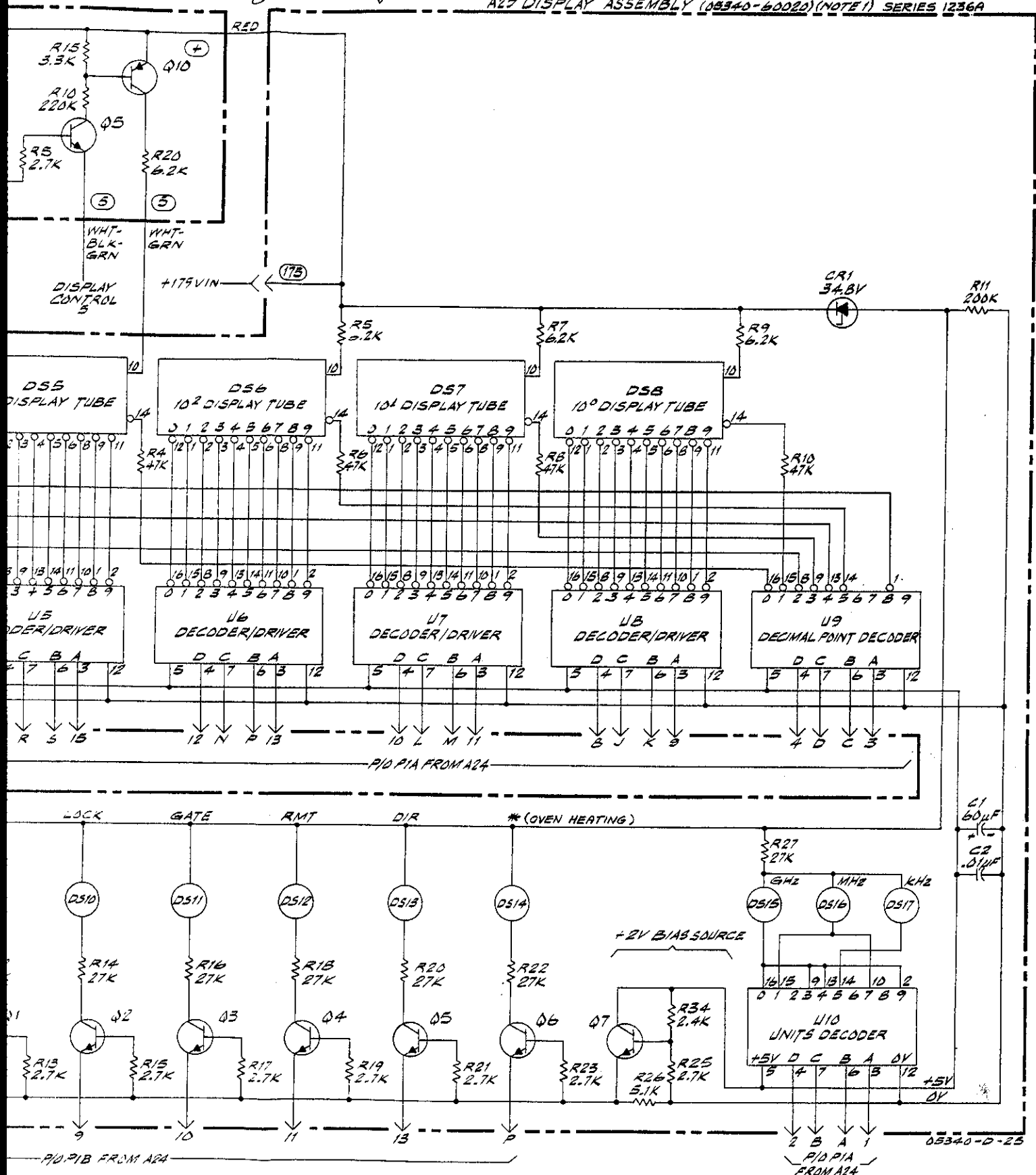
Figure 8-32. A25 Display Assembly, A26 Blanking Assembly
