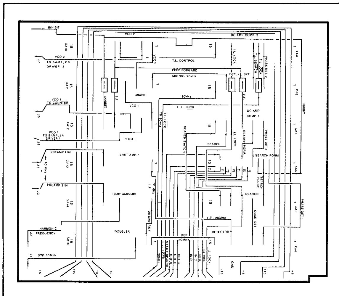
Figure 8-22. A16 Casting Motherboard
