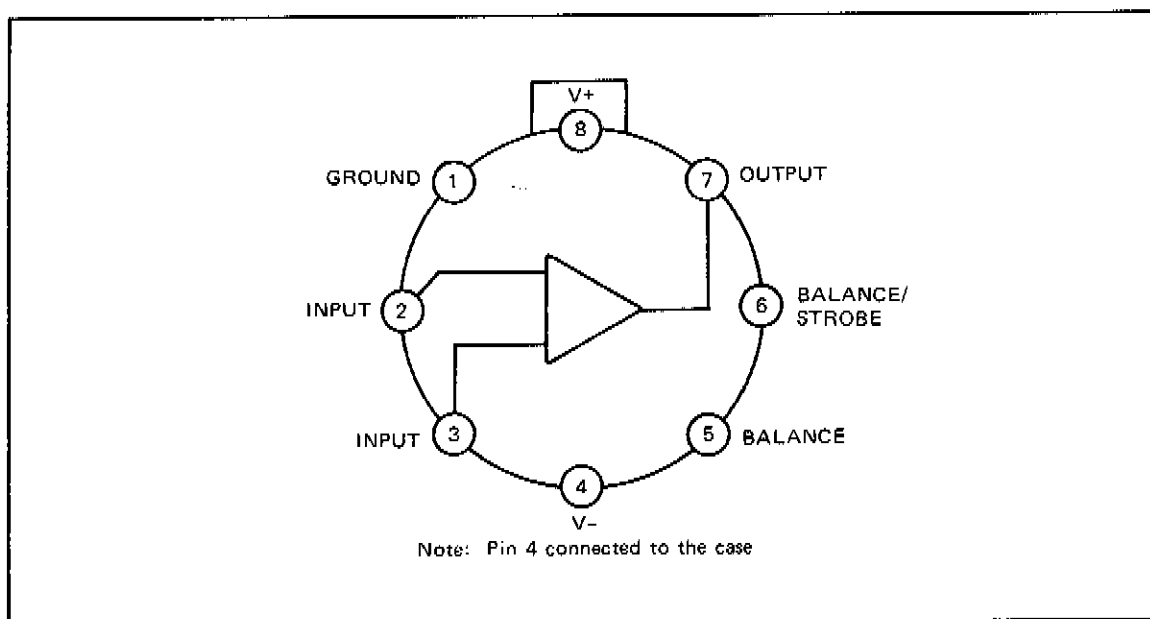
Figure 4-41. Voltage Comparator/Buffer 1826-0026
