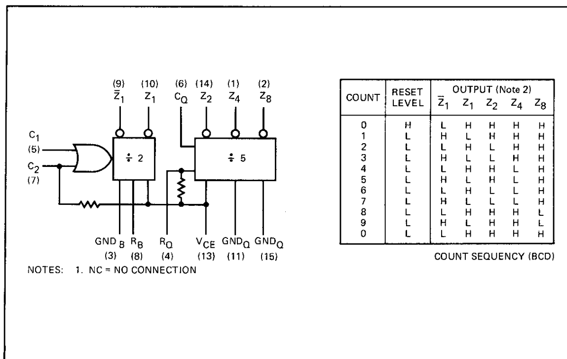
Figure 4-37. EECL Bi-Quinary Counter 1820-1019
