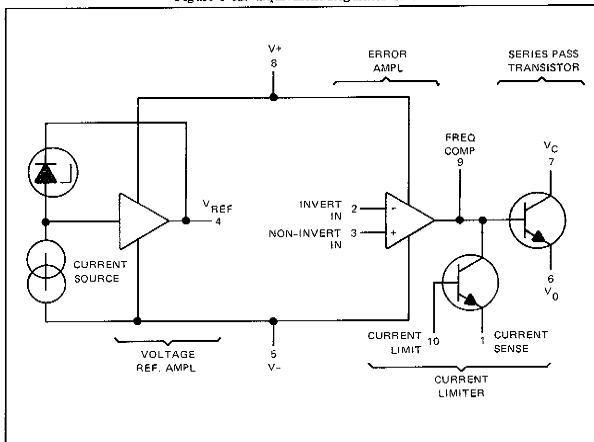
Figure 4-52. Equivalent Regulator Circuit
