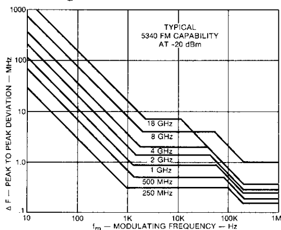
Figure 3-1. FM Characteristics
