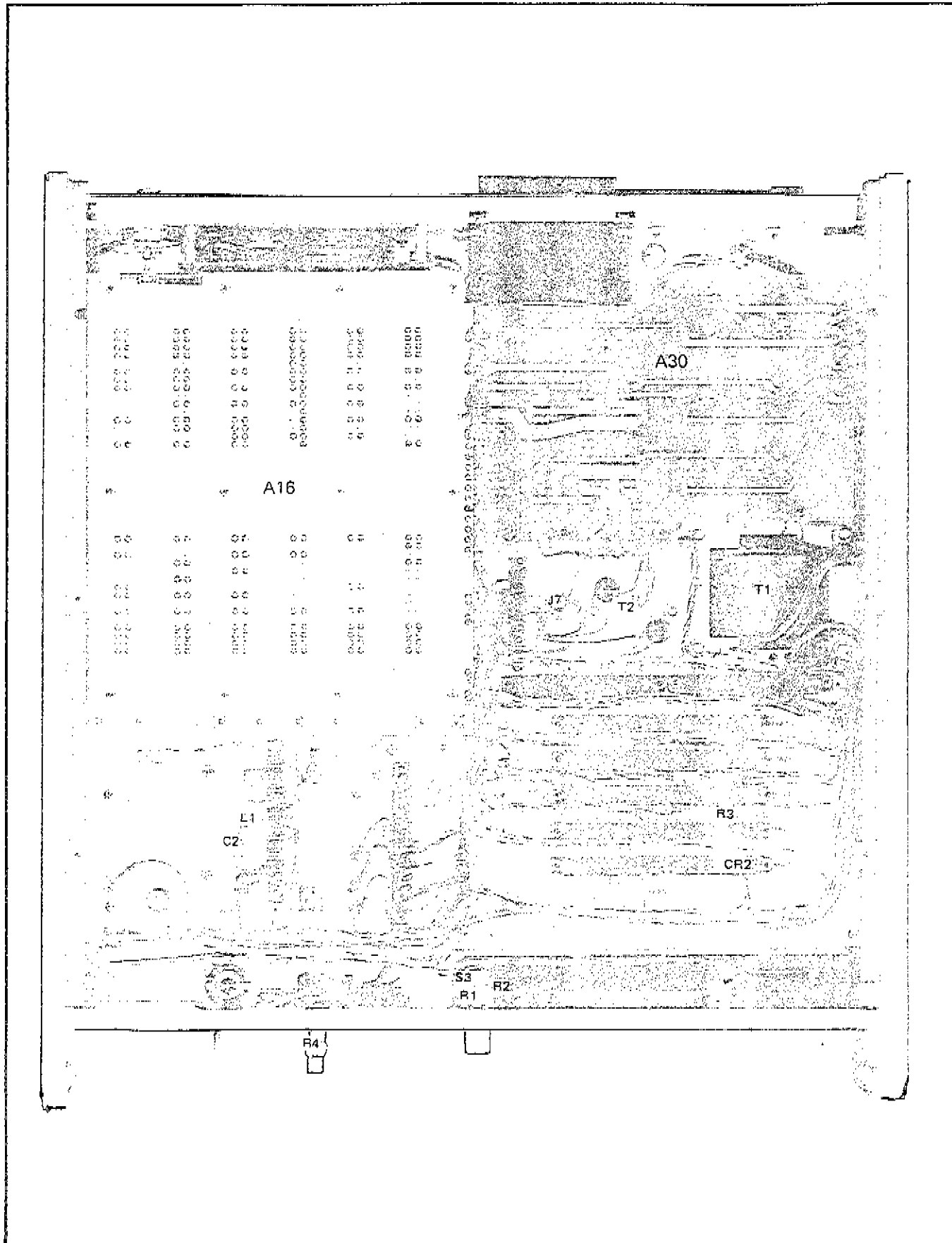
Figure 8-3. 5340A Bottom Internal View and Cable Numbers and Connections (with Options 001, 002, and 011 Installed)
