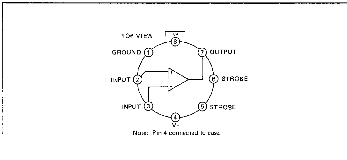
Figure 4-15. Voltage Comparator/Buffer 1820-0475
