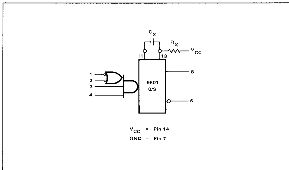
Figure 4-8. Monostable Multivibrator 1820-0207
