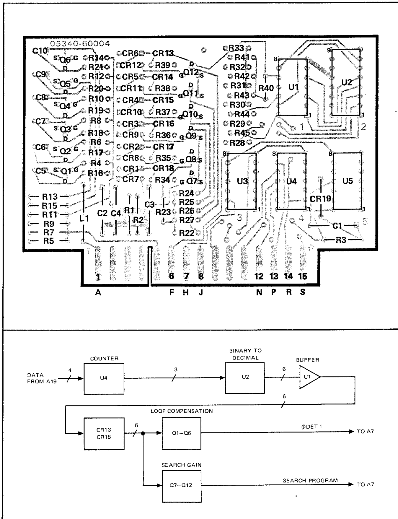
Part of Figure 8-12. A6 Search Programmer Assembly
