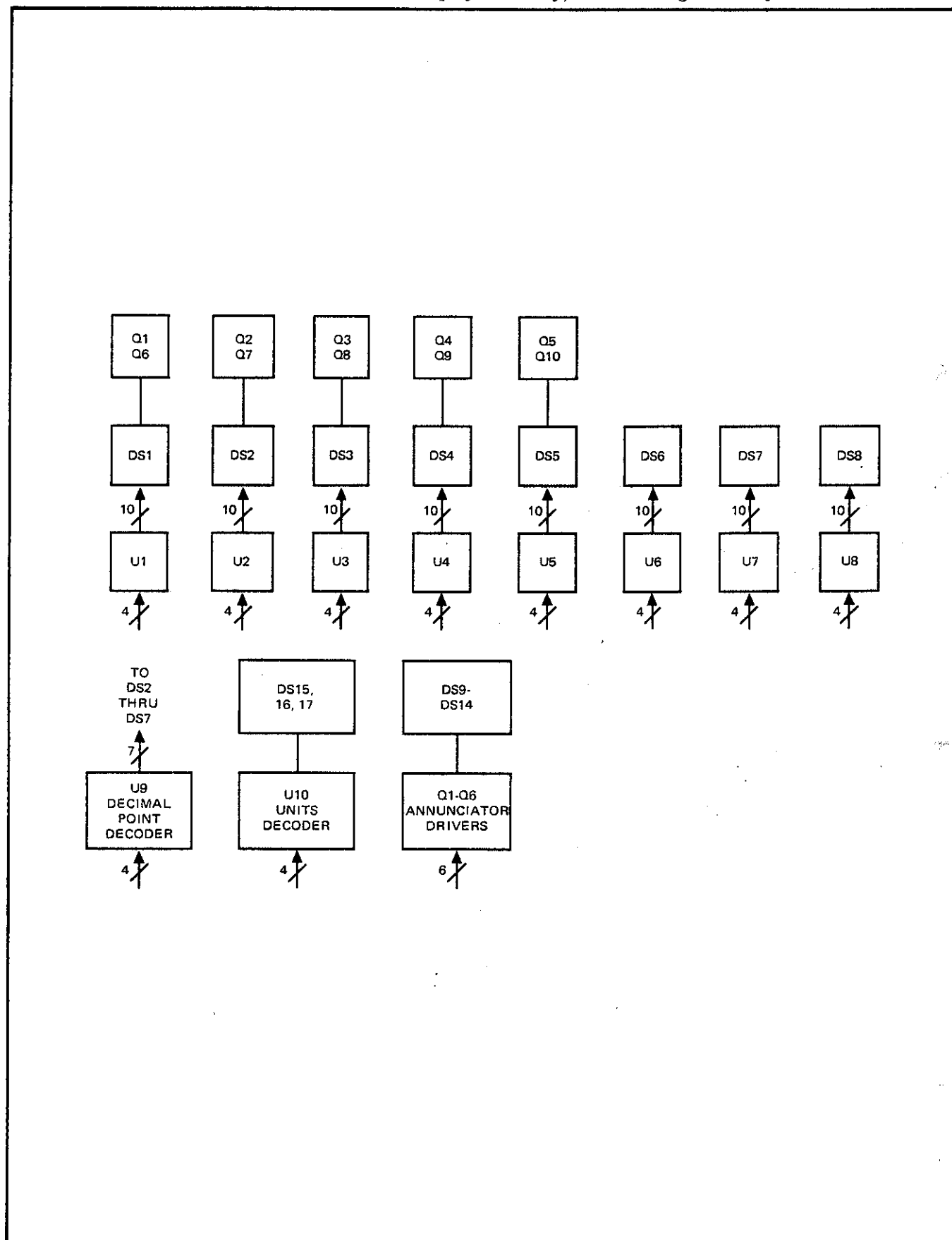
Part of Figure 8-32. A25 Display Assembly, A26 Blanking Assembly
