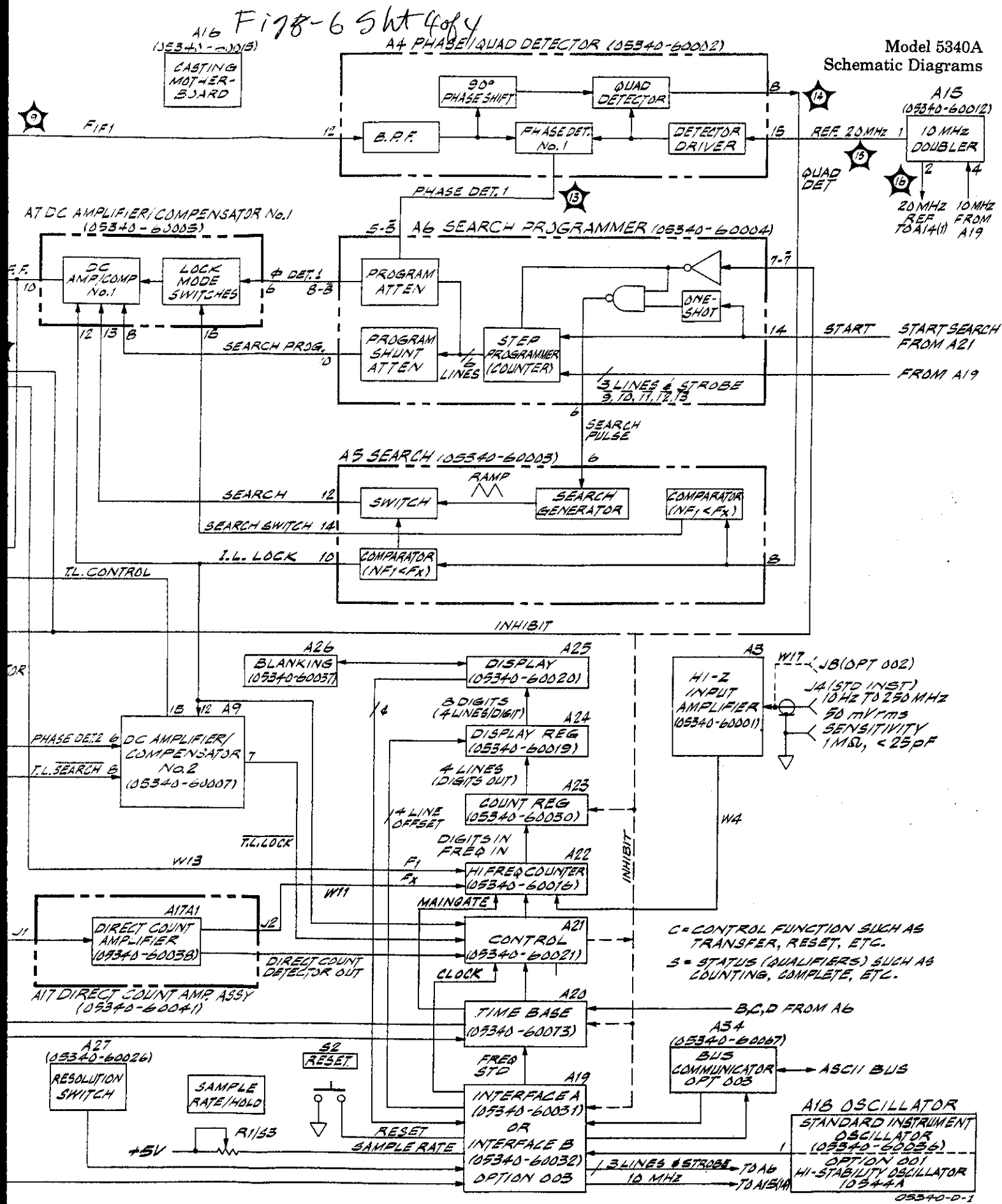
Figure 8-6. 5340A Block Diagram
