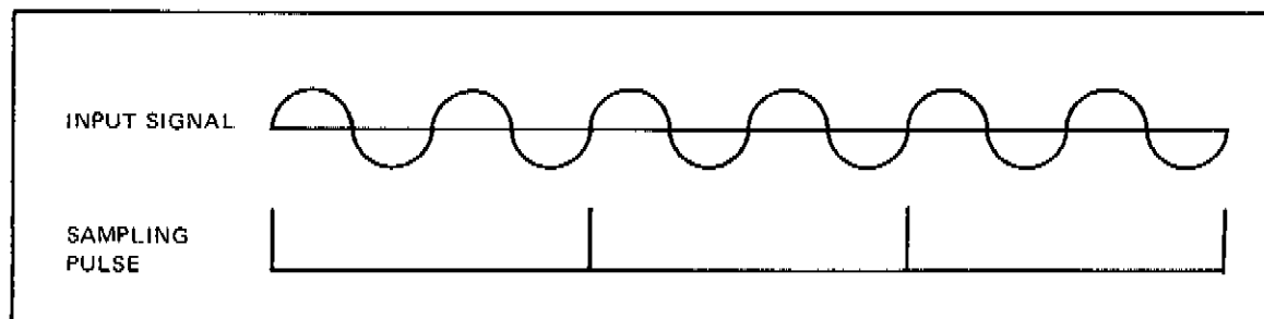
Figure 4-49. Sampling Timing
