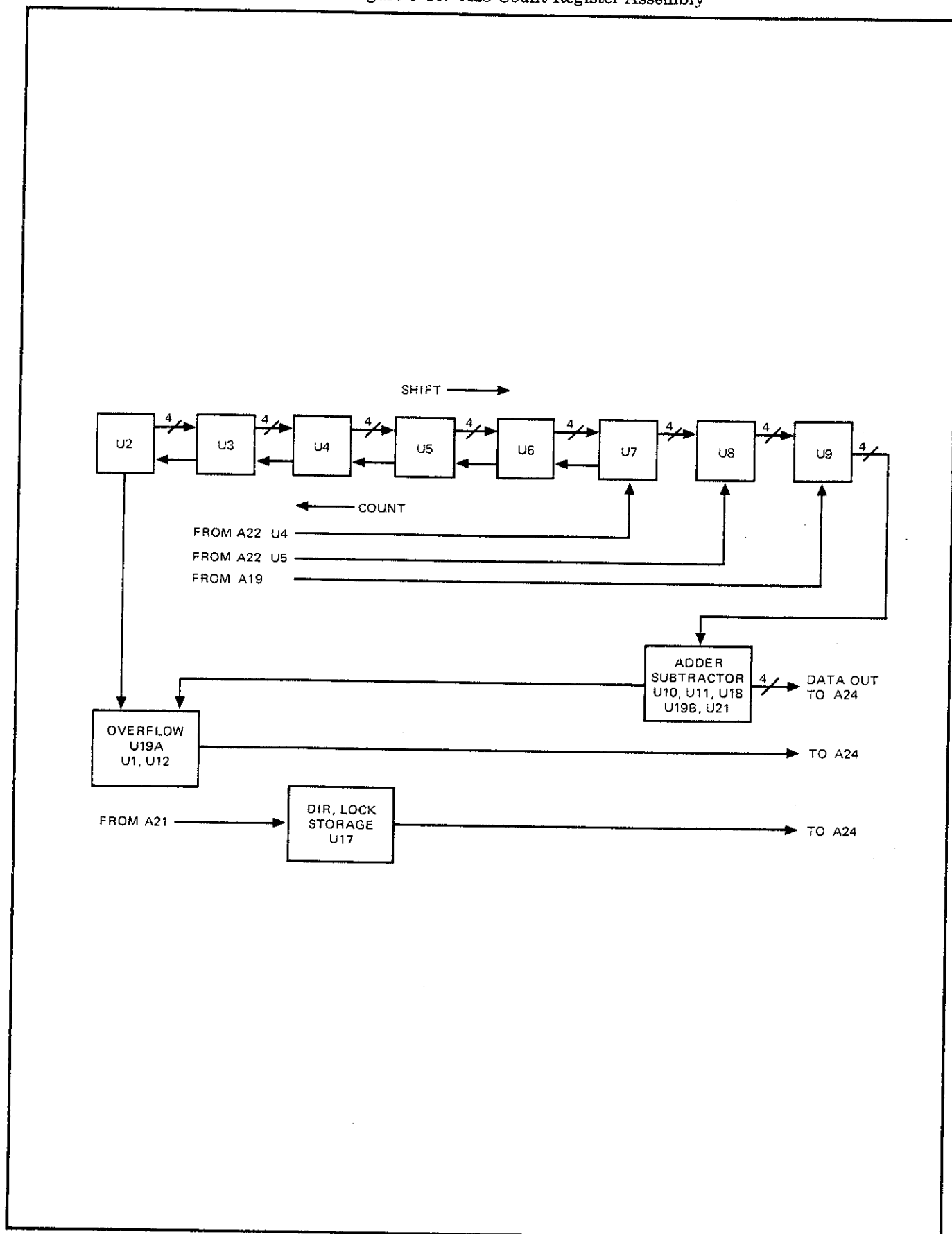
Part of Figure 8-30. A23 Count Register Assembly
