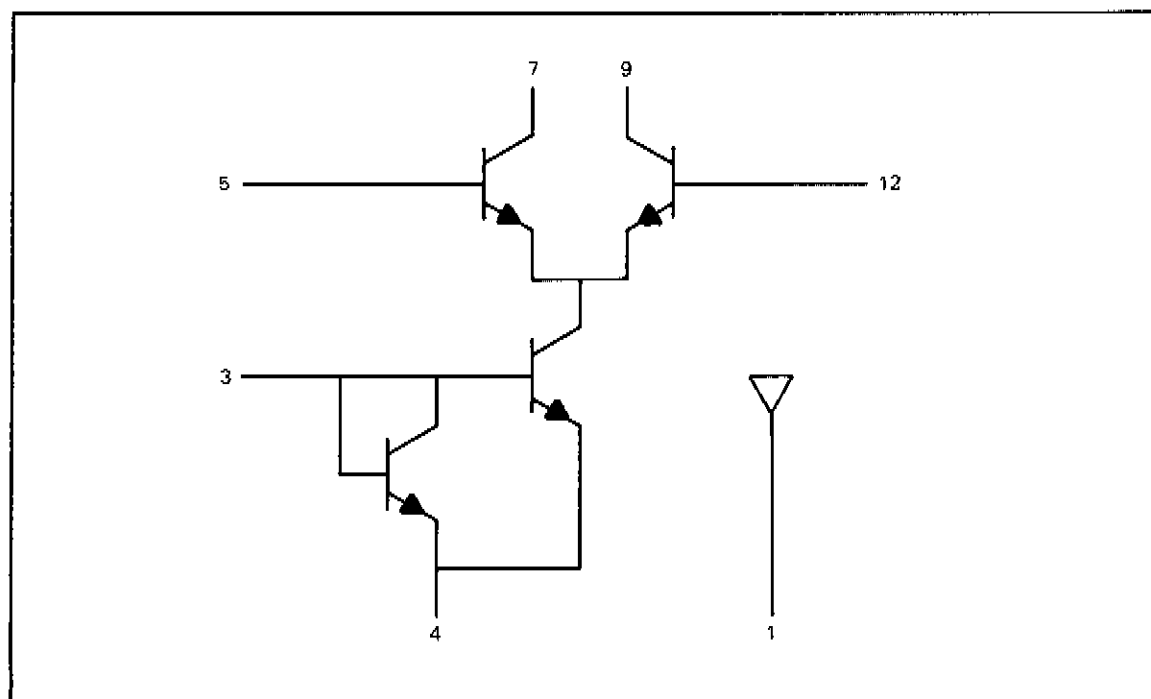
Figure 4-44. Transistor Array 1858-0018
