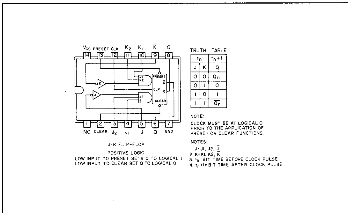
Figure 4-5. J-K Flip-Flop 1820-0065
