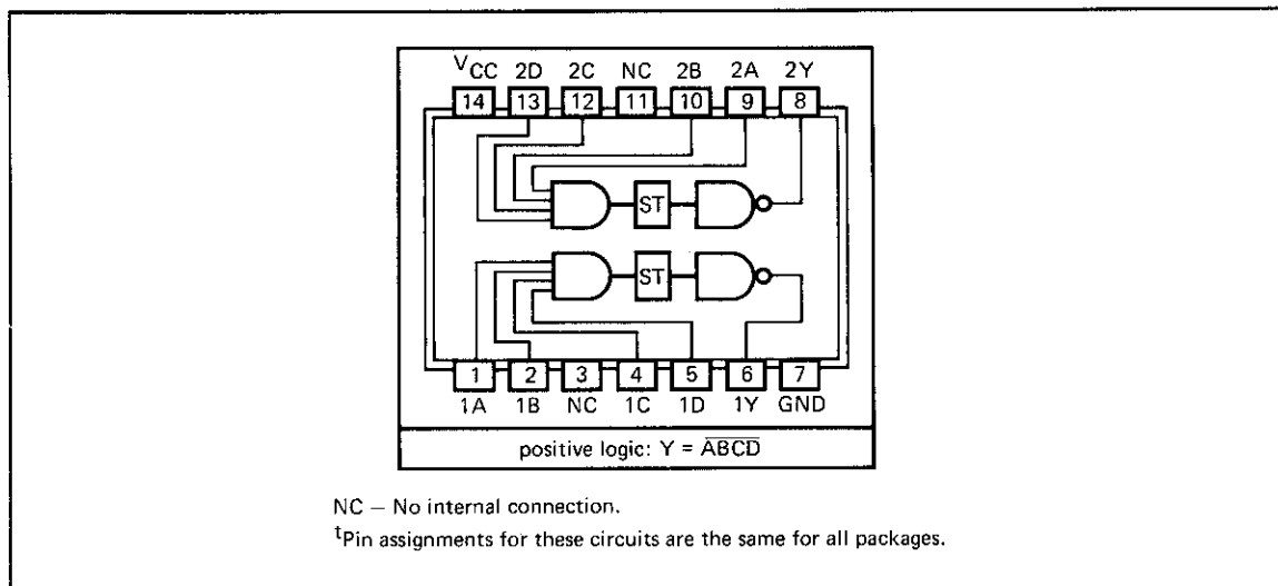
Figure 4-18. Dual NAND Schmitt Triggers 1820-0537
