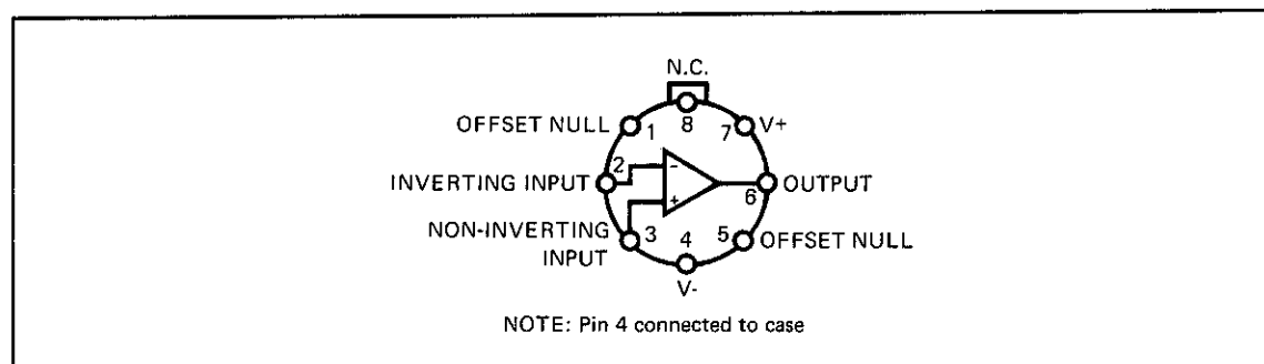
Figure 4-10. Operational Amplifier 1820-0216
