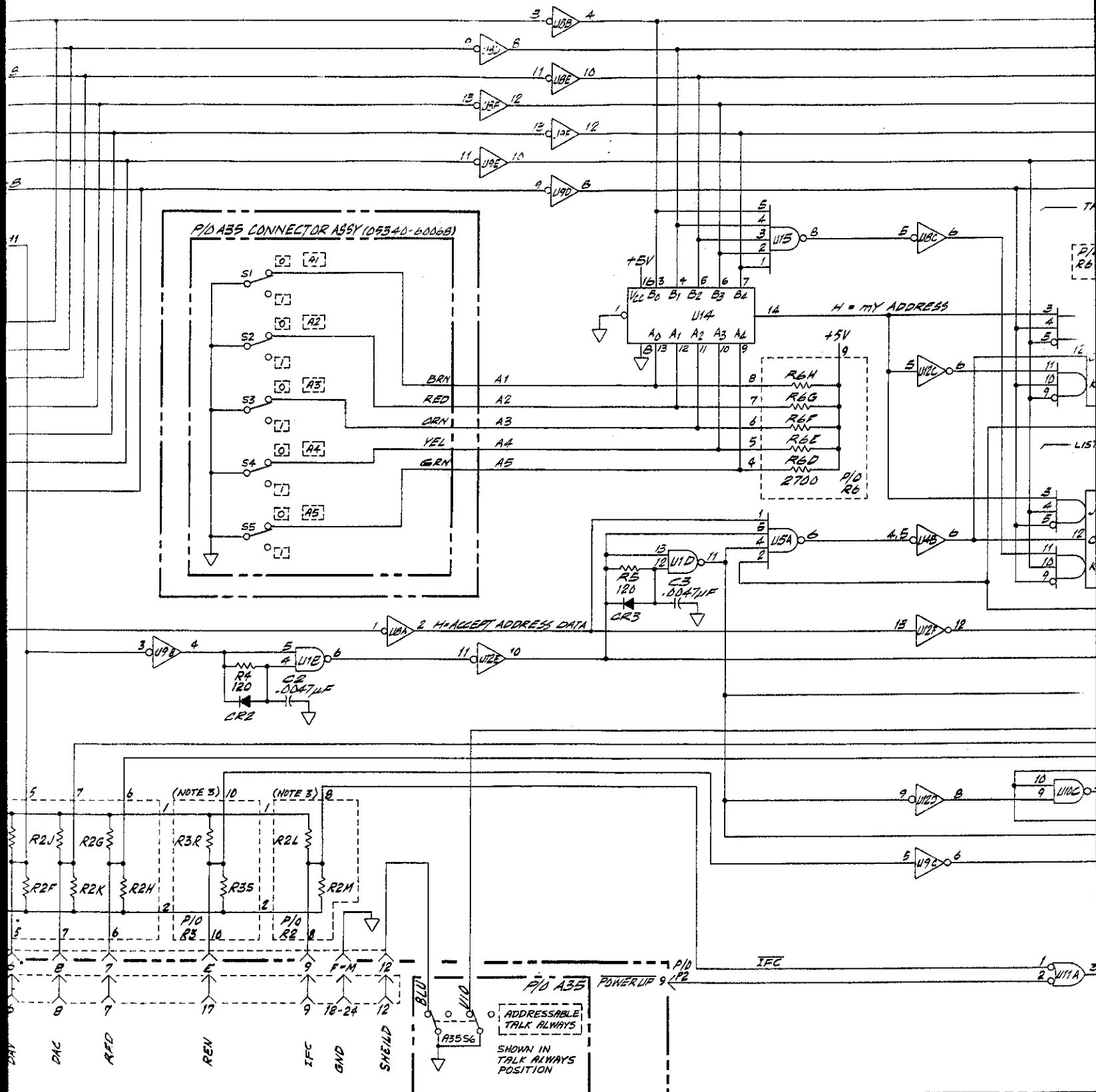
A34 BUS COMMUNICATOR ASSEMBLY (05340-60067) (NOTE 1) SERIES
