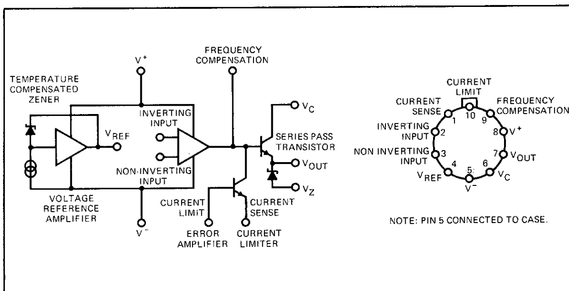
Figure 4-38. Voltage Regulator 1826-0010
