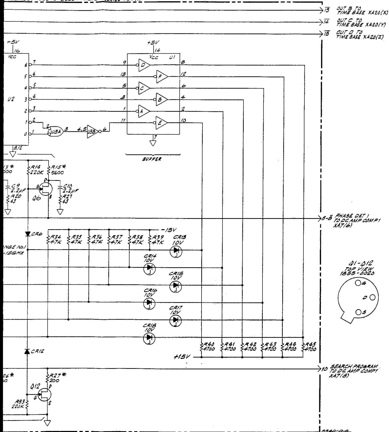
Figure 8-12. A6 Search Programmer Assembly
