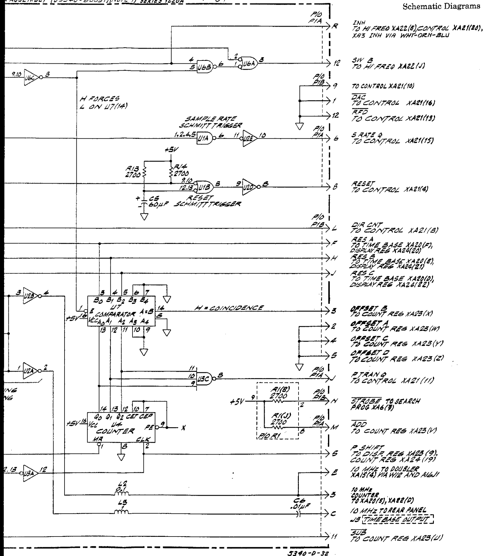
Figure 8-25. A19 Interface A Assembly (Standard Instrument), A27 Resolution Switch Assembly
