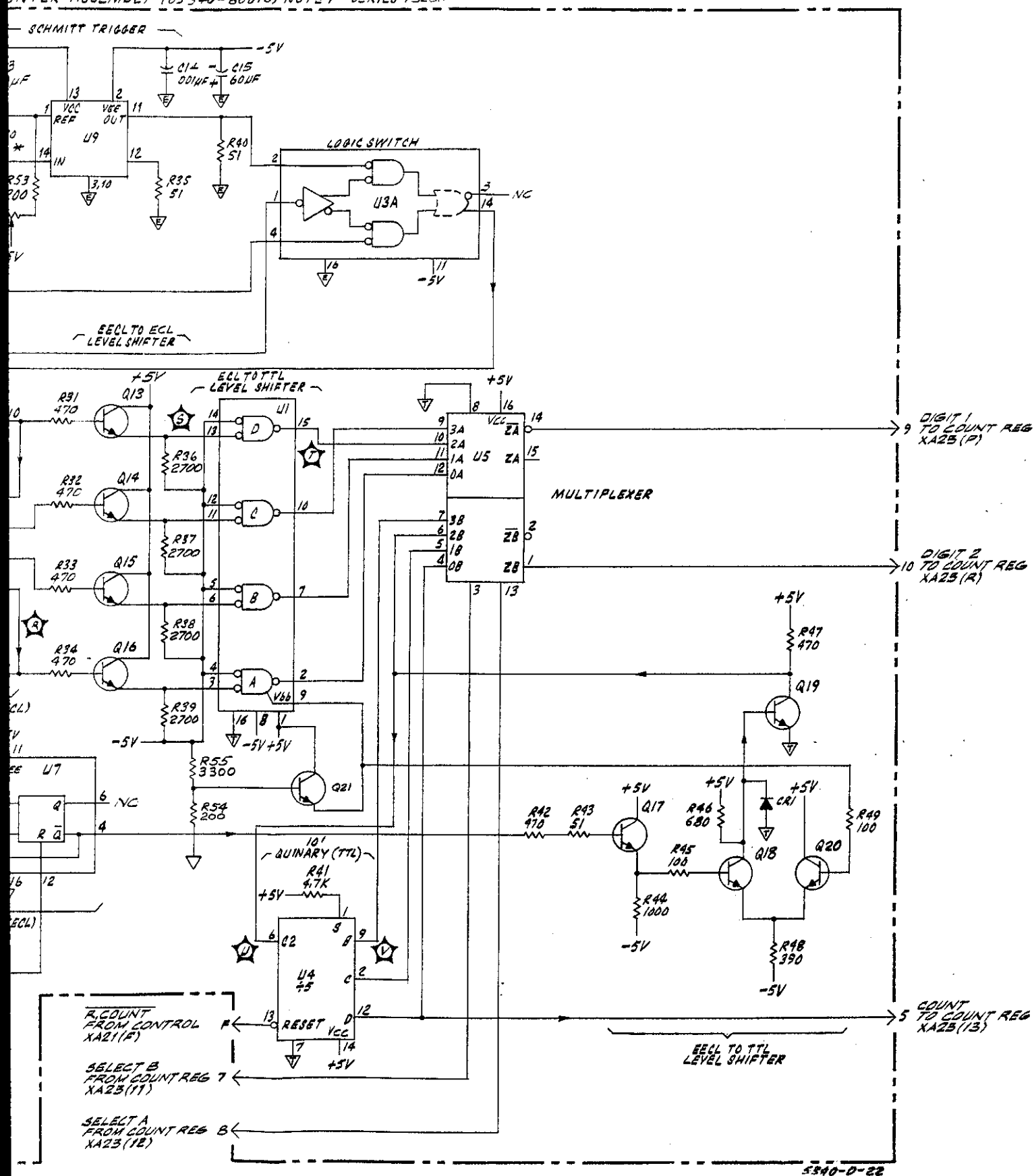
Figure 8-29. A22 High Frequency Counter Assembly
