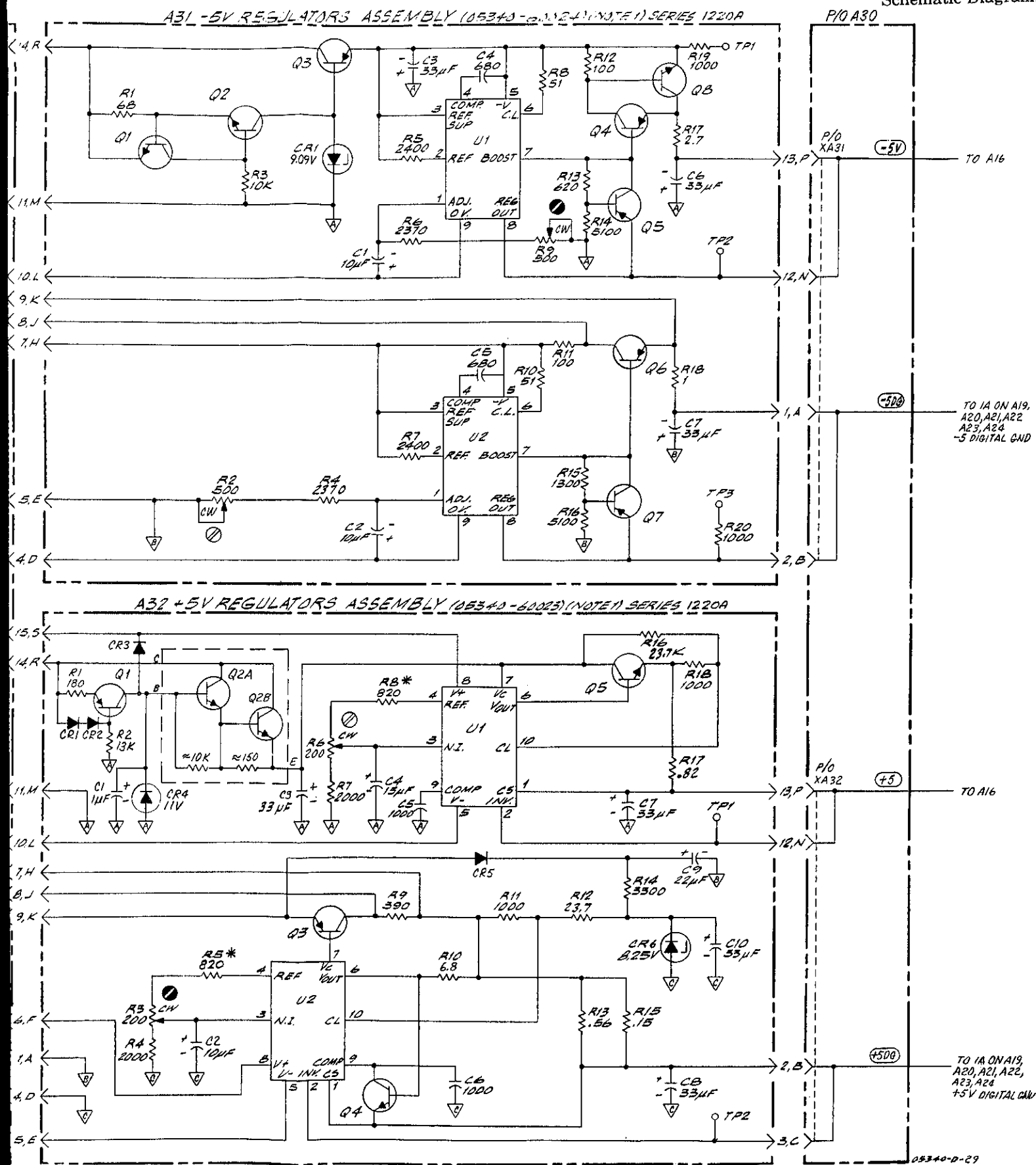
Figure 8-34. A30 Power Supply Motherboard, A31 -5V Regulator Assembly, A32 +5V Regulator Assembly
