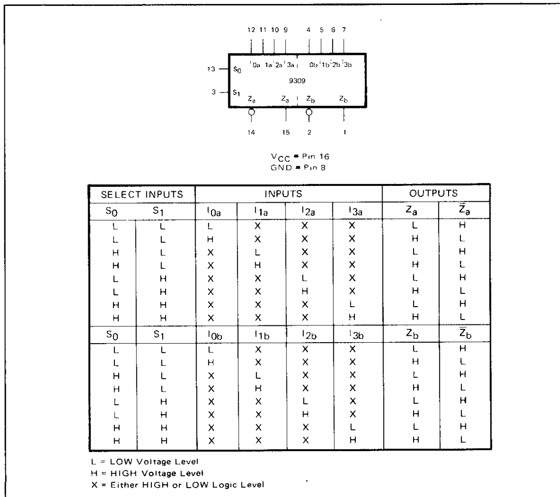
Figure 4-22. Four-Input Multiplexer 1820-0610
