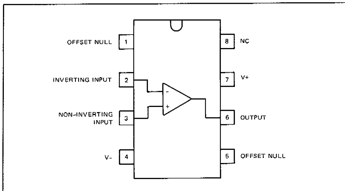
Figure 4-42. Operational Amplifier 1826-0073
