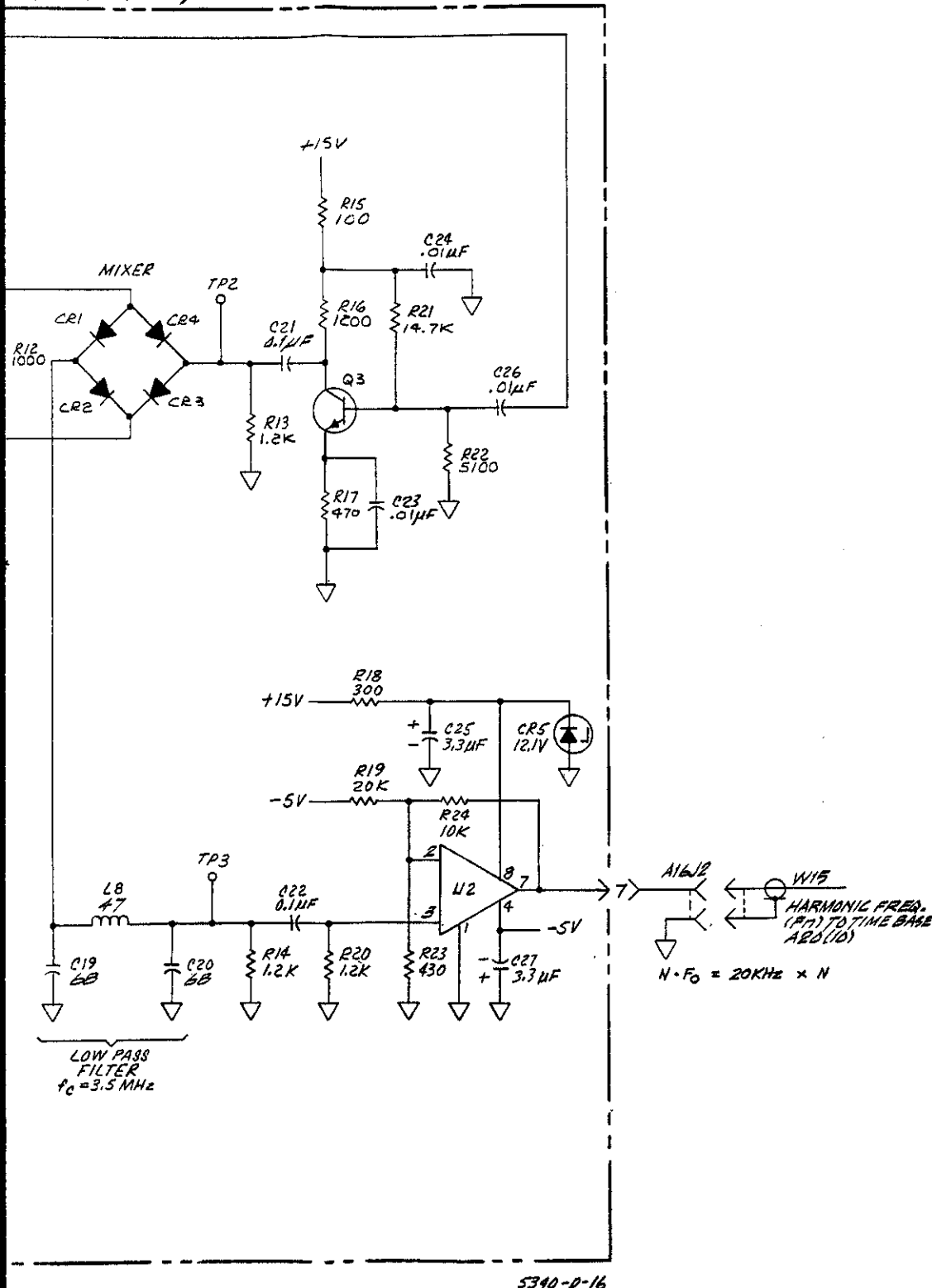
Figure 8-20. A14 Limiter/Amplifier/Mixer Assembly
