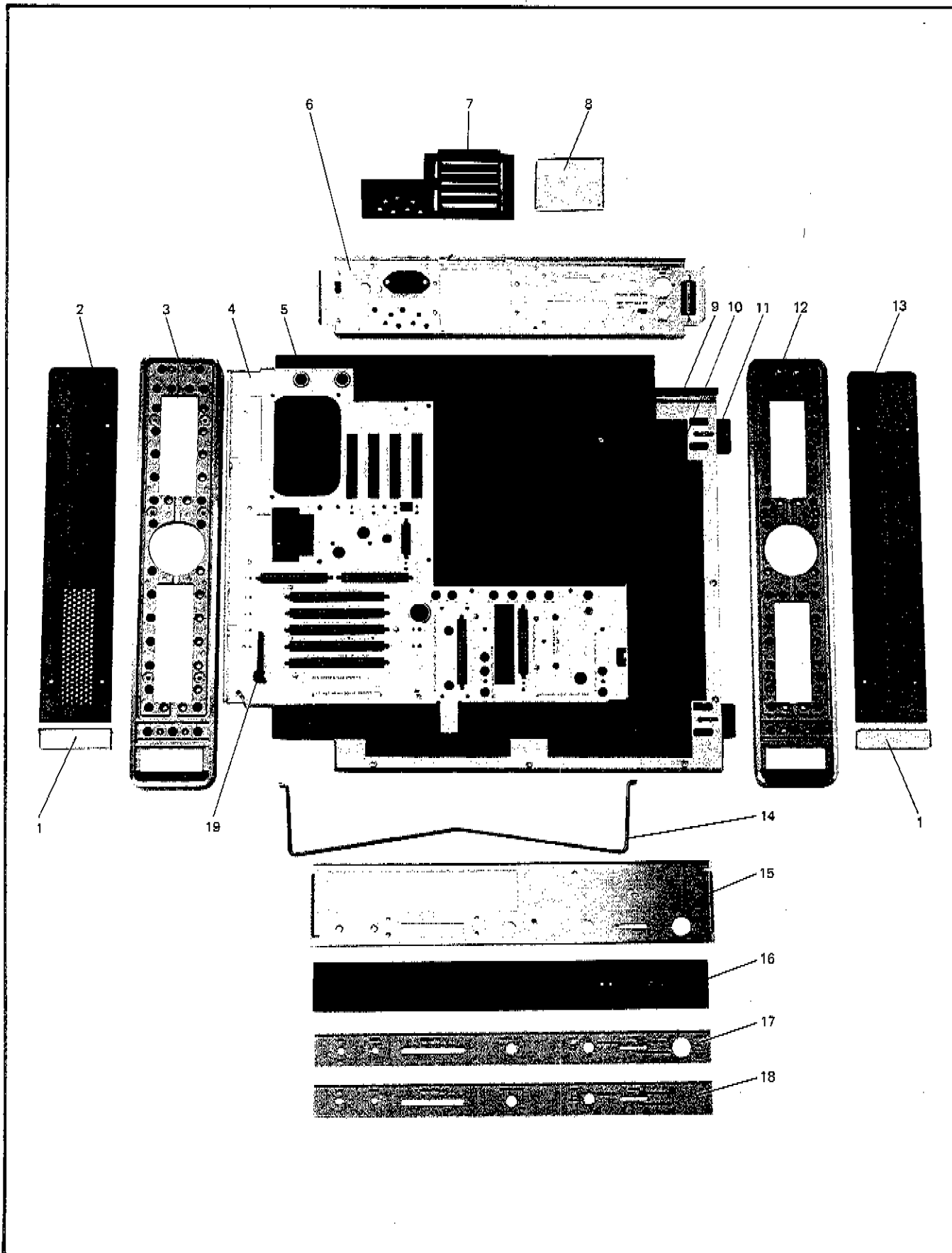
Figure 6-1. 5340A Mechanical Parts
