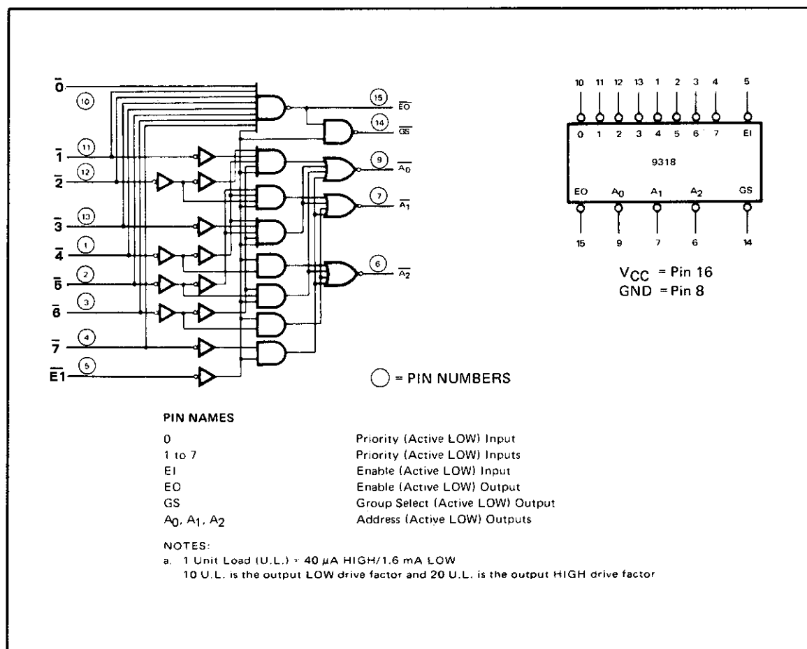
Figure 4-26. Eight-Input Priority Encoder 1820-0657
