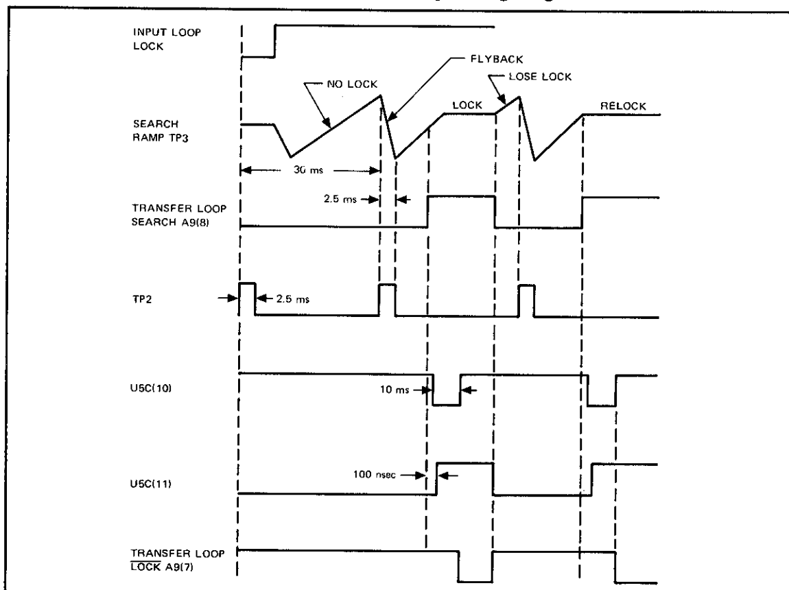
Figure 4-51. Transfer Loop Timing Diagram
