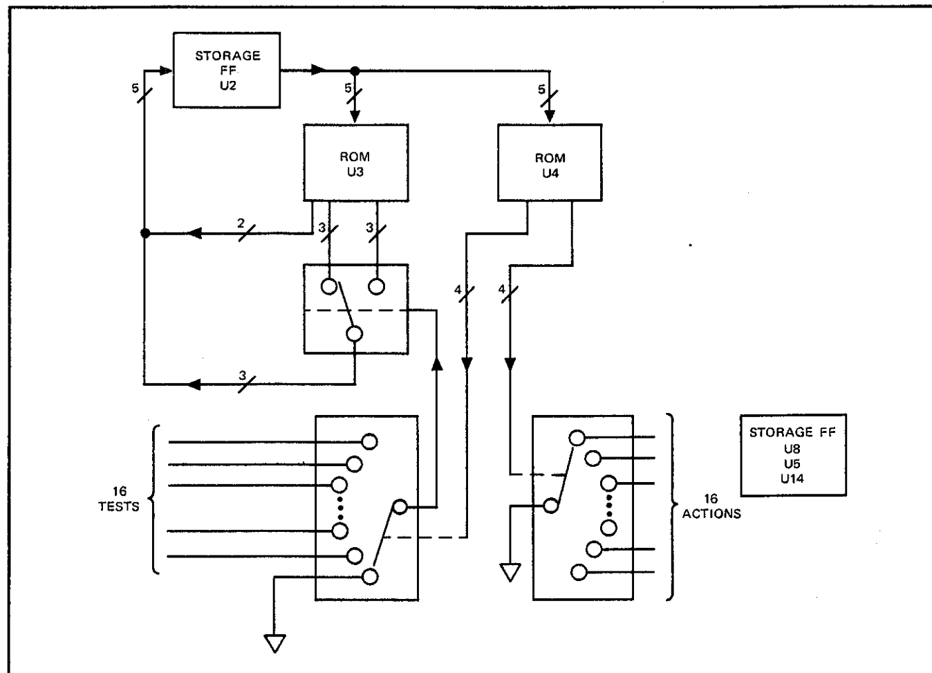
PRESENT-FUTURE ROM U3 (1816-0003) Truth Table
