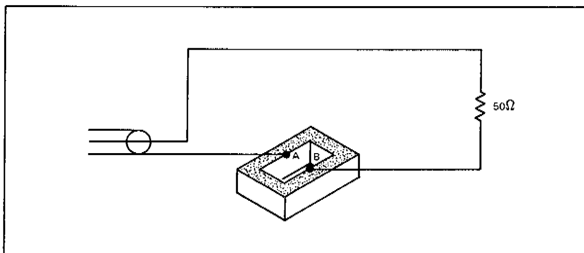
Figure 4-48. Sampler Slot
