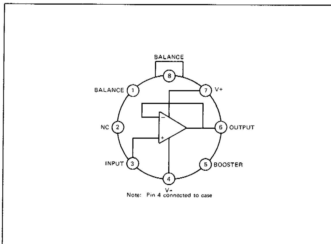
Figure 4-40. Operational Amplifier 1826-0021
