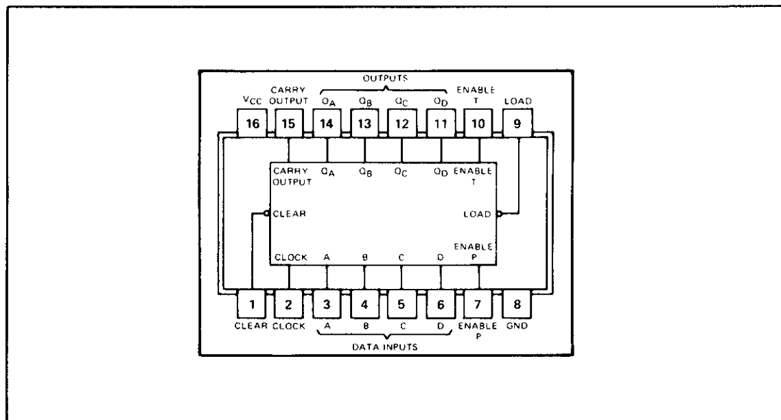
Figure 4-31. Synchronous Four-Bit Counter 1820-0716
