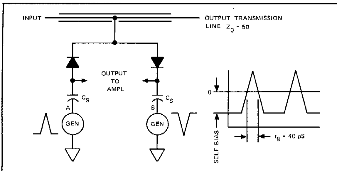
Figure 4-47. Balanced Sampler
