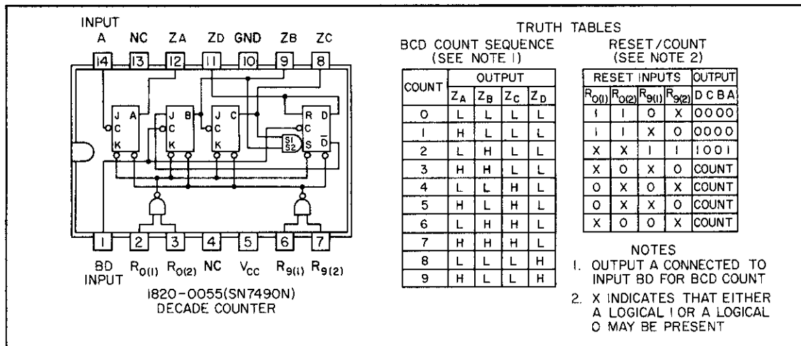
Figure 4-4. Decade Counter 1820-0055
