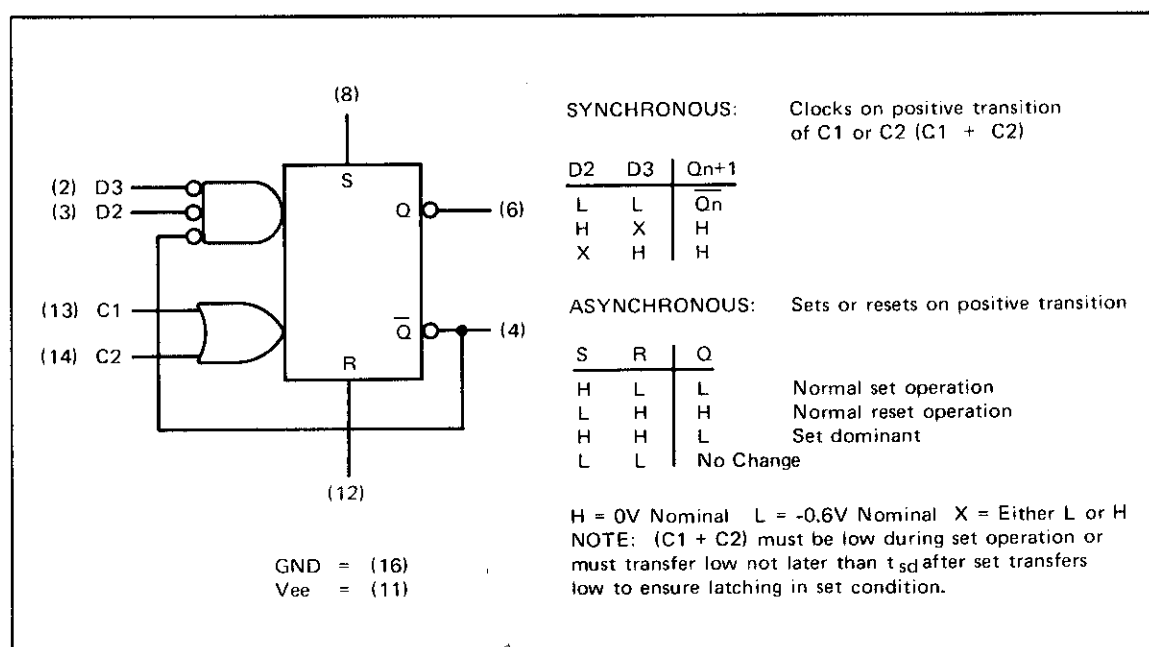
Figure 4-19. EECL High-Speed D-Binary 1820-0557
