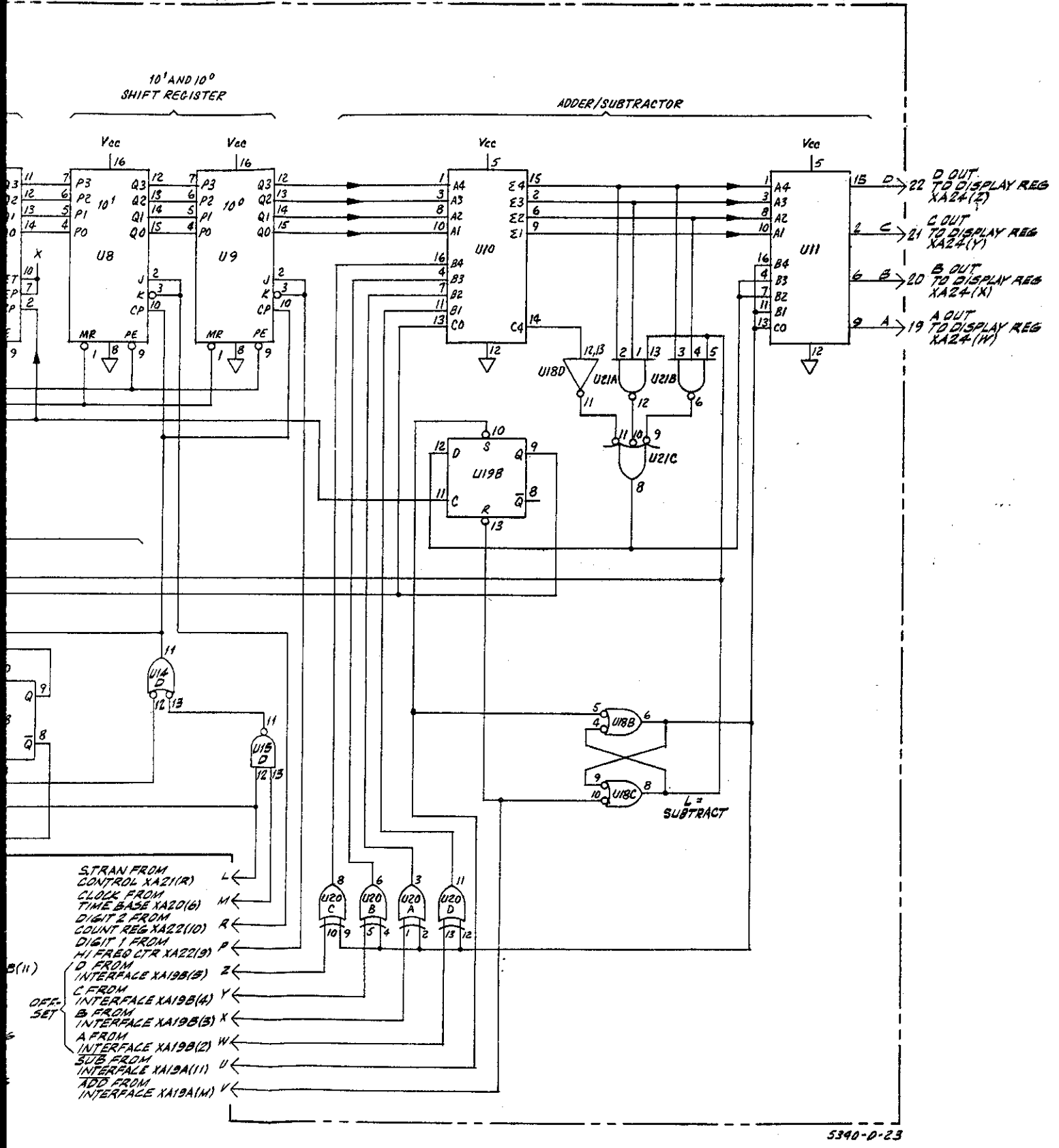
Figure 8-30. A23 Count Register Assembly
