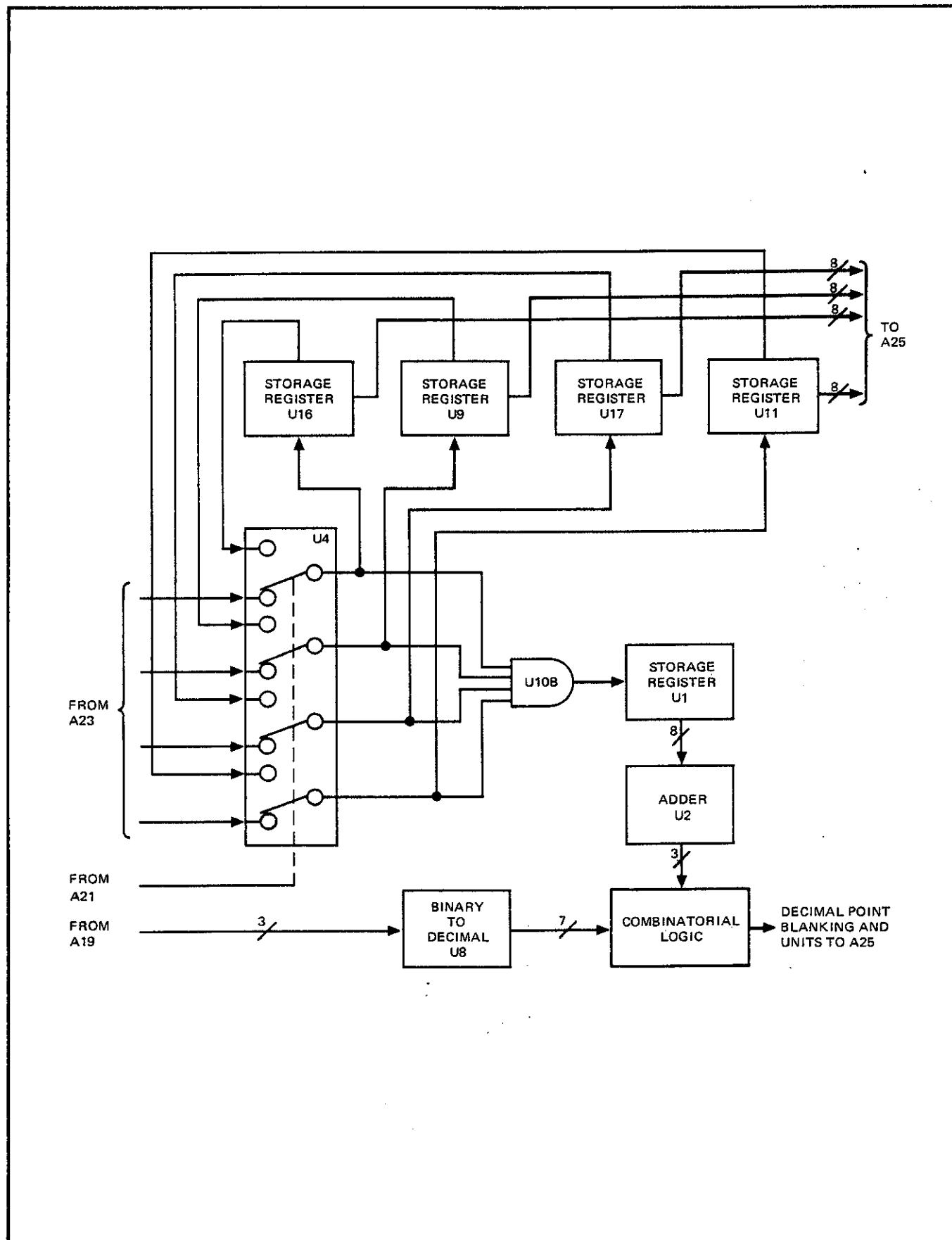
Part of Figure 8-31. A24 Display Register Assembly
