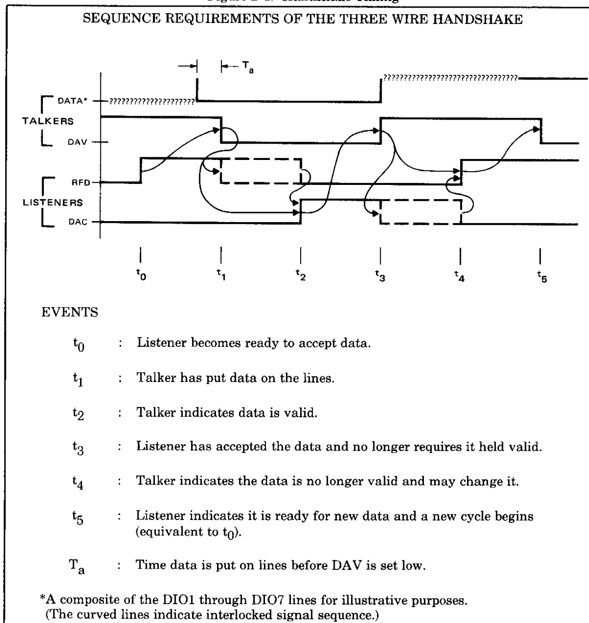
Figure 2-1. Handshake Timing
