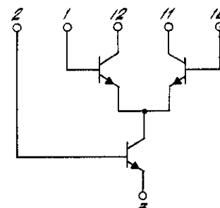
U1A SCHEMATIC DIAGRAM
