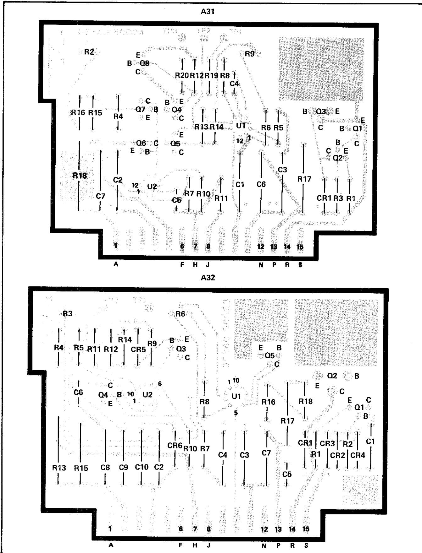
Part of Figure 8-34. A30, A31, and A32
