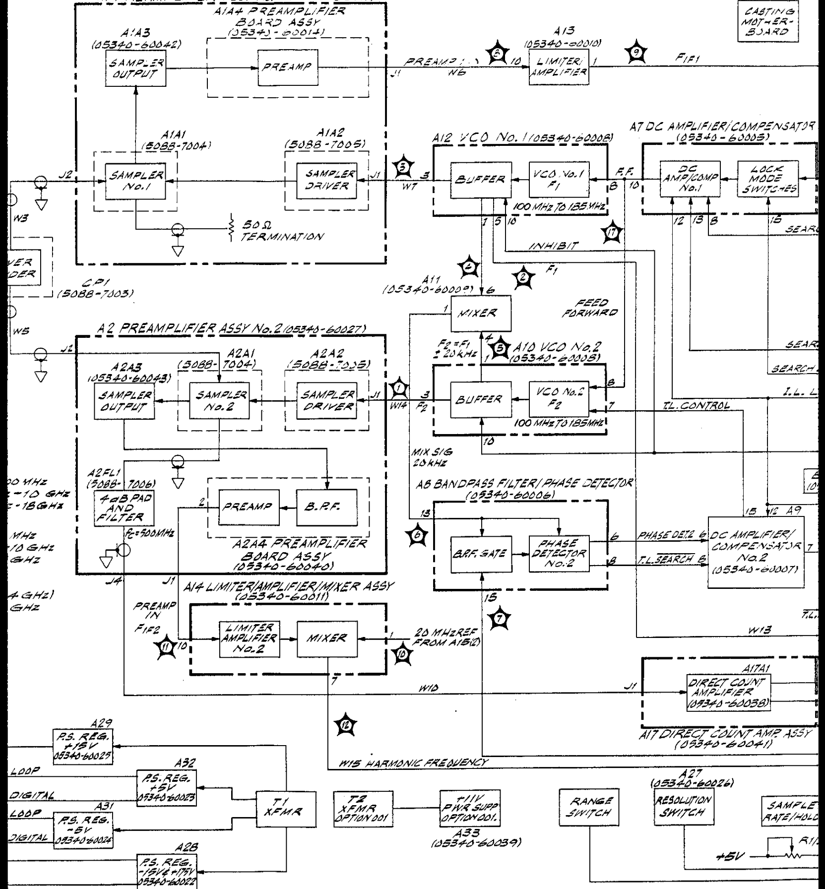
Fig 8-65 ut 3084 A1 PREAMPLIFIER ASSY No.1 (05340-60017)
