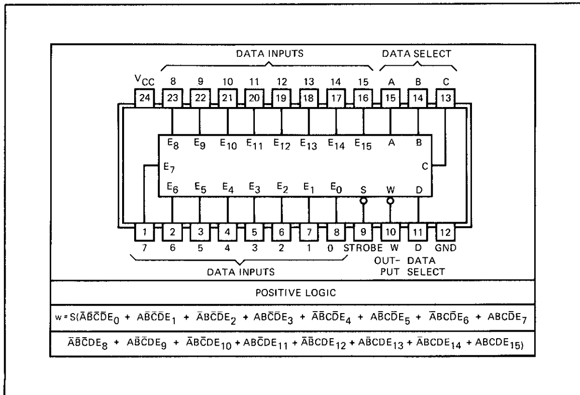
Figure 4-25. Data Selectors/Multiplexers 1820-0640
