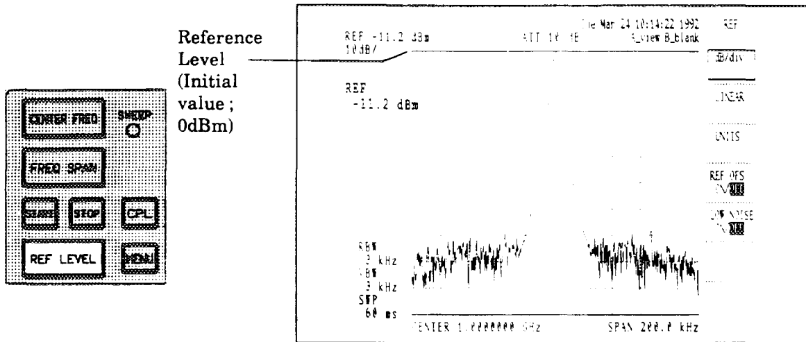
Figure 5.1-5 Reference Level
