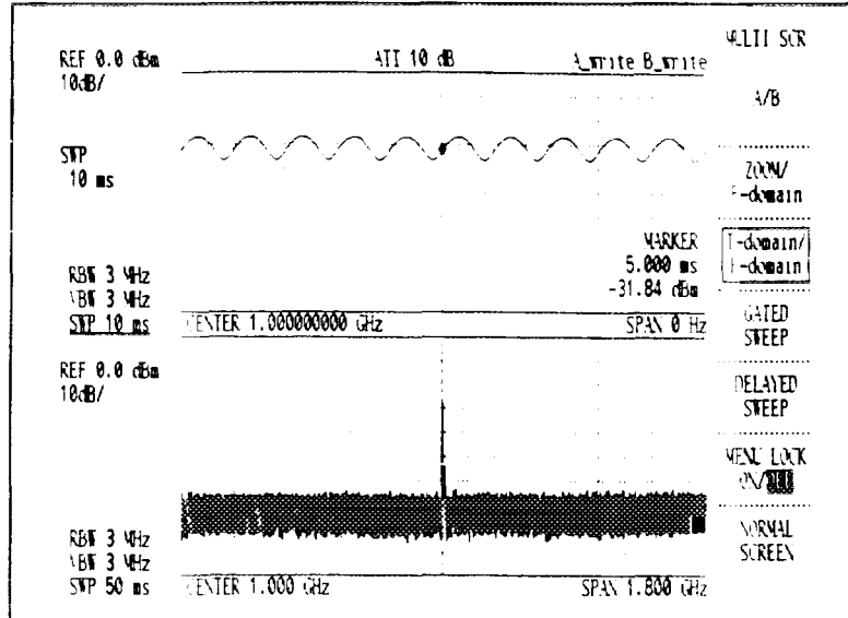
Figure 7 - 9 TIME-domain/F-domain Mode
