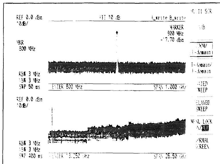
Figure 7 - 5 ZOOM/F-domain Mode
