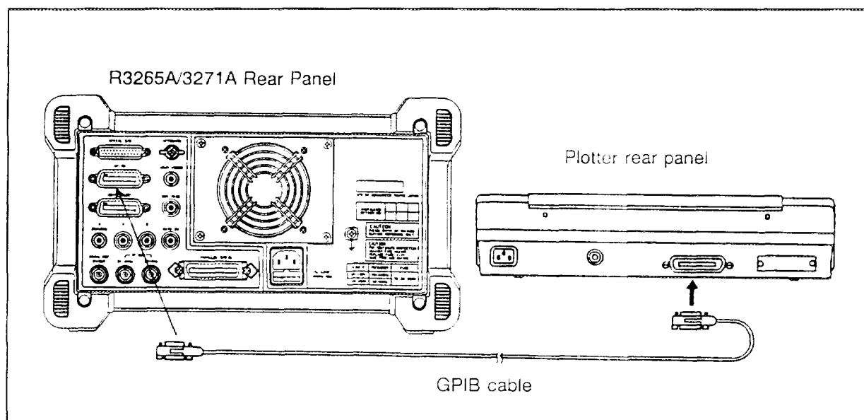
Figure 5.9-1 Plotter Connection
