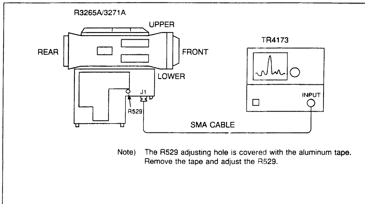
Figure 5-17 Sampler Synthe Adjustment
