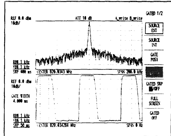
Figure 7 - 20 Measurement Screen in GATED/TIME-domain Mode
