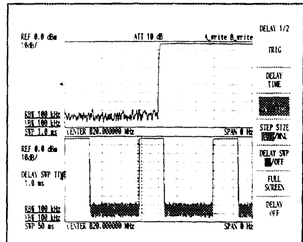
Figure 7 - 28 Measurement Screen in DELAYED/TIME-domain Mode
