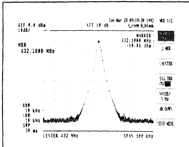
Figure 3-6 Peak Marker
