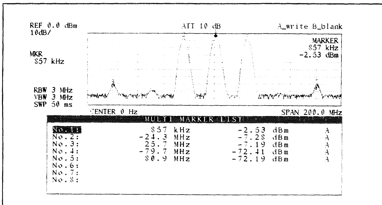
Figure 5.15-3 Printing Precision Set at LOW (Normal Size)
