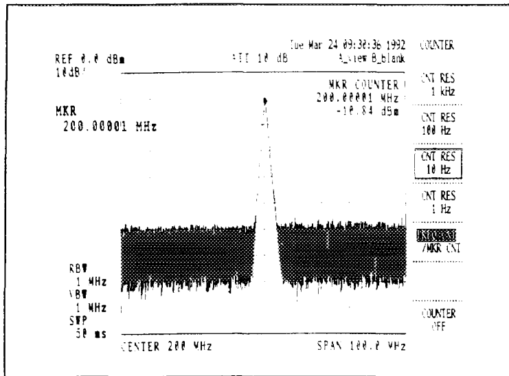
Figure 4-2 Measuring Frequency in Frequency Counter Mode
