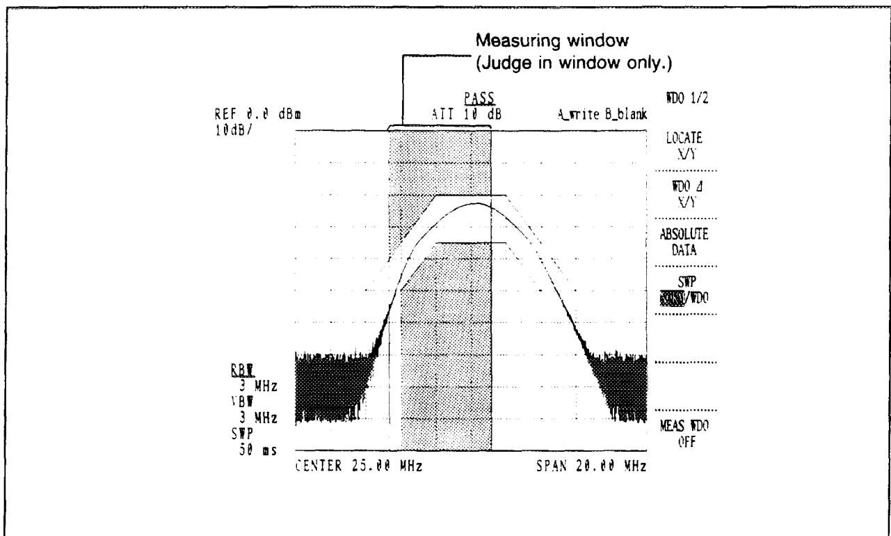
Figure 5.20-3 Judgment Range when Measuring Window is ON
