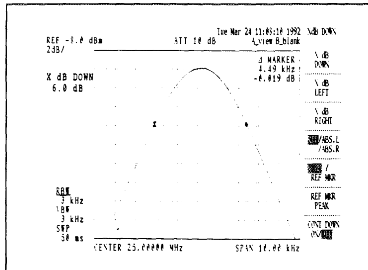
Figure 5.3-4 X dB Down
