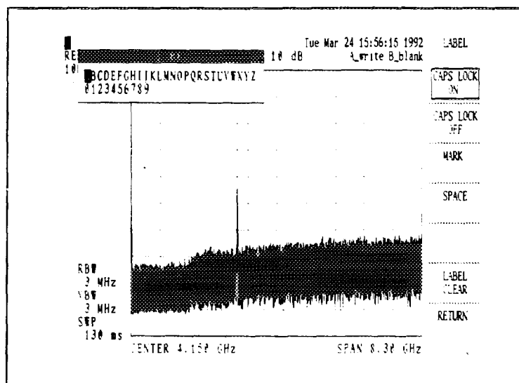
Figure 5.10-1 Label Display
