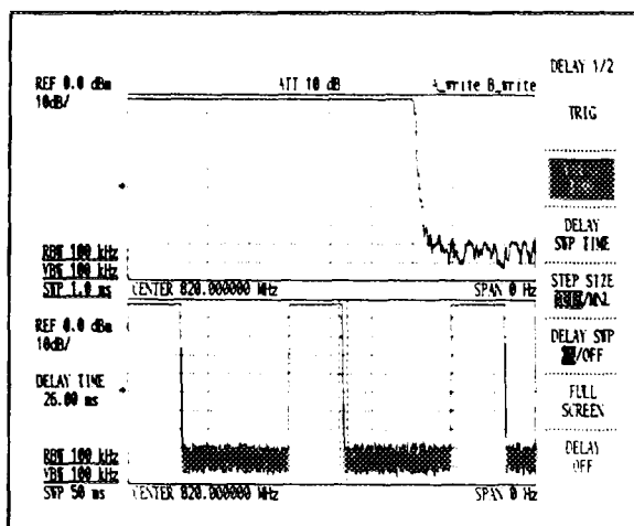
Figure 7 - 24 Split-Screen Display (DELAYED SWEEP ON)
