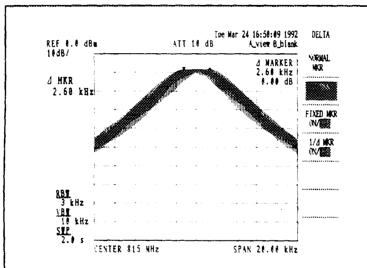
Figure 4-12 FM Signal With Small \Delta f_{\text{peak}}
