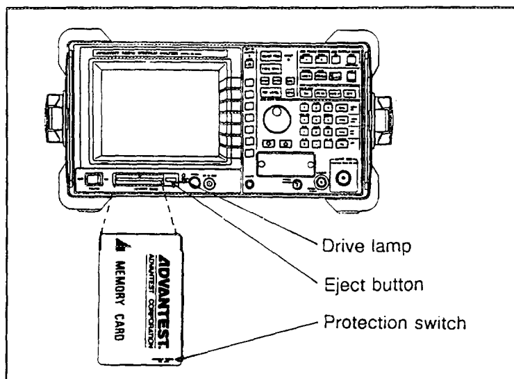
Figure 5.5-2 Inserting and Removing the Memory Card
