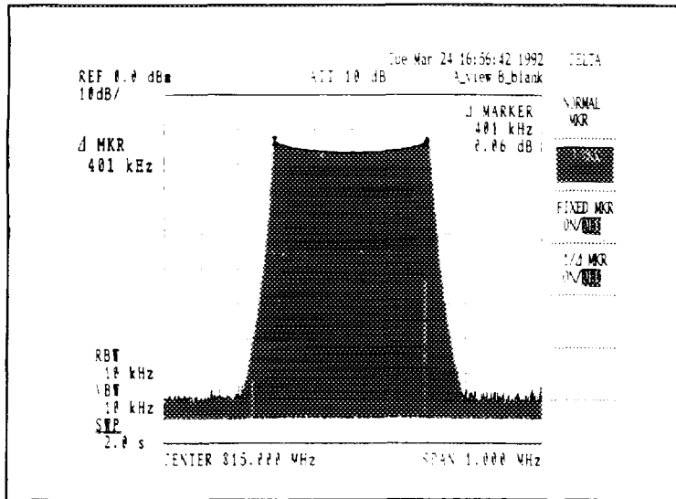
Figure 4-13 FM Signal With Large \Delta f_{\text{peak}}
