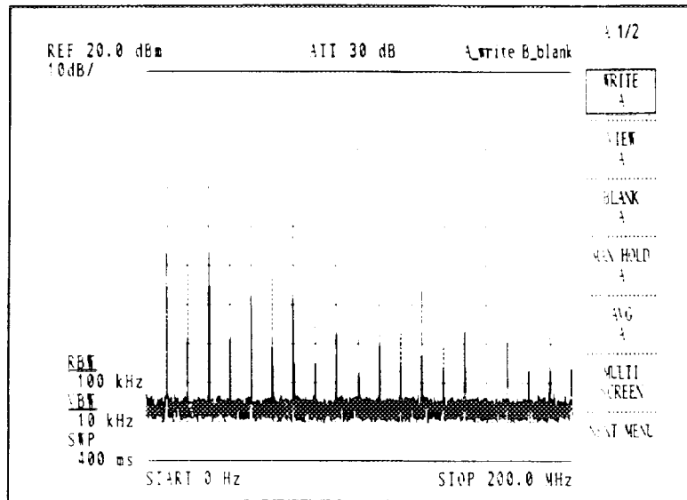
Figure 7 - 6 Full-Screen Display (ZOOM/F-domain Mode)
