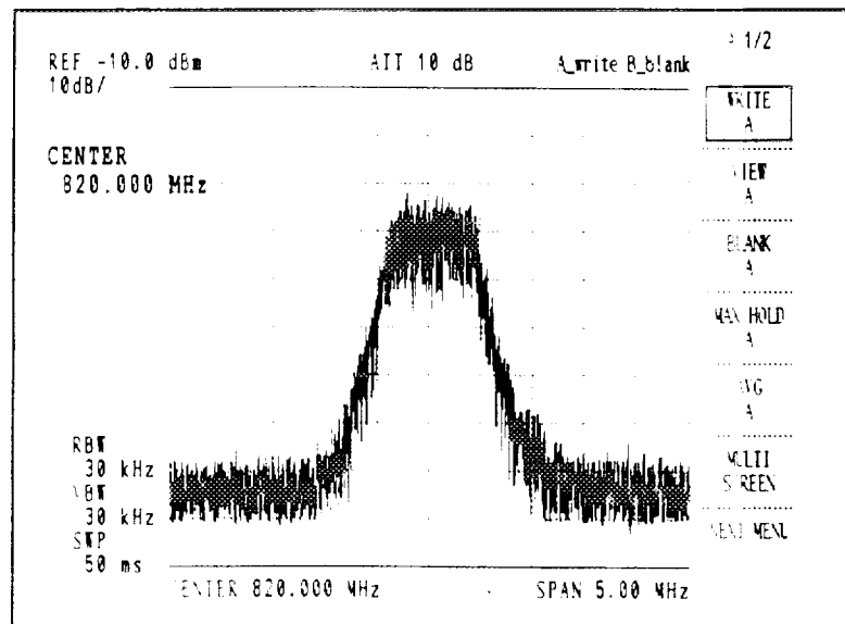
Figure 7 - 2 Full-Screen Display
