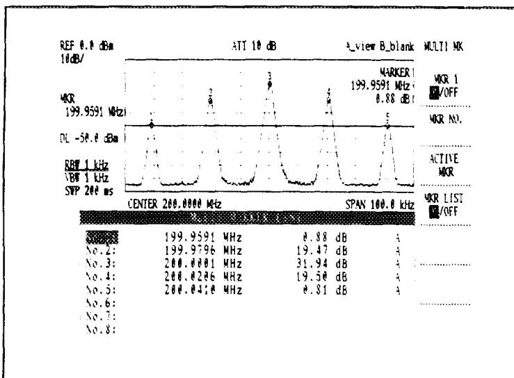
Figure 5.3-18 Example Listing with a Display Line
