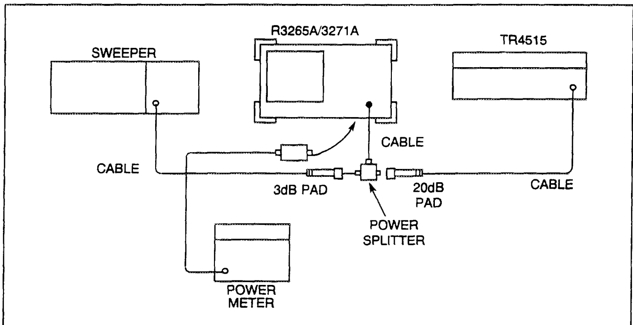
Figure 4-10 Gain Compression Test Setup
