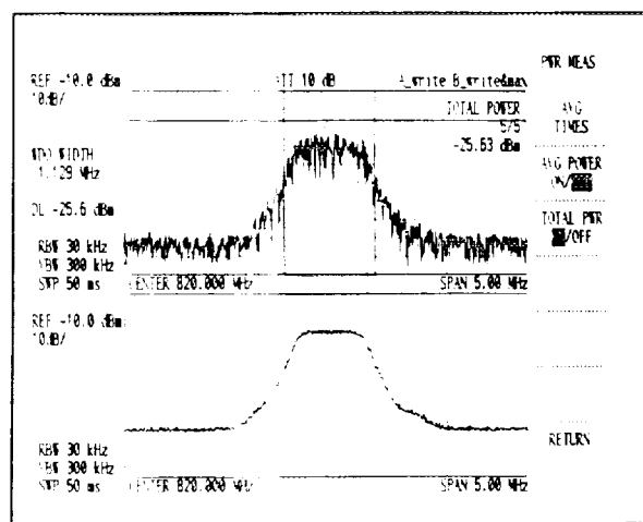
Figure 7 - 4 Measurement Screen in A/B Mode
