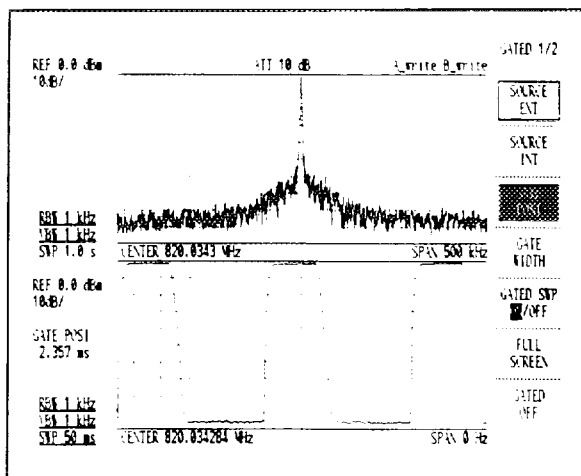
Figure 7 - 16 Split-Screen Display (GATED SWEEP ON)
