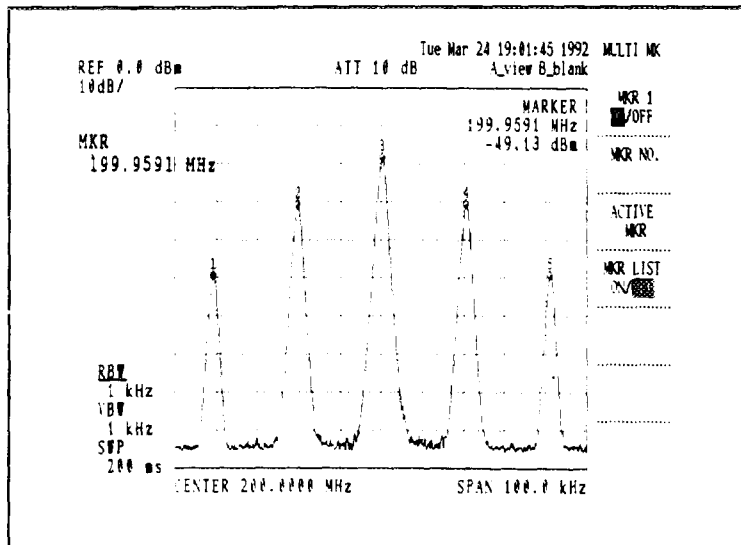
Figure 5.3-15 Multi Marker Display
