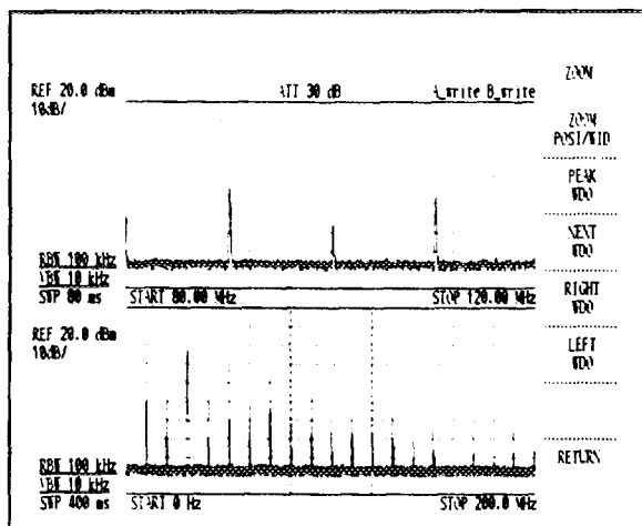
Figure 7 - 7 Split-Screen Display (ZOOM/F-domain Mode)
