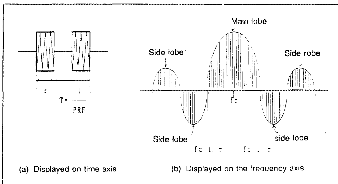
Figure 4-16 Pulse-modulated Signal
