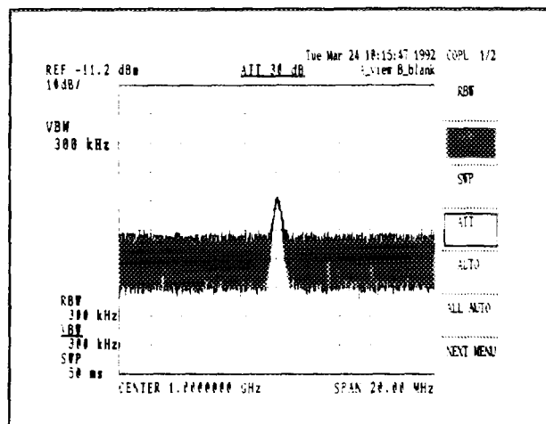
Figure 5.1-7 VBW = 300kHz
