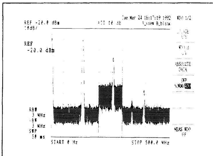
Figure 5.14-2 Partial Sweep Within a Window
