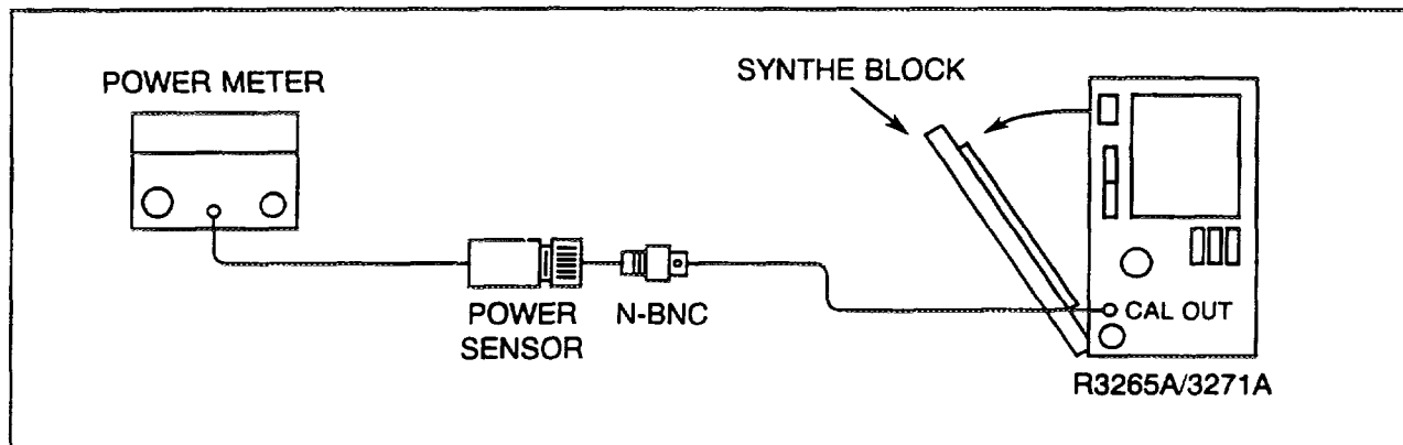
Figure 5-13 Calibrator Amplitude Adjustment Setup
