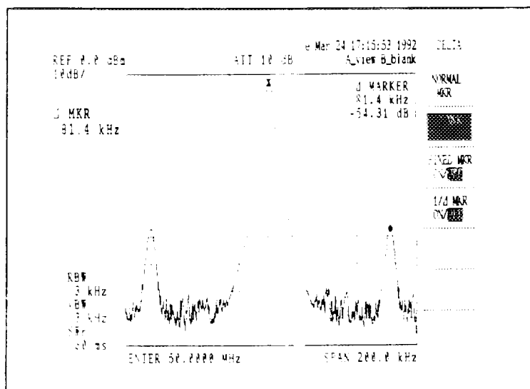
Figure 5.3-2 Delta Marker
