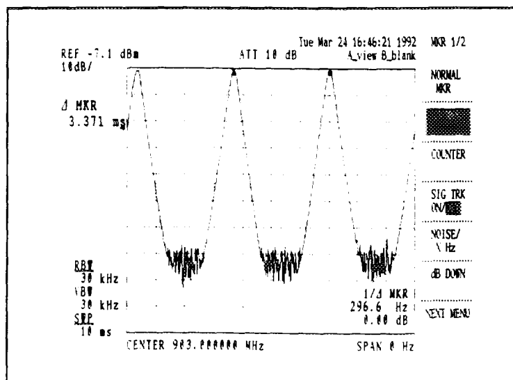
Figure 4-10 FM signal With Low Modulation Frequency
