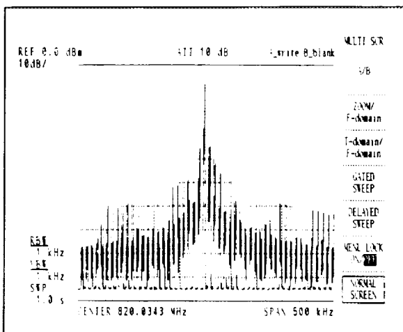
Figure 7 - 14 Full-Screen Display (GATED SWEEP OFF)
