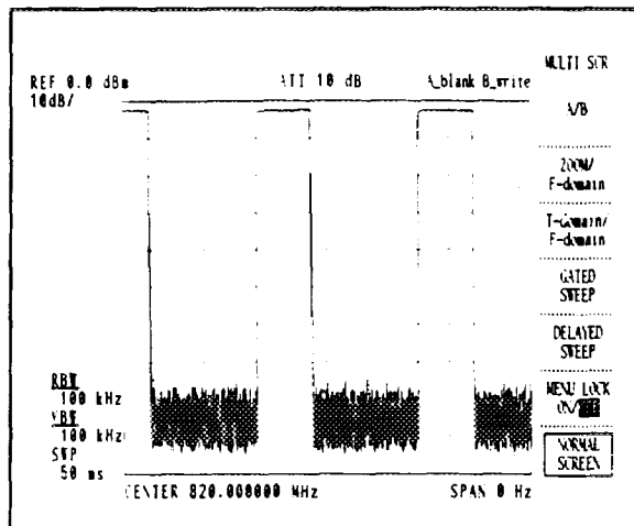
Figure 7 - 22 Full-Screen Display (DELAYED SWEEP OFF)
