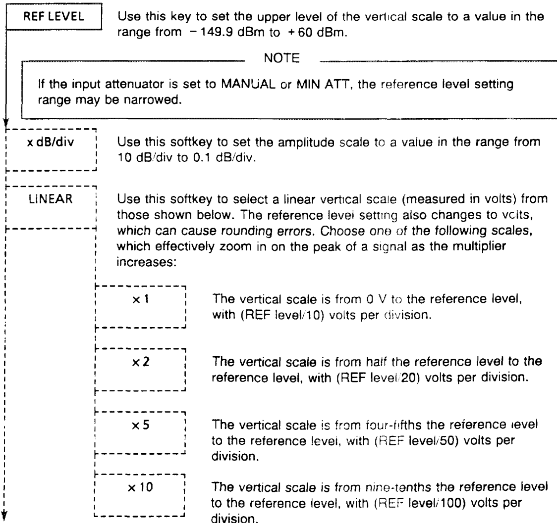
Figure 5.1-5 Reference Level
