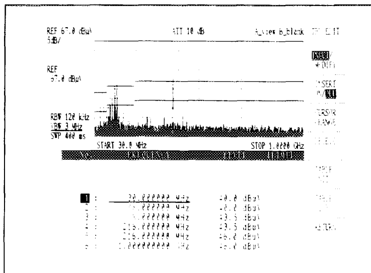
Figure 5.11-2 Entering a Limit Line
