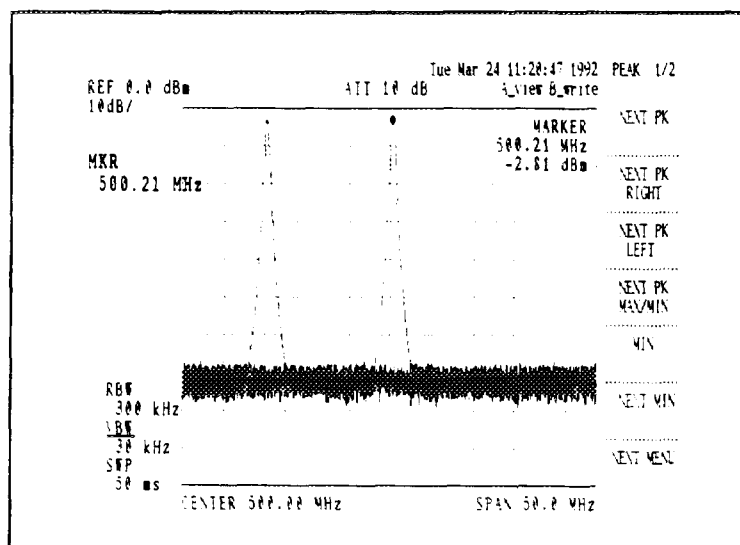
Figure 5.3-14 Setting MKR → CF
