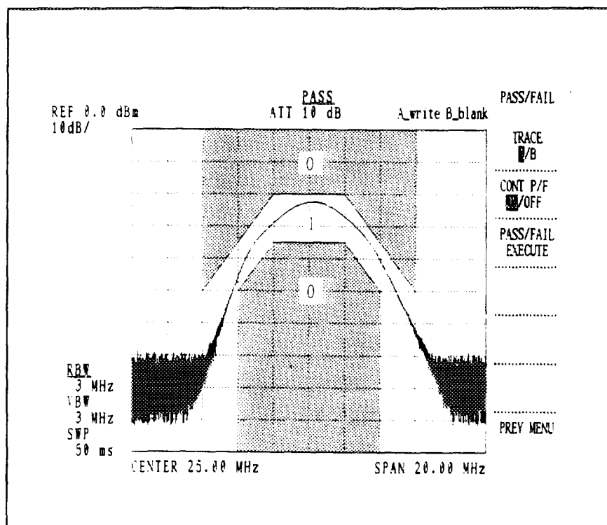
Figure 5.20-4 PASS/FAIL returned value
