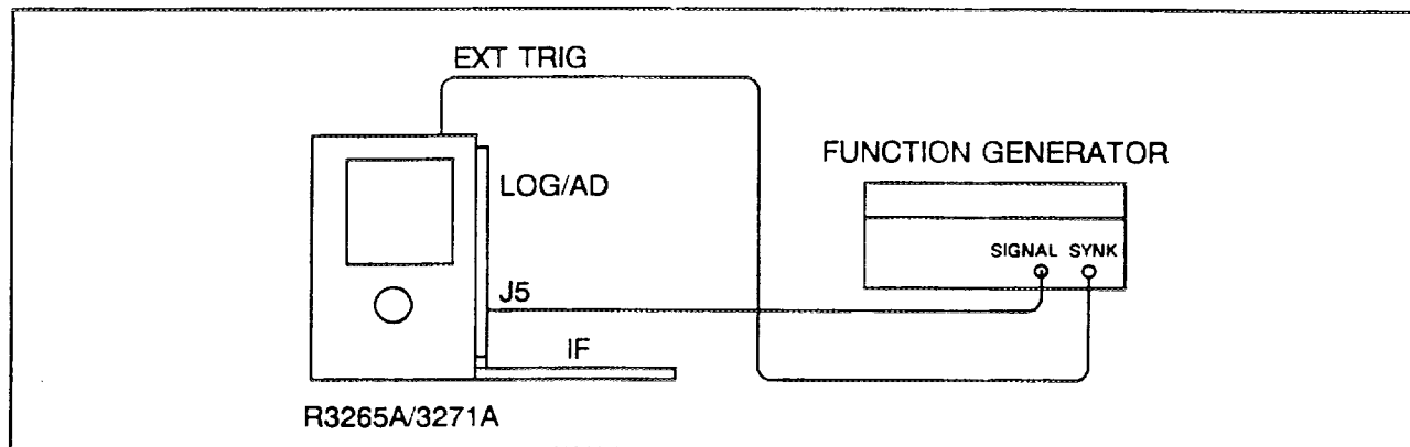
Figure 5-3 Setup for Slope Detector Adjustment
