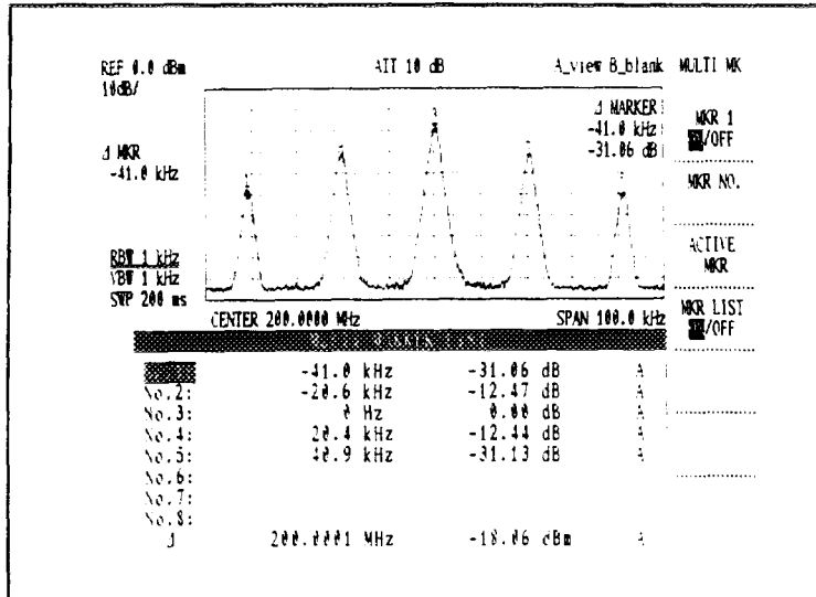
Figure 5.3-17 An Example of Delta Marker Listing
