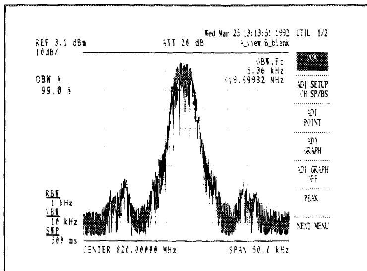
Figure 4-17 Measuring the OBW
