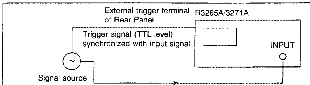
Figure 7 - 21 DELAYED SWEEP Connection Diagram
