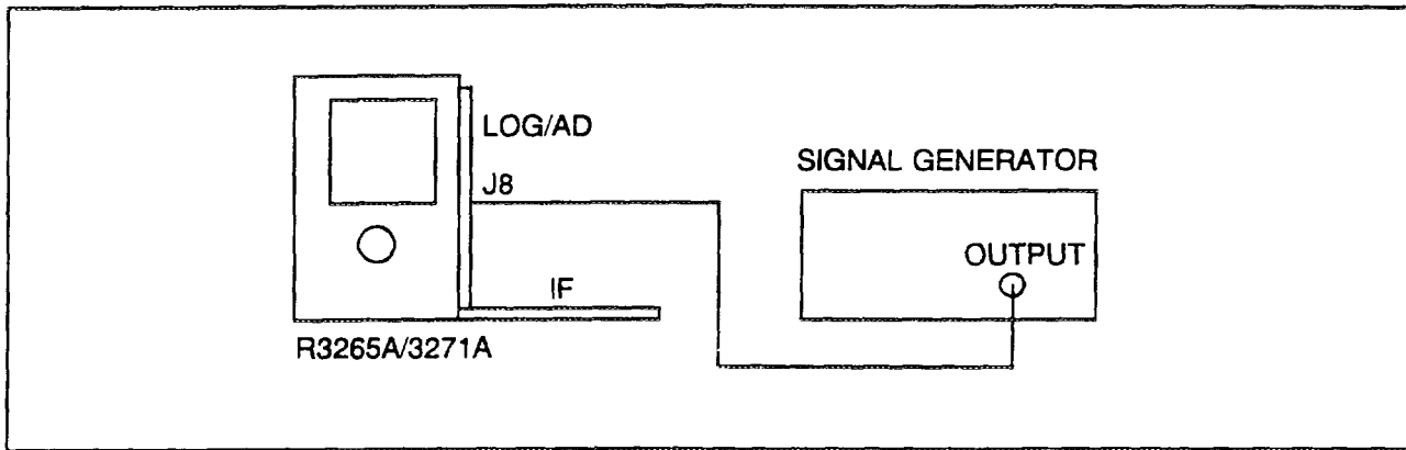
Figure 5-5 Adjustment Setup
