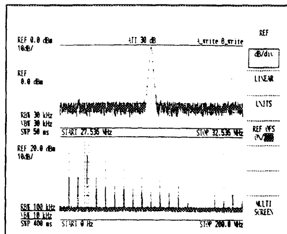
Figure 7 - 8 Measurement Screen in ZOOM/F-domain Mode
