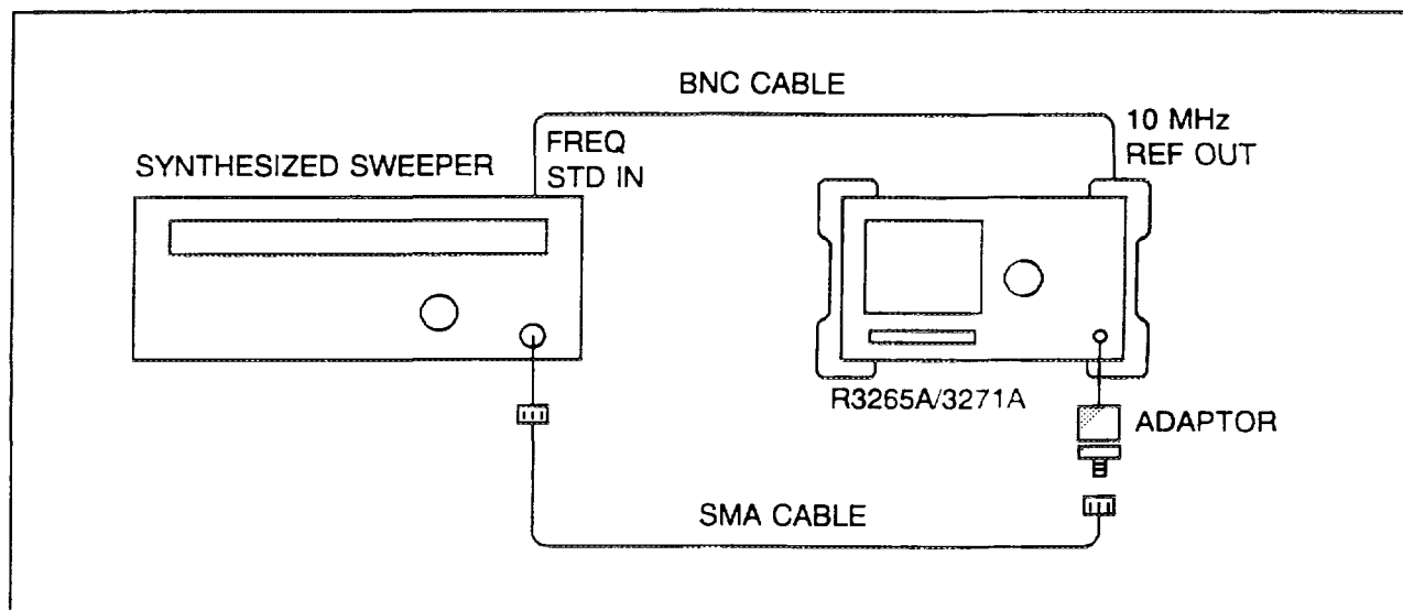
Figure 5-16 SPAN Adjustment Setup
