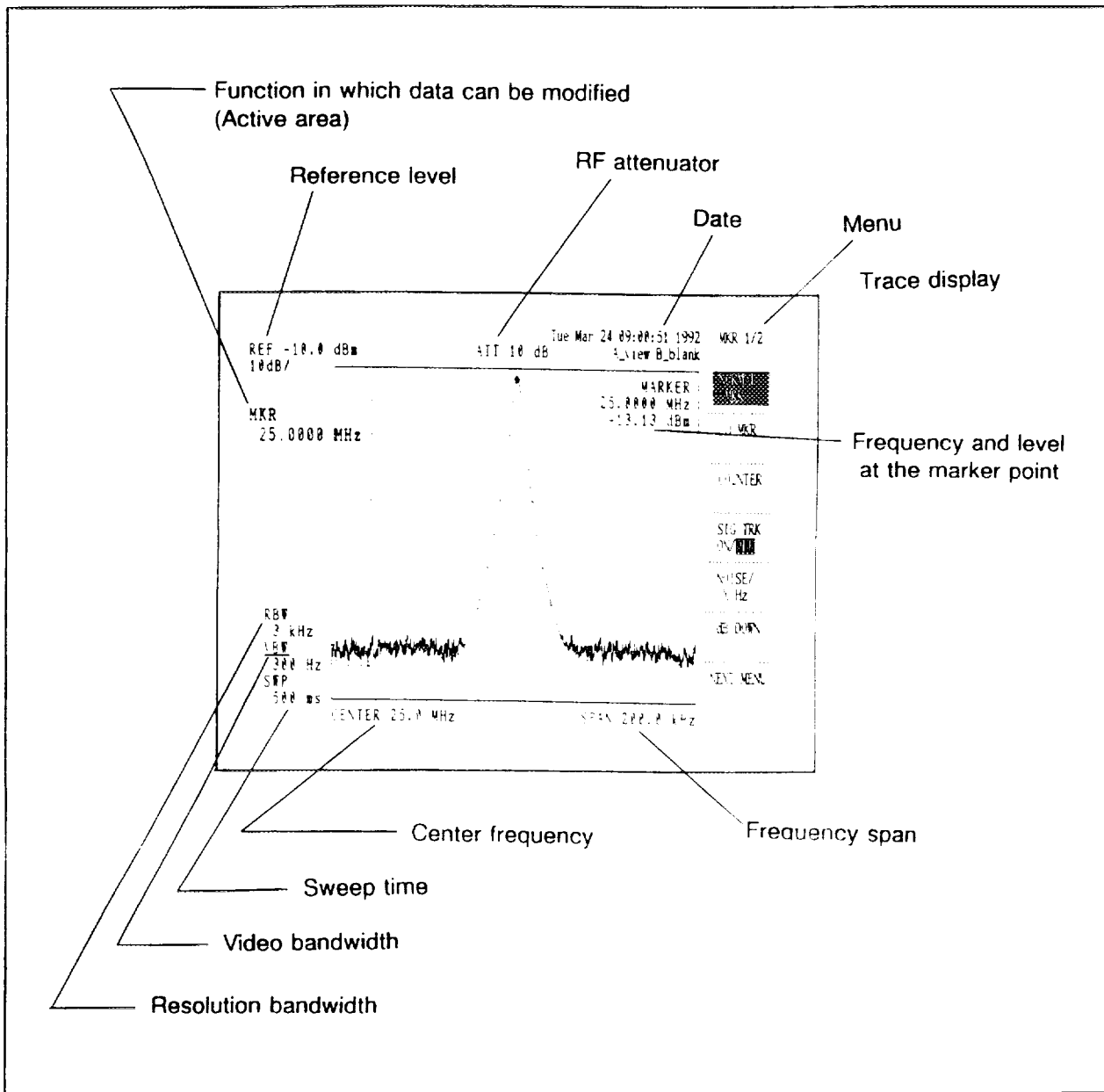
Figure 3-1 Display
