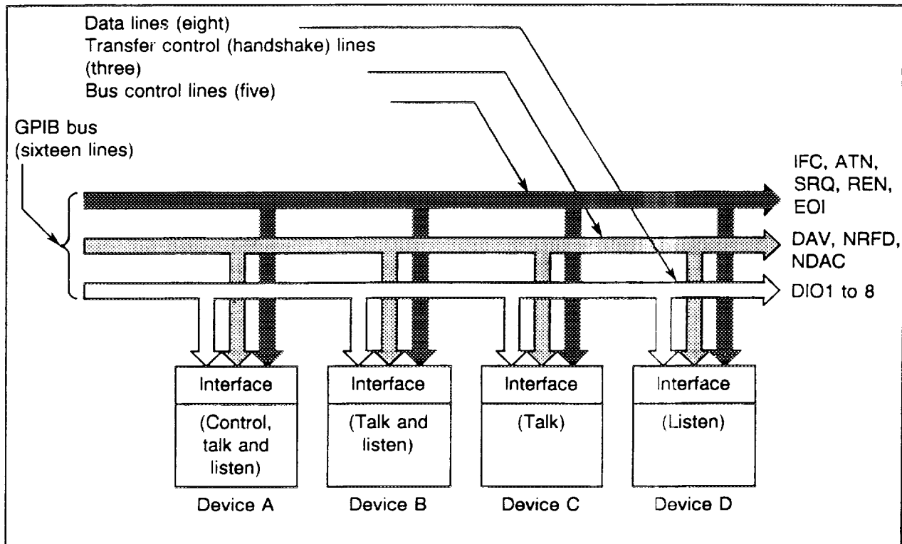
Figure 6.1-1 GPIB Bus Configuration
