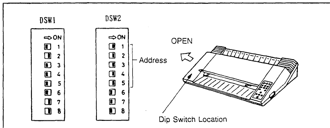
Figure 5.9-2 Example Dip Switch Setting
