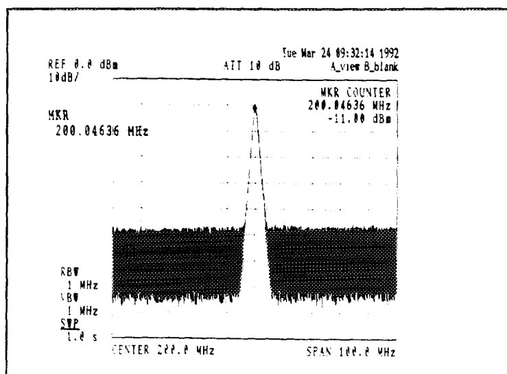
Figure 4-3 Measuring Frequency in Marker Counter Mode
