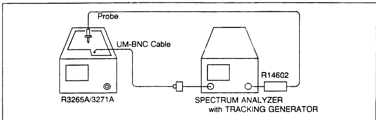
Figure 5-6 LC Filter Adjustment Setup
