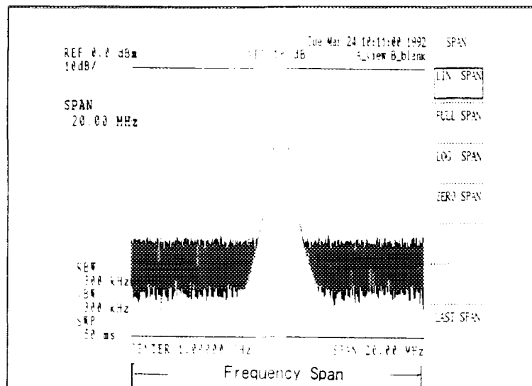
Figure 5.1-3 Frequency Span
