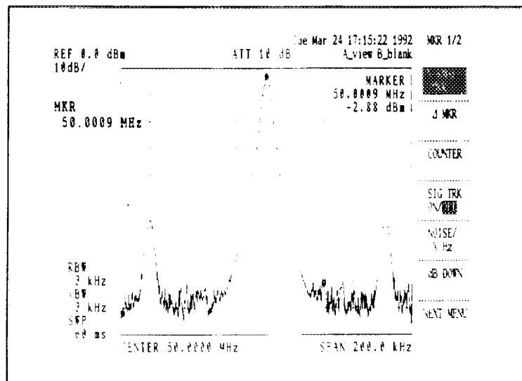
Figure 5.3-1 Normal Marker
