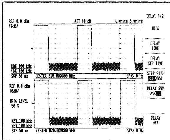
Figure 7 - 27 Split-Screen Display (DELAYED/TIME-domain Mode)
