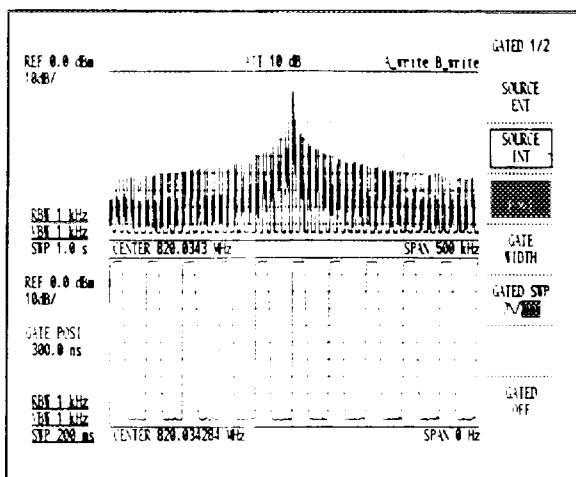
Figure 7 - 15 Split-Screen Display (GATED SWEEP OFF)
