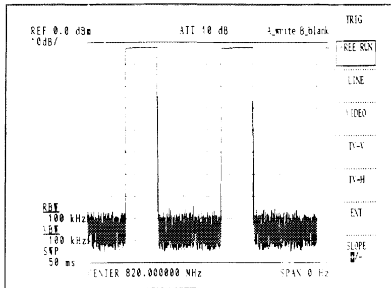
Figure 7 - 26 Full-Screen Display
