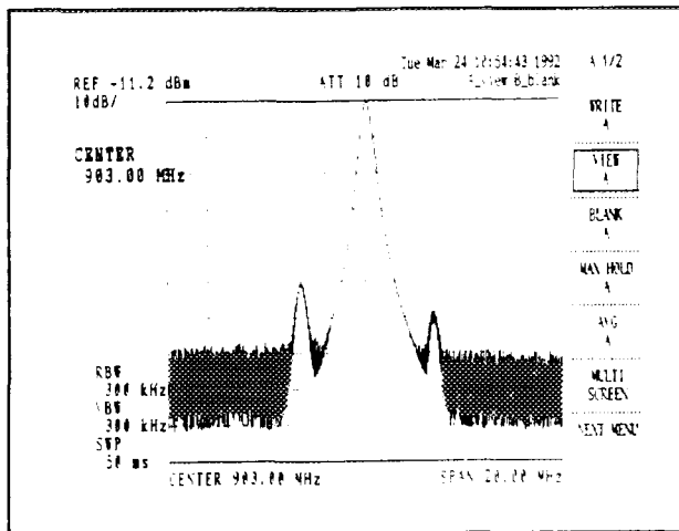
Figure 5.2-3 AVG = None
