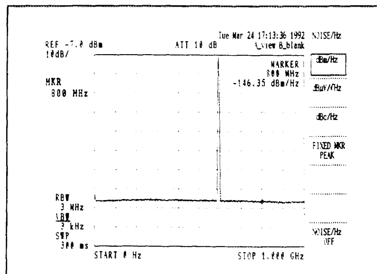
Figure 5.3-3 Noise/Hz Level Measurement
