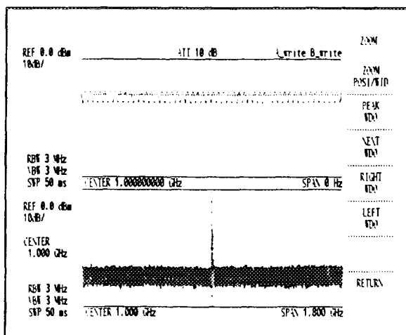
Figure 7 - 11 Split-Screen Display (TIME-domain/F-domain Mode)
