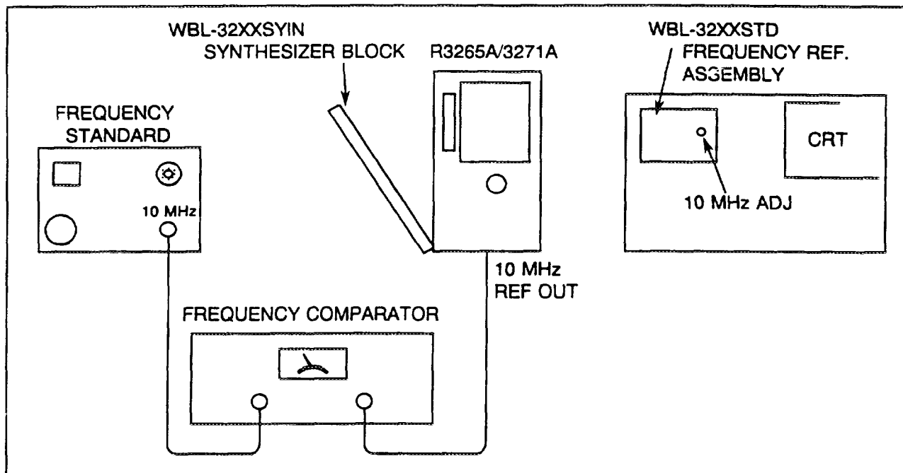
Figure 5-15 10 MHz Reference Crystal Oscillator Adjustment
