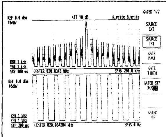
Figure 7 - 19 Split-Screen Display (GATED/TIME-domain Mode)
