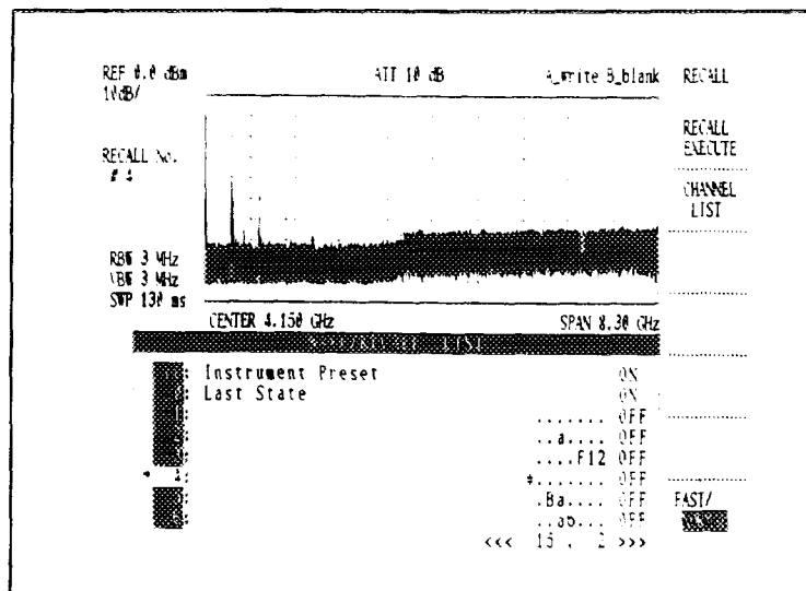
Figure 5.6-7 Recall Data List
