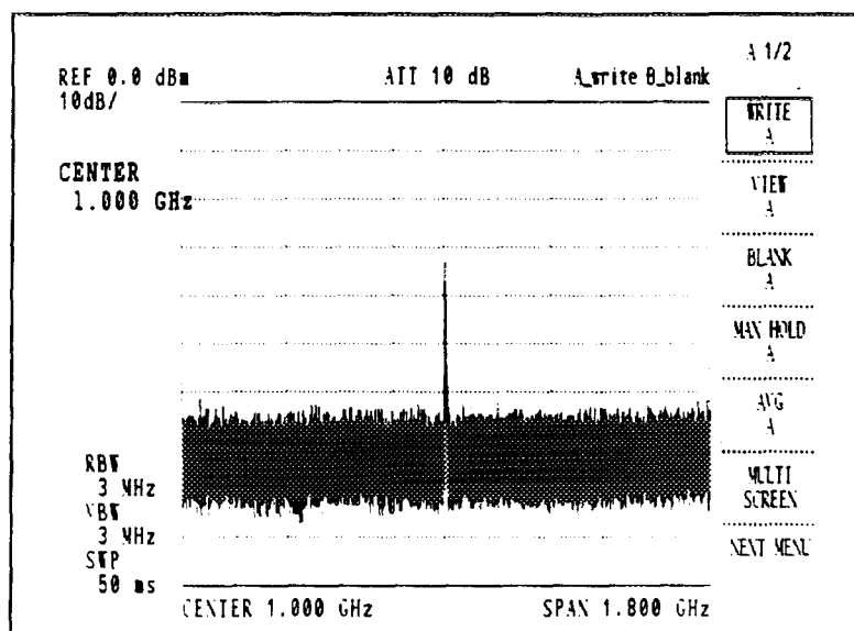
Figure 7 - 10 Full-Screen Display (TIME-domain/F-domain Mode)
