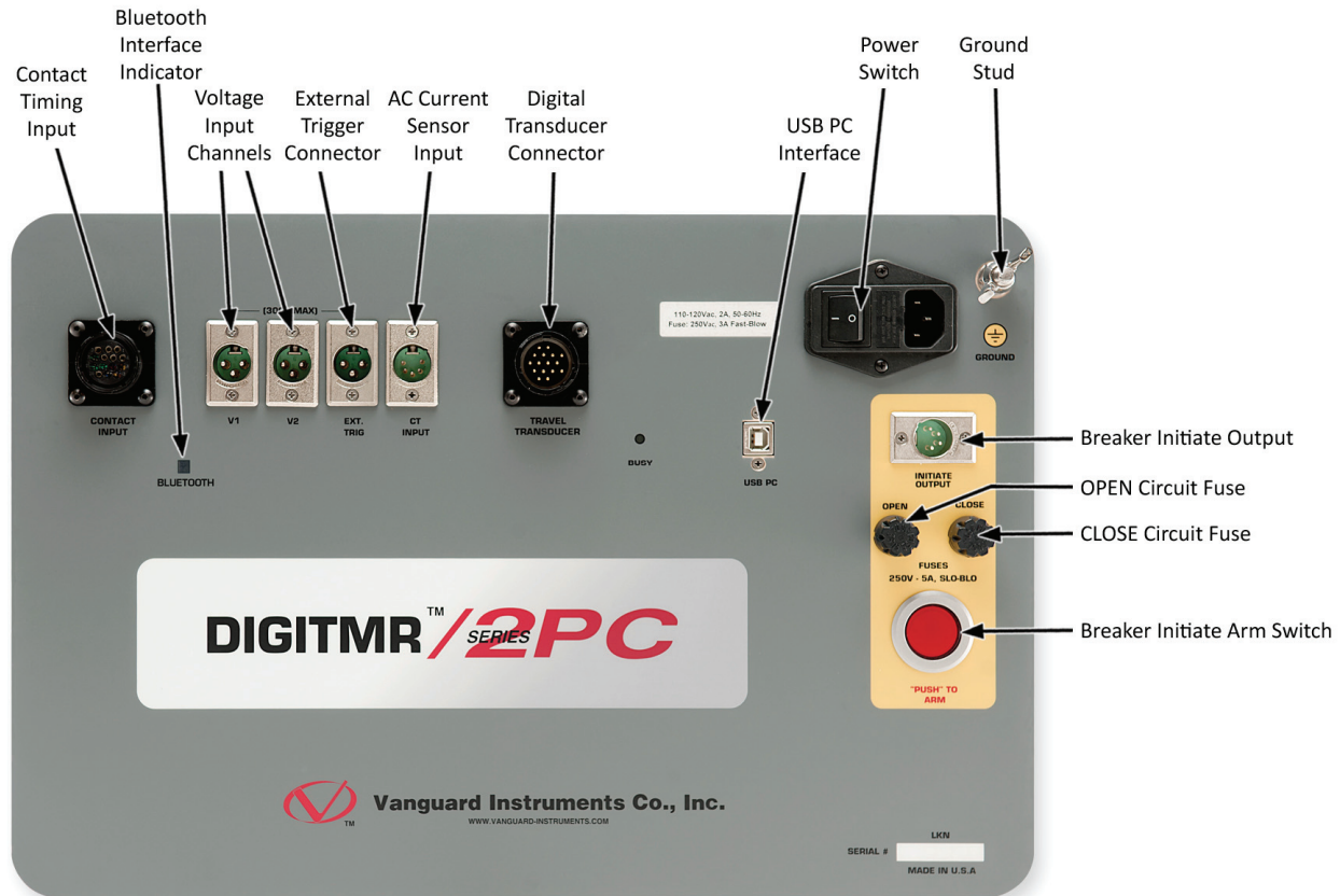
Figure 1. DigiTMR S2 PC Controls and Indicators
