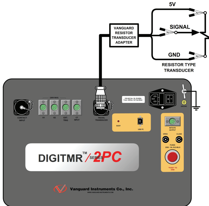
Figure 10. Typical Resistor Type Transducer Connection
