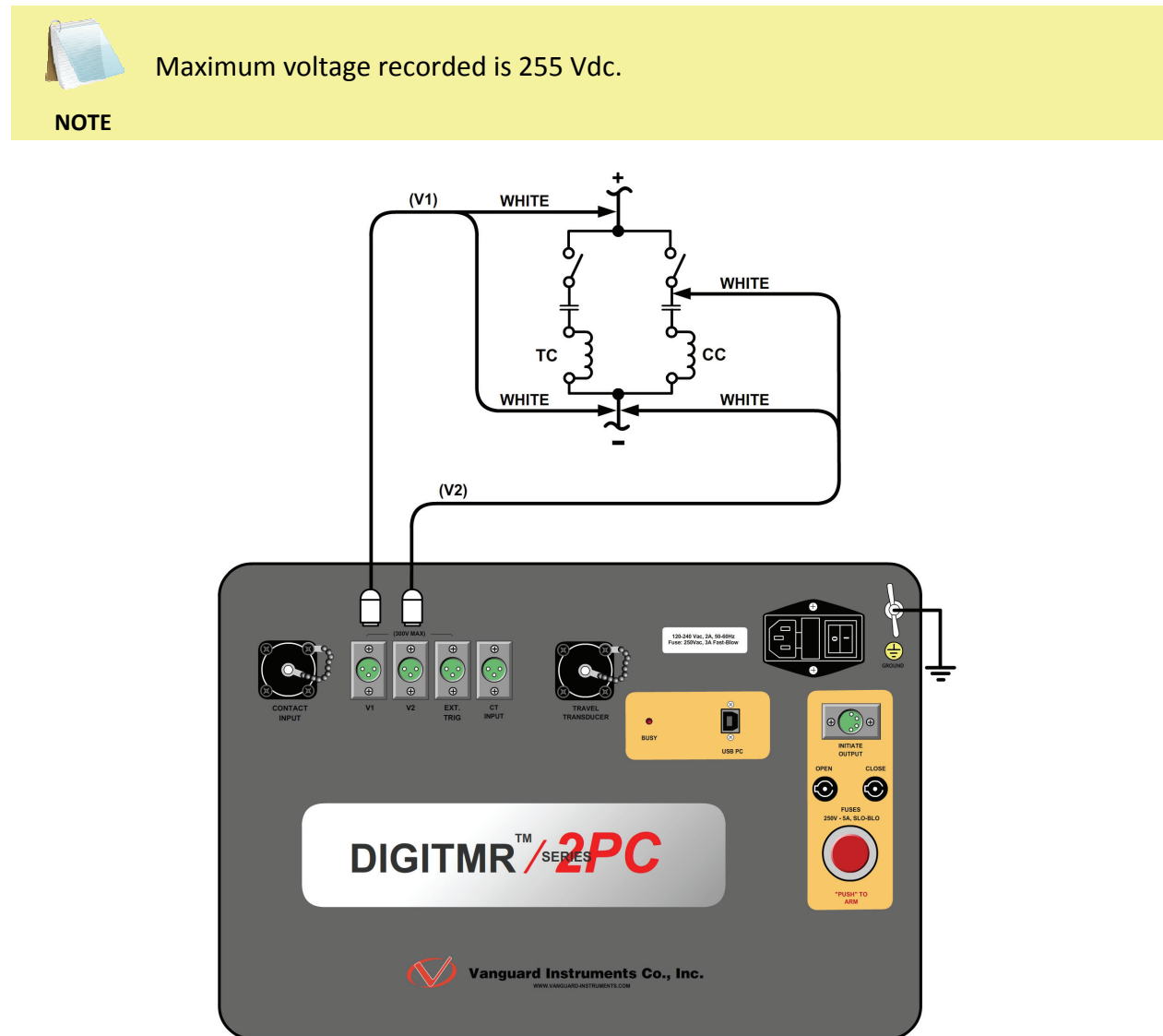
Figure 5. Analog and Digital Voltage Monitoring Cable Connections
