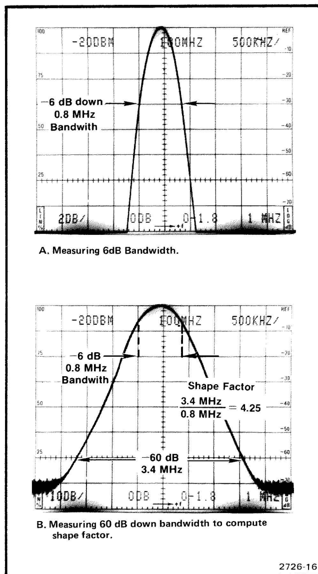
Fig. 3-5. Displays that illustrate how bandwidth and shape factor are determined.
