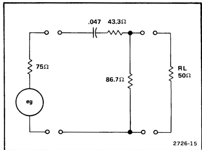
Fig. 3-10. Circuit of a 75 \Omega to 50 \Omega matching pad (ac coupled).
