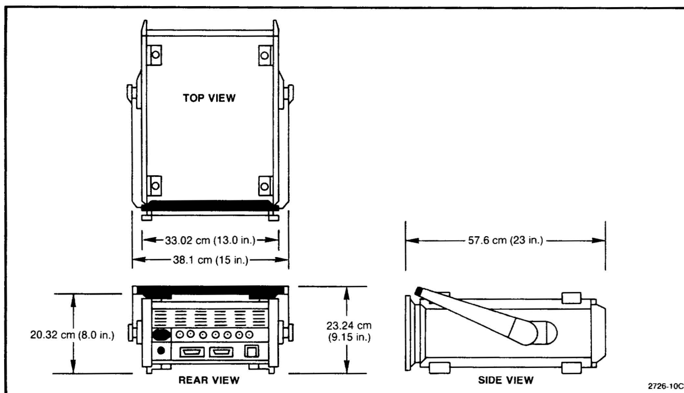
Fig. 1-2. Dimensions.
