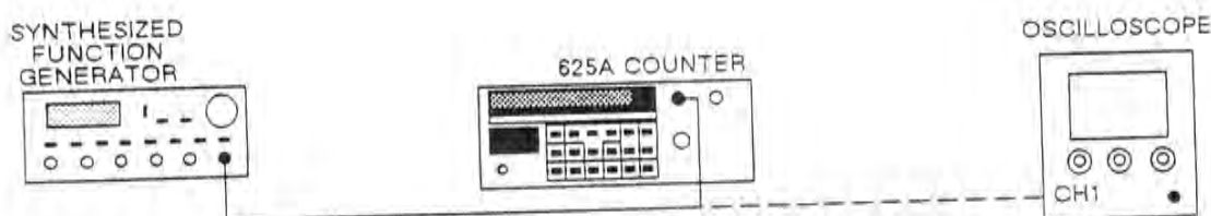
Figure 8-1. Band 1 Range and Sensitivity Test Setup (10 Hz to 10 MHz).
