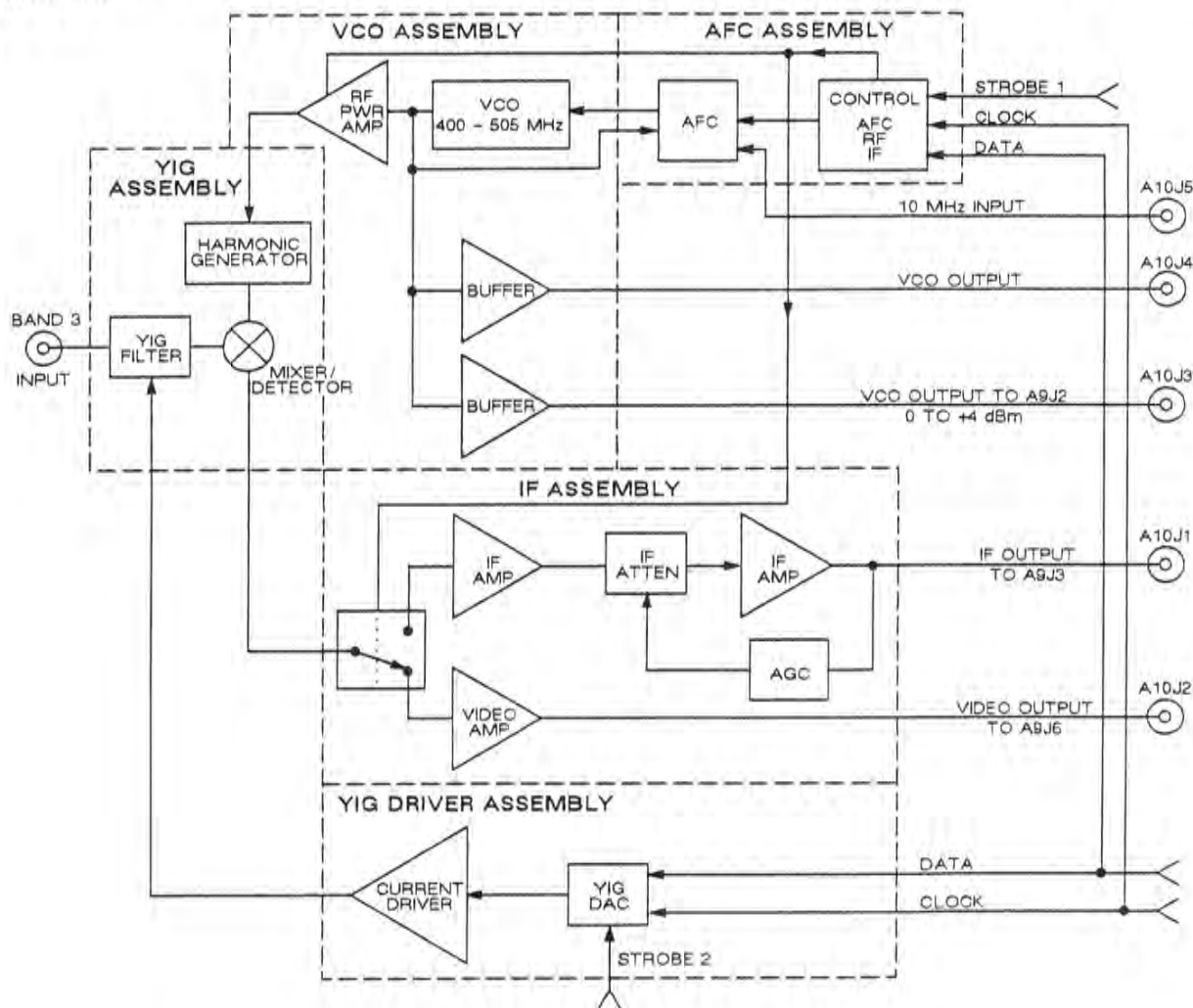
Figure 6-5. Band 3 Microwave Converter Functional Block Diagram.
