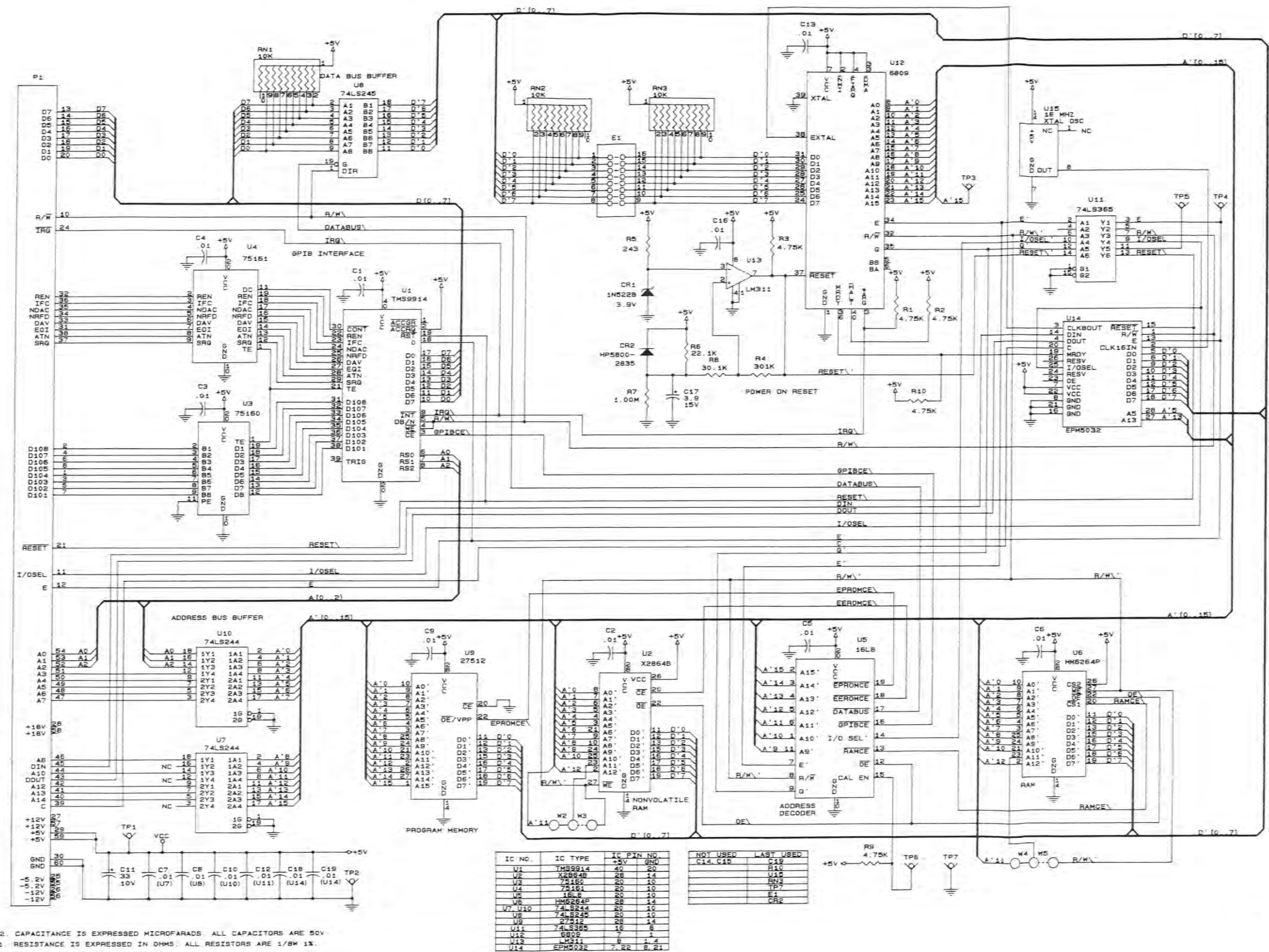
Figure 10-13. Processor/GPIB (A5) Schematic Diagram
