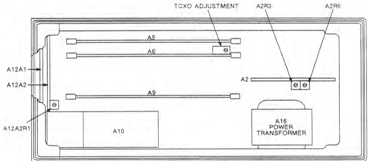
Figure 7-1. Adjustment Control Locations.
