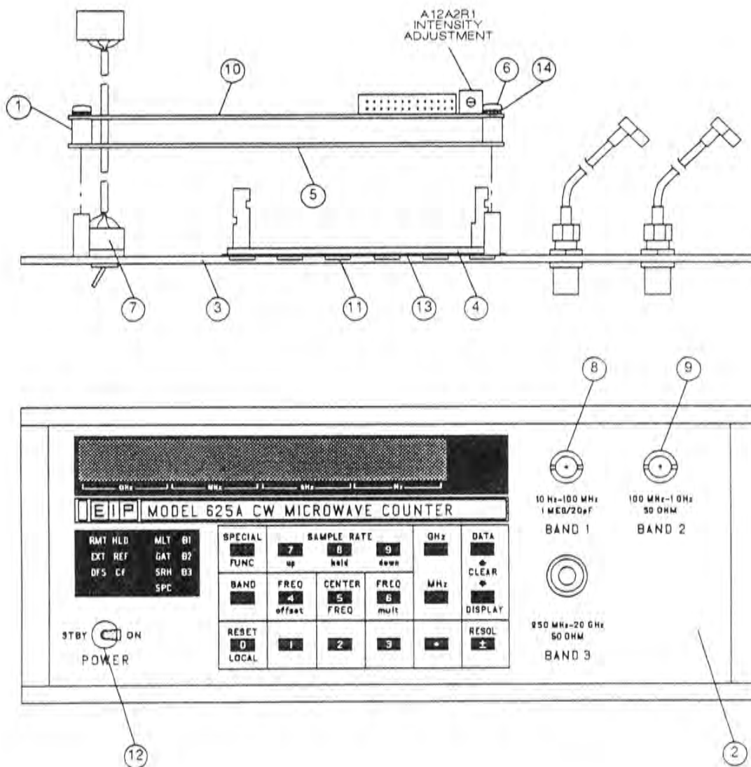
Figure 10-33. Front Panel (A12).
