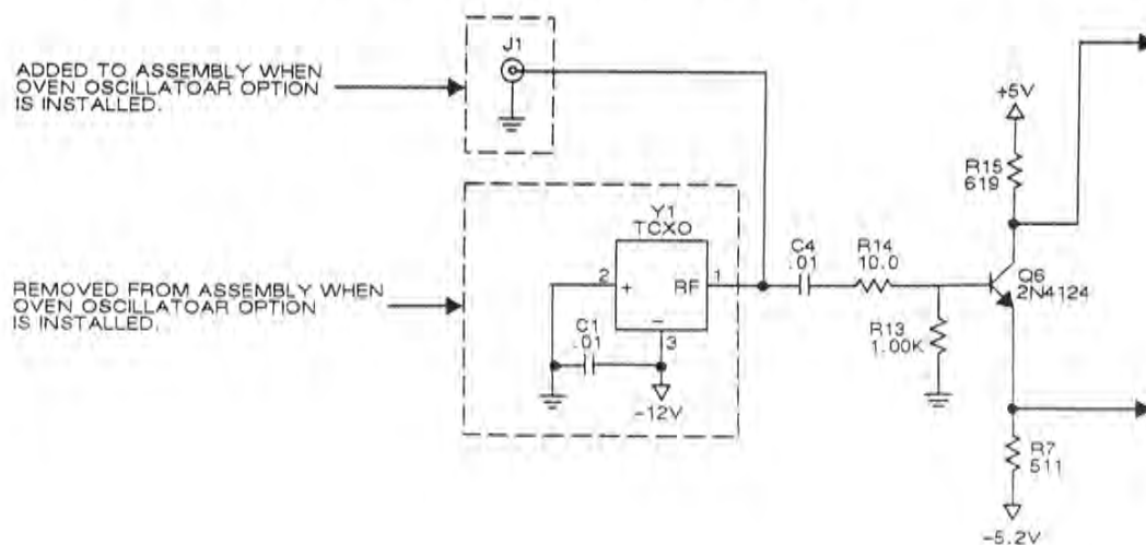
Figure 11-4. Count Chain/Gate Modifications for Option 05.
