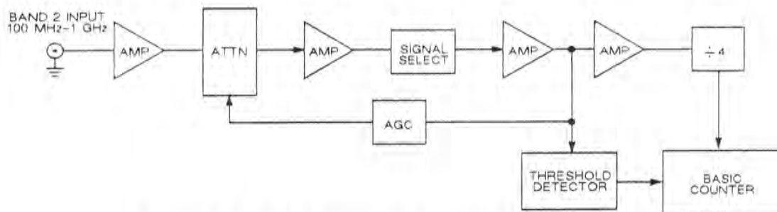
Figure 6-3. Band 2 Converter Functional Block Diagram.
