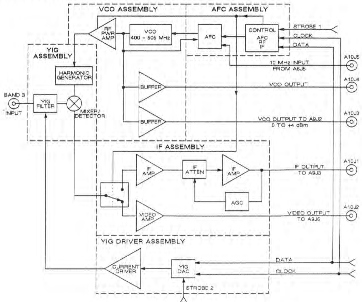
Figure 10-27. Band 3 Microwave Converter Functional Block Diagram.
