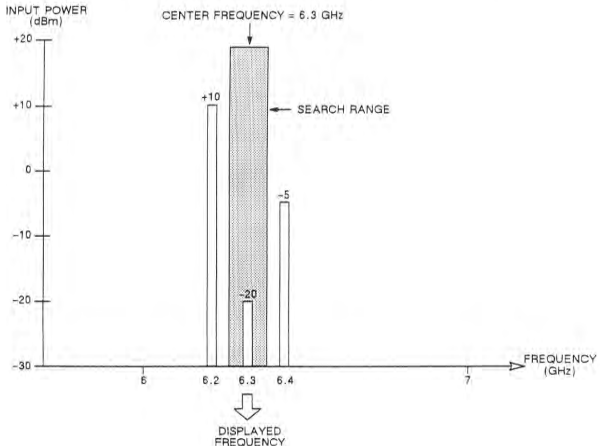
Figure 3-7. Center Frequency.
