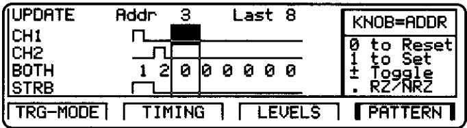
Figure 3-39. PATTERN screen, Bit-editing window
