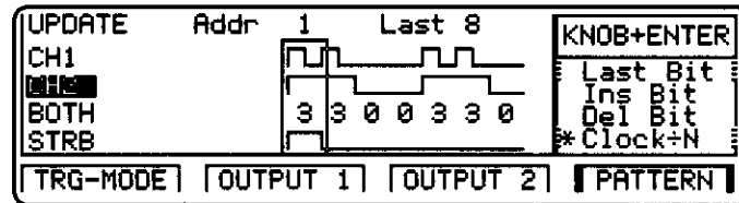
Figure 3-42. PATTERN Clock \div 4, CH1 = RZ, CH2 = NRZ
