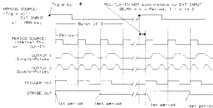
Figure 3-10. Timing Diagram: TRIGGERED BURST Pulse-Period: internal PLL or CLK-IN
