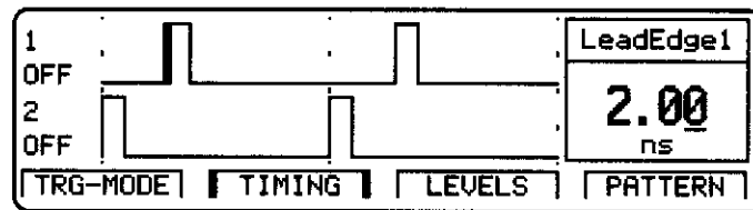
Figure 3-33. TIMING / OUTPUT Timing parameter graphics, Leading-edge
