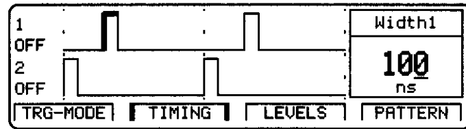
Figure 3-31. TIMING / OUTPUT Timing parameter graphics, Width
