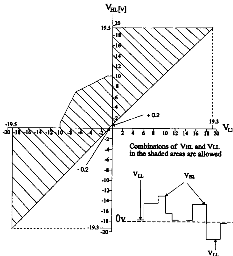
Figure 6-2. Highest and lowest level combinations
