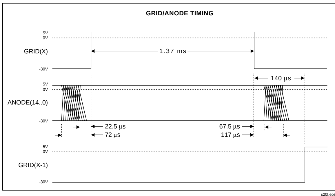
Figure 2A-10. Grid-Anode Timing Relationships (2635A)
