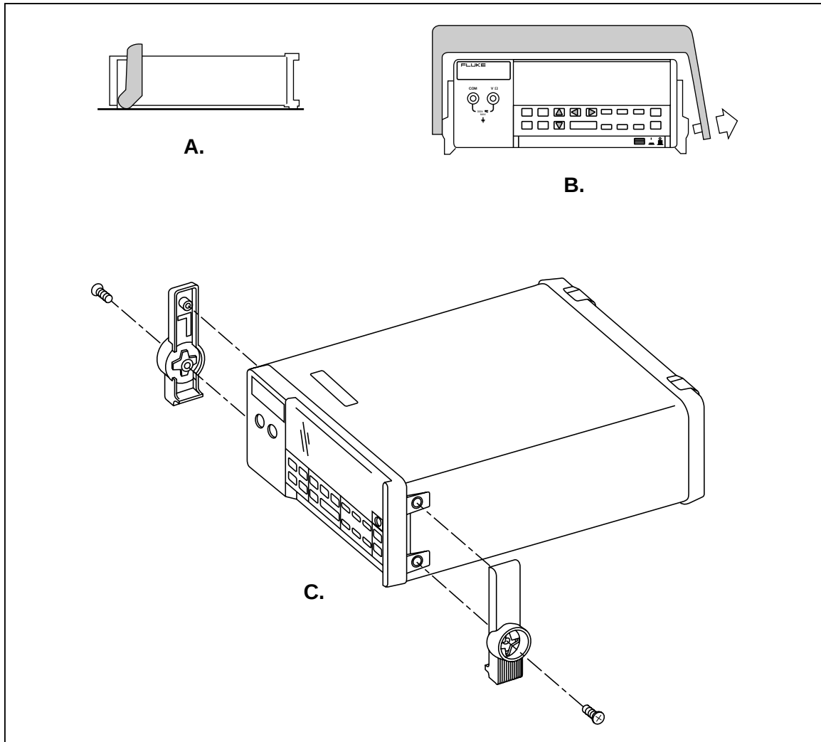
Figure 3-3. Removing the Handle and Handle Mounting Brackets
