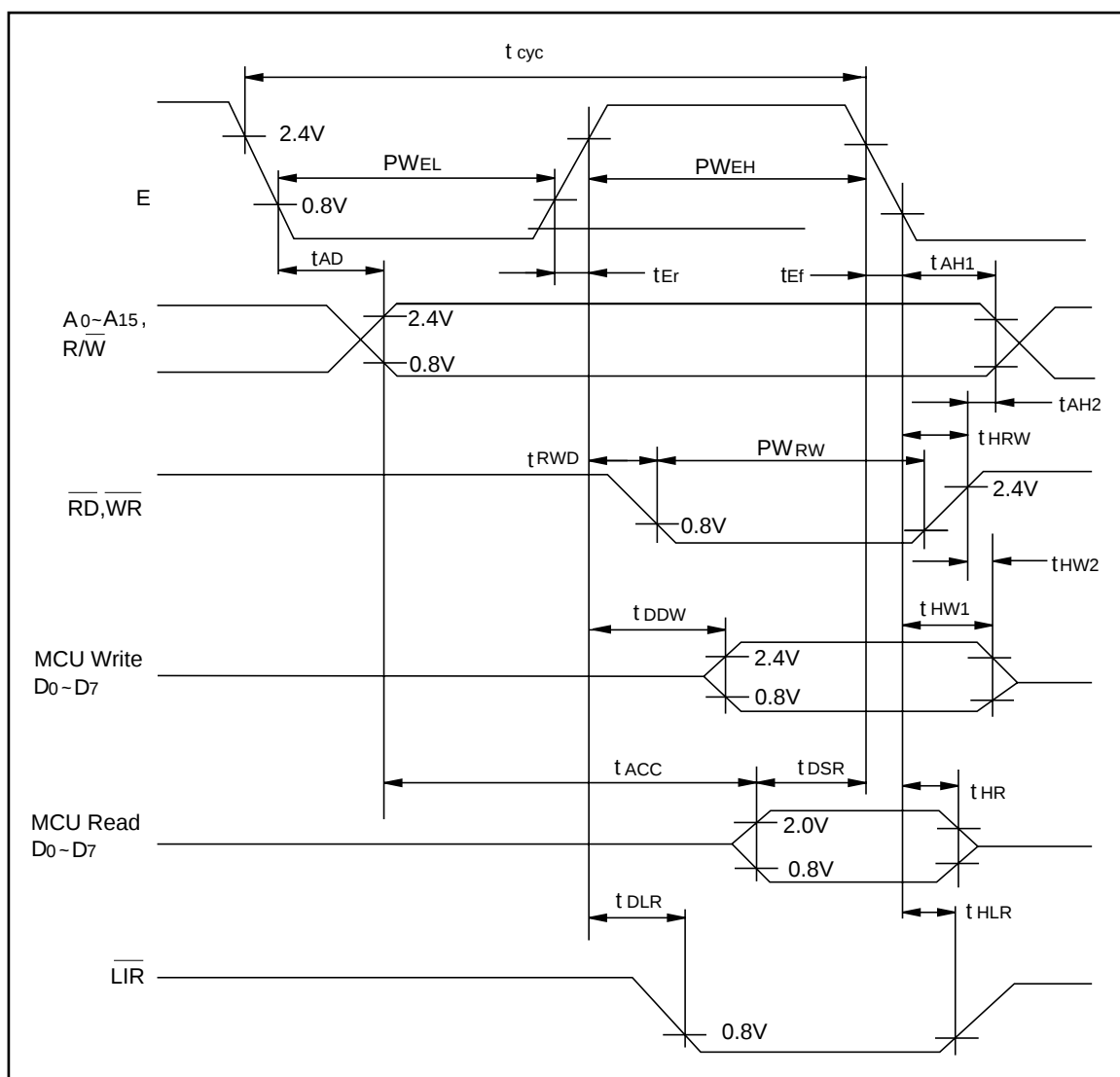
Figure 5-7. Microprocessor Timing
