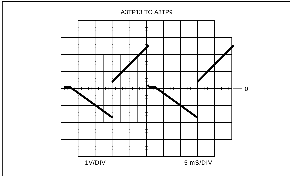
Figure 5-6. Integrator Output
