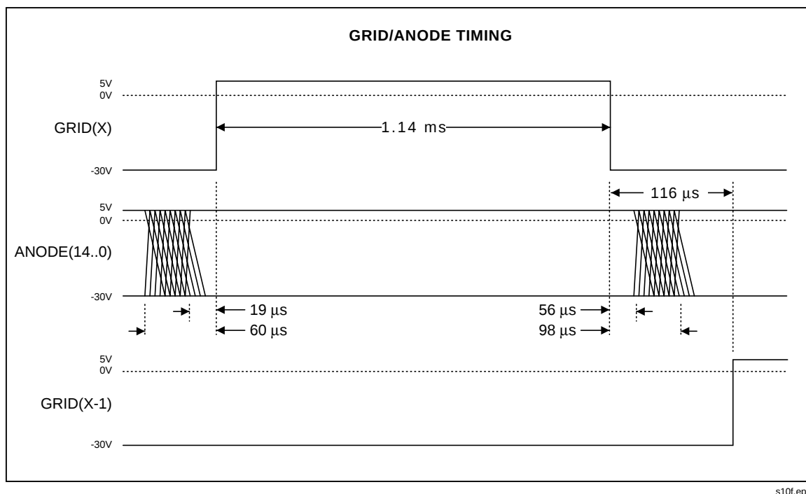
Figure 2-10. Grid-Anode Timing Relationships
