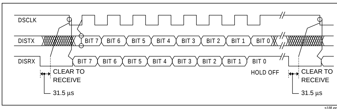
Figure 2A-8. Command Byte Transfer Waveforms (2635A)
