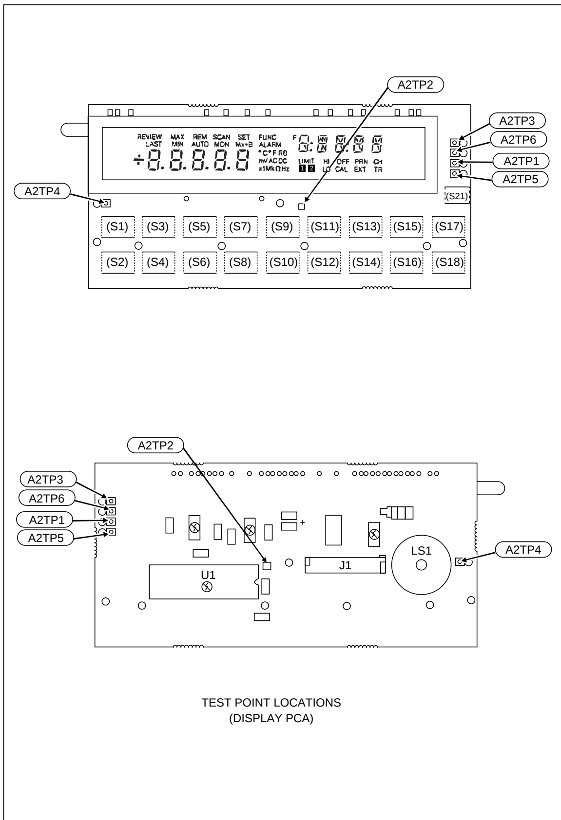
Figure 5-8. Test Points, Display PCA (A2)
