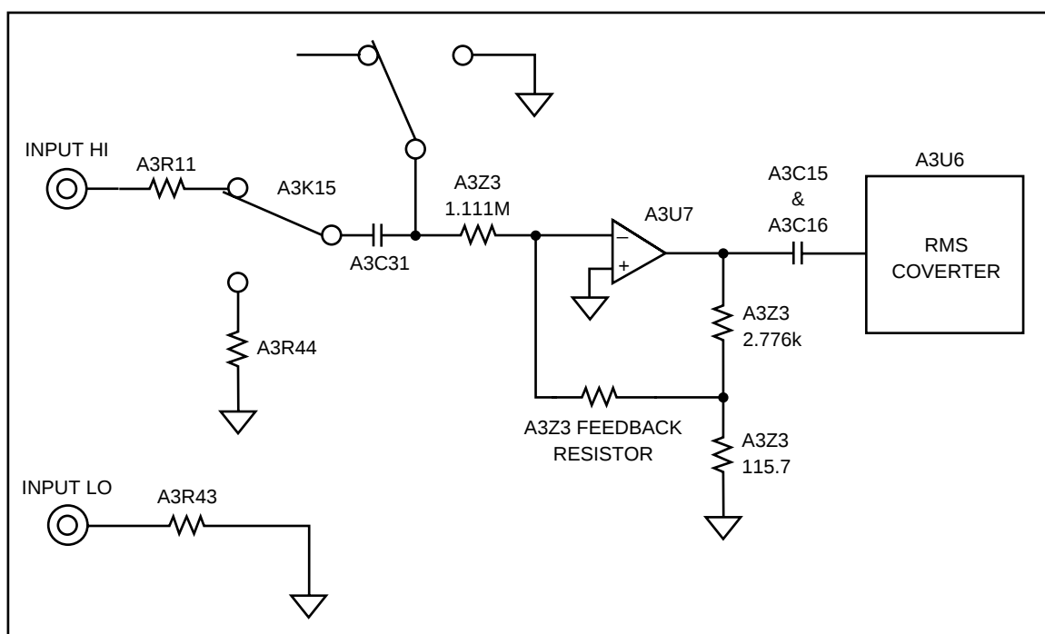
Figure 2-6. AC Buffer Simplified Schematic
