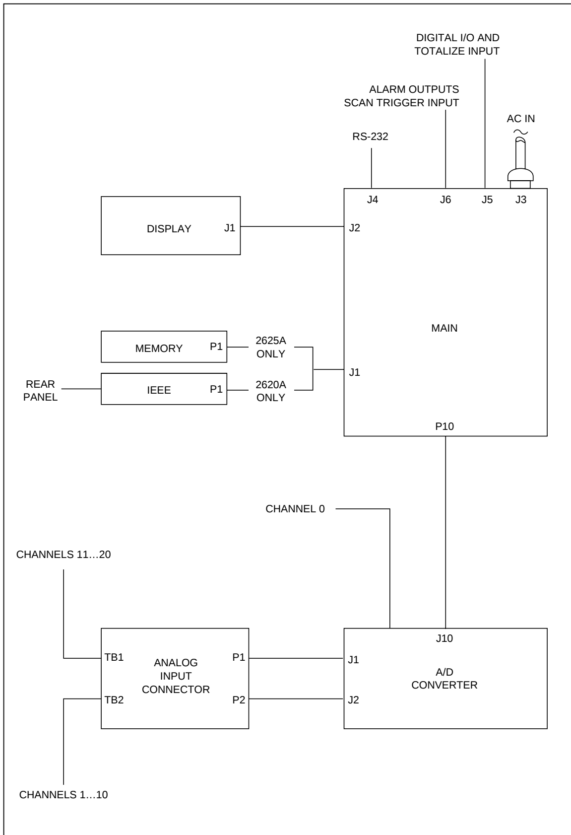
Figure 2-1. Interconnect Diagram
