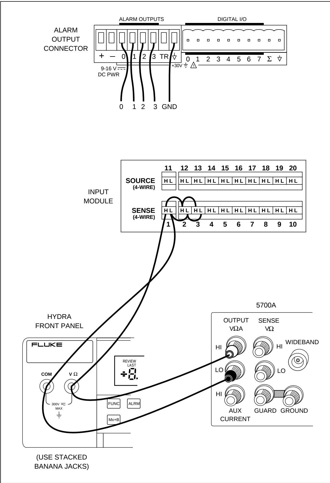
Figure 4-3. Dedicated Alarms Test
