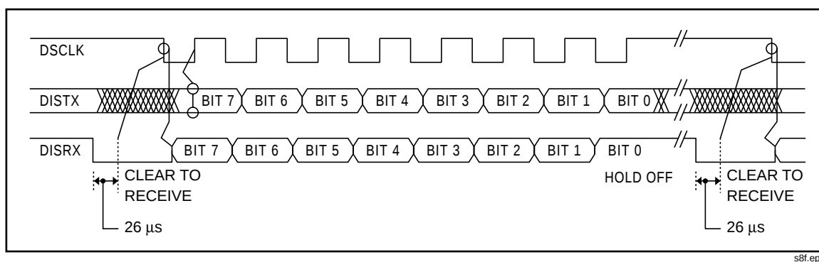
Figure 2-8. Command Byte Transfer Waveforms
