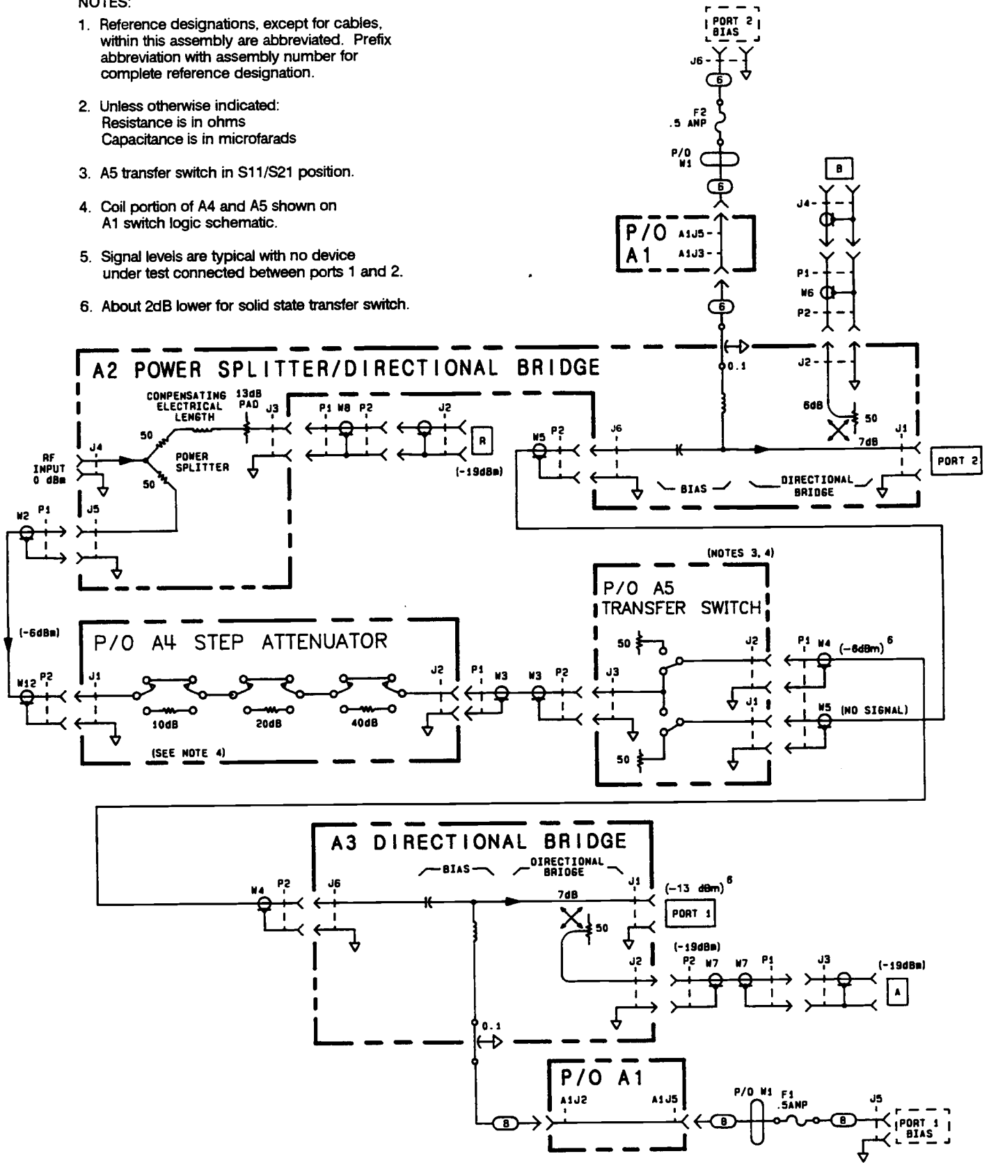
Figure 8-3. Schematic Diagram
