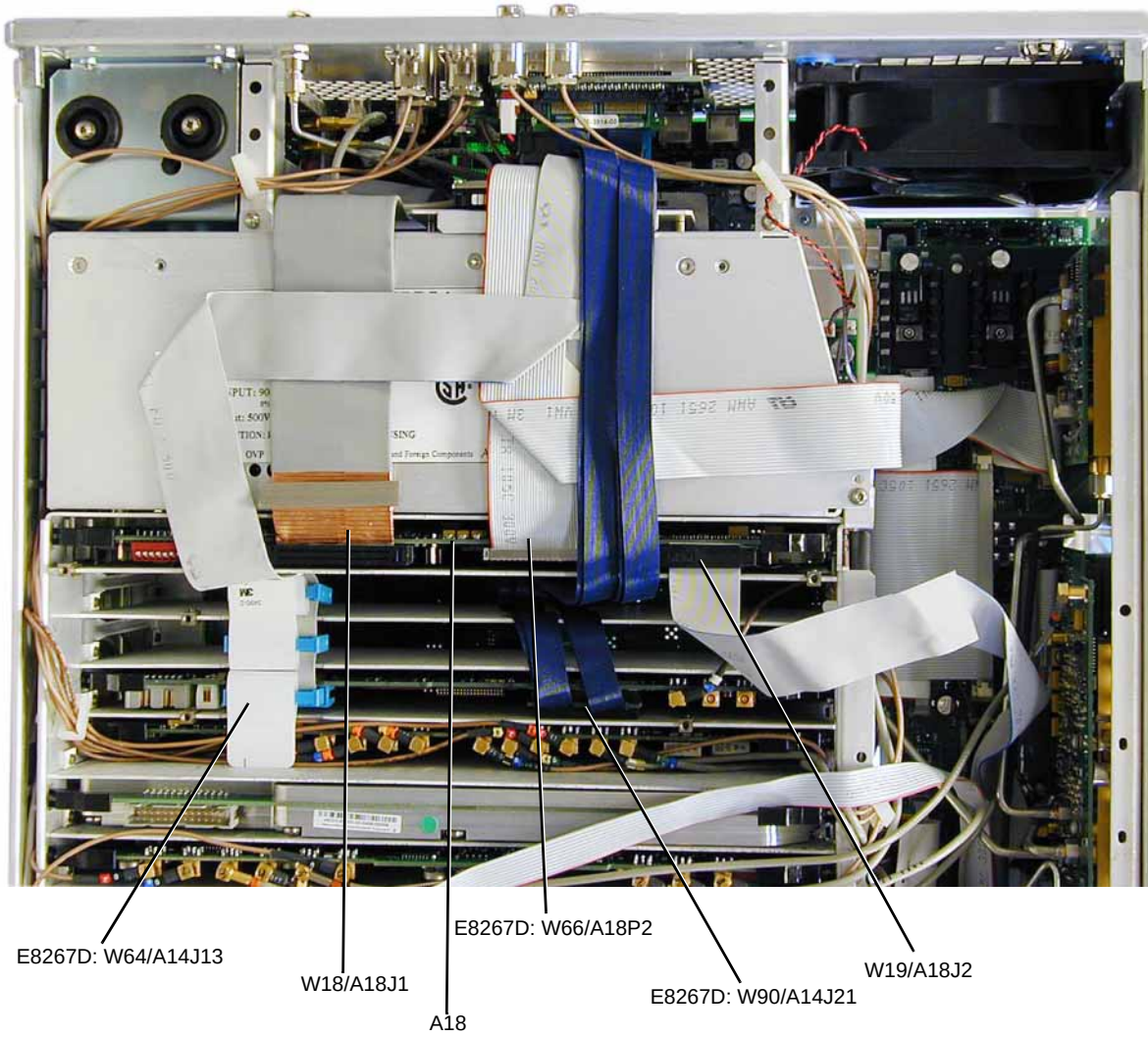
Figure 3-23 A18 CPU
