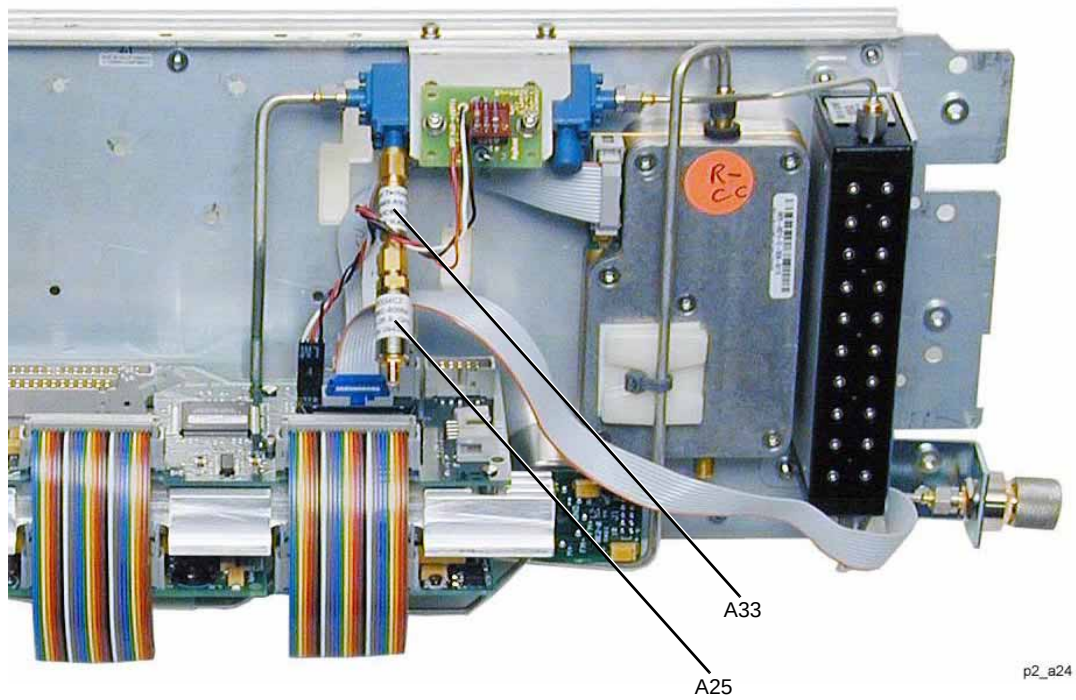
Figure 3-40 A25 20 GHz Highband Detector (Options 503, 509, 513, and 520)
