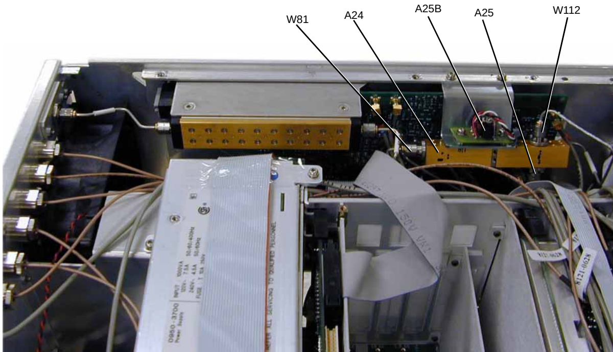
Figure 3-39 A24 67 GHz Highband Coupler (Options 550 & 567 and Option 1EM)
