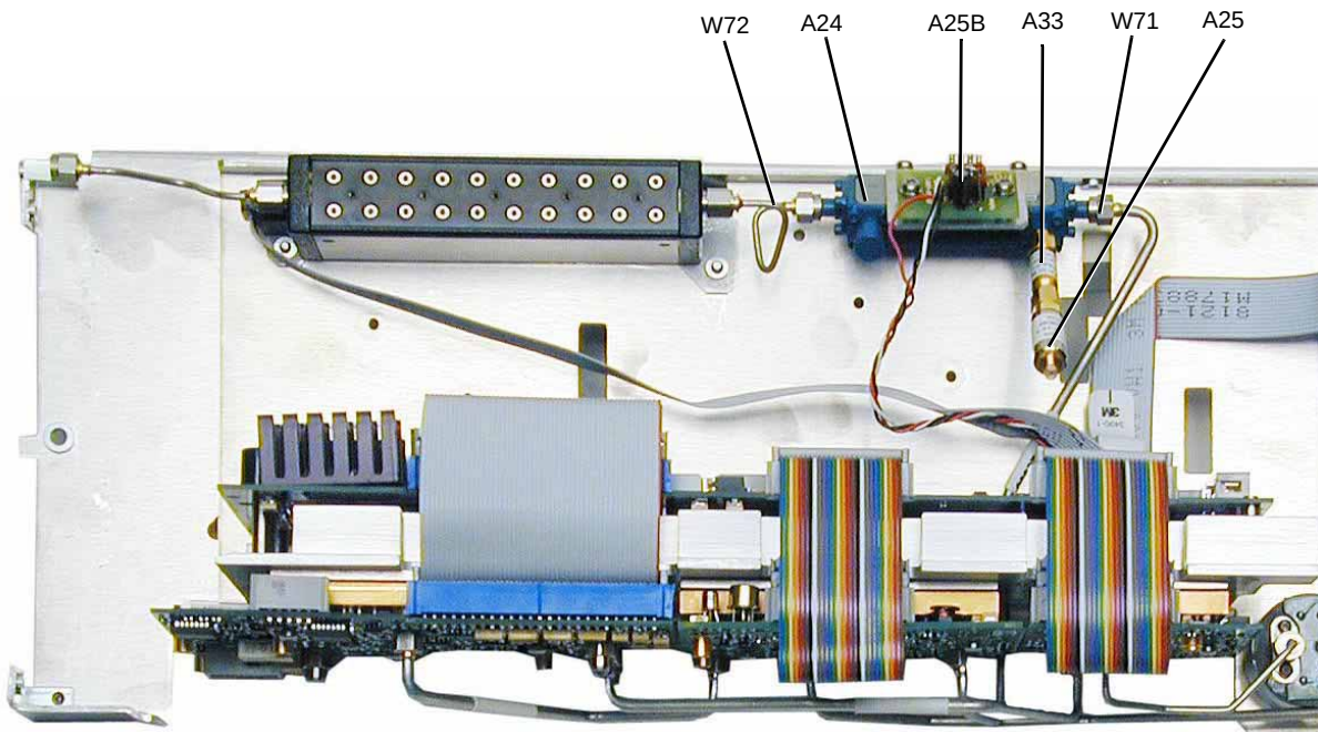
Figure 3-31 A24 20 GHz Highband Coupler (Options 503, 509, 513, and 520 – Option 1EM)
