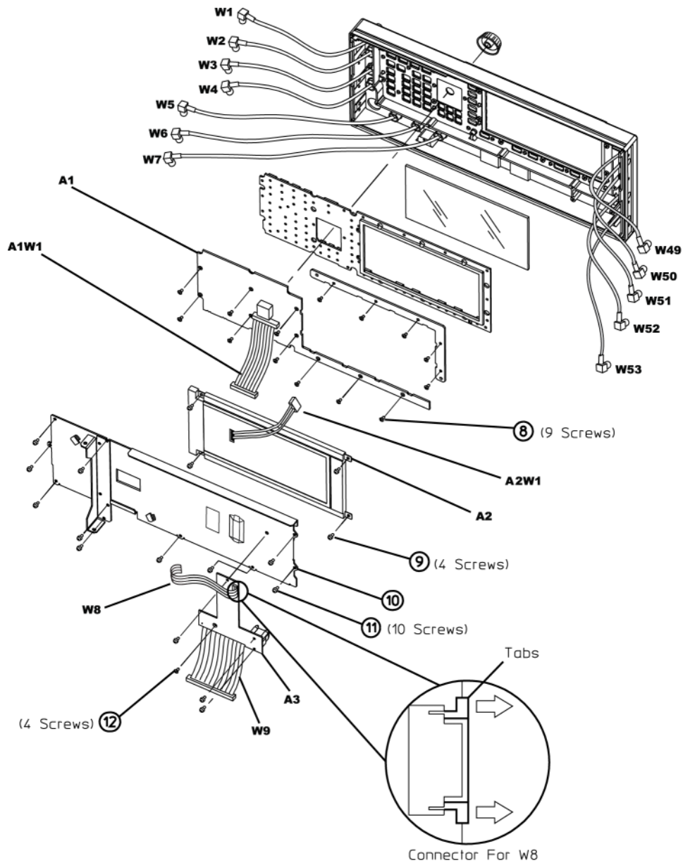
Figure 3-11 A3 Power Switch Removal with serial number prefix \geq US/MY5XXX3XXX
