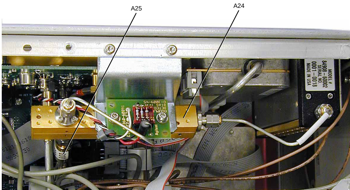
Figure 3-44 A25 67 GHz Highband Detector (Options 550 and 567)
