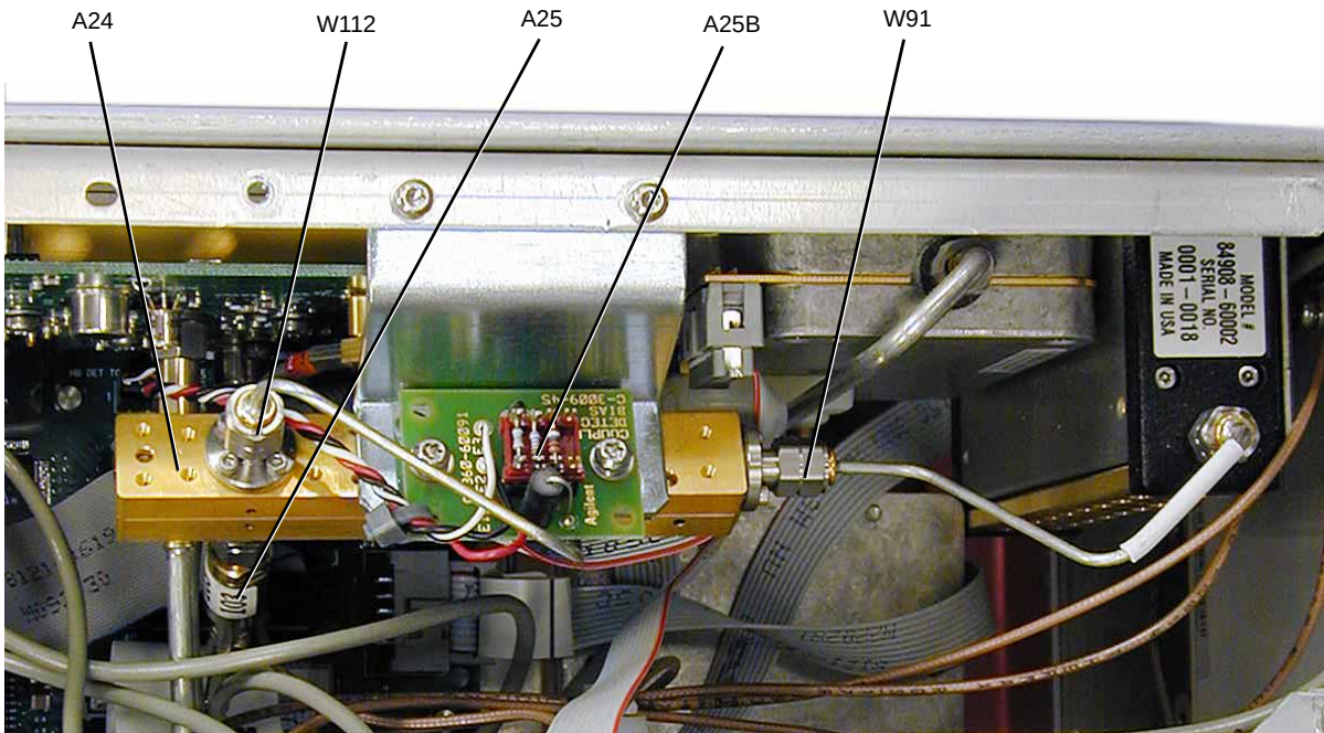
Figure 3-39 A24 67 GHz Highband Coupler (Options 550 & 567 and Option 1EM)
