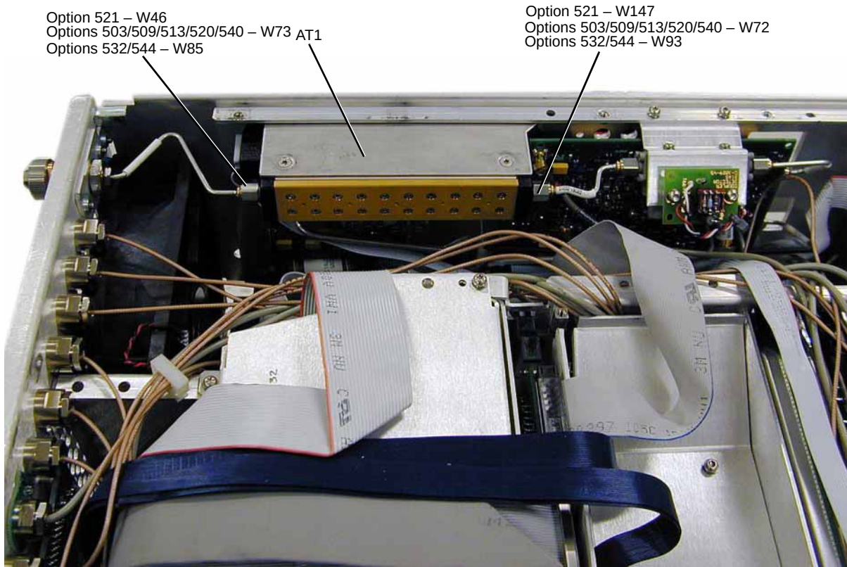
Figure 3-76 AT1 115dB Attenuator (Option 1EM)
