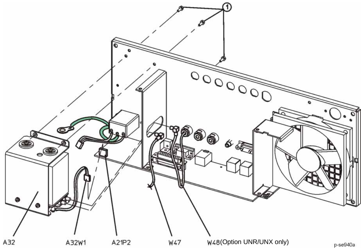
Figure 3-55 A32 Crystal Oscillator
