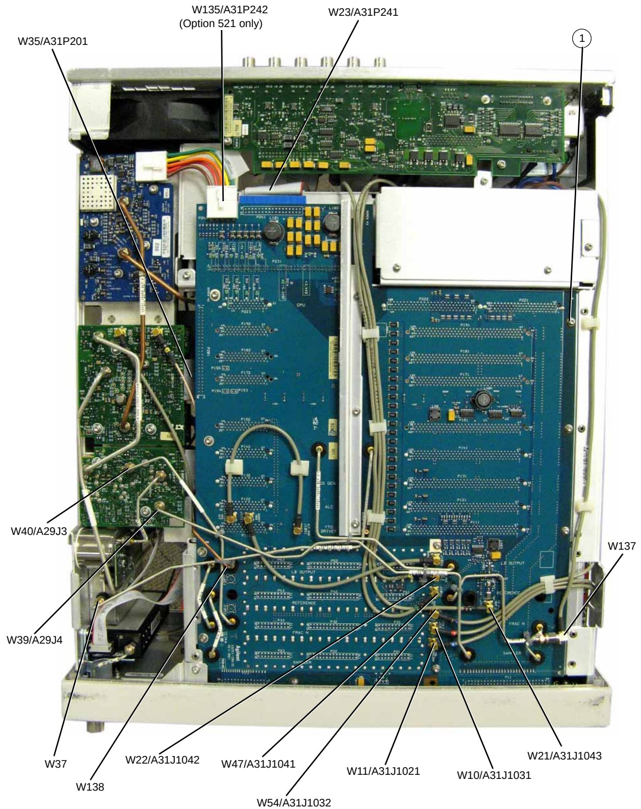
Figure 3-53 A31 Motherboard (E8257D & E8663D)
