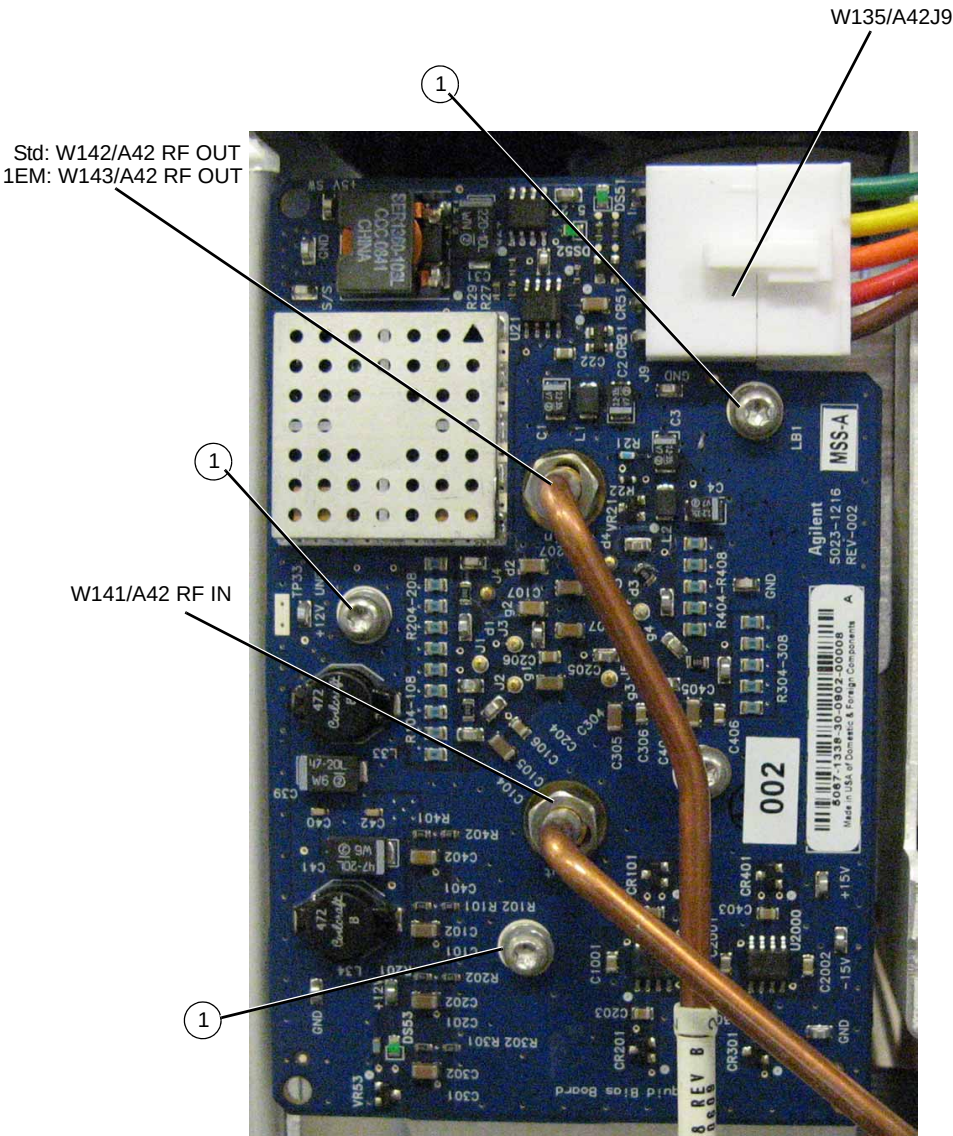
Figure 3-70 A42 20 GHz Power Amp
