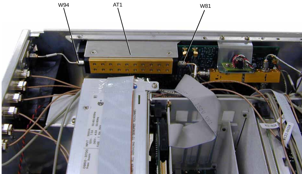
Figure 3-75 AT1 90 dB Attenuator (Options 1EM)
