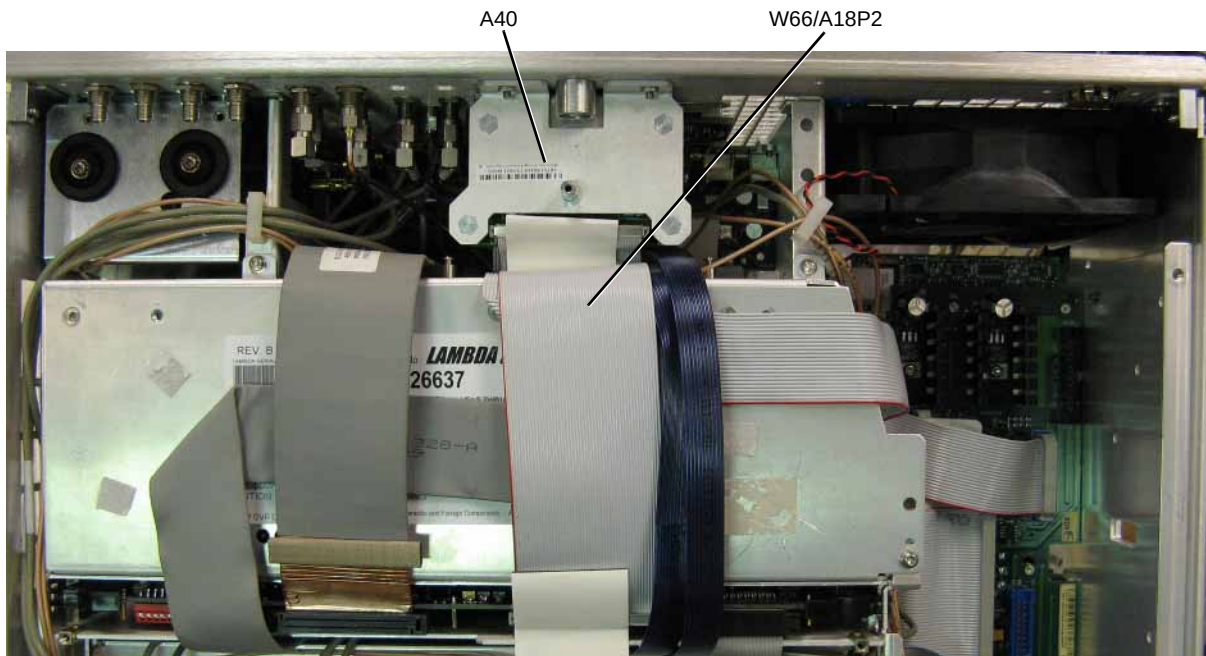
Figure 3-67 A40 Flash Drive Assembly
