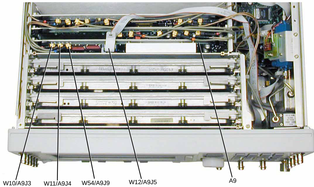
Figure 3-15 A9 YIG Driver
