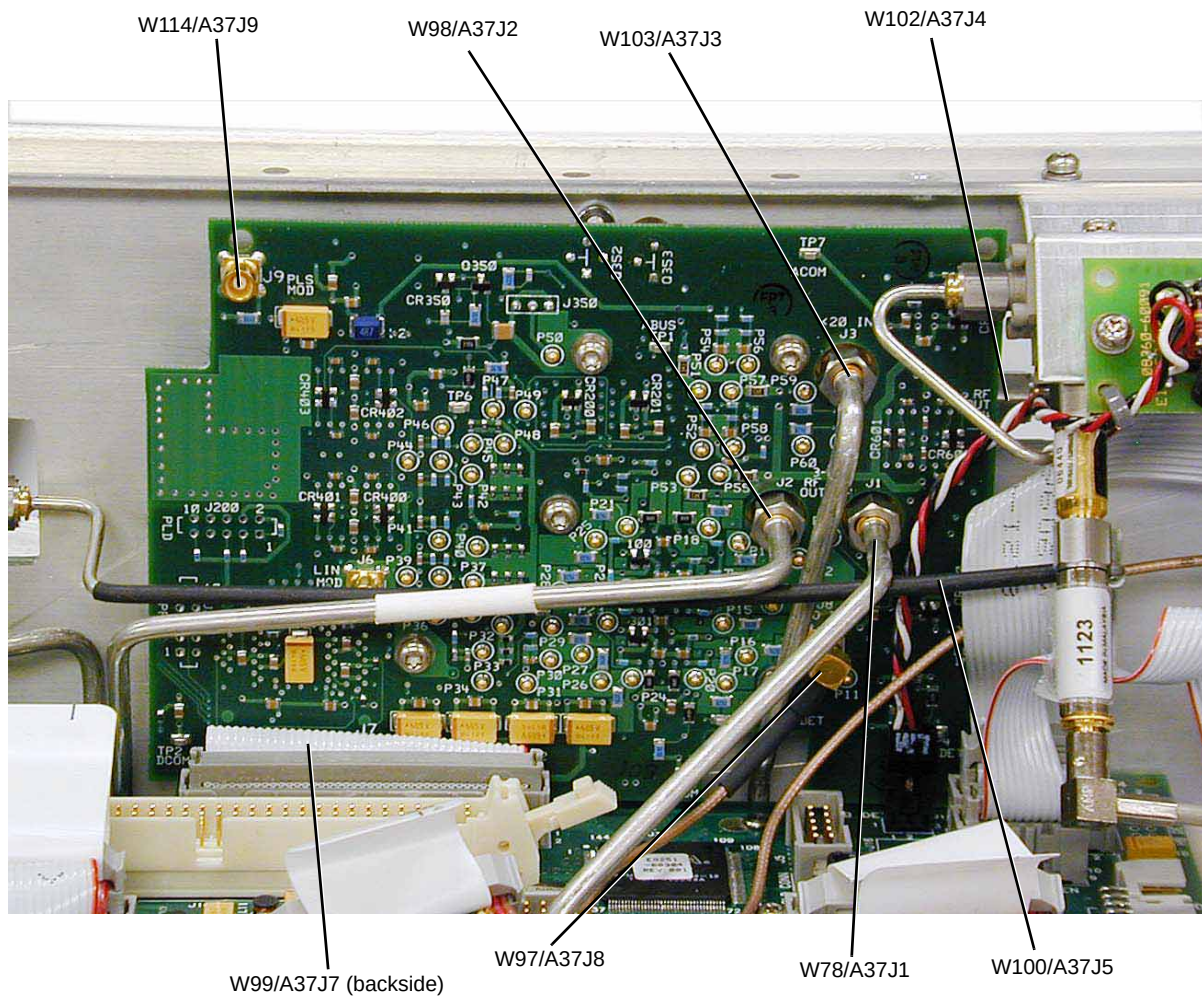
Figure 3-64 A37 Upconverter
