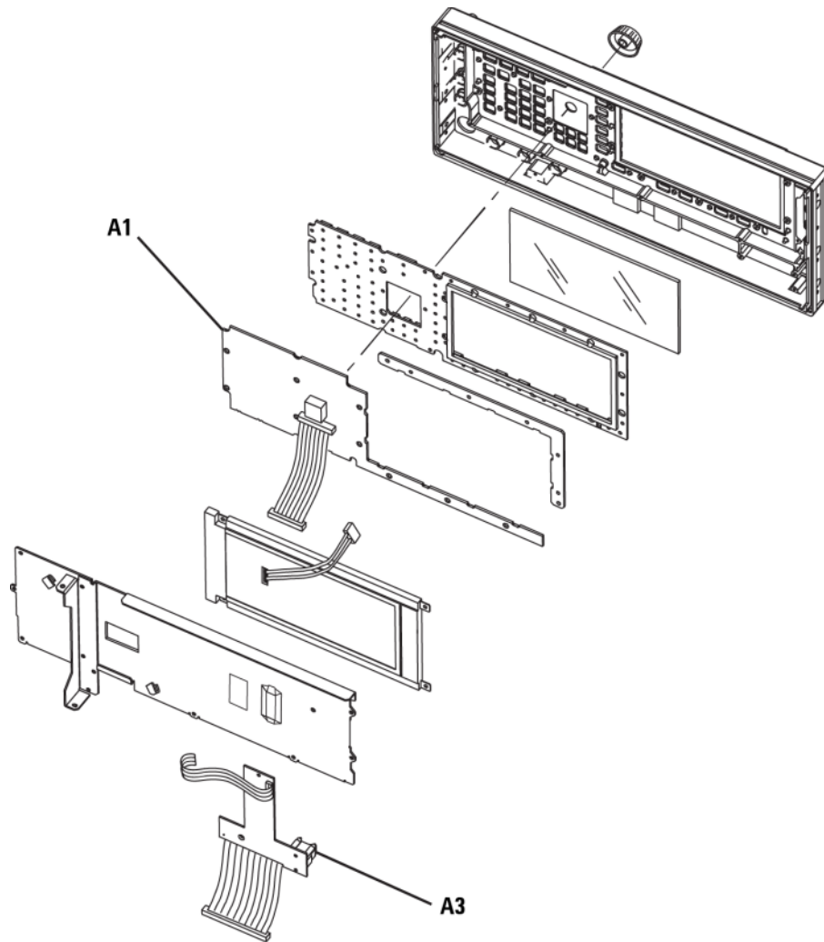
Figure 2-2 Assemblies from the Inside Front Panel View for with serial prefixes \geq US/MY5XXX3XXX
