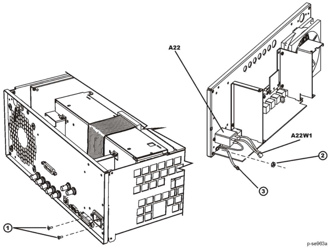
Figure 3-28 A22 Line Module Removal
