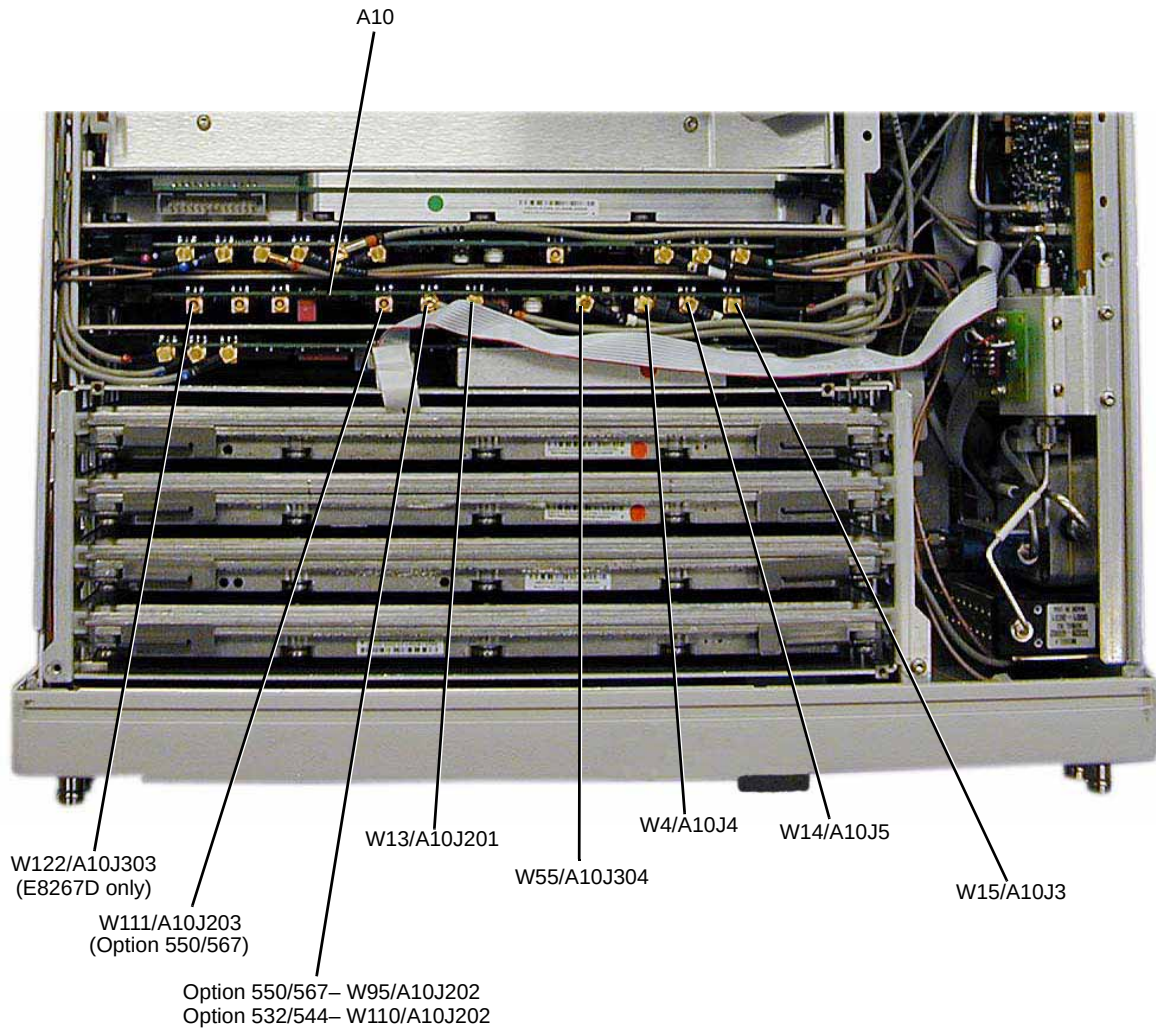
Figure 3-16 A10 ALC
