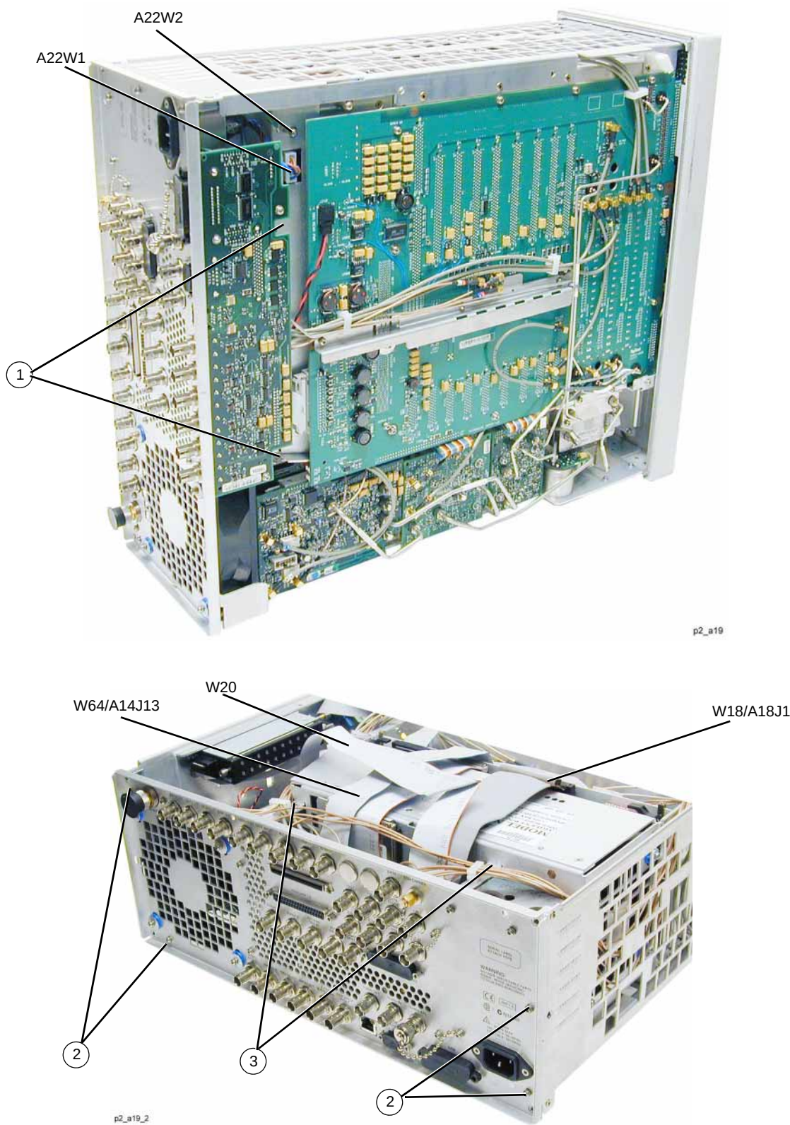
Figure 3-59 Rear Panel Removal (Option 1EM)
