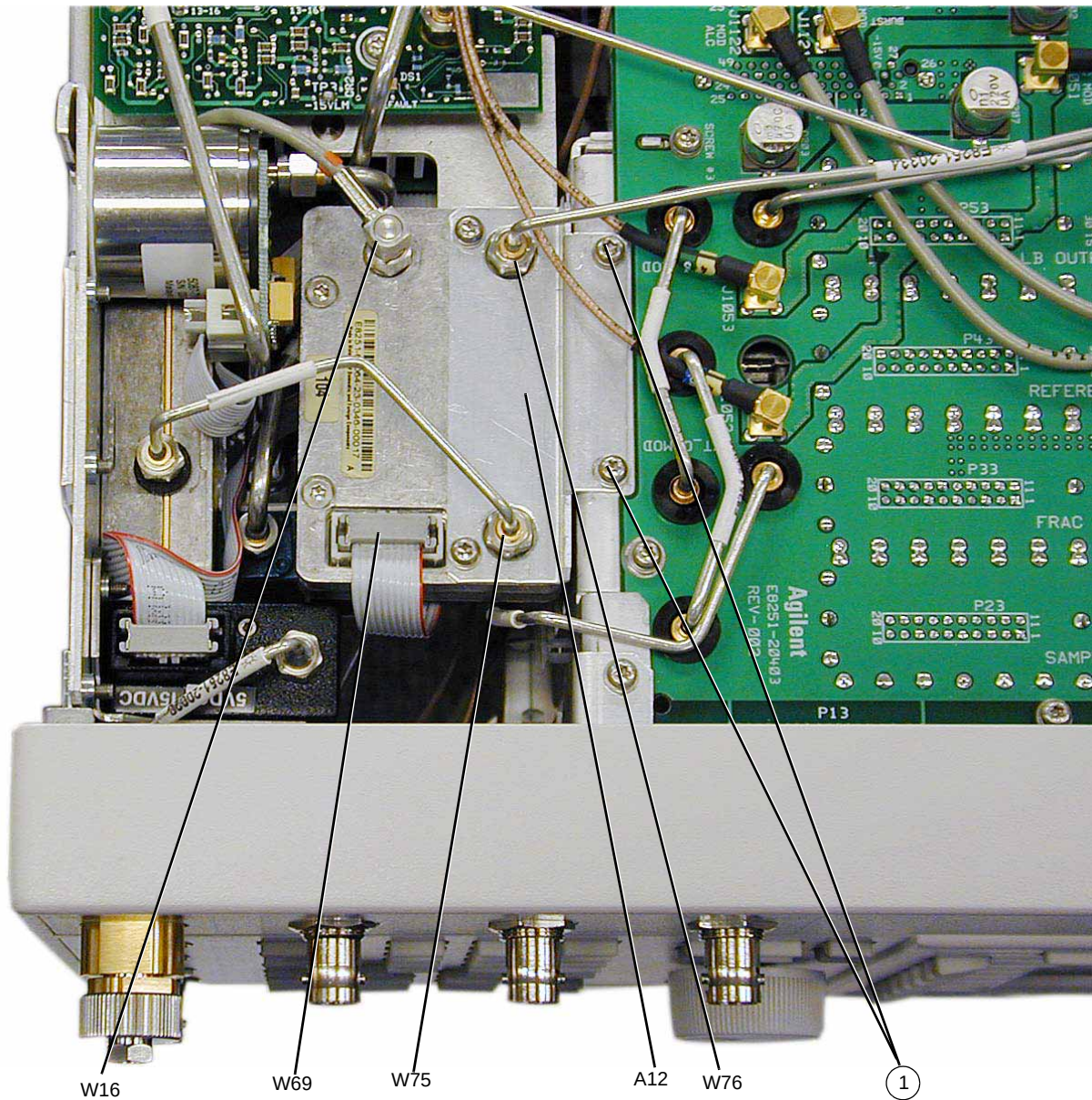
Figure 3-18 A12 Pulse Modulator Board
