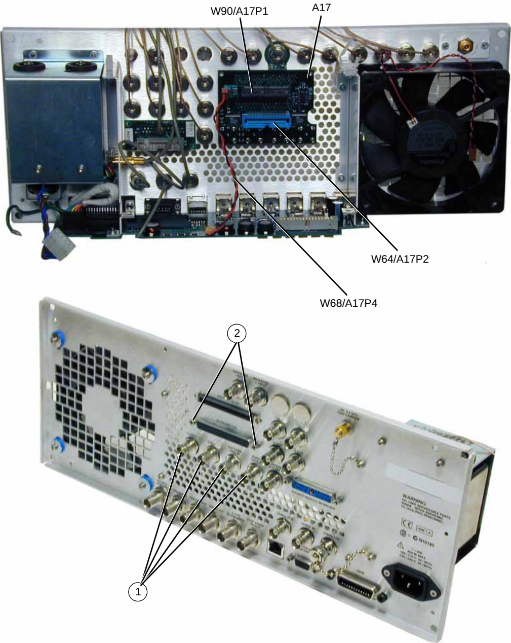
Figure 3-22 A17 Rear Panel Interface Board
