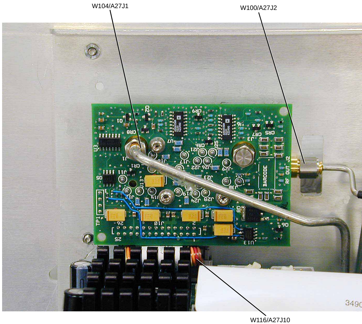
Figure 3-49 A27 40 GHz Doubler (Options 532 and 544)
