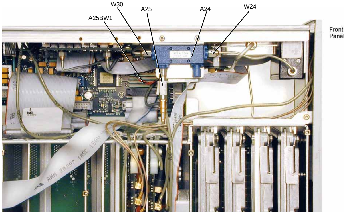
Figure 3-34 A24 40 GHz Highband Coupler (Option 540 – Standard)
