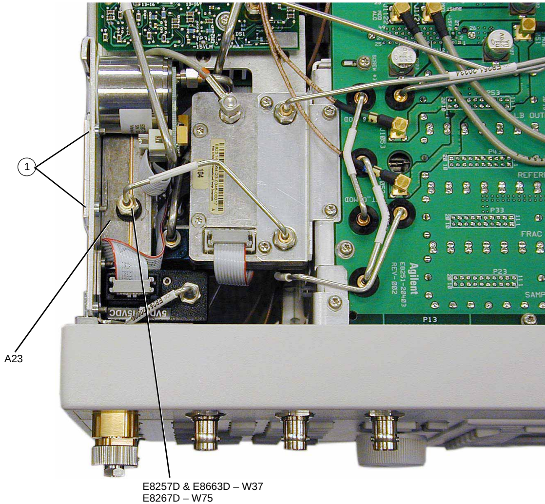
Figure 3-29 A23 Lowband Coupler/Detector
