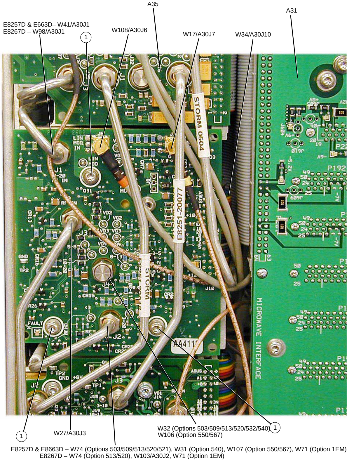
Figure 3-52 A30 Modulator Filter
