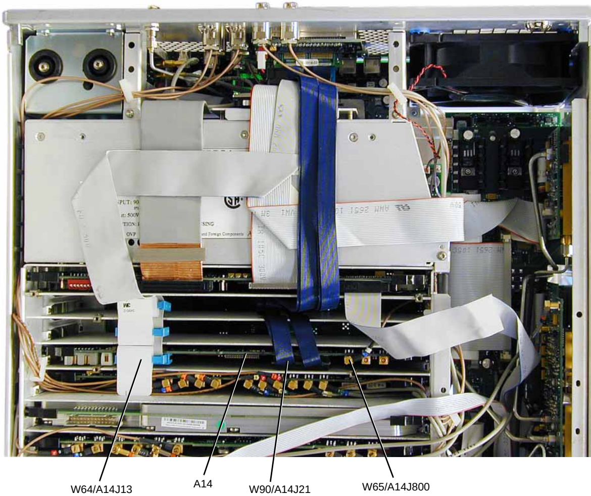
Figure 3-21 A14 Baseband Generator
