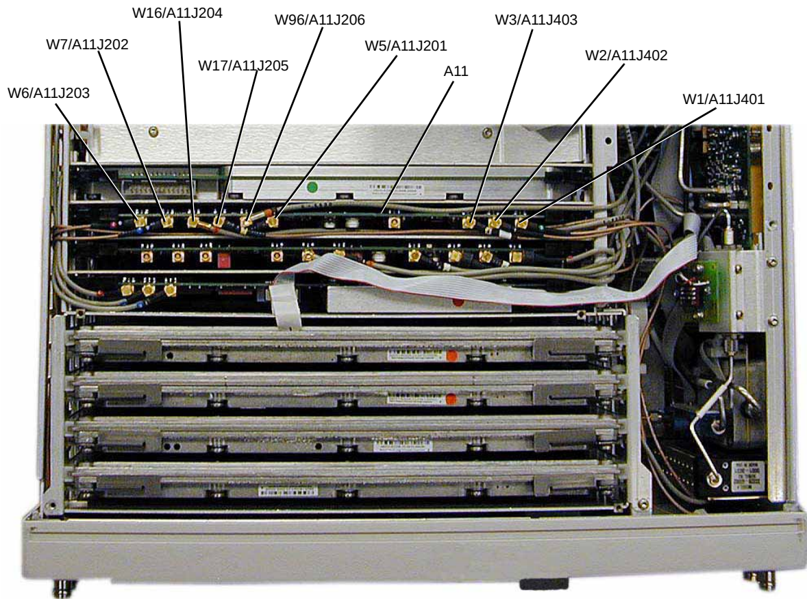
Figure 3-17 A11 Pulse/Analog Modulation Generator
