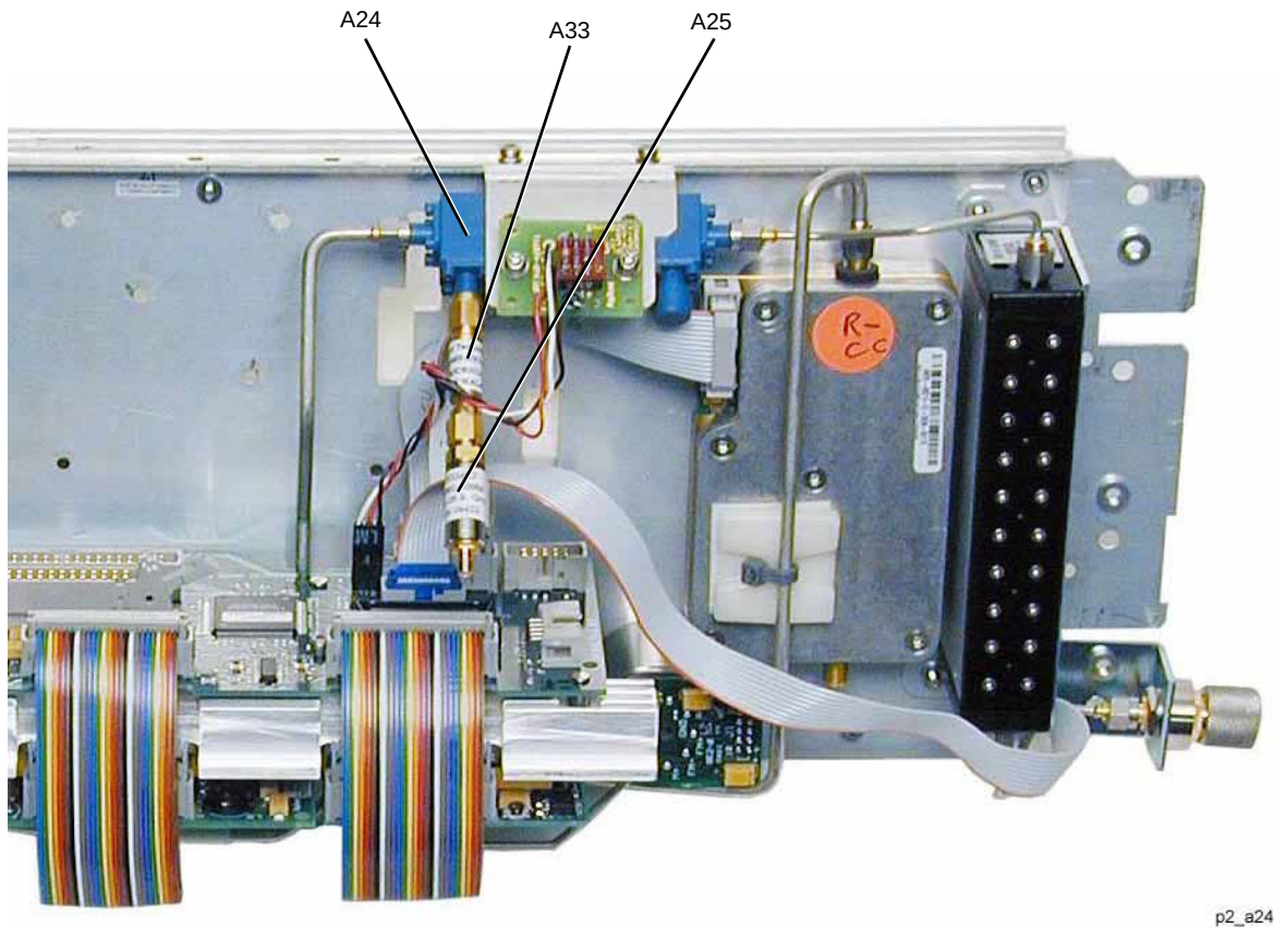
Figure 3-56 A33 6dB PAD (Options 503, 509, 513, 520, and 521)
