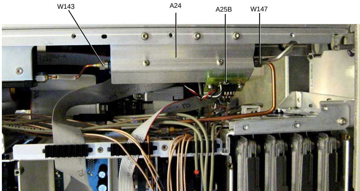
Figure 3-33 A24 20 GHz Highband Coupler (Option 521 - Option 1EM)
