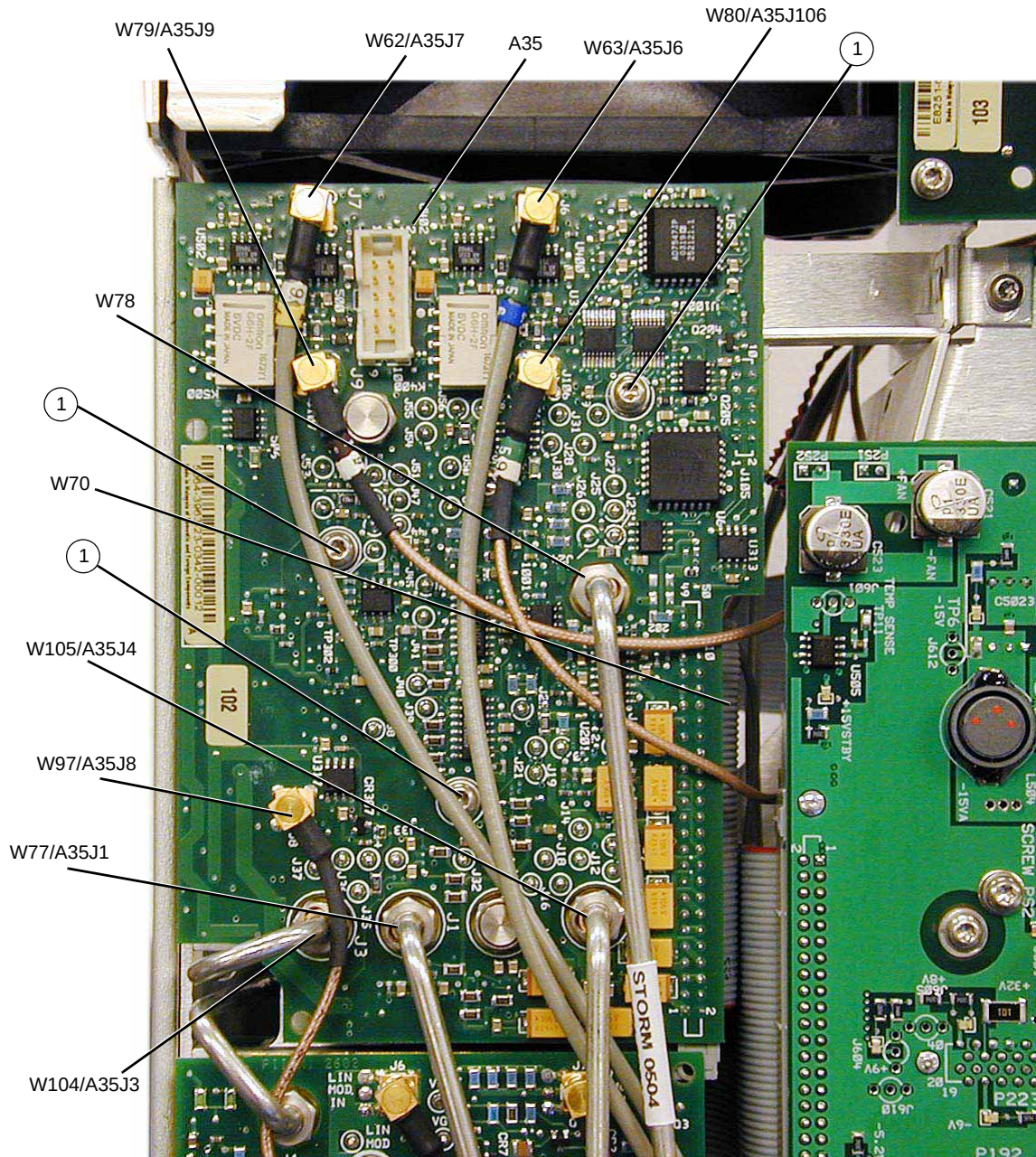
Figure 3-61 A35 3–20 GHz I/Q MOD
