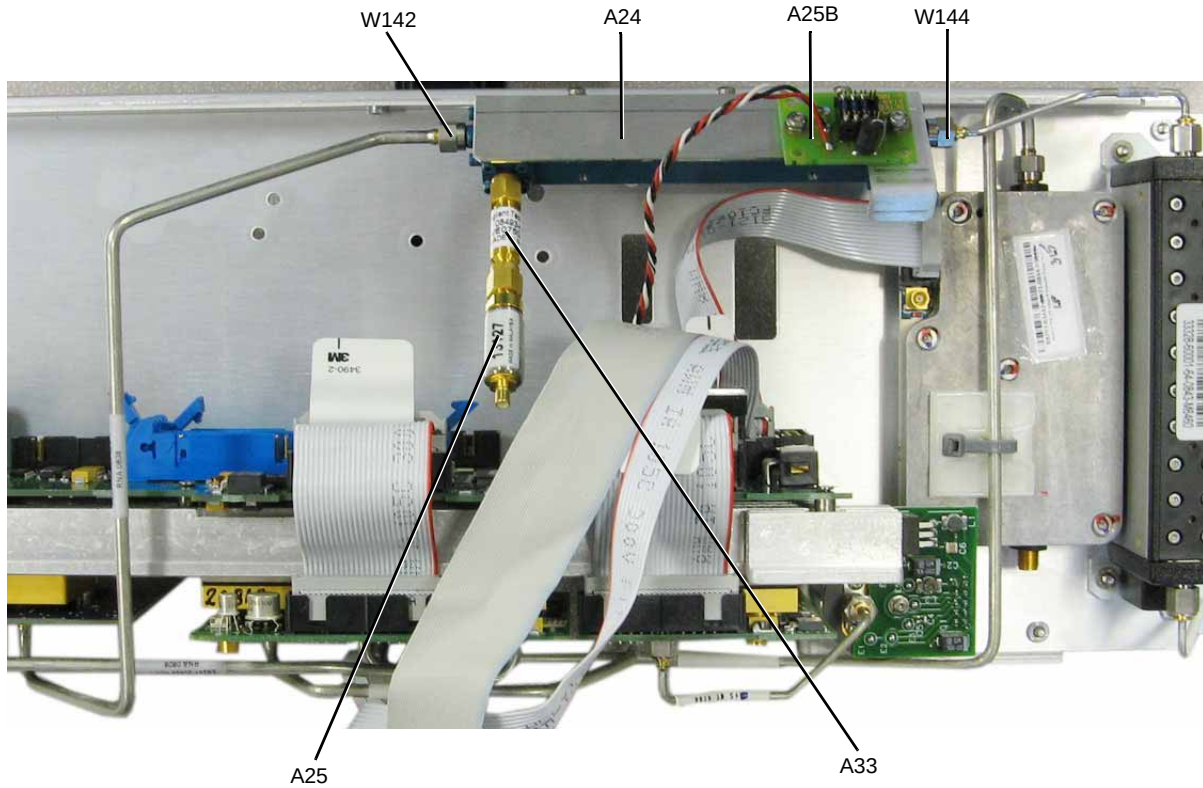
Figure 3-32 A24 20 GHz Highband Coupler (Option 521 - Standard)
