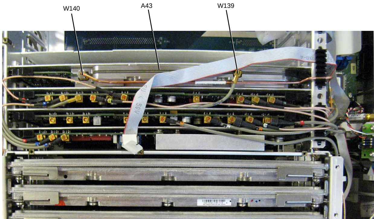
Figure 3-71 A43 Lowband Amp Filter
