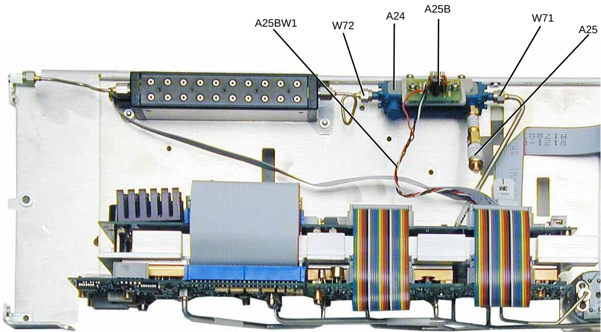
Figure 3-35 A24 40 GHz Highband Coupler (Option 540 – Option 1EM)
