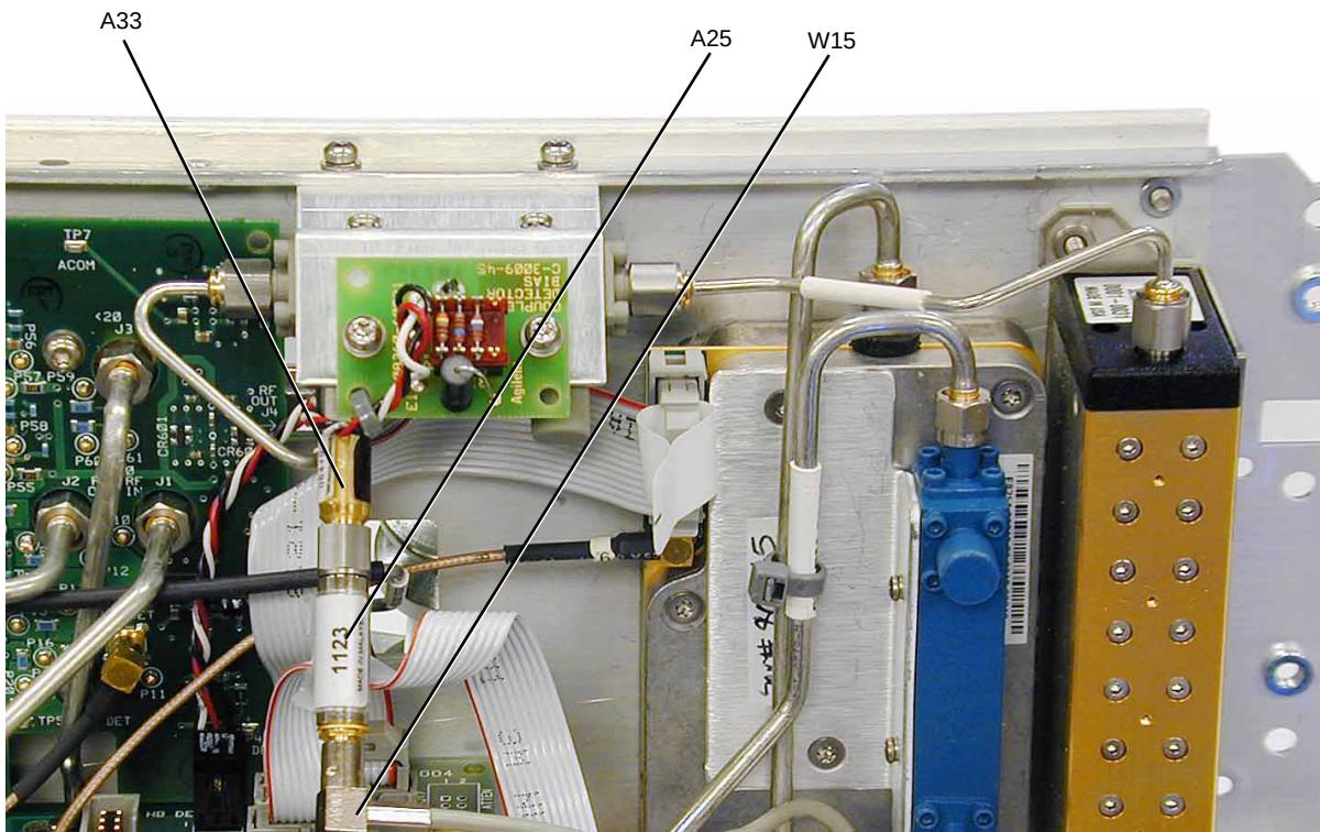
Figure 3-43 A25 50 GHz Highband Detector (Options 532 and 544)
