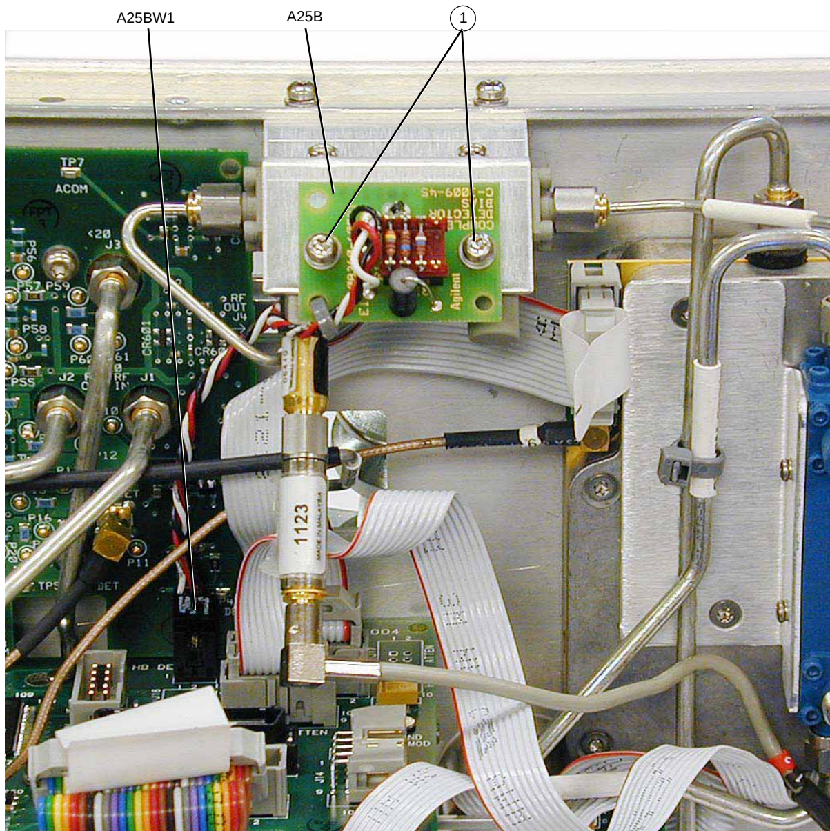
Figure 3-45 A25B Highband Detector Bias Board
