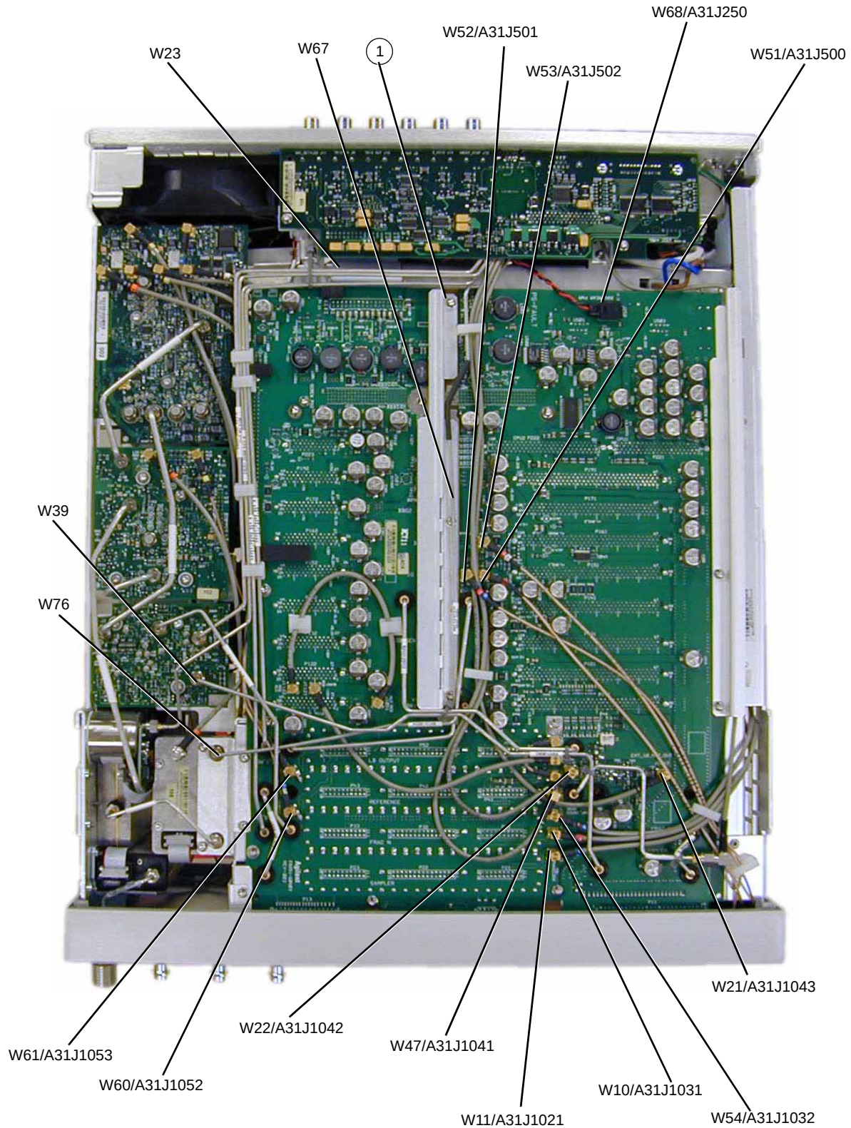
Figure 3-54 A31 Motherboard (E8267D)
