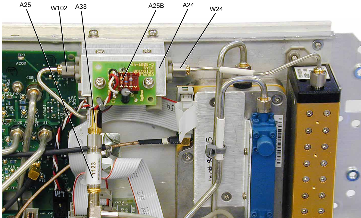
Figure 3-36 A24 50 GHz Highband Coupler (Options 532 & 544 – Standard)
