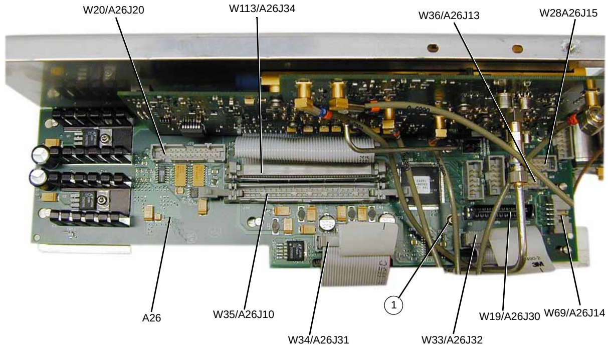
Figure 3-46 A26 MID (E8257D & E8663D)
