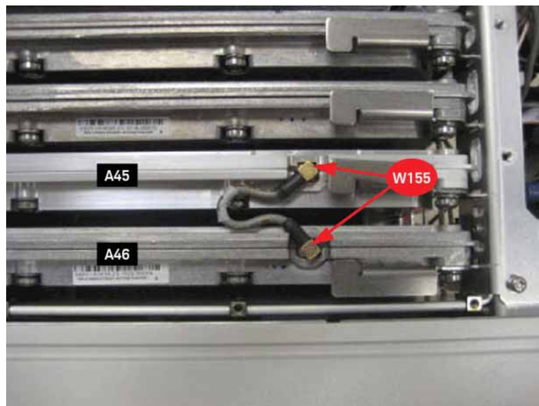
Figure 3-14 W155 Reference (Option UNY) with A45 and A46
