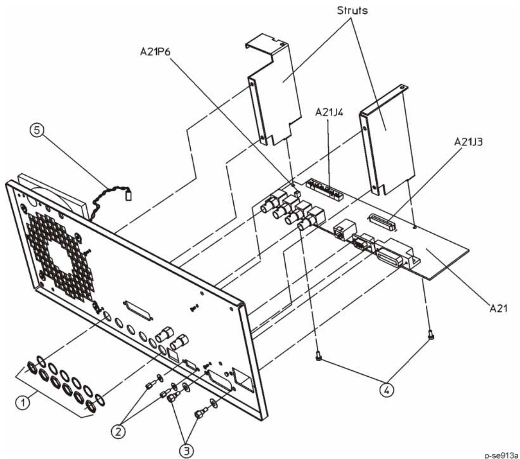
Figure 3-27 A21 Rear Panel Interface
