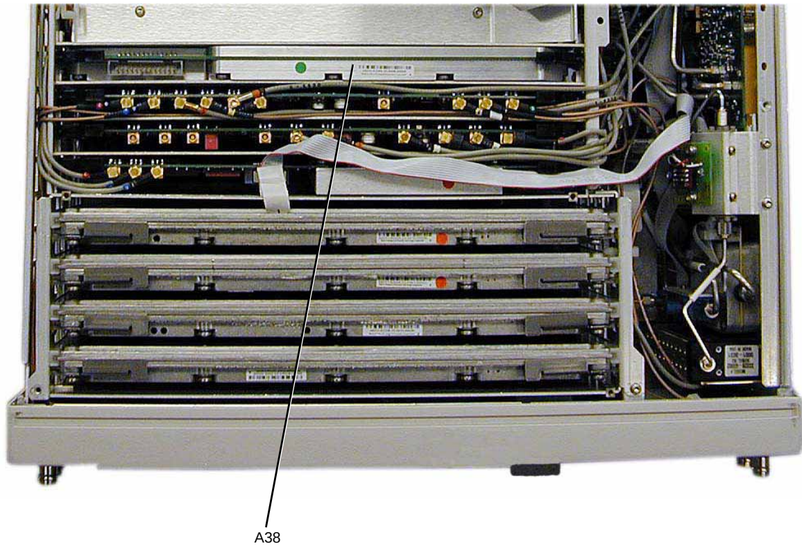
Figure 3-65 A38 Low Band Switch Filter
