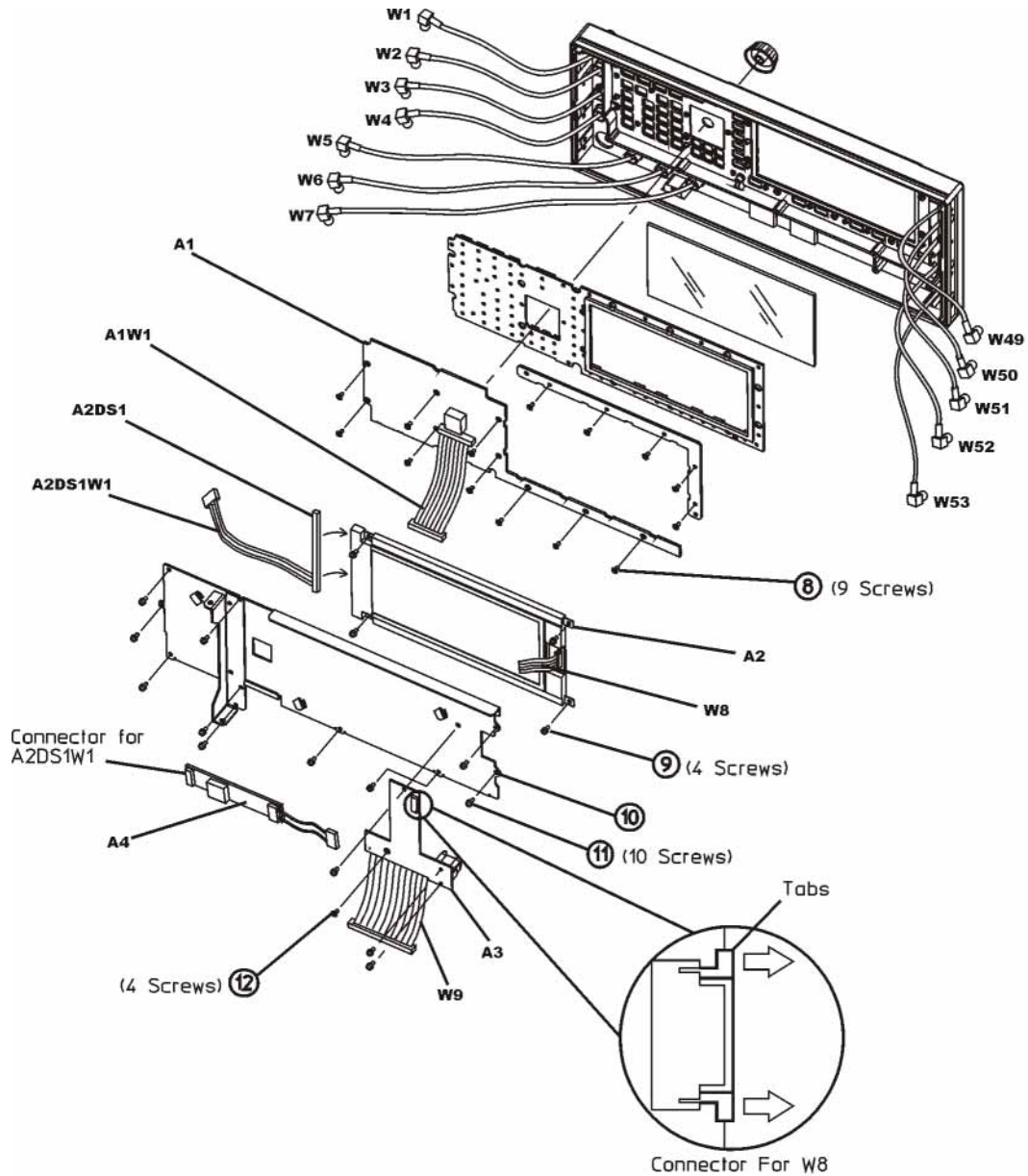
Figure 3-7 A2 Display Removal with serial prefixes < US/MY5XXX3XXX 1
