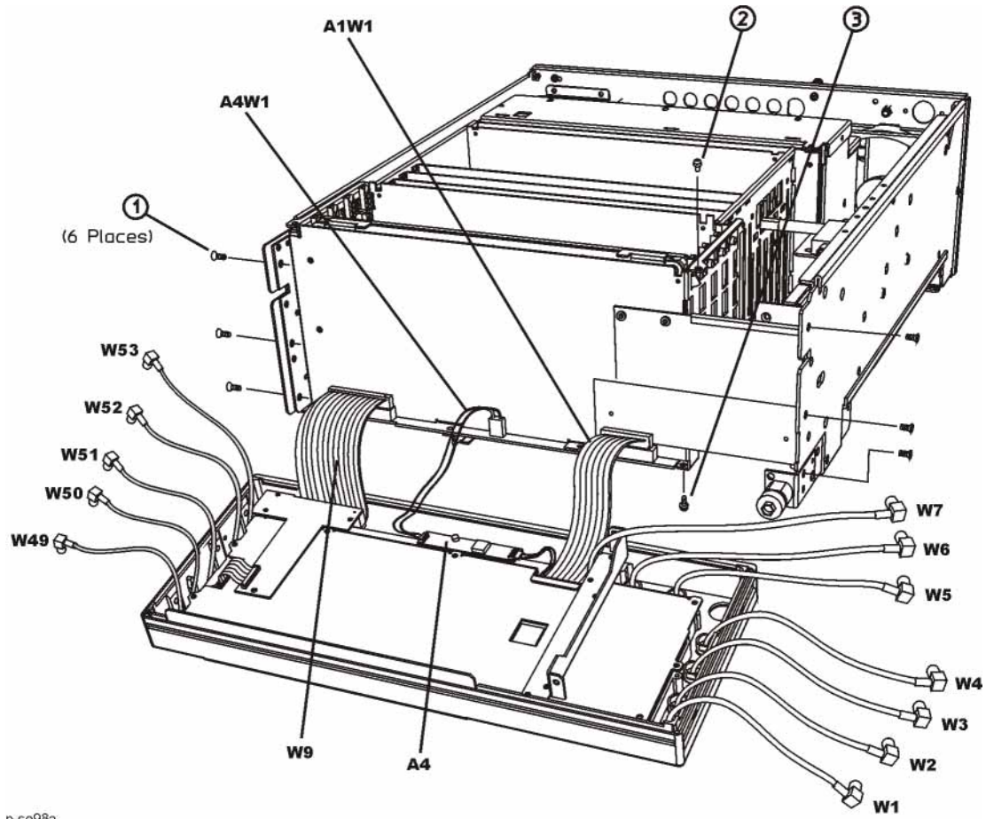
Figure 3-12 A4 Inverter Removal
