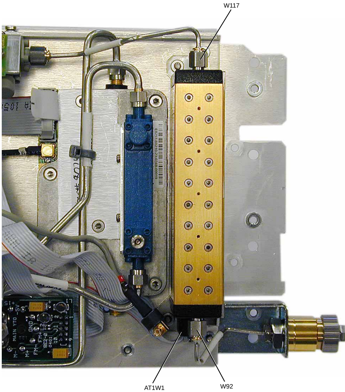
Figure 3-73 AT1 90 dB Attenuator
