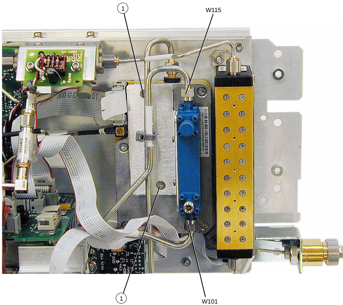
Figure 3-66 A39 Directional Sweep Coupler
