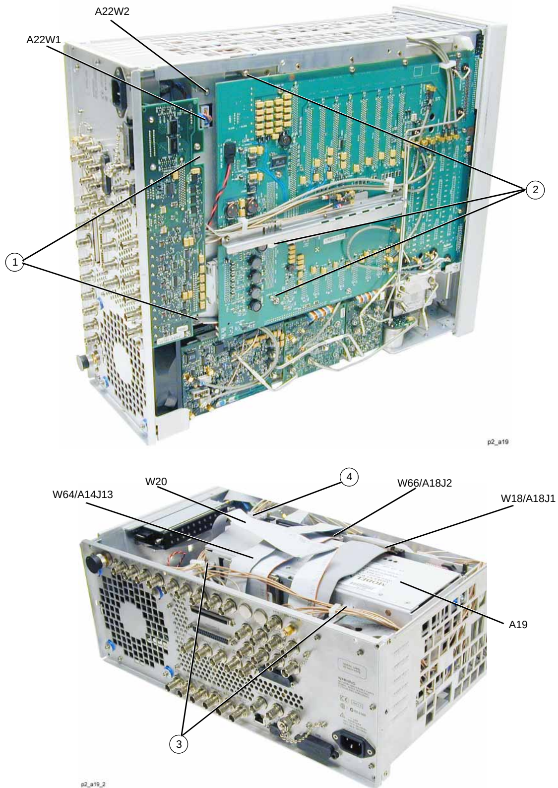
Figure 3-25 A19 Power Supply Removal
