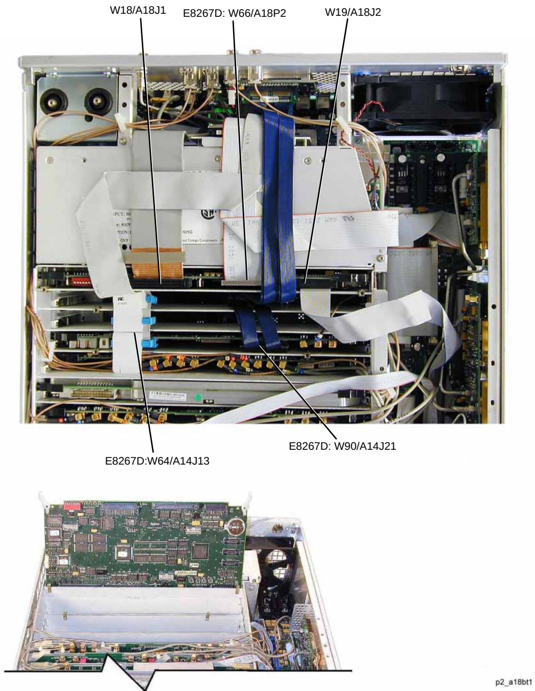
Figure 3-24 A18BT1
