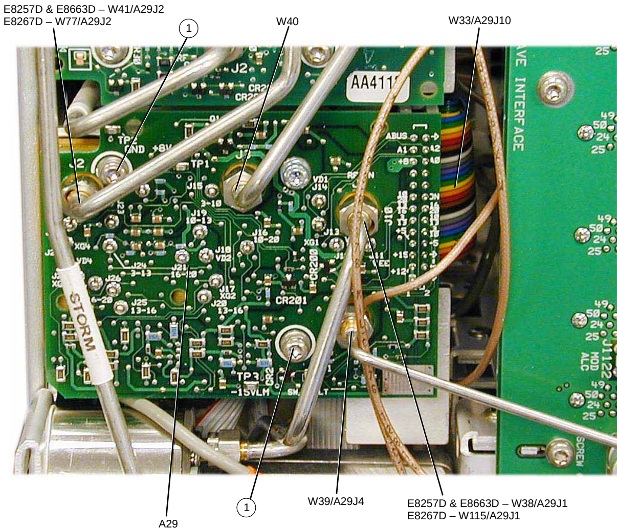
Figure 3-51 A29 20 GHz Doubler
