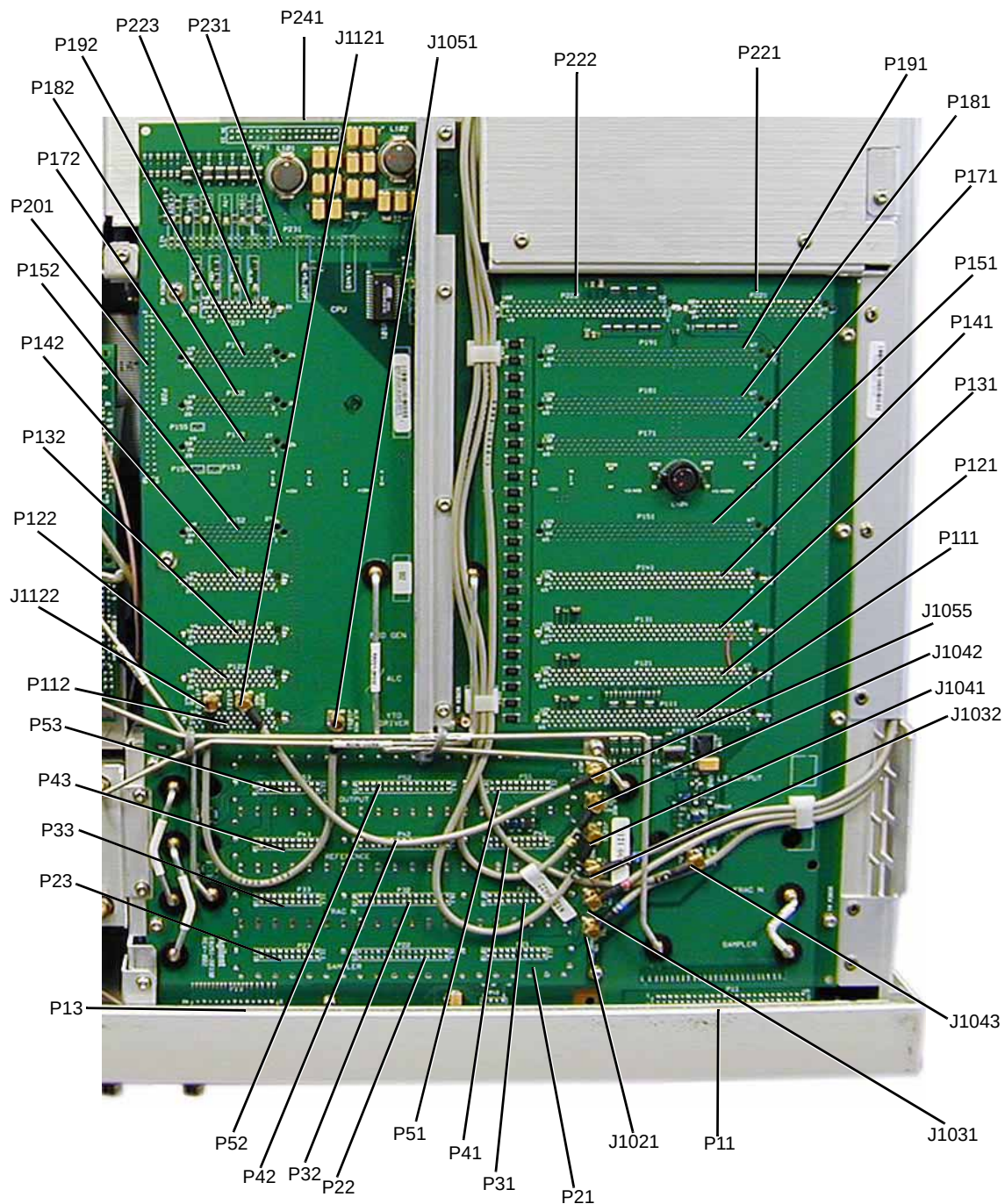
E8257D (Analog) Motherboard Connectors – Bottom View
