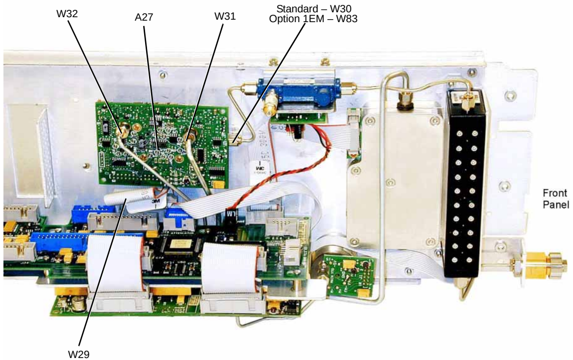
Figure 3-48 A27 40 GHz Doubler (Option 540)
