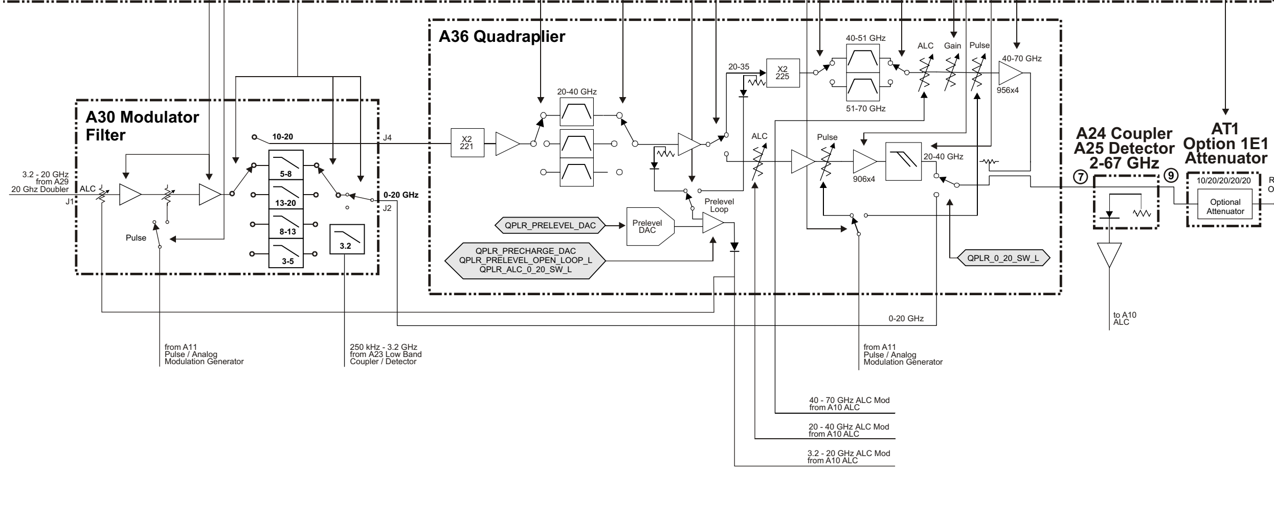
Quadrupler Block for the E8257D PSG Analog RF Path (Analog Models Over 40 GHz), Service Guide E8251-90359
