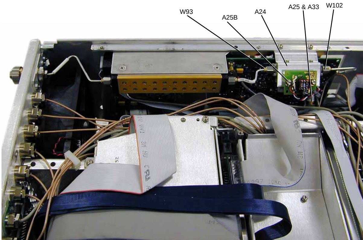
Figure 3-37 A24 50 GHz Highband Coupler (Options 532 & 544 – Option 1EM)
