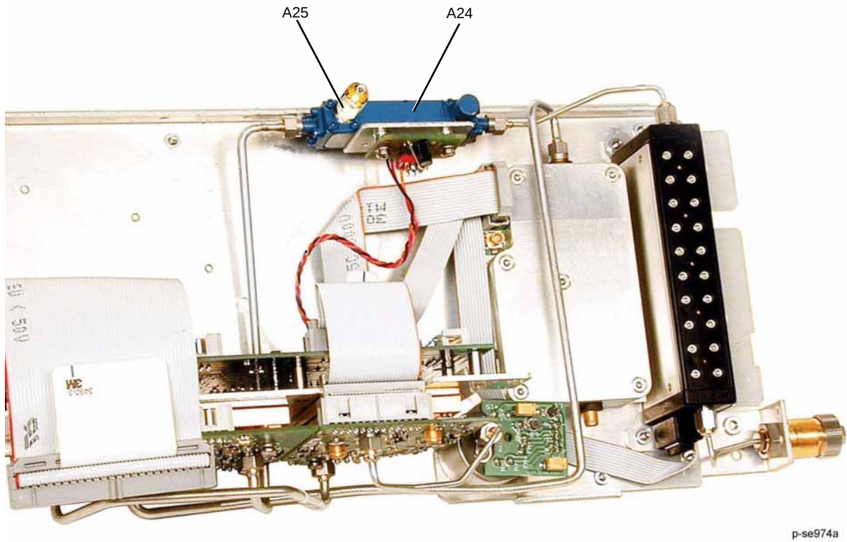
Figure 3-42 A25 40 GHz Highband Detector (Option 540)
