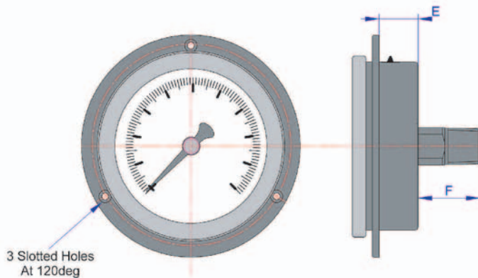
Front Flange Panel Mounting (FP)
