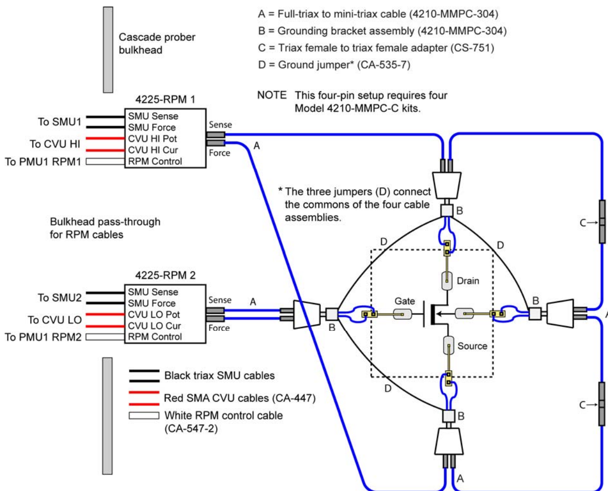
Figure 19: Test setup for four-terminal C-V testing
