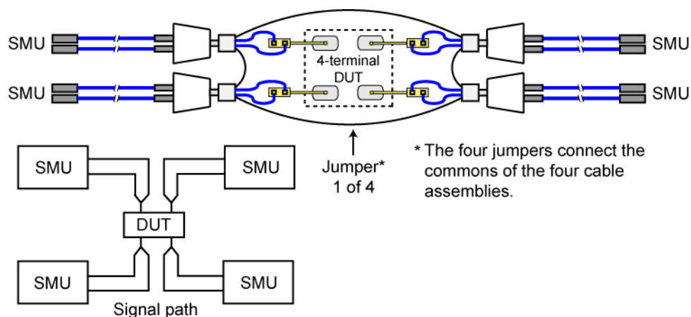
Figure 9: Test setup for 4-pin I-V testing
