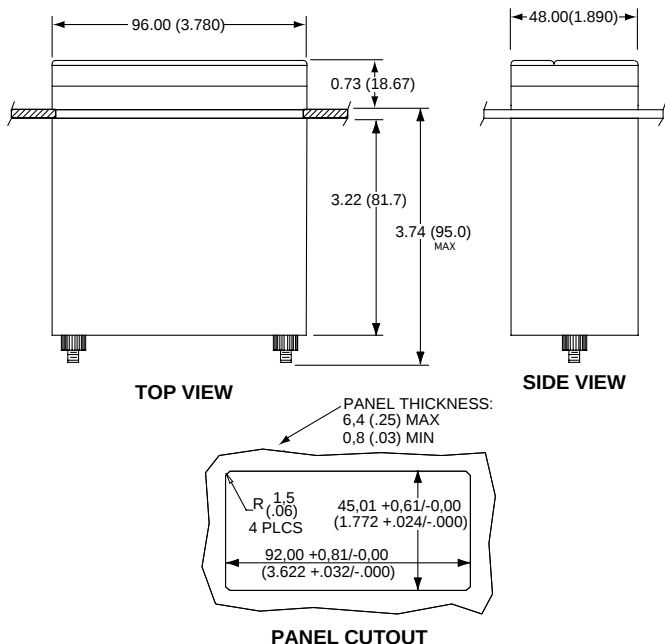
Figure 3.6 — Meter Dimensions
