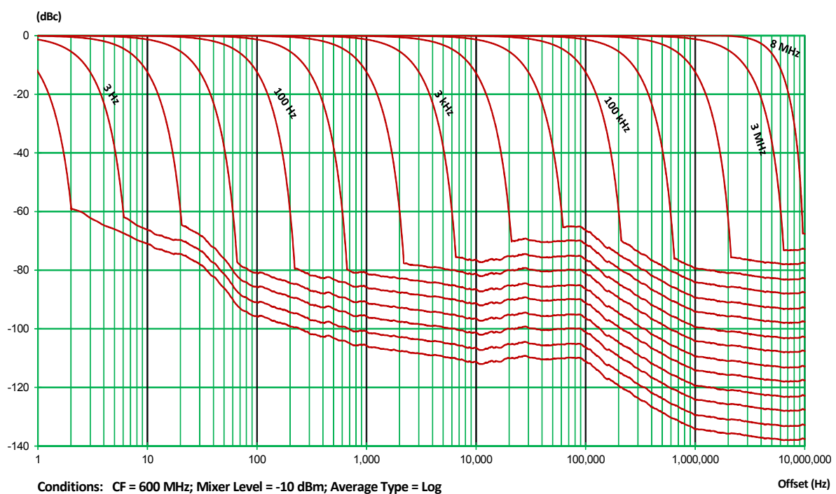
Nominal Dynamic Range vs. Offset Frequency vs. RBW [Plot] (Option 513/526)
