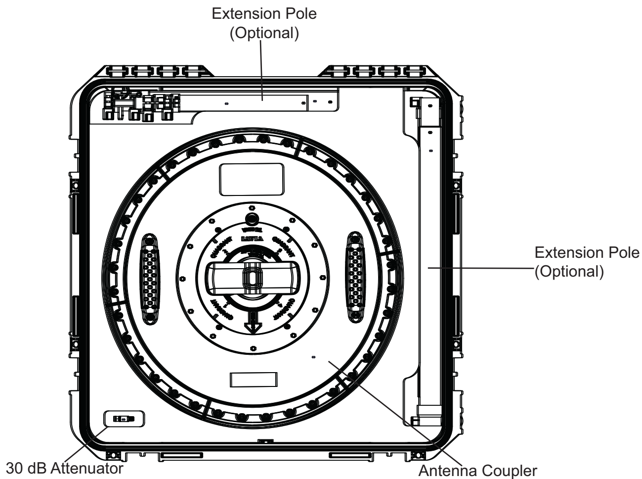
Figure 2 Transit Case
