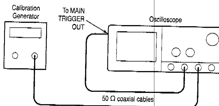
Figure 1–20: Initial test hookup
