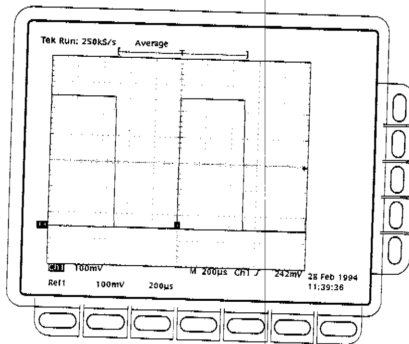
Figure 1-25: Measurement of probe compensator amplitude
