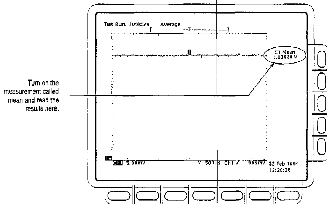
Figure 1-6: Measurement of DC accuracy at maximum offset and position
