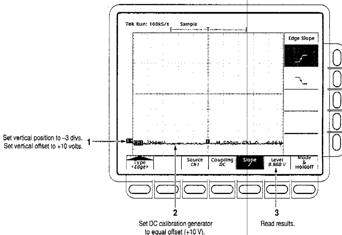
Figure 1-17: Measurement of trigger-level accuracy
