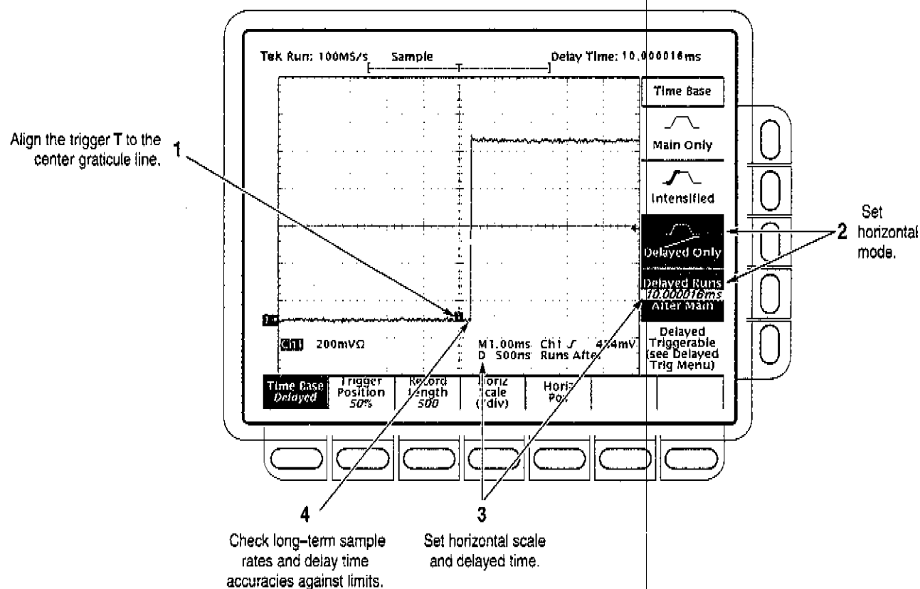
Figure 1-13: Measurement of accuracy – Long-term and delay time
