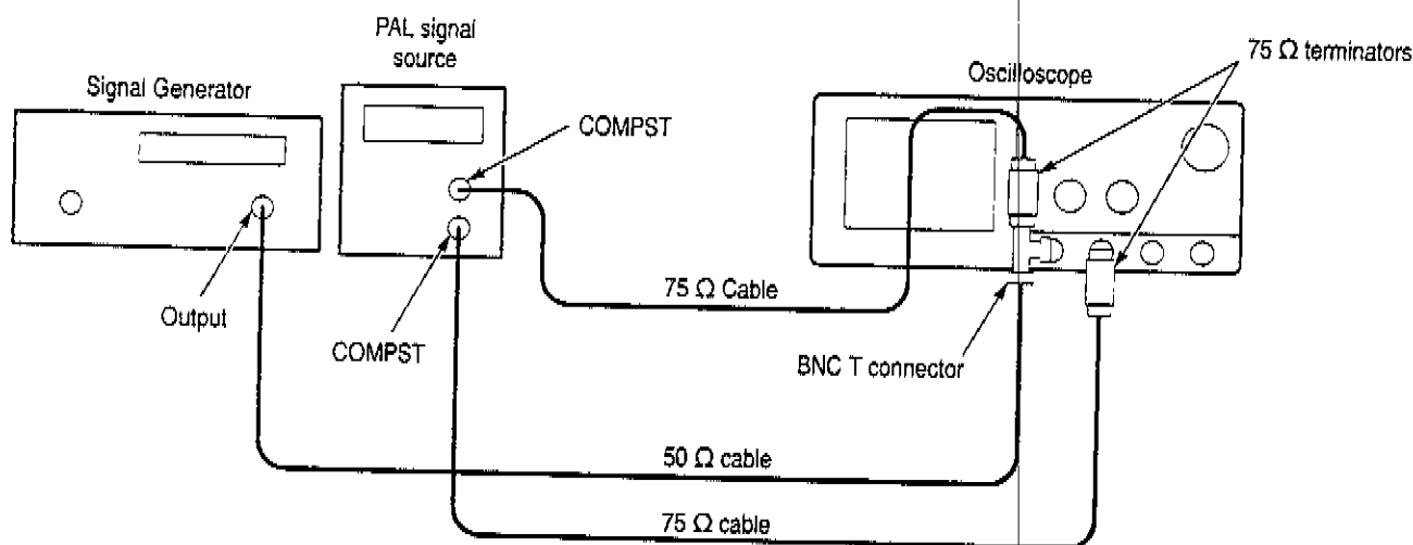
Figure 1-33: Subsequent 60 Hz Rejection test hookup
