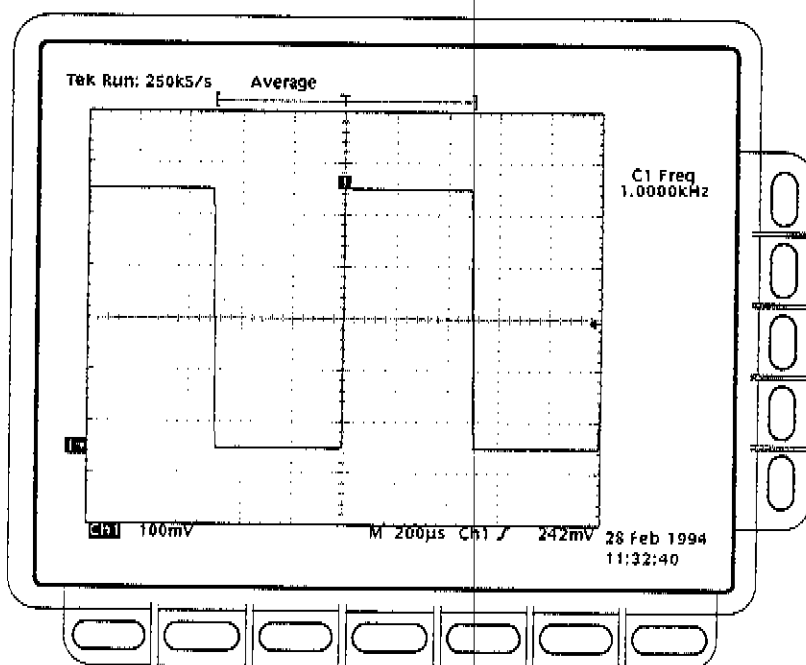
Figure 1-23: Measurement of probe compensator frequency
