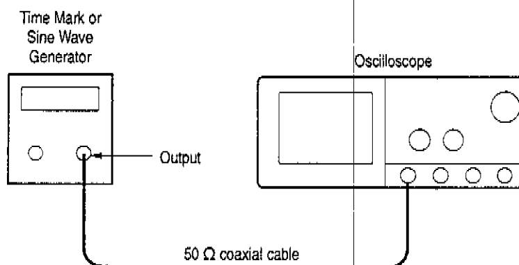
Figure 1-12: Initial test hookup
