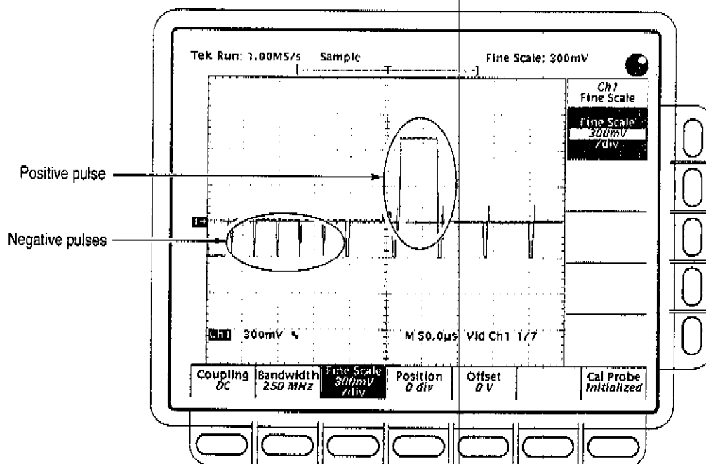
Figure 1-29: Triggered signal range test – 300 mV
