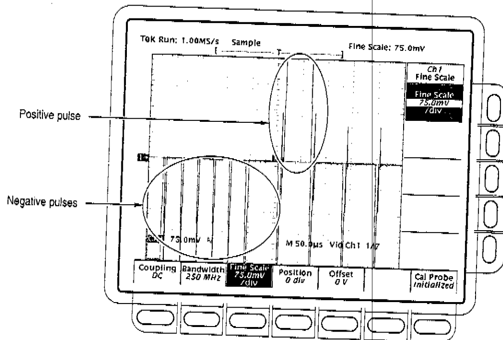
Figure 1-30: Triggered signal range test - 75 mV
