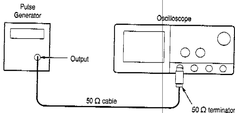
Figure 1-38: Setup for sync duty cycle test
