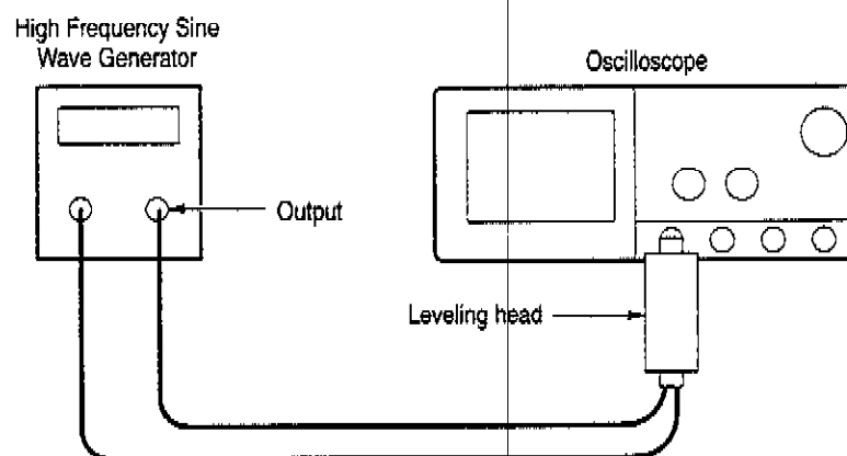
Figure 1-8: Optional initial test hookup
