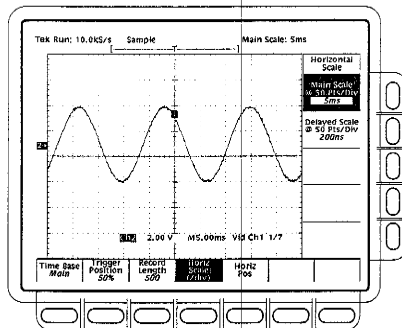
Figure 1-32: 60 Hz Rejection test setup signal
