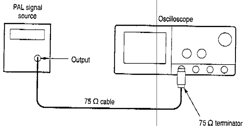
Figure 1-35: Line count accuracy test hookup
