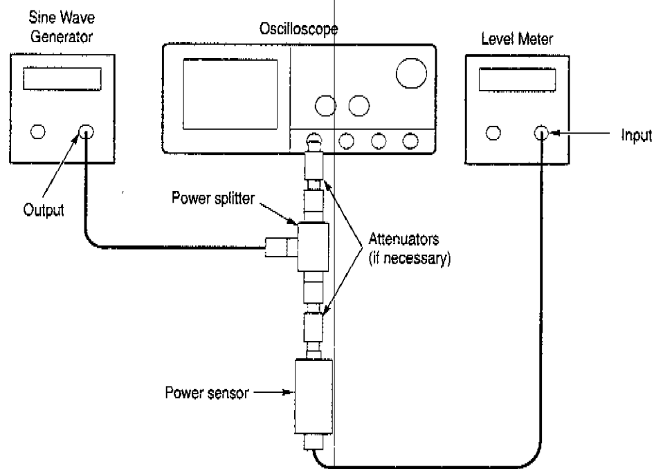
Figure 1-41: Sine wave generator leveling equipment setup
