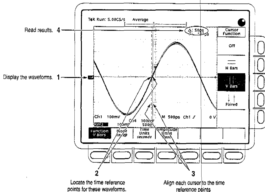
Figure 1-11: Measurement of channel delay – TDS 684B shown
