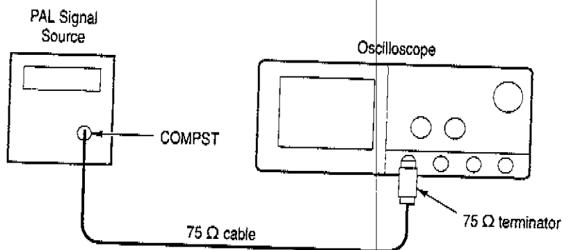
Figure 1-26: Jitter test hookup
