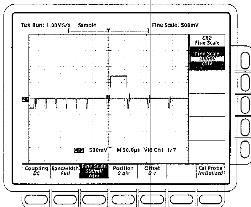
Figure 1-34: 60 Hz Rejection test result – TDS 684B shown
