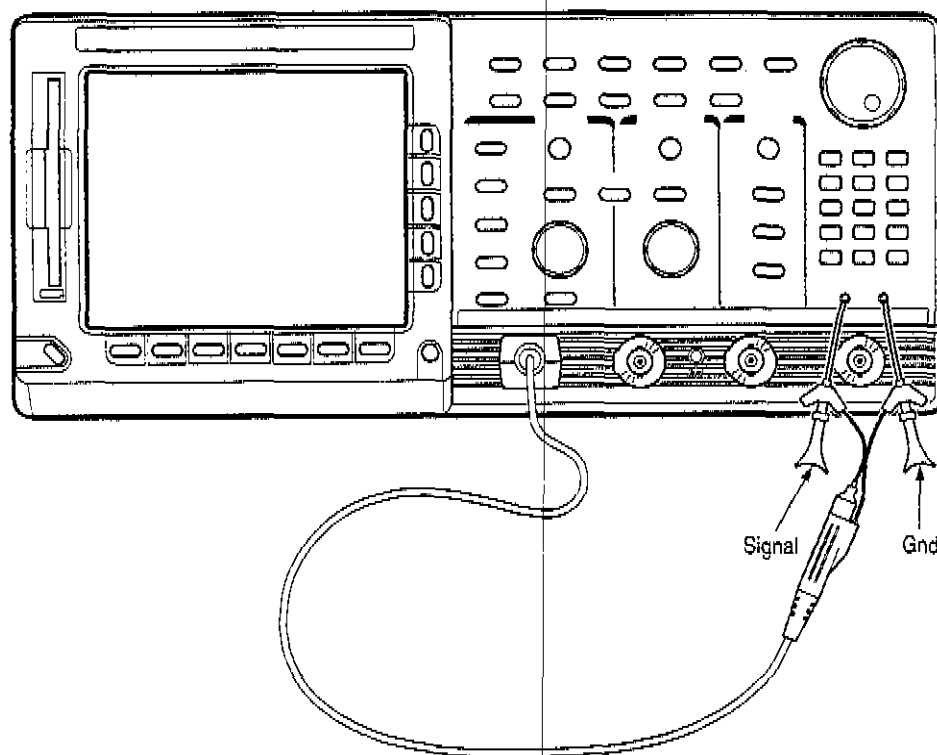
Figure 1-3: Universal test hookup for functional tests – TDS 600B shown
