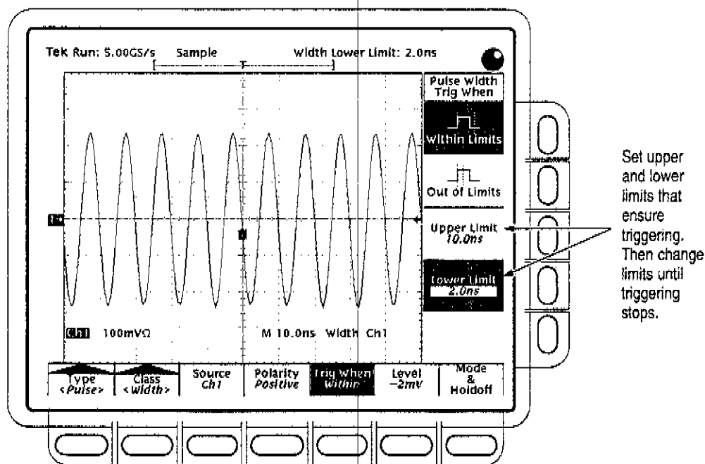
Figure 1-15: Measurement of time accuracy for pulse and glitch triggering
