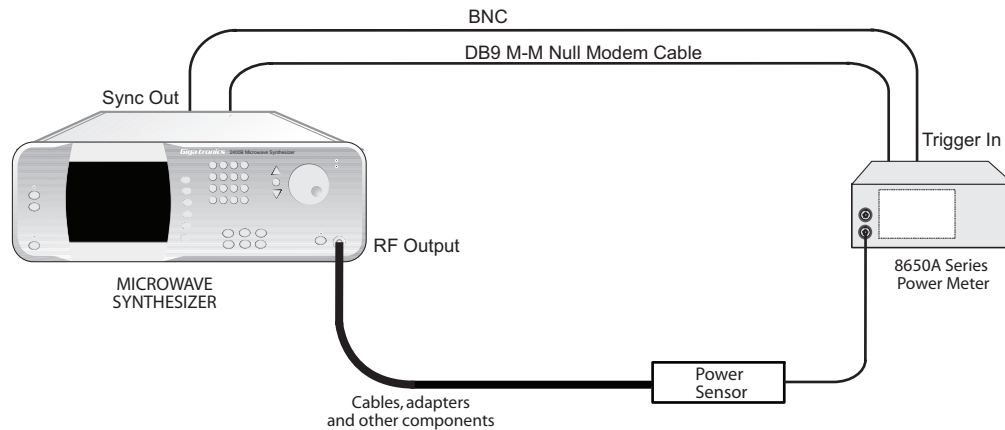
Figure 2-28: Cable Correction Set Up
