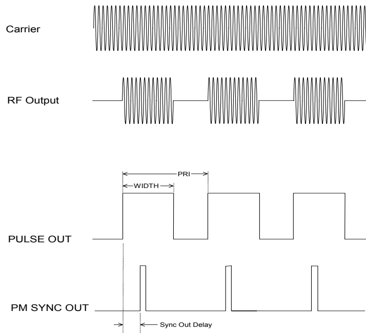
Figure 2-30: Internal Continuous Pulse Modulation
