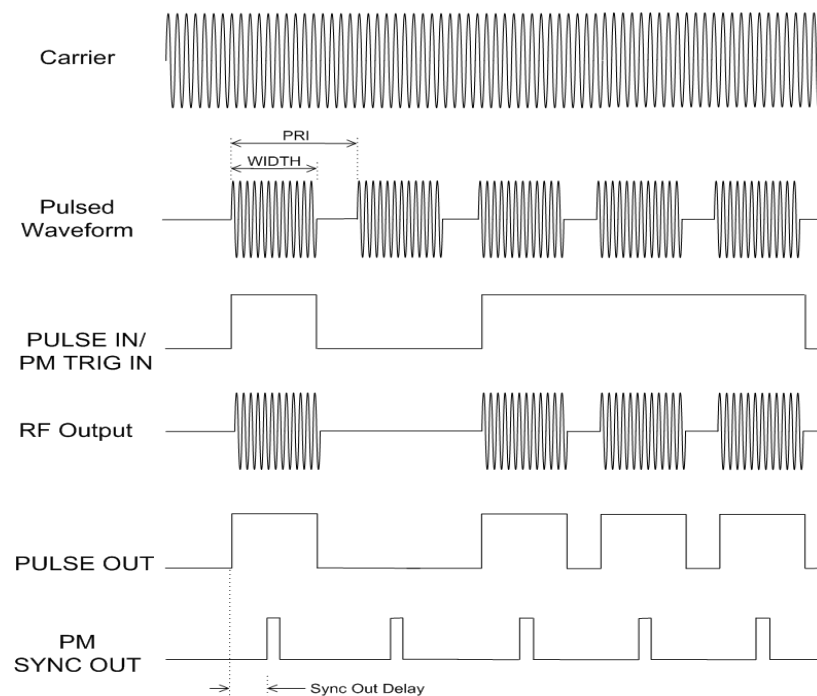
Figure 2-31: Internal Gated Pulse Modulation
