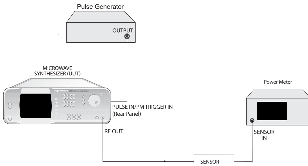
Figure 4-8: Pulse Modulation Level Accuracy Test
