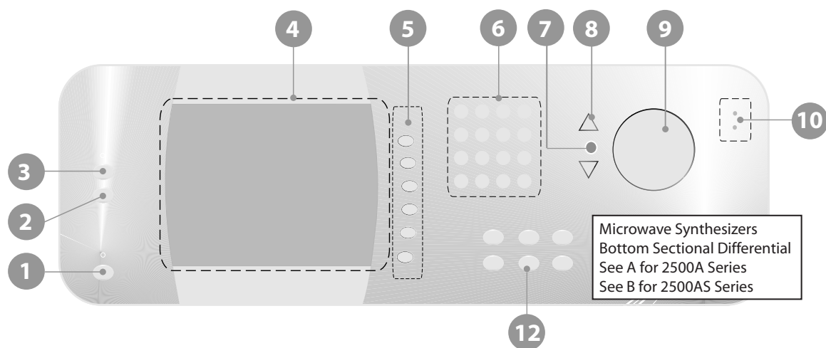
Front Panel Layout of 2500 Series Microwave Synthesizers
