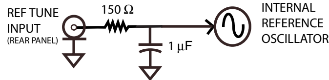
Figure 2-27: REF TUNE Input Circuit
