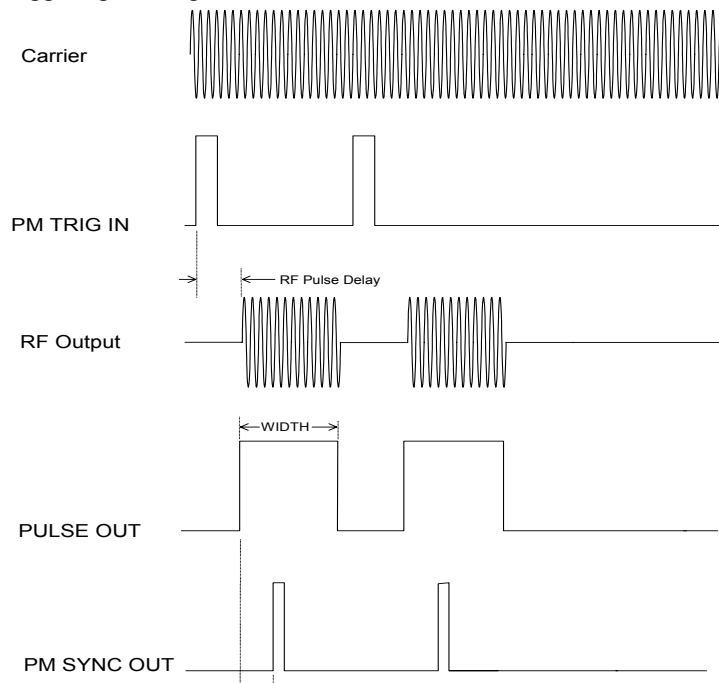
Figure 2-32: Internal Triggered Pulse Modulation
