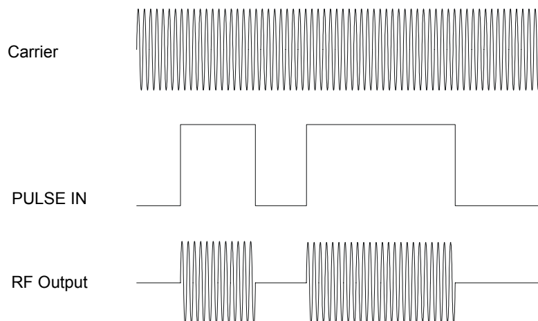
Figure 2-29: External Pulse Modulation
