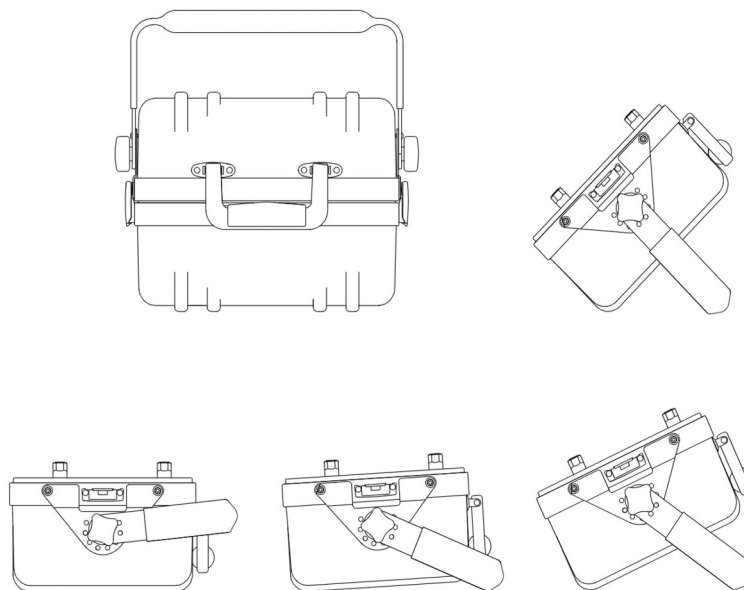
Figure B.1: Model 931A Case with Handle/Bail
