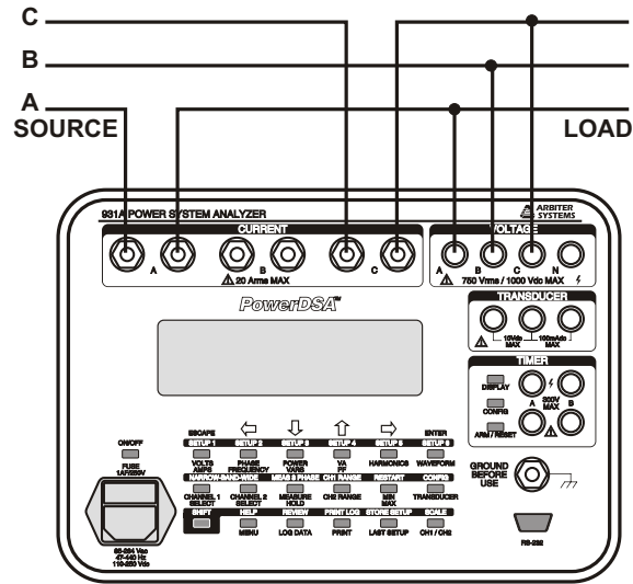
Figure 3.10: 3-Phase, 3-Wire, 2-Element Connections
