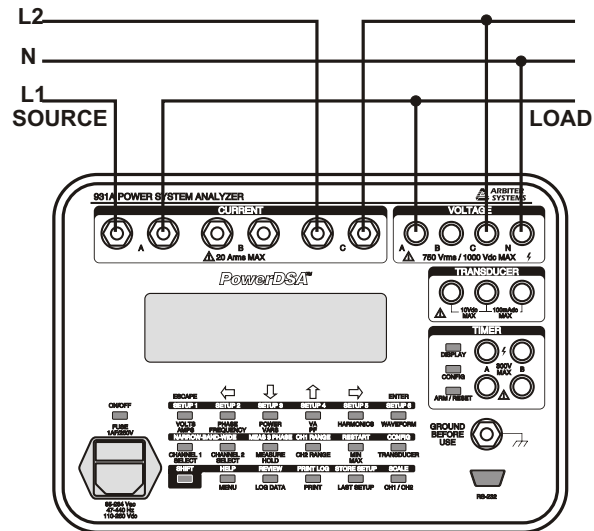
Figure 3.9: 1-Phase, 3-Wire, 2-Element Connections
