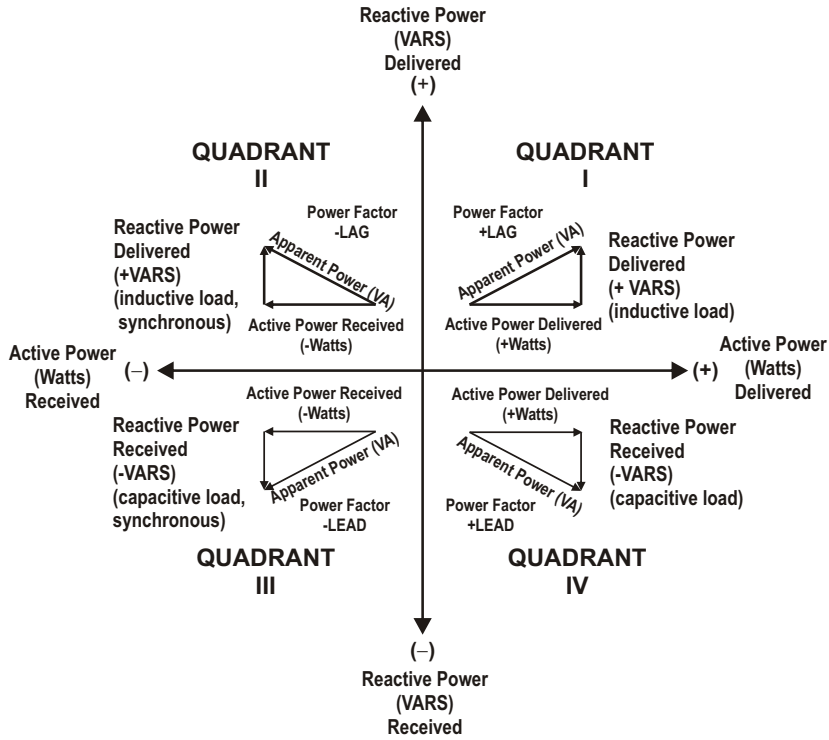
Figure 3.2: Phase, Power Factor, VAR Quadrants
