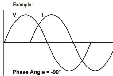
Figure 3.1: Phase, Power Factor, and VAR Definitions
