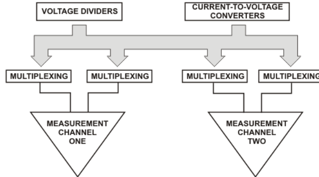
Figure 2.2: Input Multiplexing
