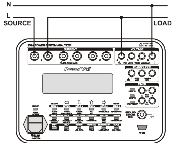
Figure 3.8: 1-Phase, 2-Wire, 1-Element Connections
