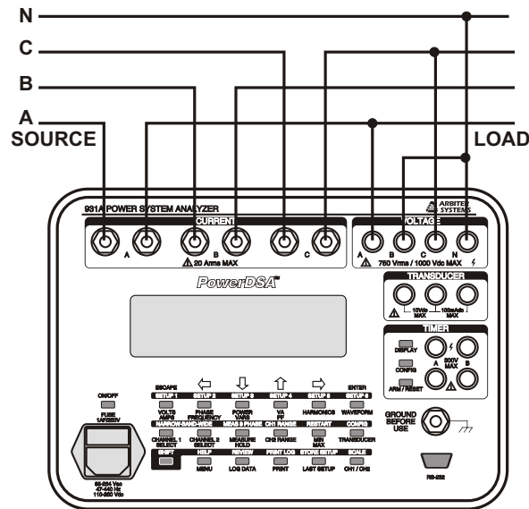
Figure 3.11: 3-Phase, 4-Wire, 2.5-Element Connections
