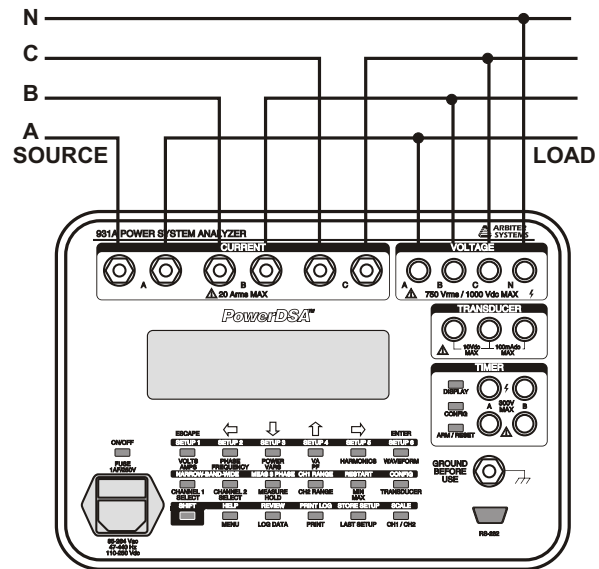
Figure 3.12: 3-Phase, 4-Wire, 3-Element Connections
