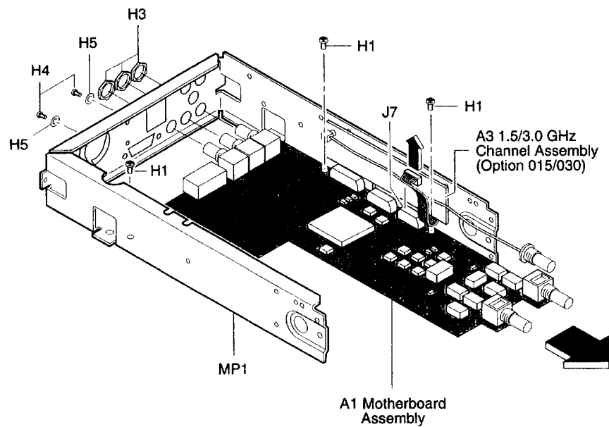
Figure 3-6. A1 Motherboard Assembly Removal
