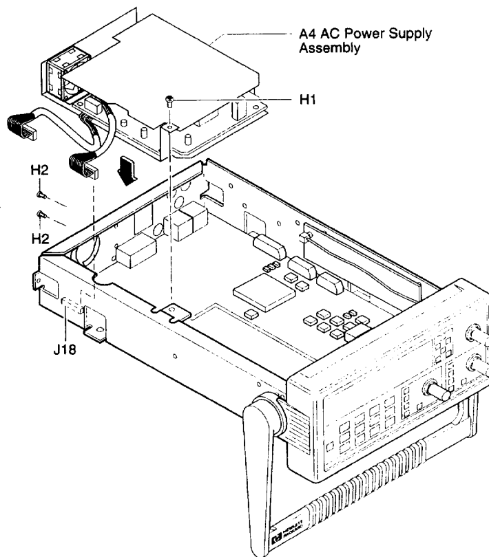
Figure 4-1B. DC Power Input Assembly Retrofitting
