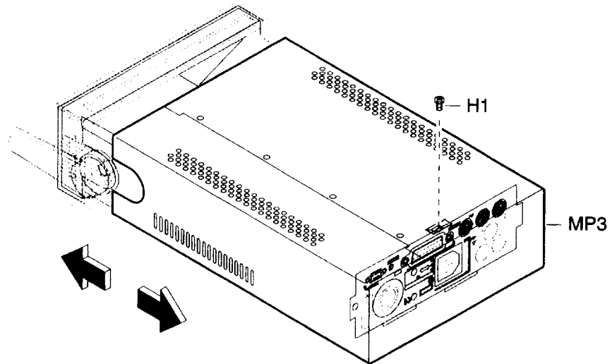
Figure 3-2. Bottom View for Cover Removal
