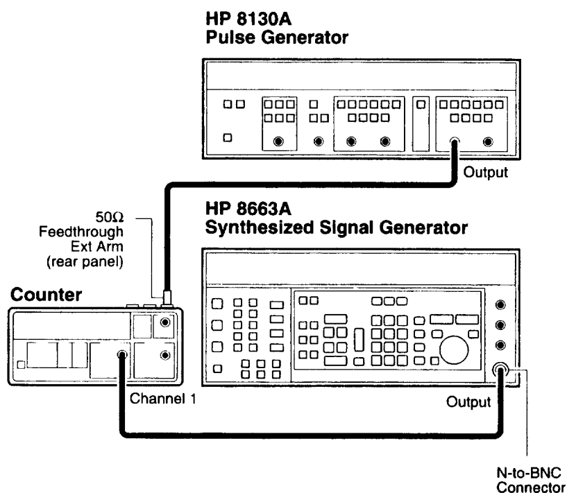
Figure 1-3. External Arm Test Setup (HP 53131A/132A Only)
