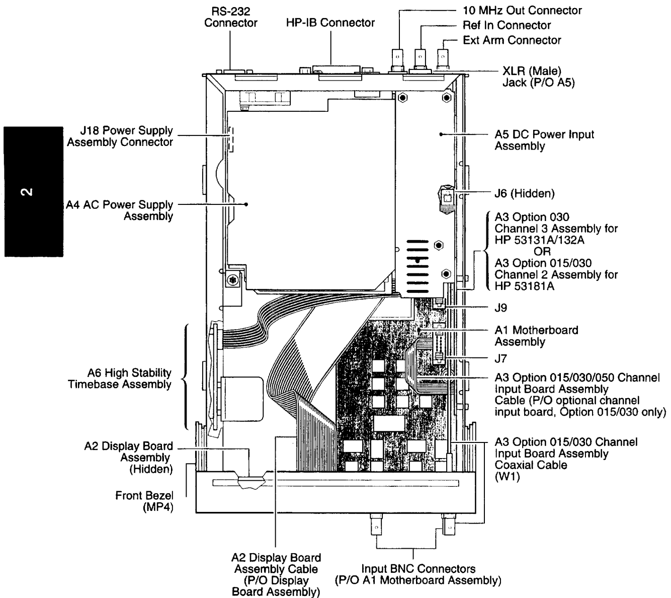
Figure 2-8B. Instrument Top Internal View (Option 002)
