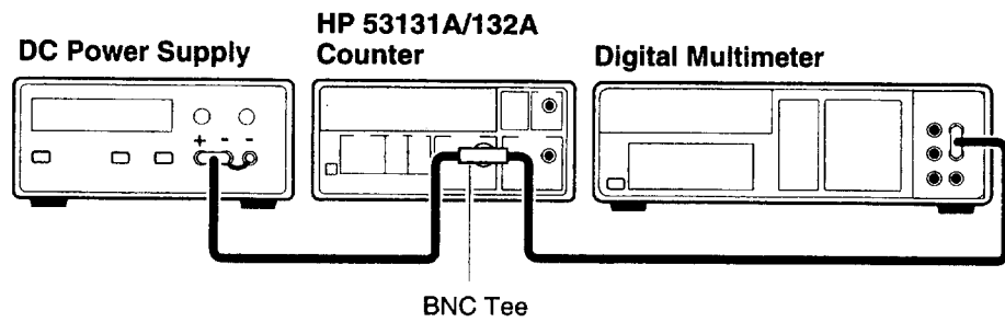
Figure 2-2. Gain Calibration Setup
