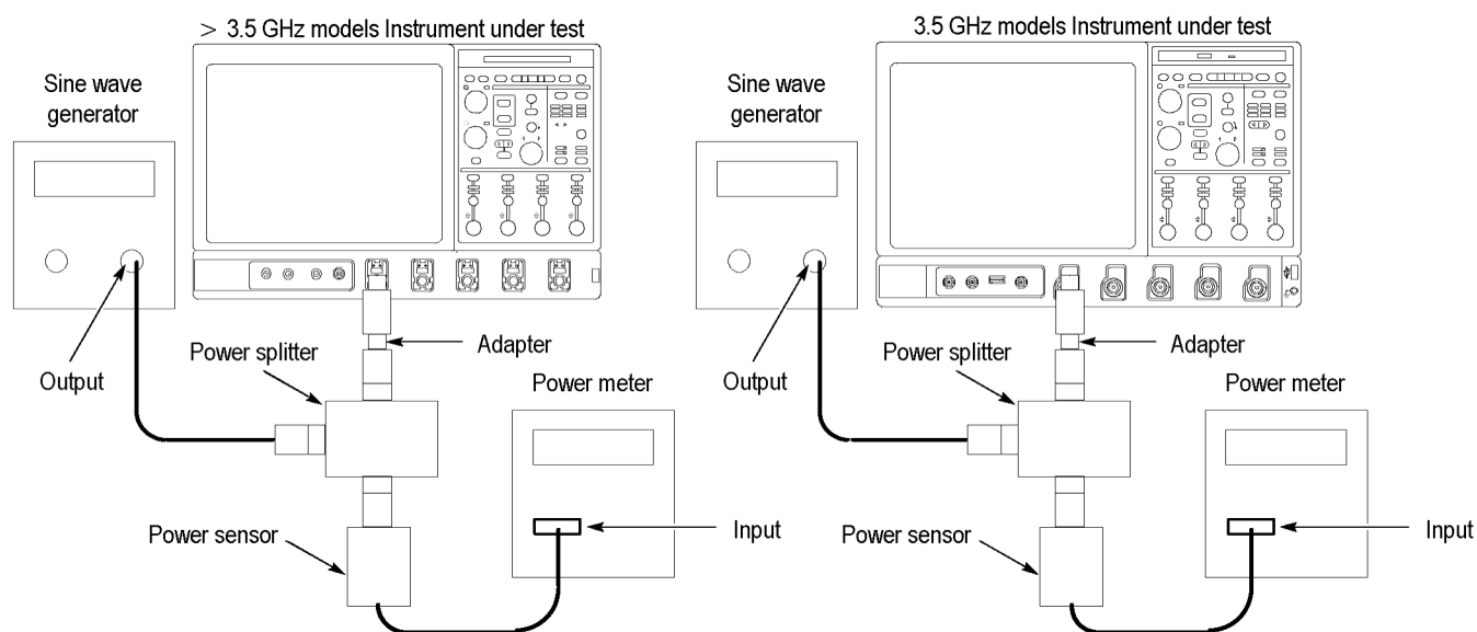
Figure 2-16: Initial test hookup
