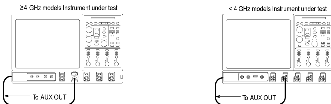
Figure 2-28: Initial test hookup
