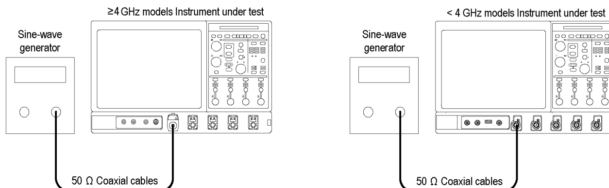
Figure 2-20: Initial test hookup
