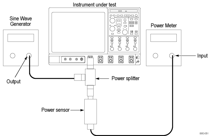
Figure 2-14: Initial test hookup
