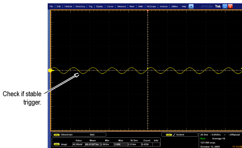
Figure 2-27: Measurement of trigger sensitivity - 50 MHz results shown
