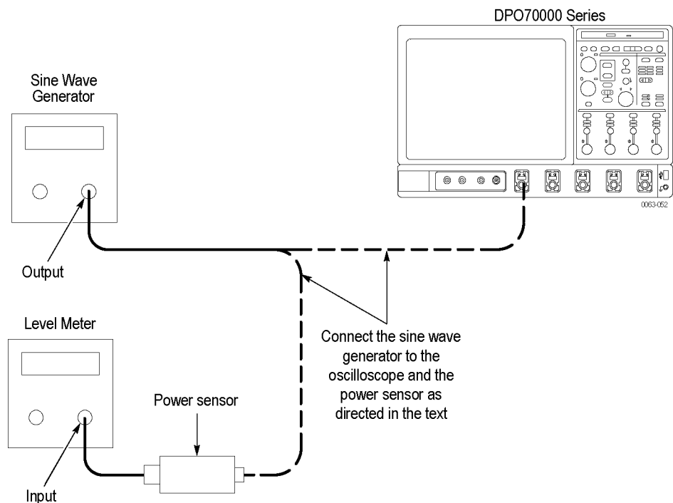
Figure 2-40: Equipment setup for maximum amplitude
