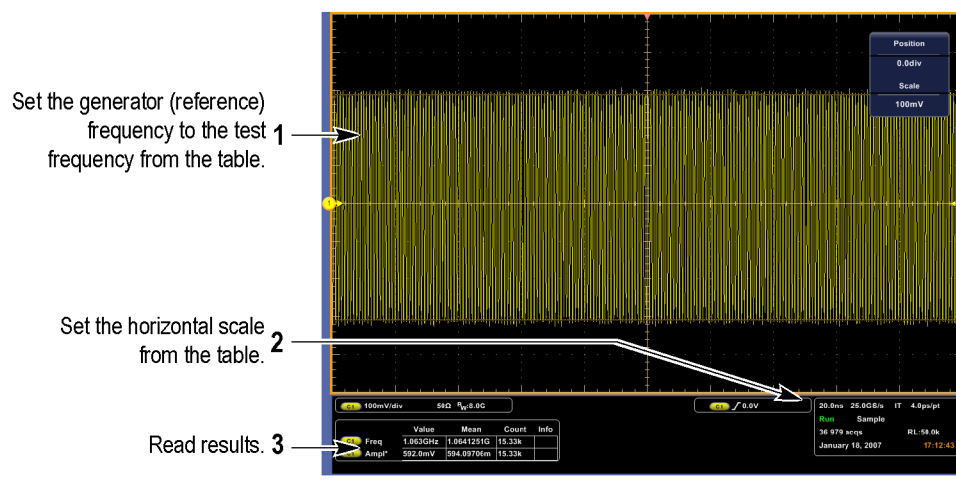
Figure 2-17: Measurement of analog bandwidth
