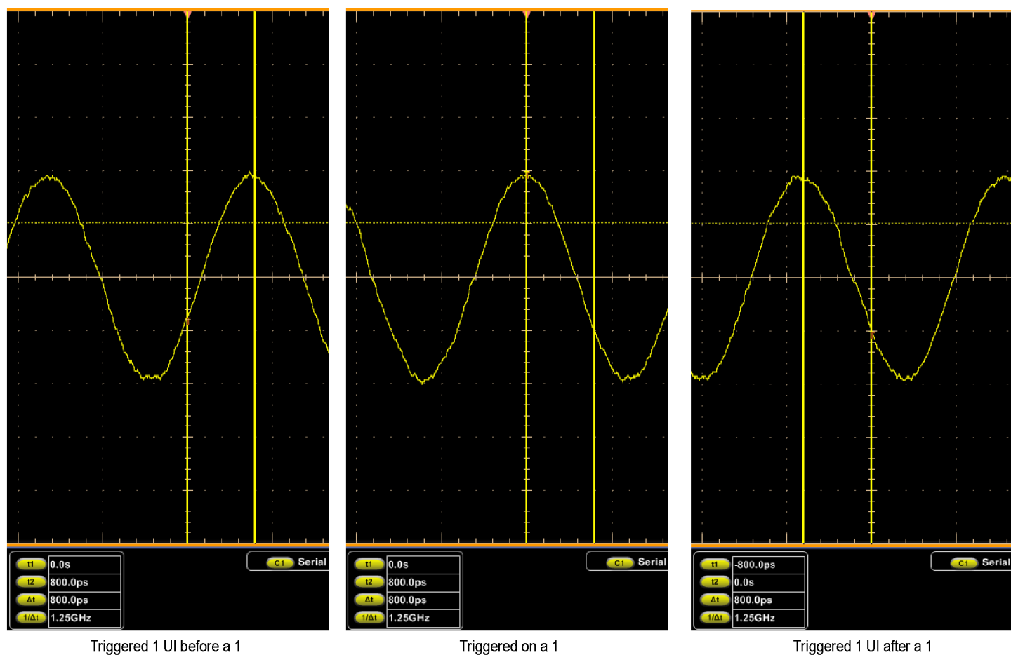
Figure 2-36: Isolated 1 triggering
