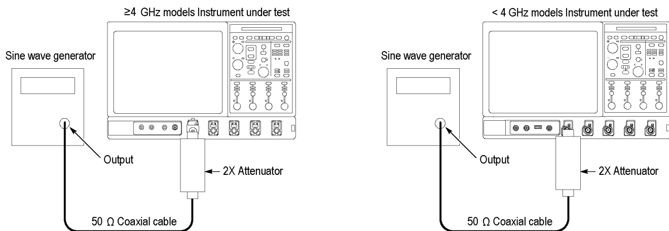
Figure 2-24: Initial test hookup
