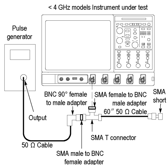
Figure 2-22: Delta time accuracy test hookup
