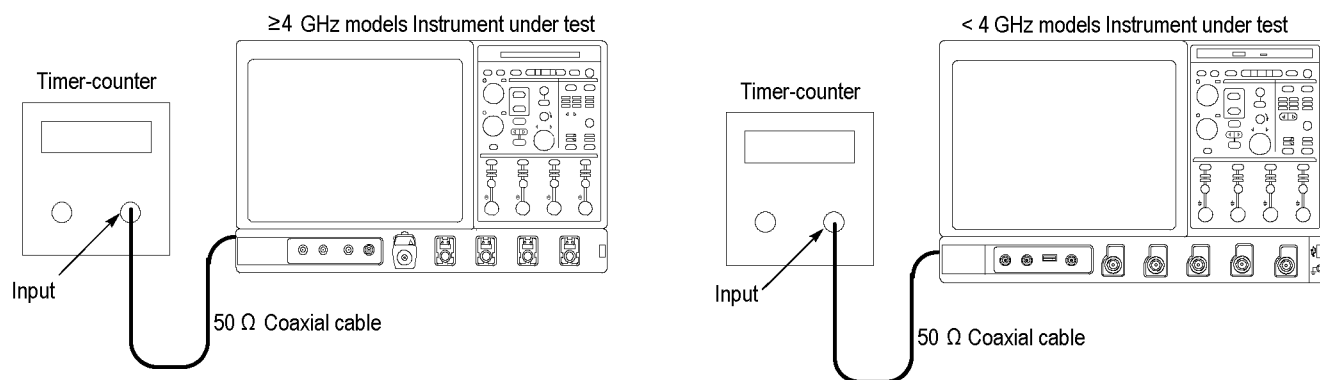
Figure 2-19: Initial test hookup
