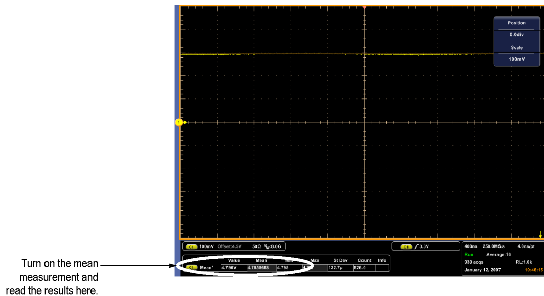
Figure 2-9: Measurement of DC accuracy at maximum offset and position
