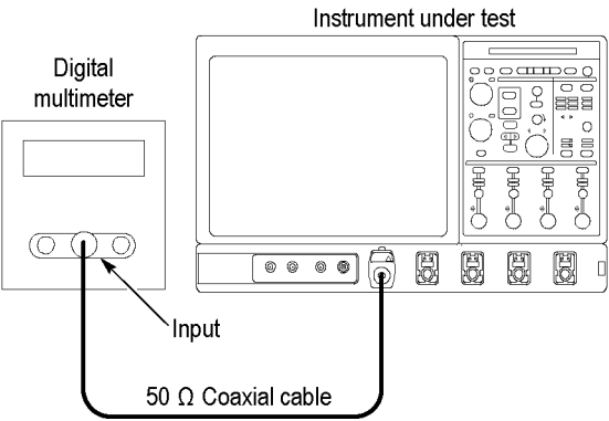
Figure 2-18: Initial test hookup
