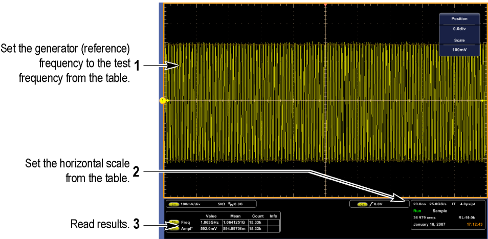
Figure 2-15: Measurement of analog bandwidth
