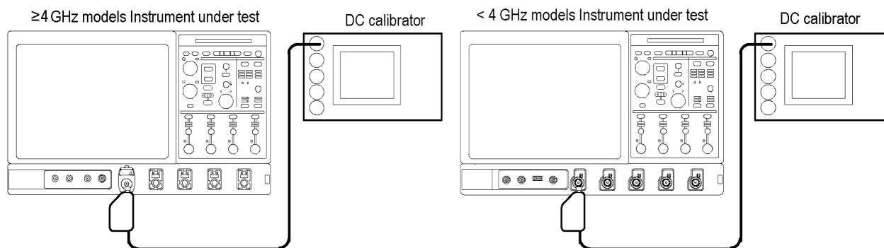
Figure 2-32: Subsequent test hookup
