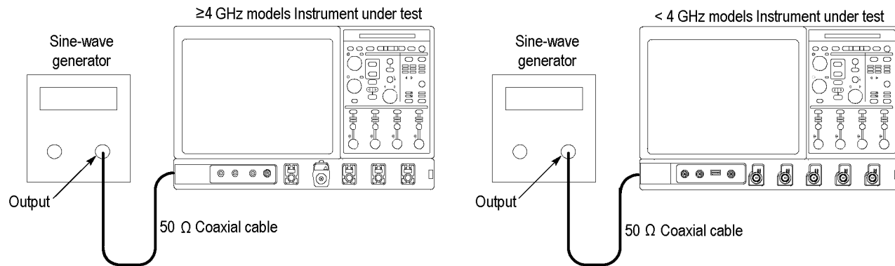
Figure 2-21: Final test hookup
