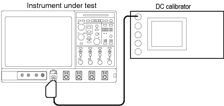
Figure 2-12: Initial test hookup
