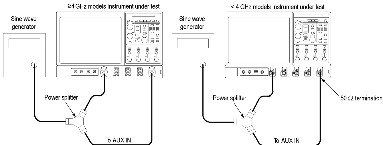
Figure 2-26: Initial test hookup
