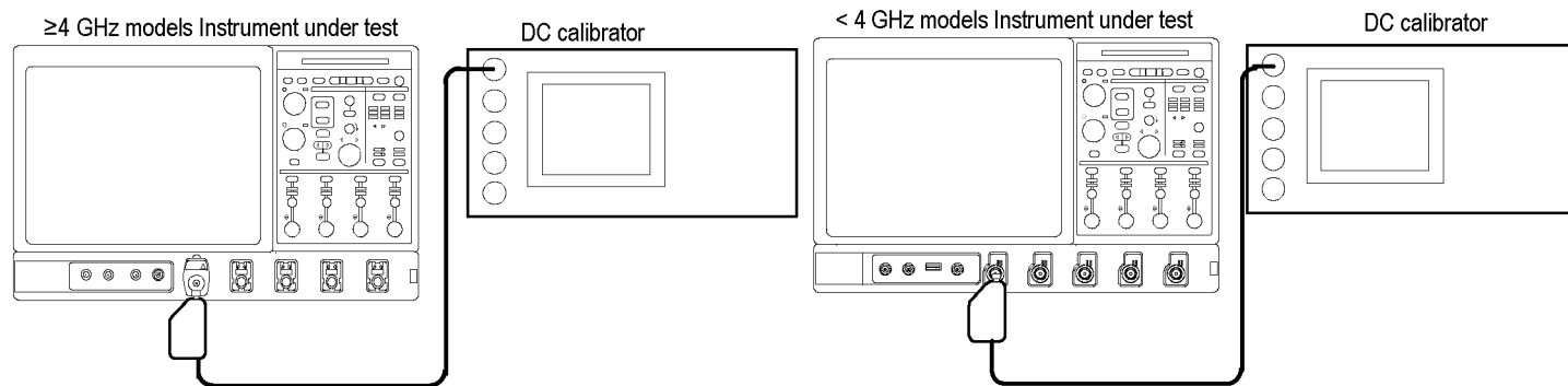
Figure 2-8: Initial test hookup
