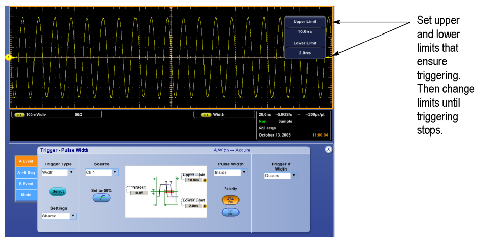
Figure 2-25: Measurement of time accuracy for pulse and glitch triggering
