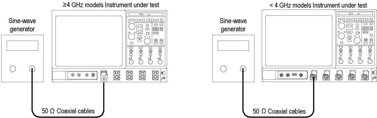
Figure 2-37: Initial test hookup
