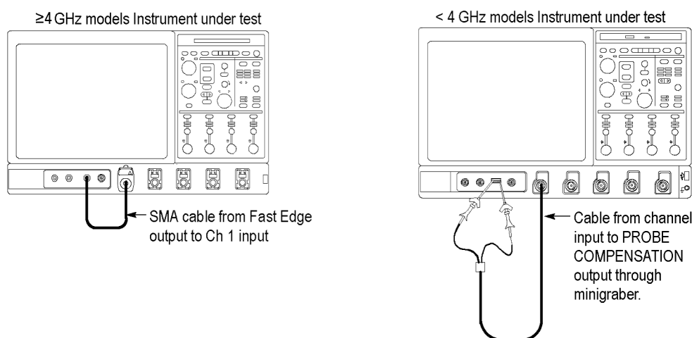
Figure 2-30: Initial test hookup
