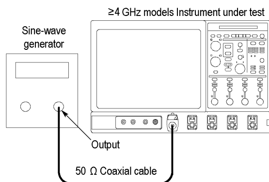
Figure 2-23: Delta time accuracy test hookup
