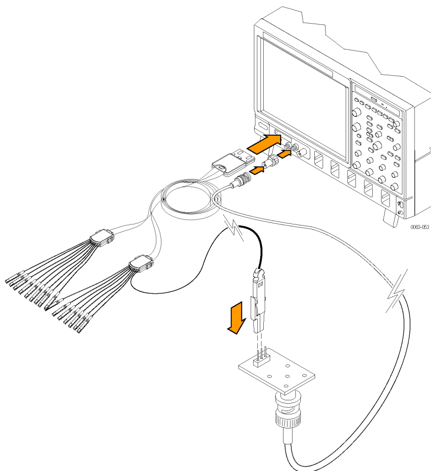
Figure 2-7: Setup for the digital channels test
