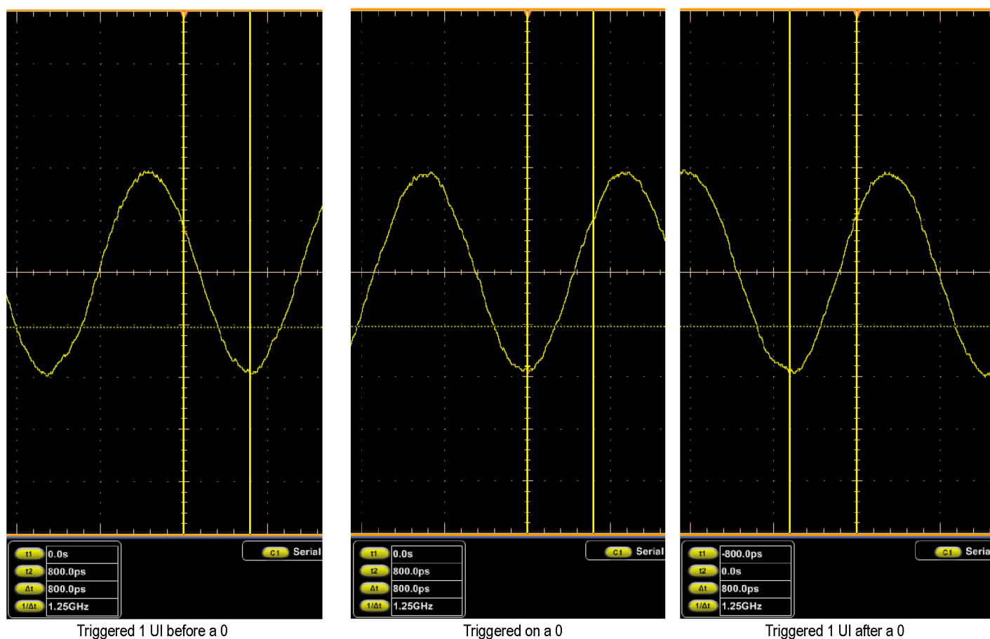
Figure 2-35: Isolated 0 triggering
