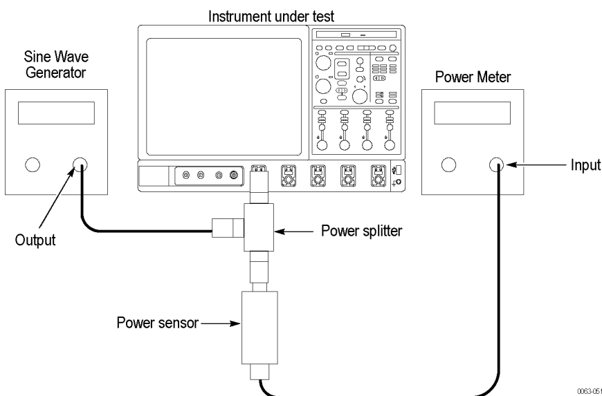
Figure 2-39: Sine wave generator leveling equipment setup
