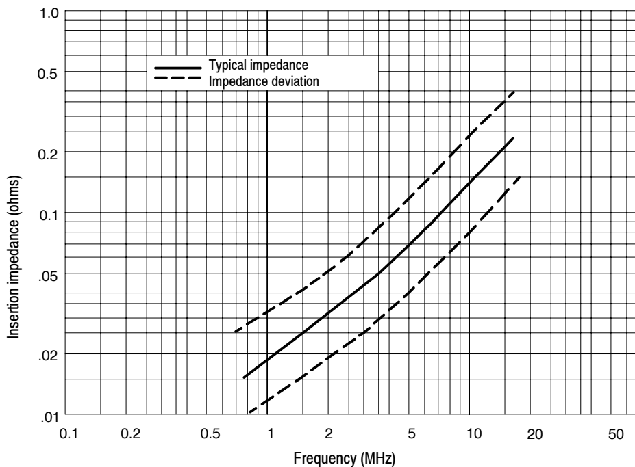
Figure 6: A6303 and A6303XL insertion impedance curve
