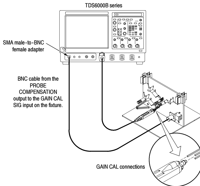
Figure 3-1: Universal test hookup for functional tests - CH 1 shown
