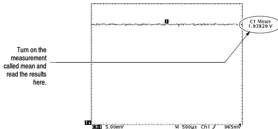
Figure 4-2: Measurement of DC accuracy at maximum offset and position
