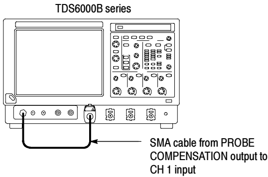
Figure 4-23: Initial test hookup
