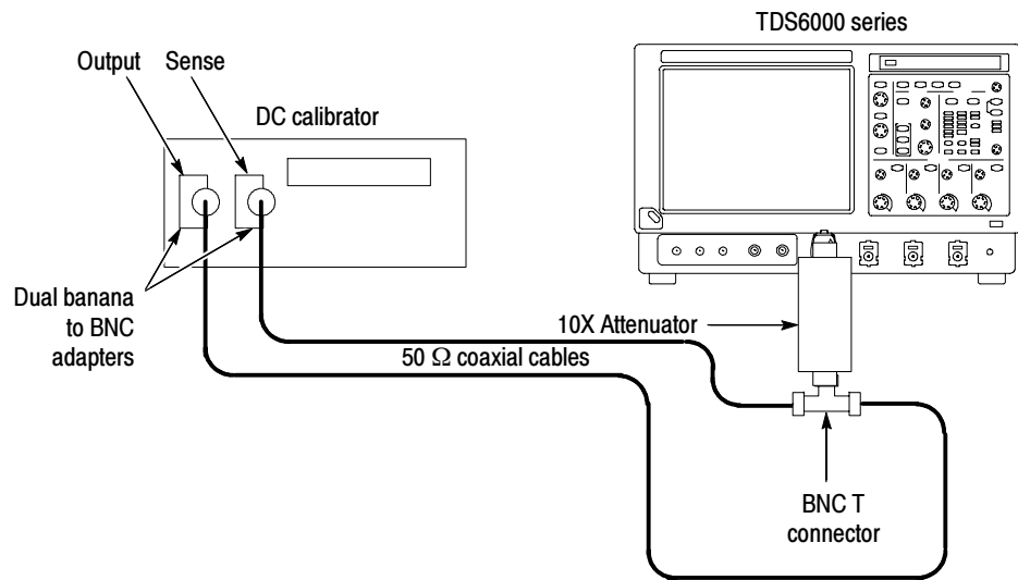
Figure 4-5: Initial test hookup
