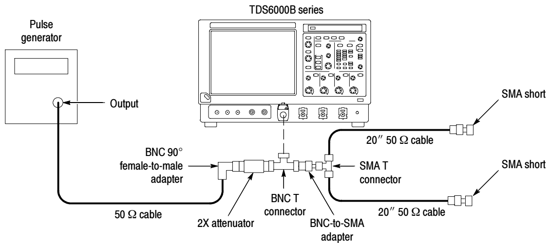
Figure 4-16: Delta time accuracy test hookup
