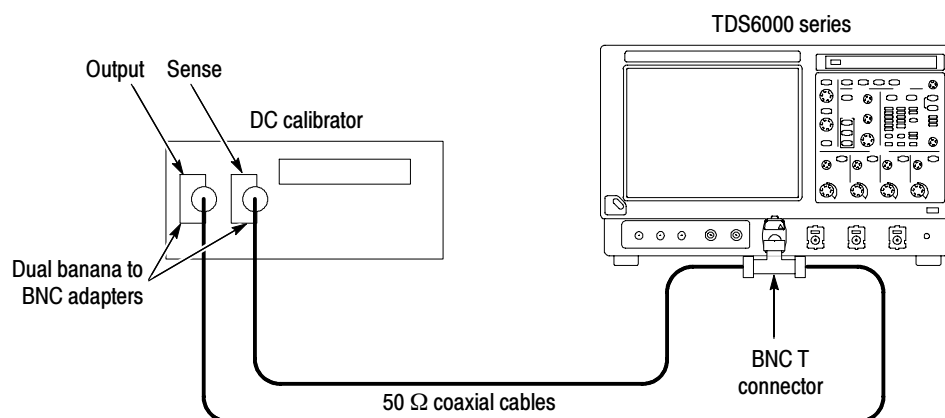
Figure 4-3: Initial test hookup
