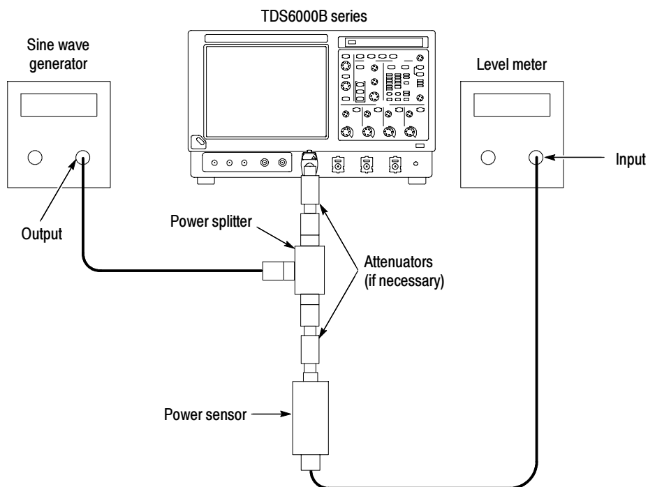
Figure 4-33: Sine wave generator leveling equipment setup
