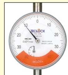
Dial Indicator used. For outer frame diameter φ55-φ59. It can be used for TM-110 / TM-1201
