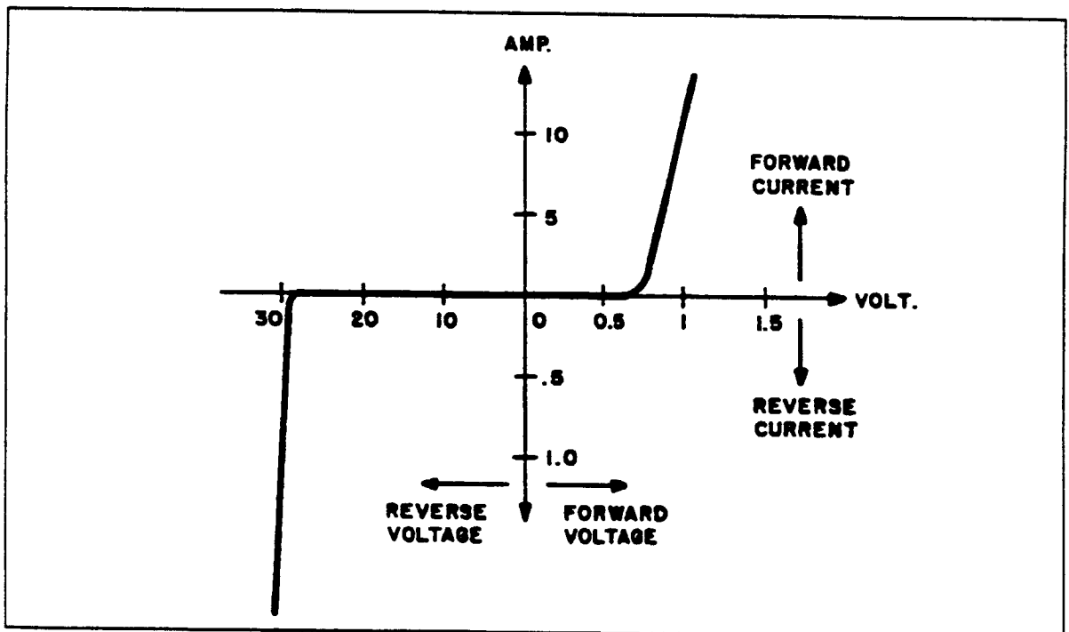
Figure 8-20. Characteristics of a Typical 30V Zener Diode.
