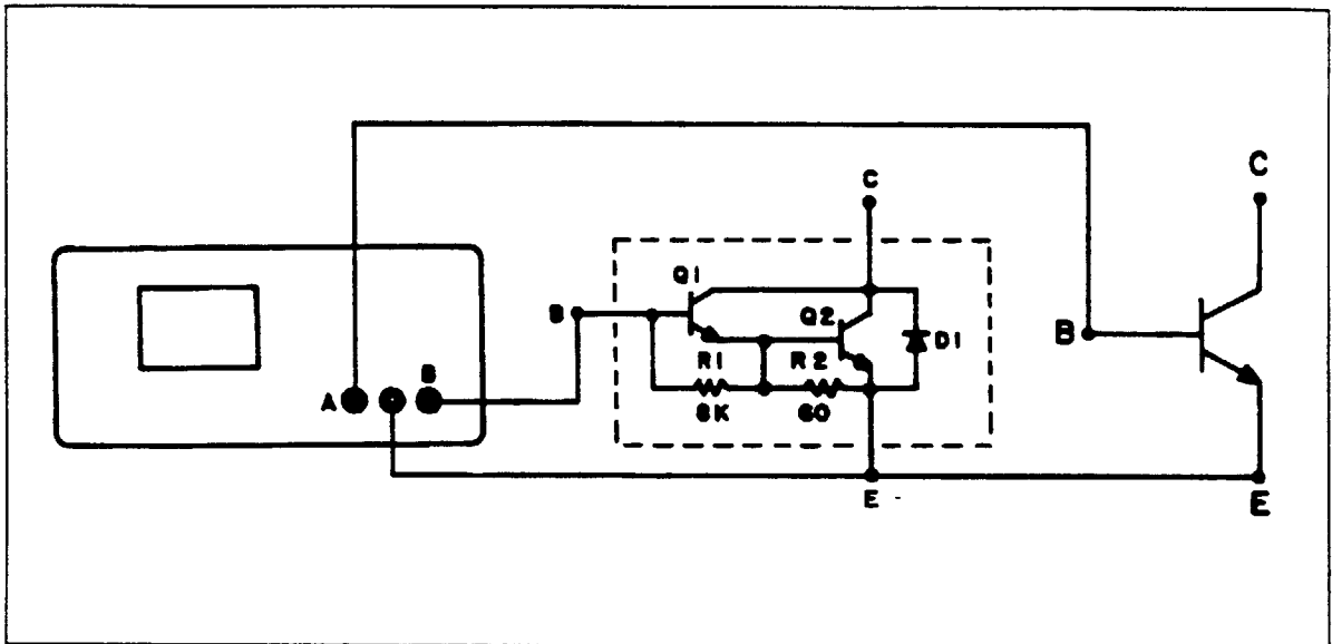
Figure 9-14. Base-Emitter Test Circuit.
