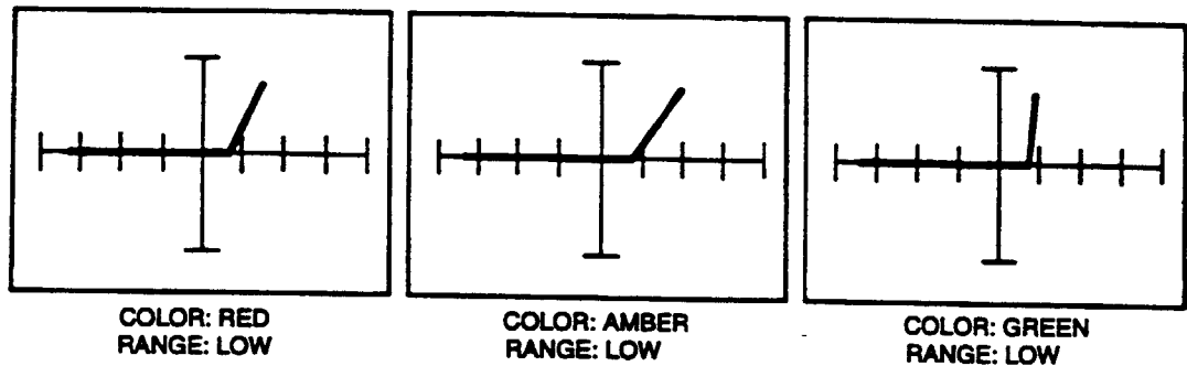
Figure 8-19. LED Signatures.
