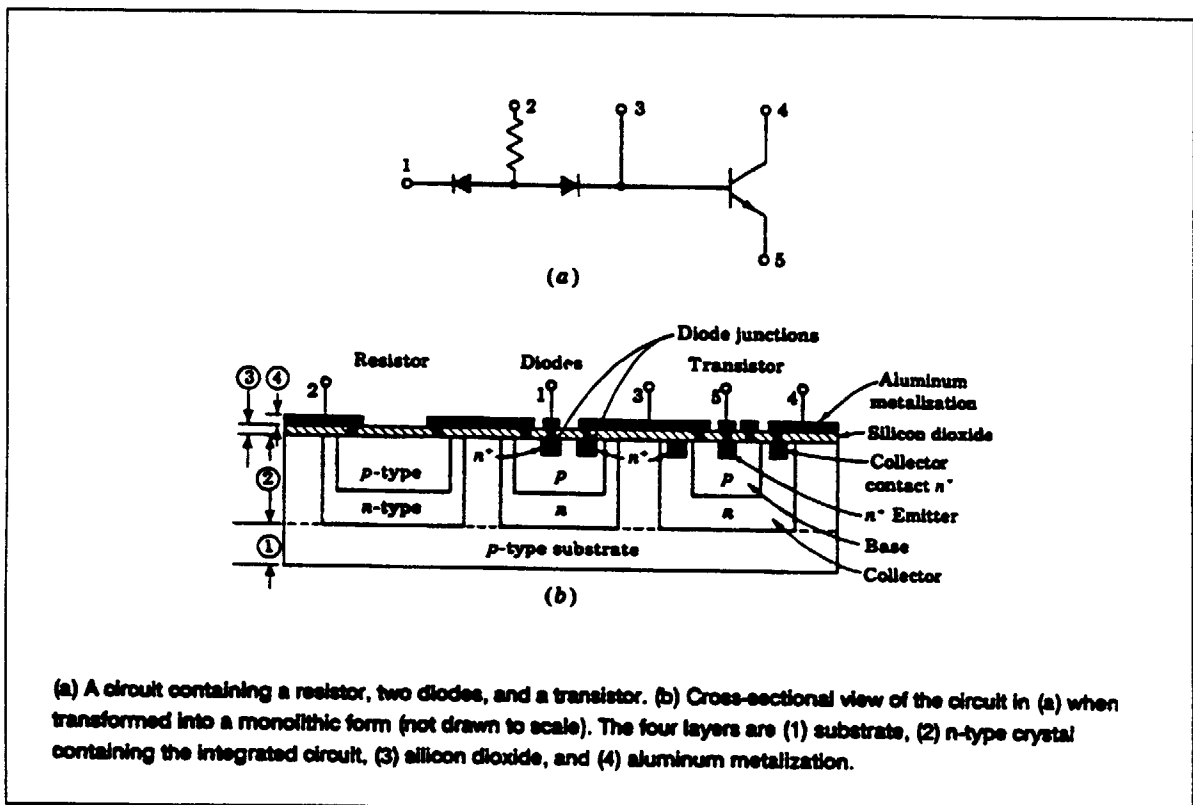
Figure 12-1. Typical Integrated Circuit Construction.
