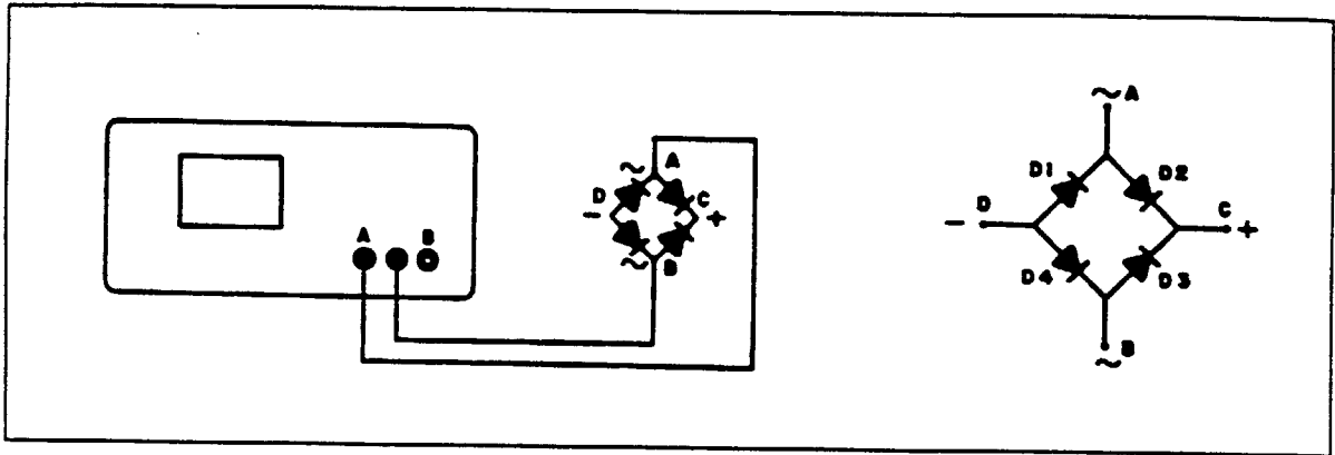
Figure 8-11. Rectifier Bridge Test Connections - AC Input.
