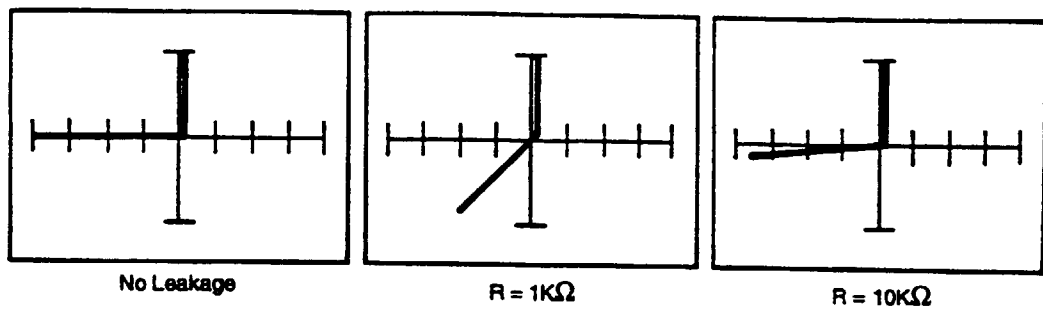
Figure 8-9c. Influence of Leakage Resistance in Medium 1 Range at 60 Hz.
