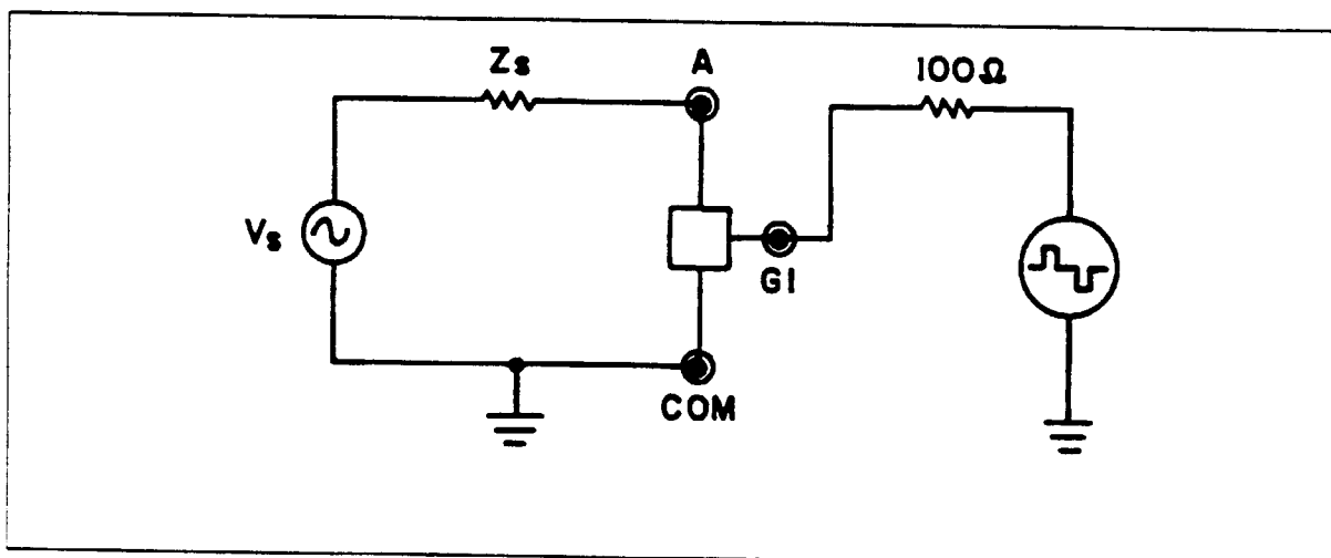
Figure 3-5. Pulse Generator/Signal Section Equivalent Circuit.
