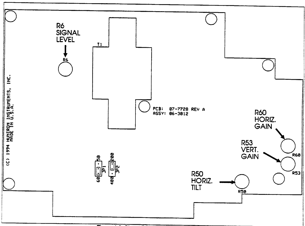
Figure 4-9. Signal PCB Adjustment Locations.
