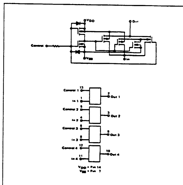
Figure 12-46. Schematic and Pin Layout of a 4016B.
