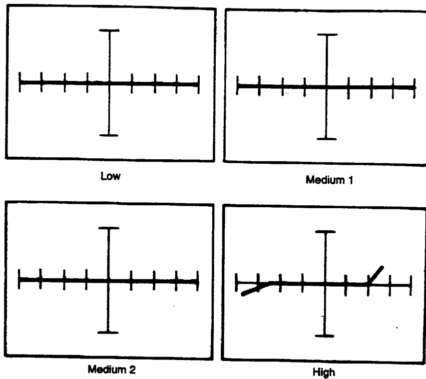
Figure 12-5. Signatures Between Pin 3 (Non-Inverting Input) and Pin 8 (V+) of an LM1458 at 60 Hz.
