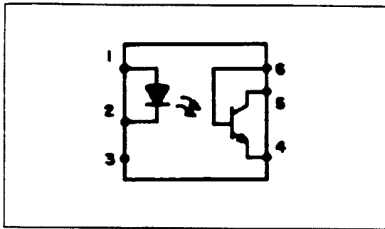
Figure 10-16. Pin Configuration of a 4N25 Transistor Optocoupler.
