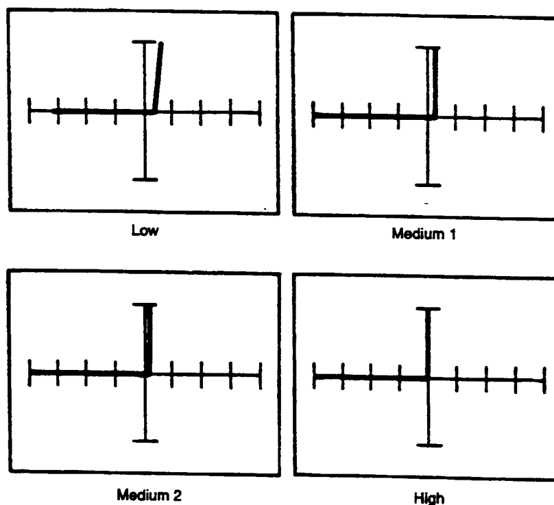
Figure 8-5. Signatures of a Silicon Diode at 60 Hz.
