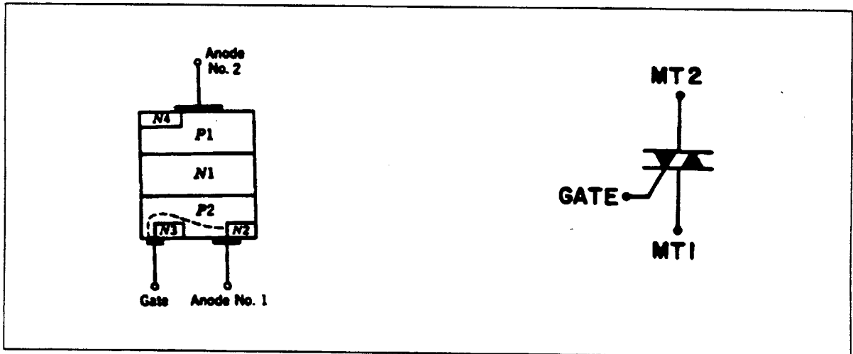
Figure 10-8. The Construction and Symbol of a Triac.
