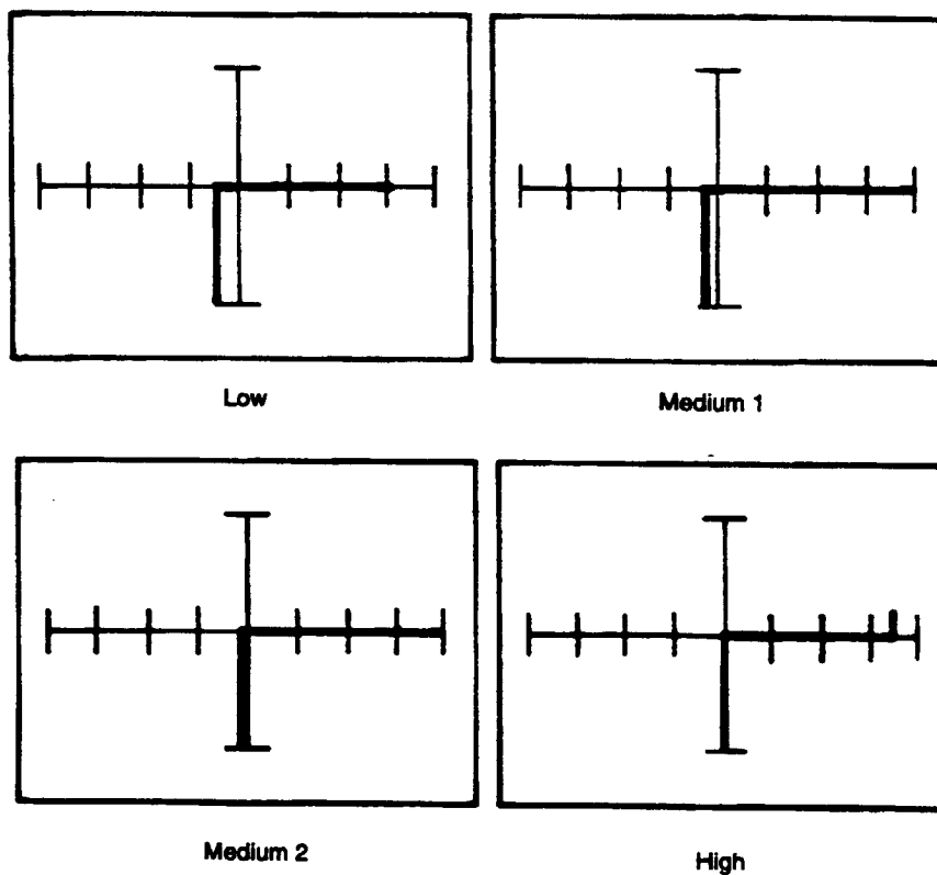
Figure 9-21. Signatures of an N-Channel JFET (2N5638) at 60 Hz. Drain with Gate as Common.
