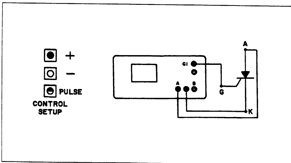
Figure 10-3. SCR Test Circuit Using the Pulse Generator.
