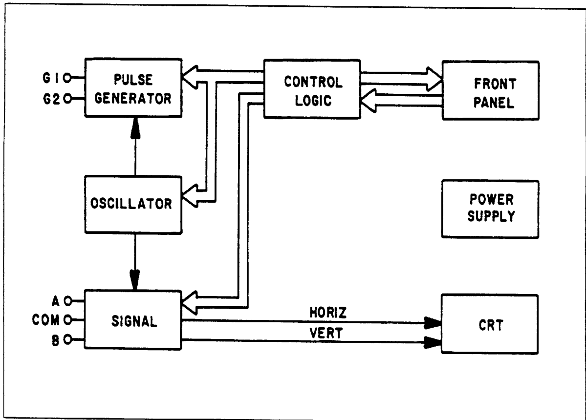
Figure 3-1. 2000 Block Diagram.
