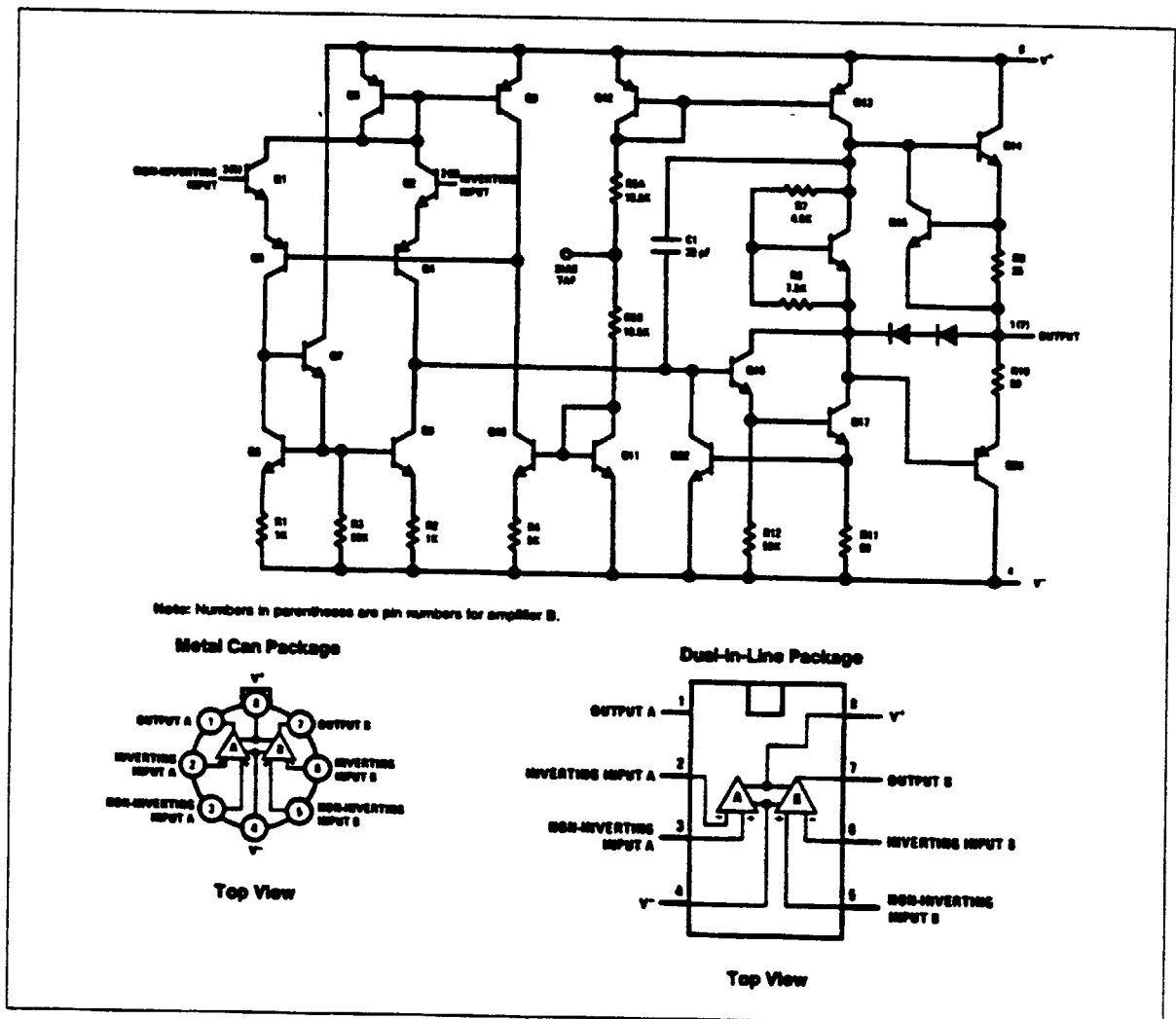
Figure 12-2. The LM1458 Op Amp, Schematic and Connections.
