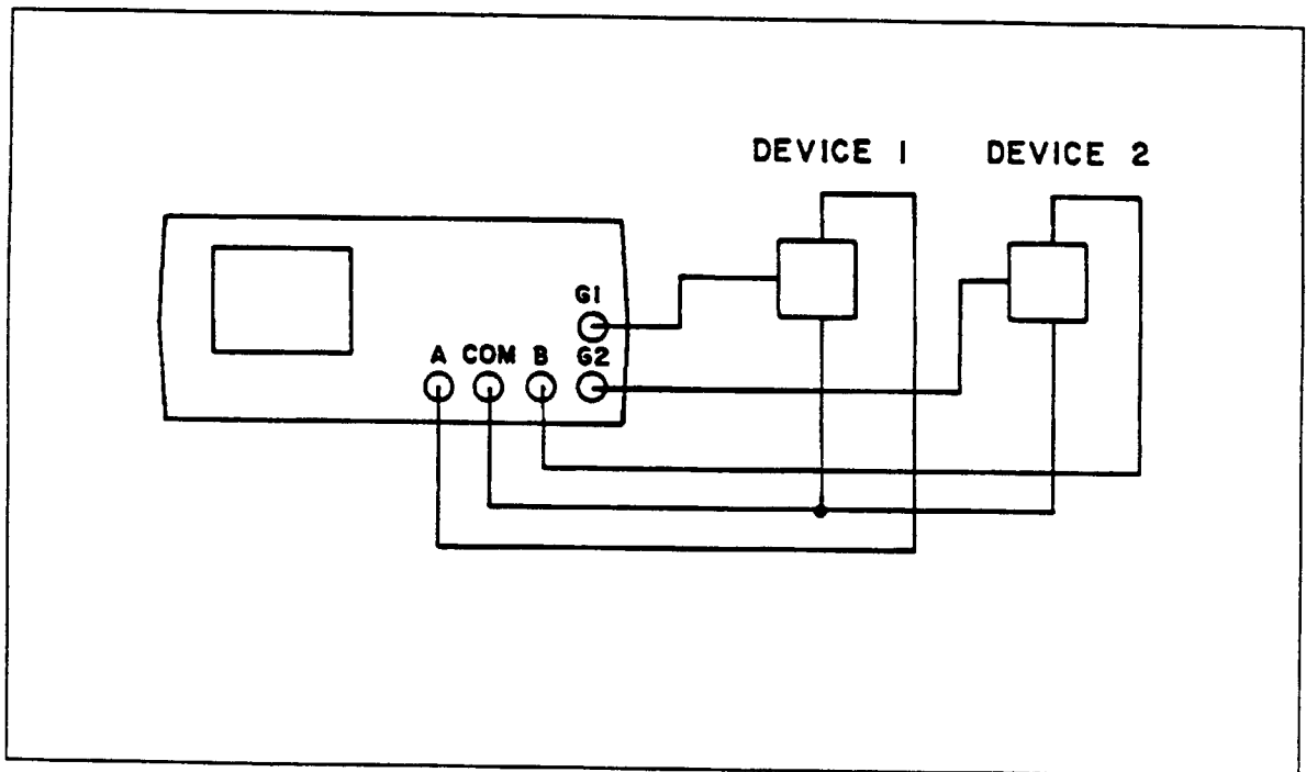
Figure 2-6. Pulse Generator Comparison Mode.
