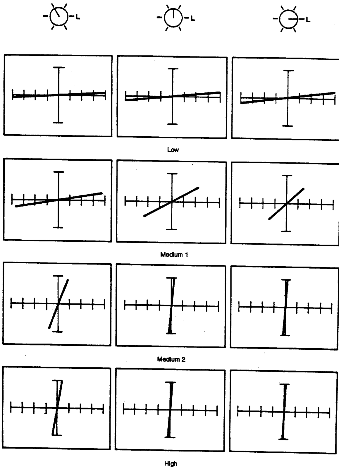
Figure 10-44. Signature Variations of a CLM51 as a Function of the Pulse Level (Maximum Pulse Width) at 60 Hz.
