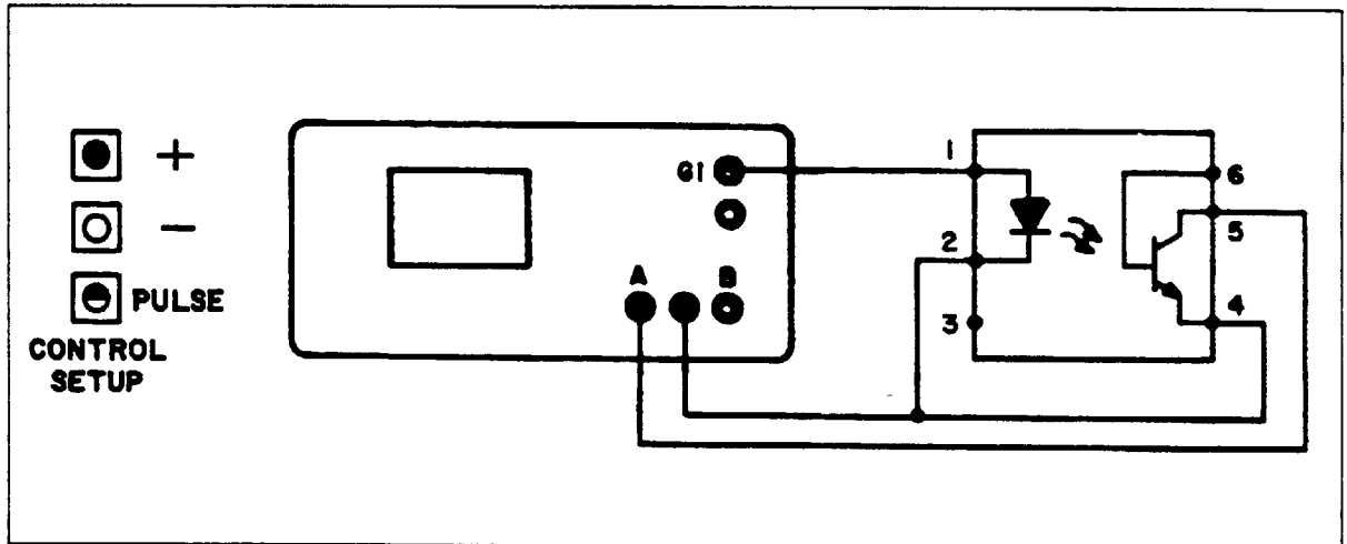
Figure 10-20. Optocoupler Test Connections Using the Pulse Generator.
