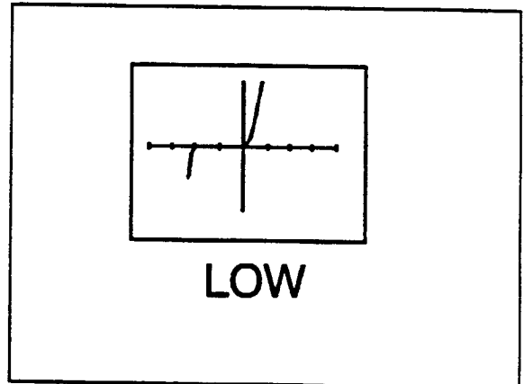
Figure 3-9b. Zener Diode Signature.
