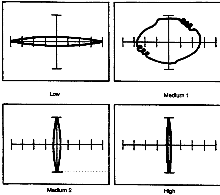
Figure 7-8. Signatures of 490mH Ferrite Inductor at 400 Hz.
