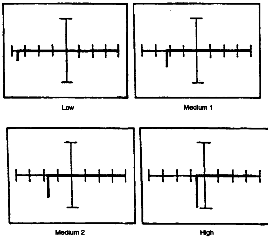
Figure 9-6. Signatures of an NPN Transistor (2N3904) at 60 Hz Collector with Emitter as Common.
