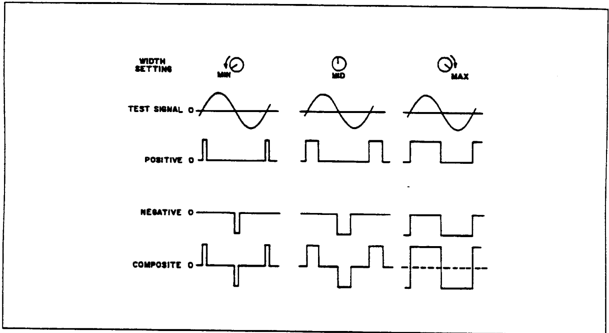
Figure 3-6. Pulse Generator Waveforms.
