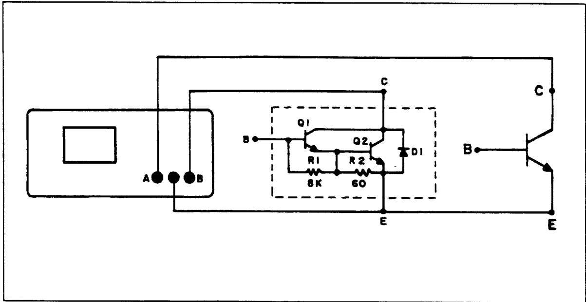
Figure 9-16. Collector-Emitter Test Circuit.
