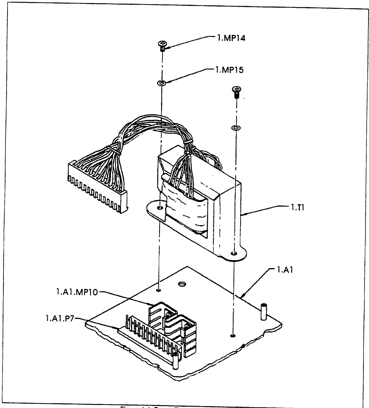
Figure 4-4. Power Transformer Removal.
