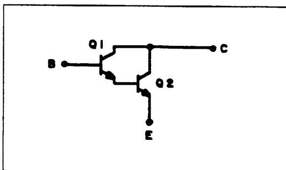
Figure 9-12. Darlington Transistor - Schematic Diagram.
