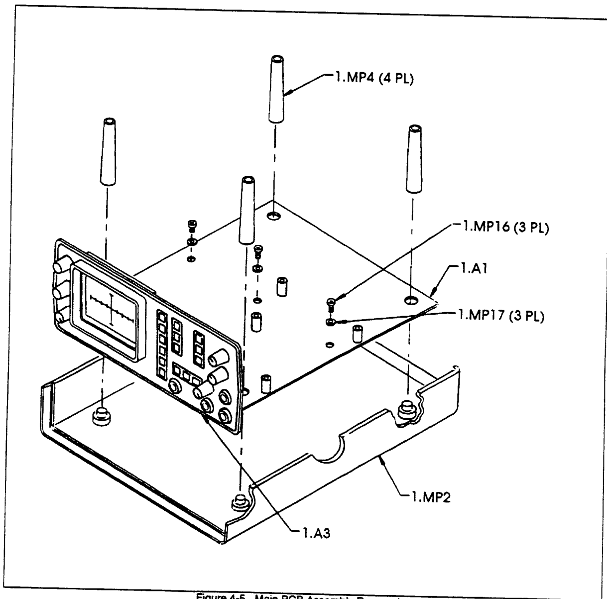
Figure 4-5. Main PCB Assembly Removal.
