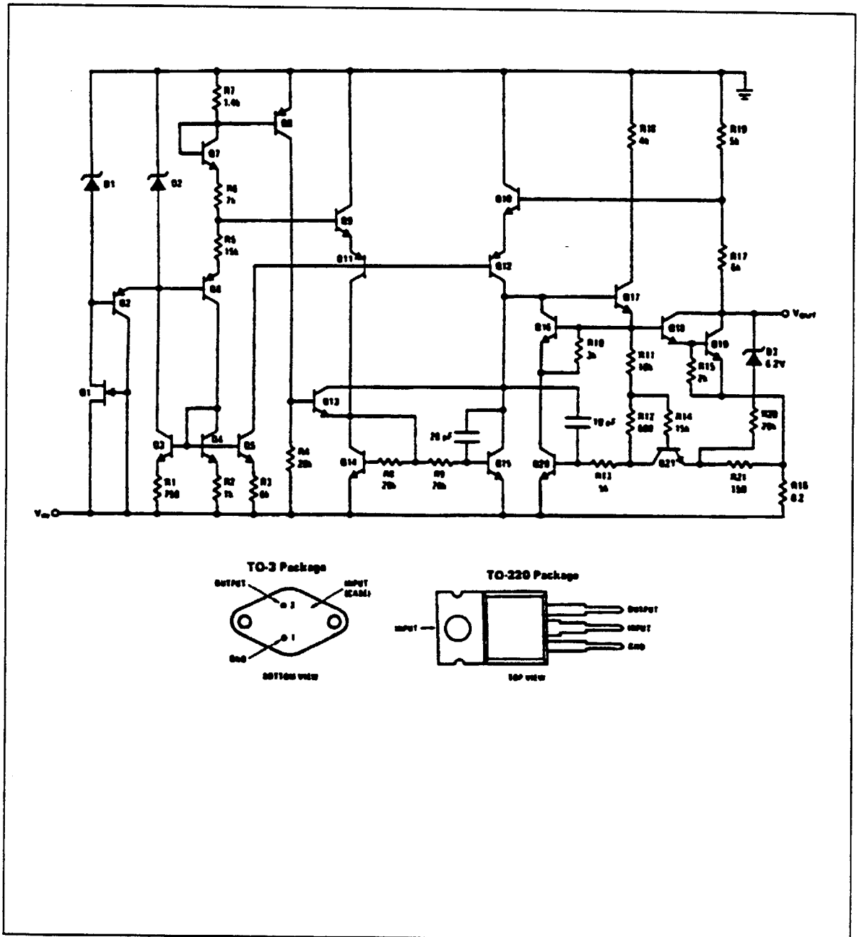
Figure 12-16. Schematic and Pin Layout of the 7905.
