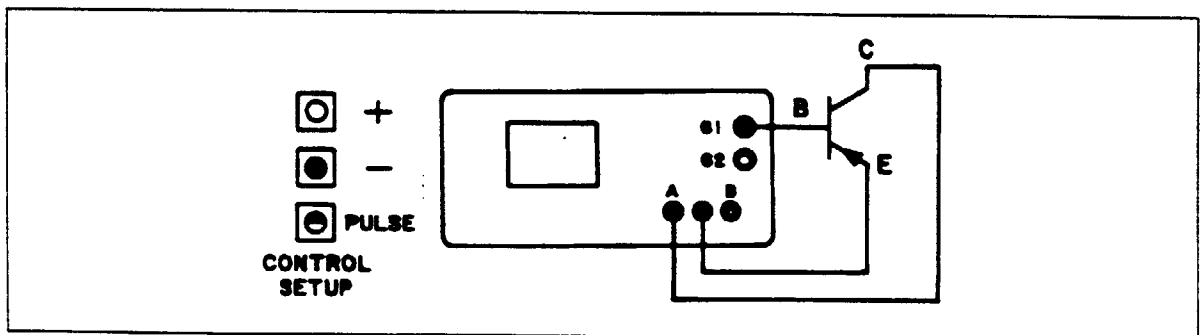
Figure 10-15a. PNP Transistor Test Circuit using the Pulse Generator.
