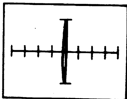
High, 1 \mu F, 60 Hz
