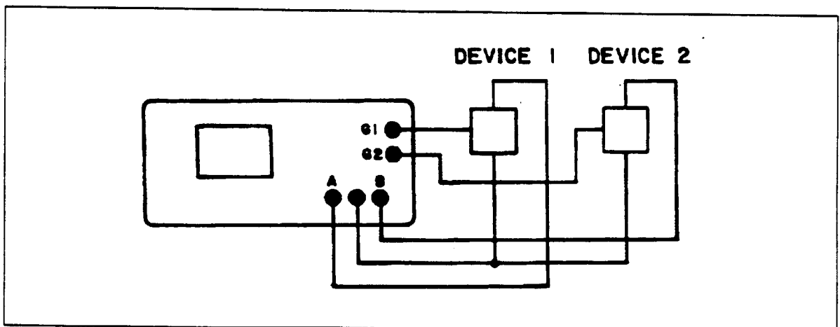
Figure 10-22. Pulse Generator Comparison Mode.
