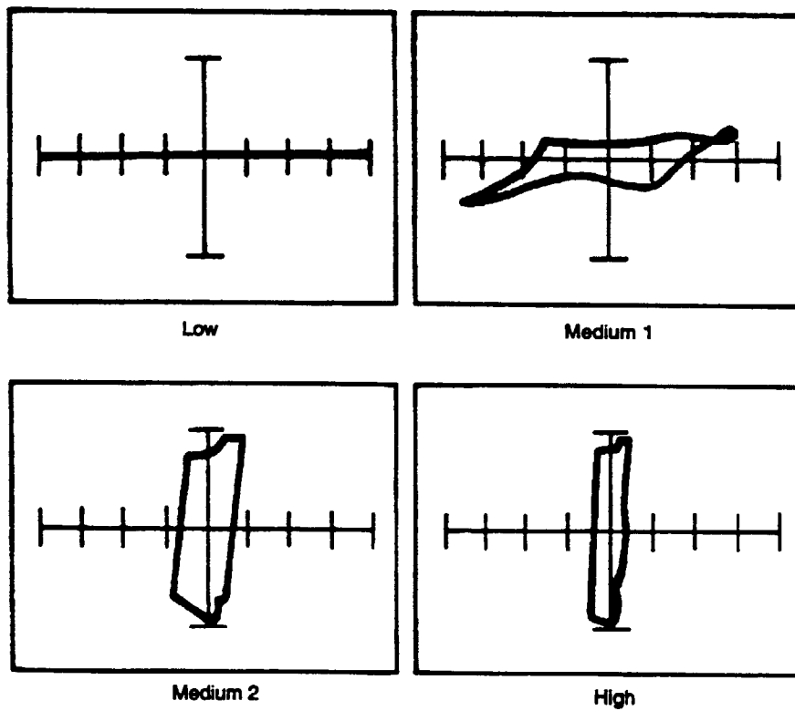
Figure 7-9. Signatures of a 490mH Ferrite Inductor at 2000 Hz.
