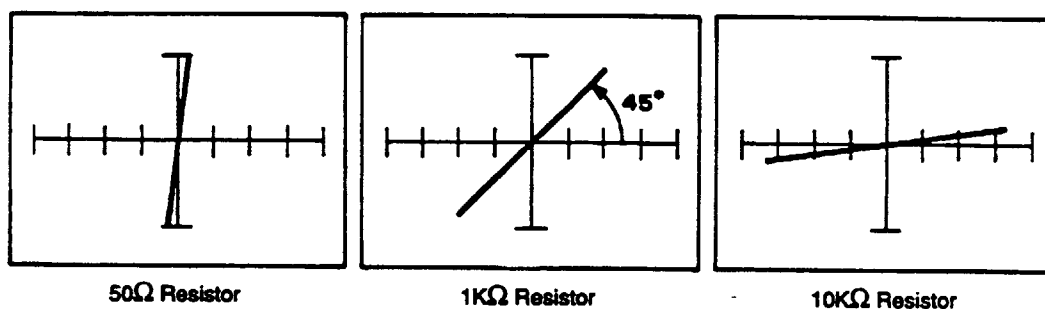
Figure 7-2. Effects of Resistance on the Rotation Angle - Medium 1 Range.
