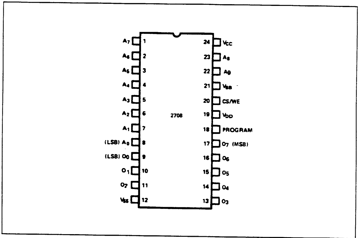
Figure 12-57. Pin Layout of a 2708JL.
