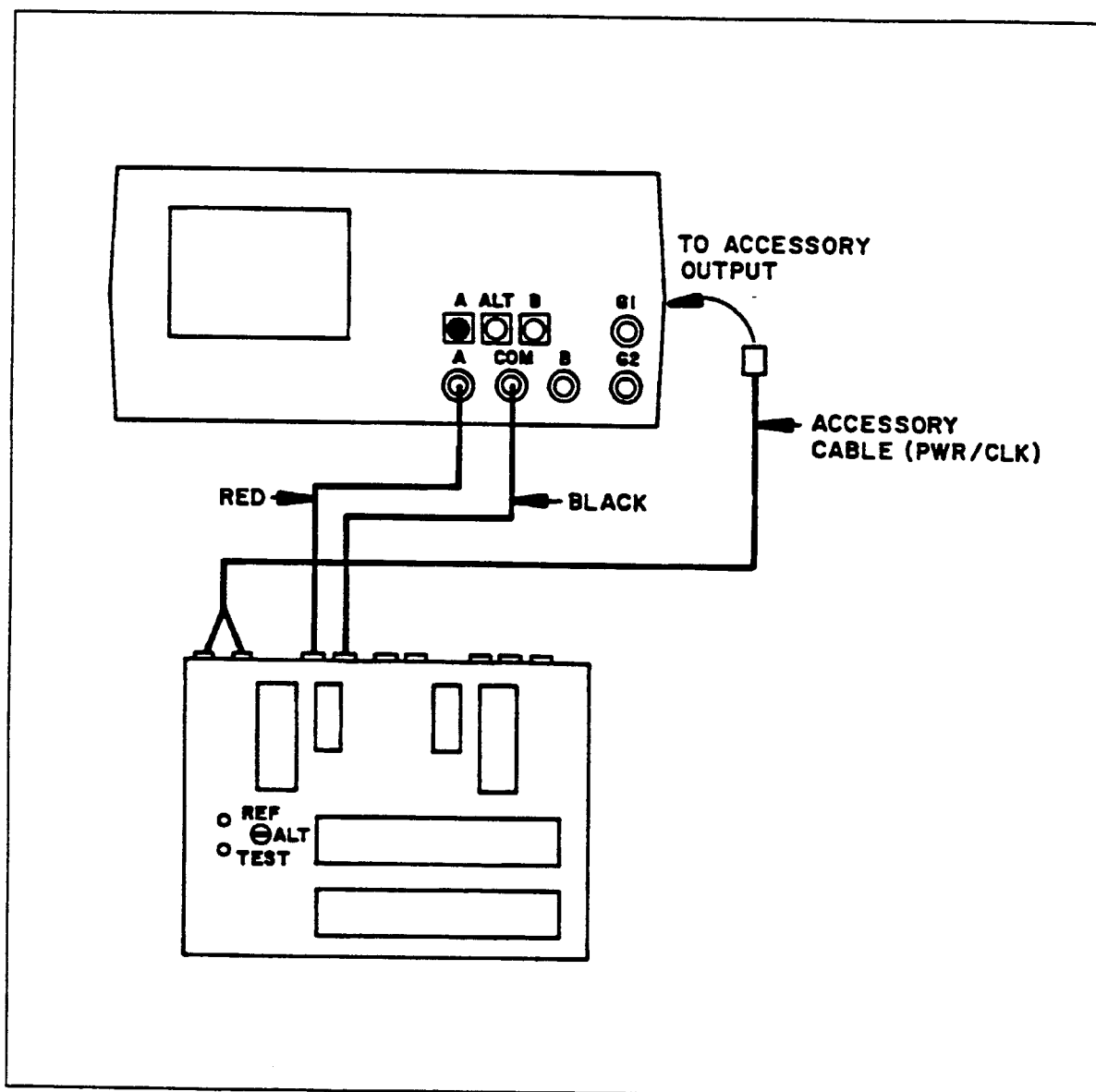
Figure 2-8. 2000/Switcher Interconnection.
