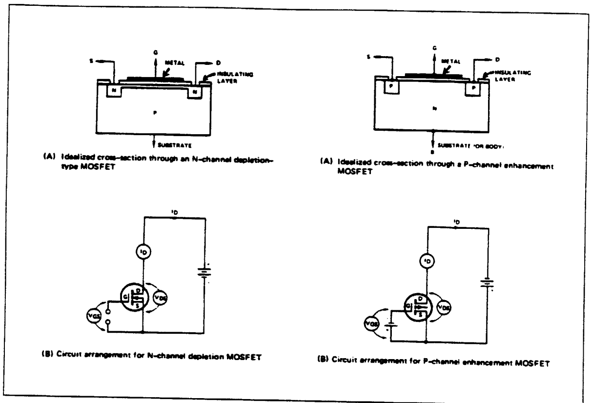
Figure 9-23. N-Channel and P-Channel MOSFET Devices.
