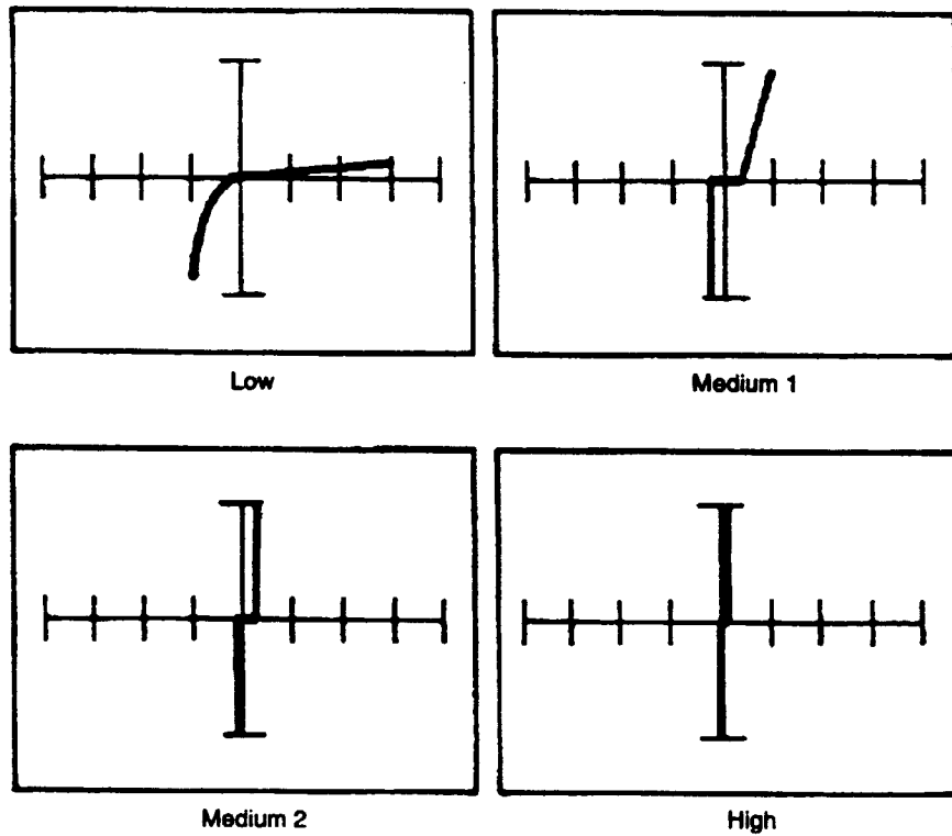
Figure 12-34. Signatures Between the V_{cc} Pin and the Ground Pin of a 7410 at 60 Hz.
