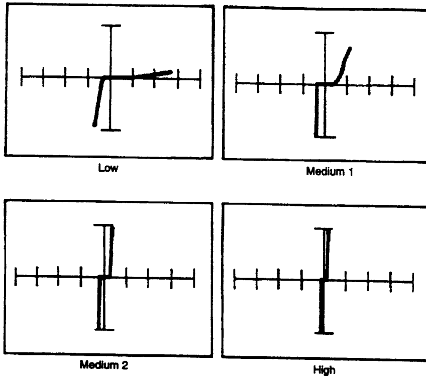
Figure 12-42. Signatures Between the V cc Pin and the Ground Pin of a 74LS125 at 60 Hz.
