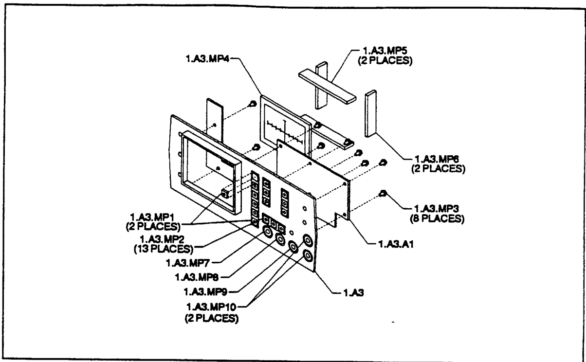
Figure 5-2. Front Control Assembly.
