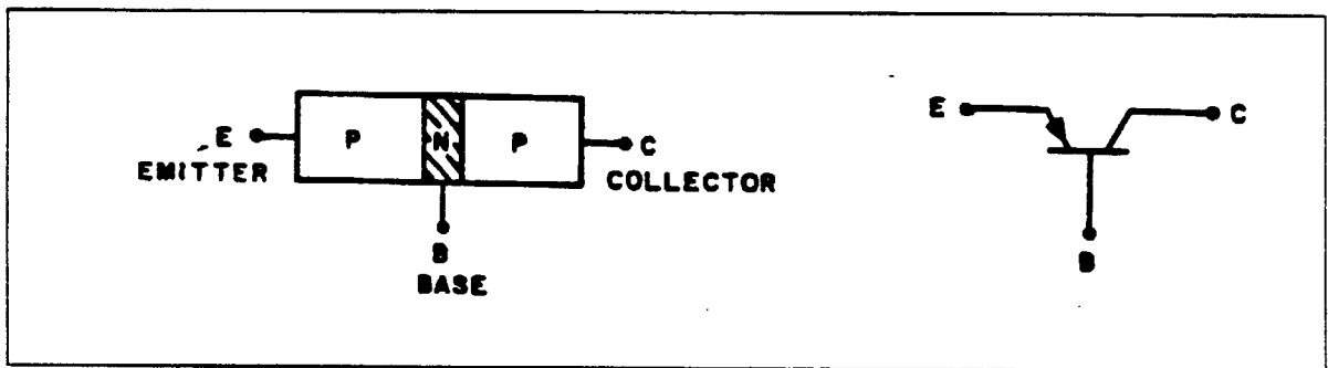
Figure 9-1. PNP Transistor and circuit Symbol.
