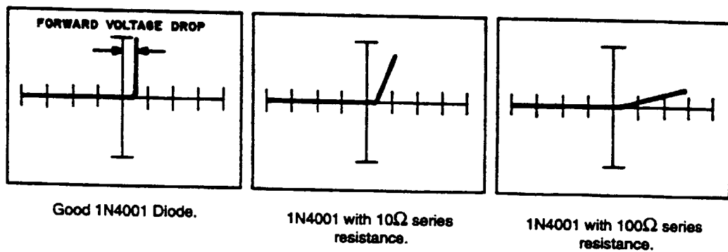
Figure 8-8a. Signature Deviation from a Good Diode in Low Range at 60Hz.
