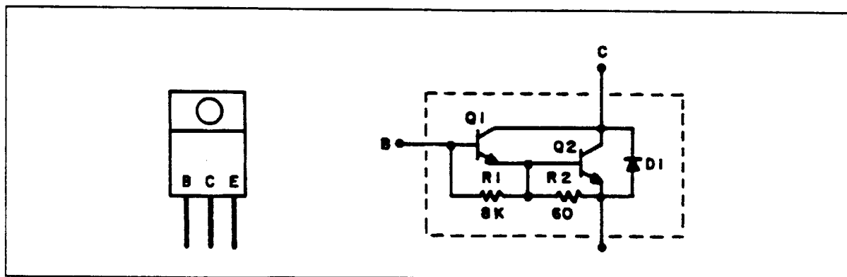
Figure 9-13. The TIP112 Darlington Transistor.
