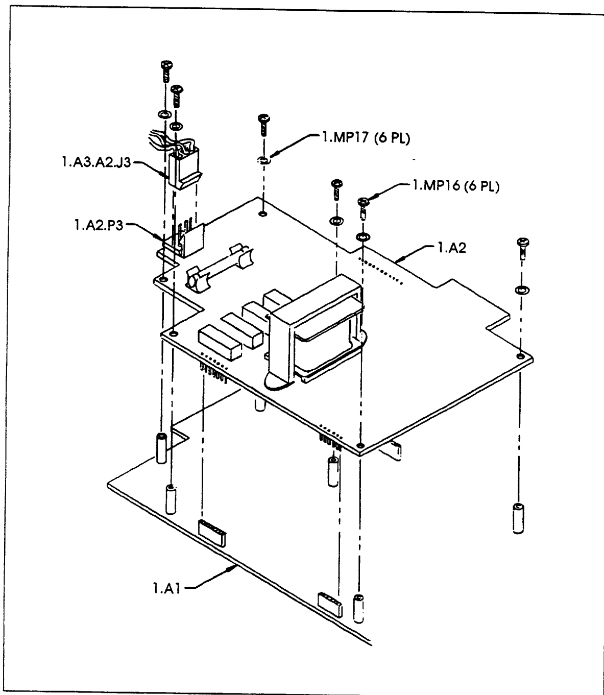
Figure 4-3. Signal PCB Assembly Removal.
