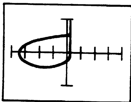
Medium 1, 1 \mu F, 60 Hz
