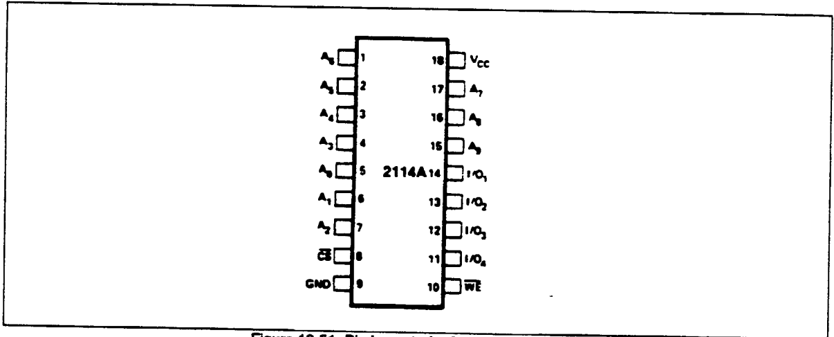
Figure 12-51. Pin Layout of a 2114A Static RAM.
