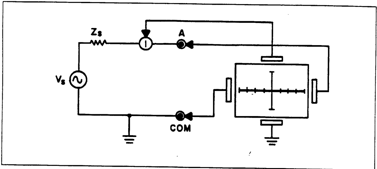
Figure 3-3. Signal Section Equivalent Circuit.
