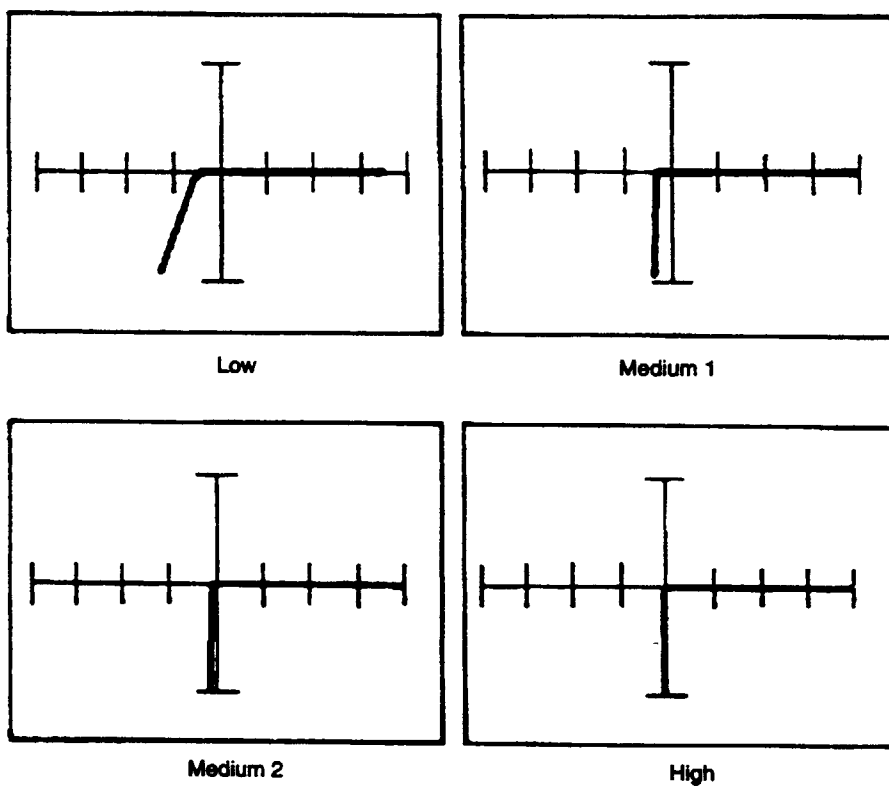
Figure 12-75. Signatures Between the V_{ref}(-) Pin and the V^- Pin of a DAC0800L at 60 Hz.
