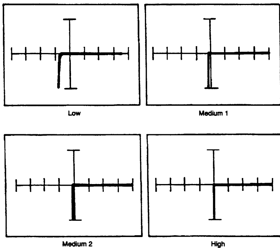
Figure 12-72. Signatures Between the I_{out} Pin and the V' Pin of a DAC0800L at 60 Hz.
