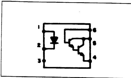
Figure 10-23. Pin Configuration of a 4N31 Darlington Transistor Optocoupler.
