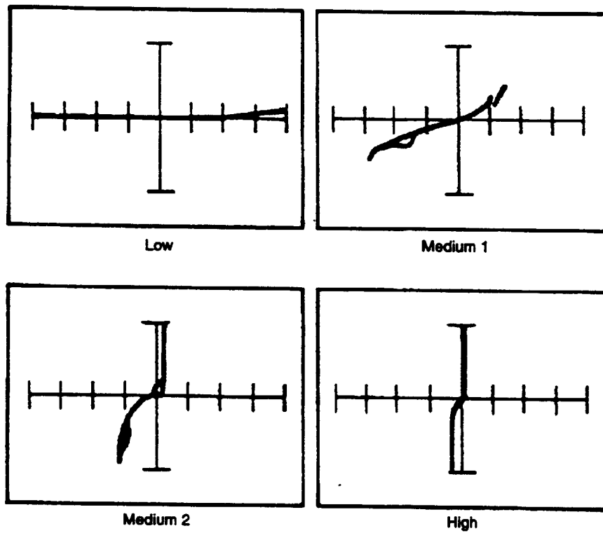
Figure 12-61. Signatures Between the V dd Pin and the V ss Pin of a 2707JL at 60 Hz.
