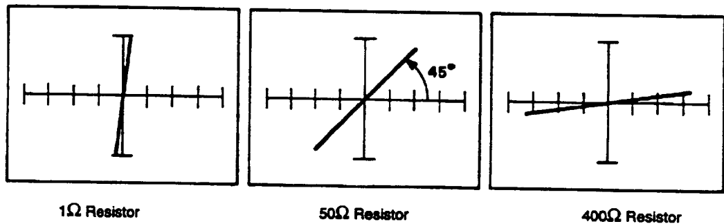
Figure 7-1. Effects of Resistance on the Rotation Angle - Low Range.
