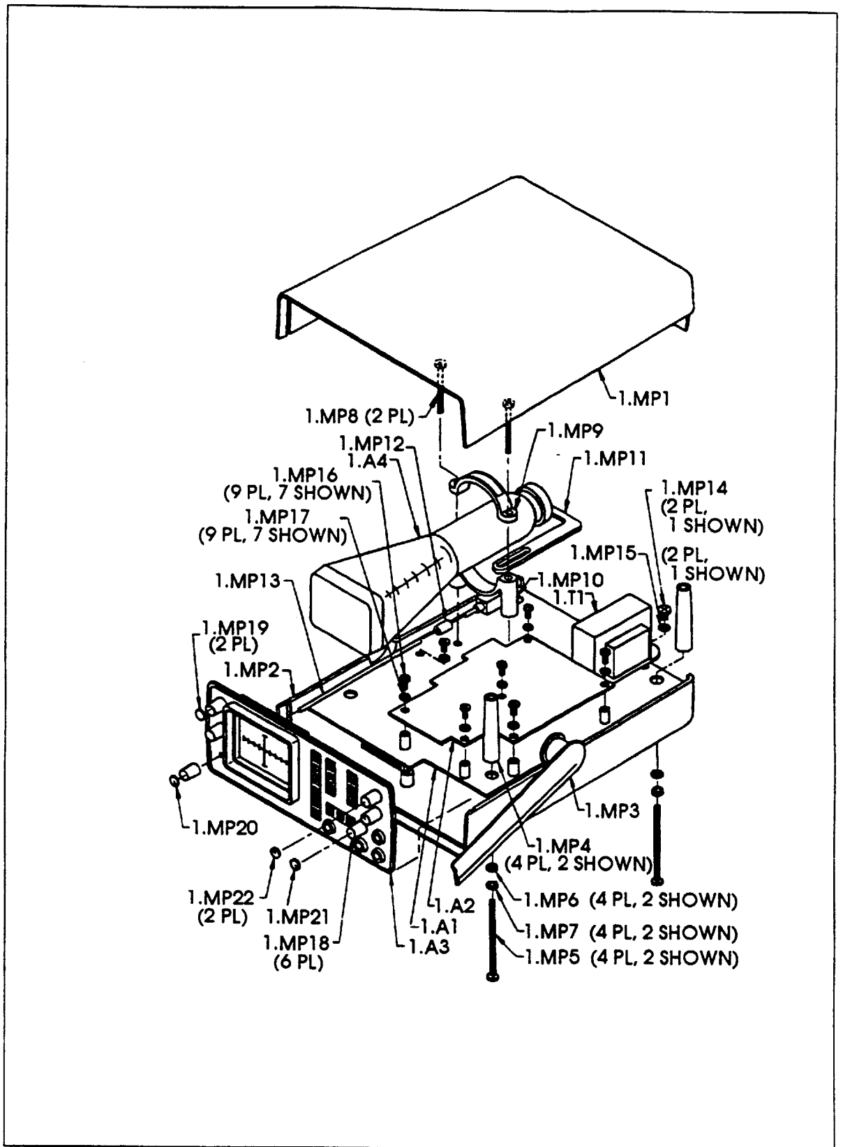
Figure 5-1. Final Assembly.
