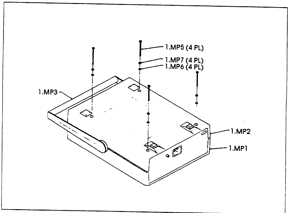
Figure 4-1. Case Screws Removal.
