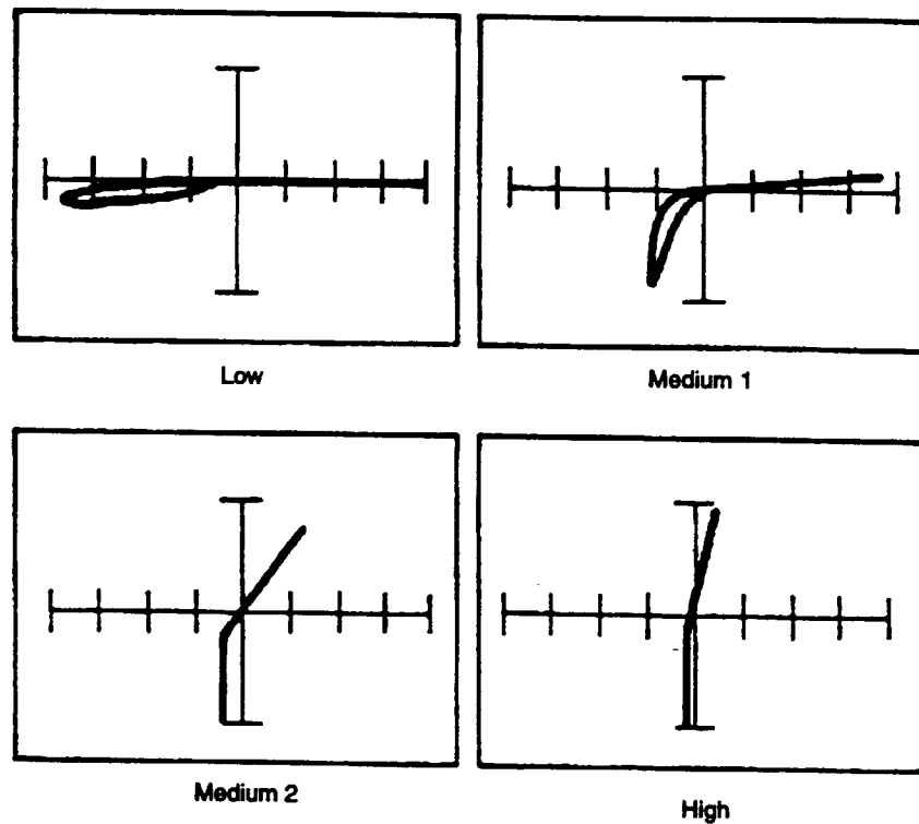
Figure 12-64. Signatures Between the V_{CC} Pin and the V_{SS} Pin of a 2708JL at 60 Hz.
