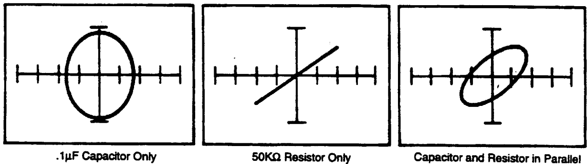
Figure 11-11. Effect of a 50\text{K}\Omega Resistor on a .1\mu\text{F} Capacitor in the High Range at 60 Hz.
