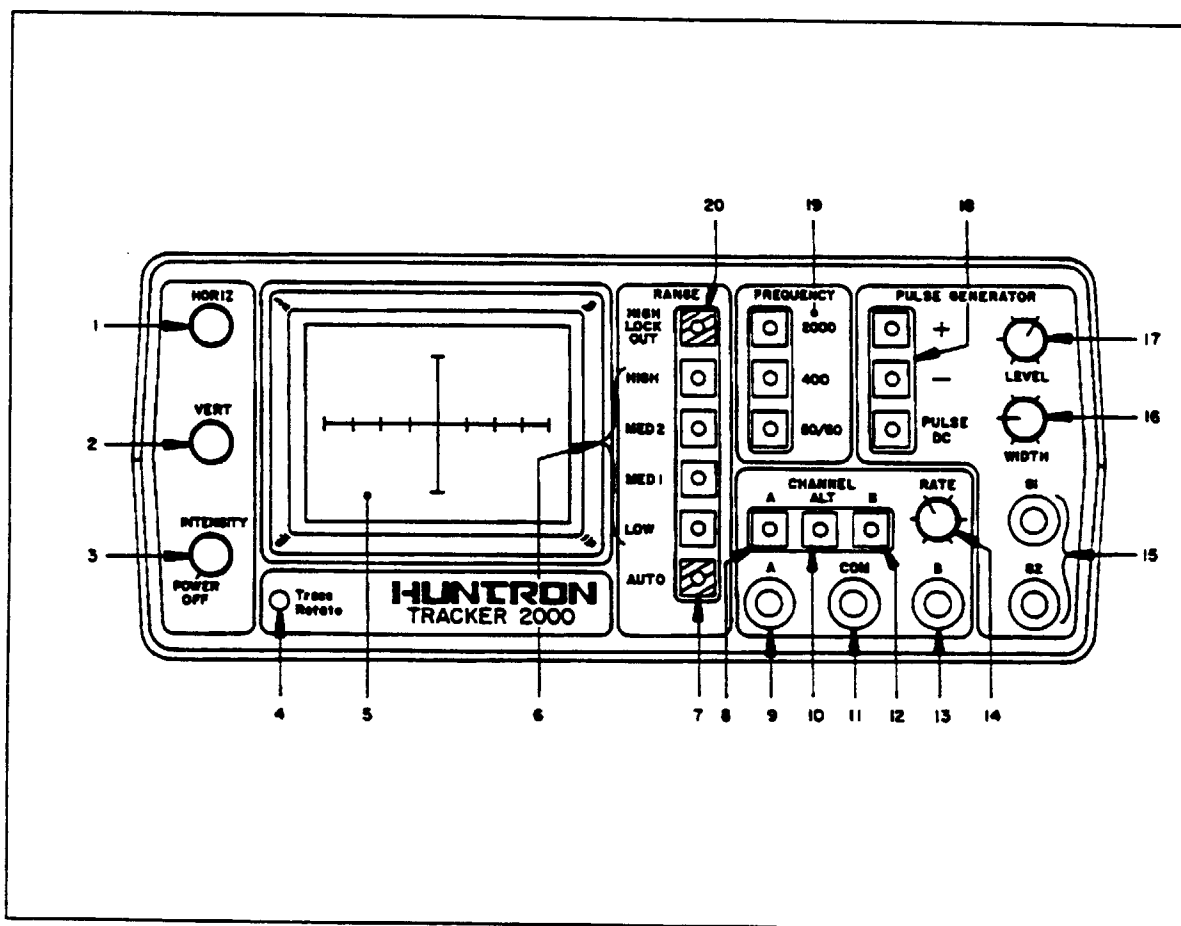
Figure 2-1. Front Panel.
