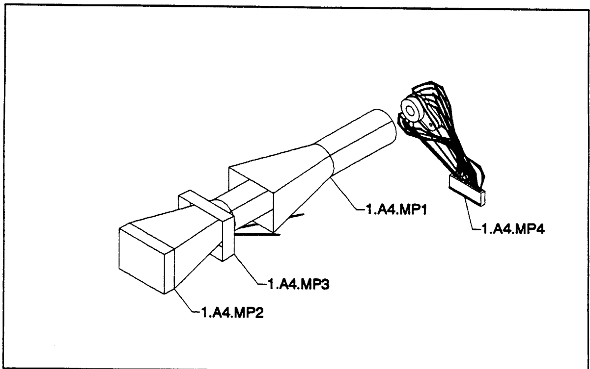
Figure 5-3. CRT Assembly.
