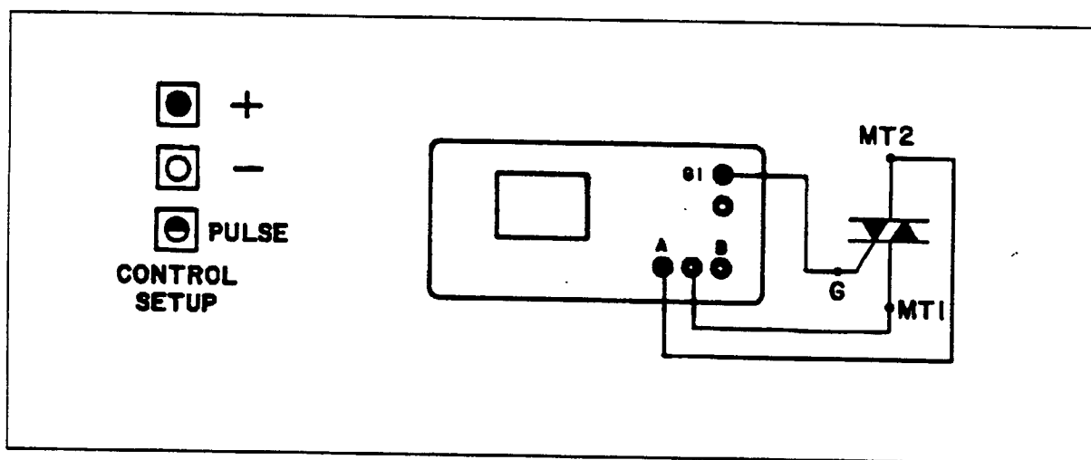
Figure 10-11. Triac Test Circuit Using the Pulse Generator.
