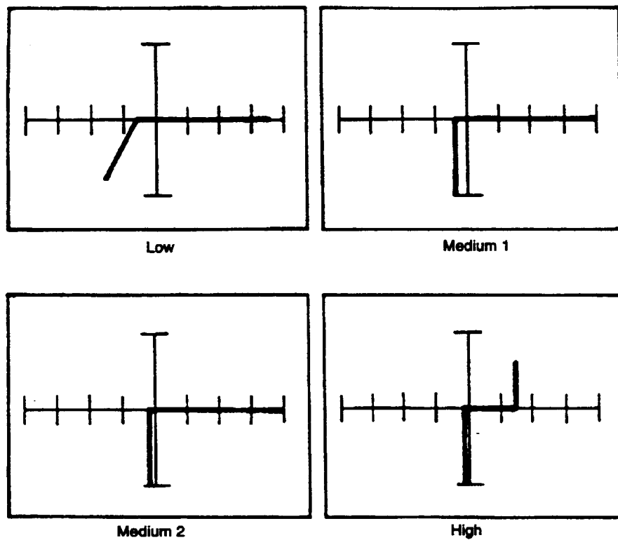
Figure 12-71. Signatures Between the V_{L0} Pin and the V' Pin of a DAC0800L at 60 Hz.
