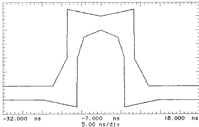
34 Mb/s Pulse Mask
