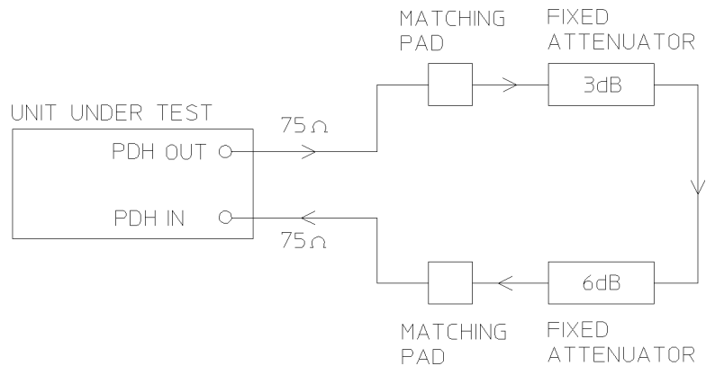
SPDH Receiver Monitor Input
