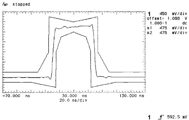
8 Mb/s Isolated Positive Pulse
