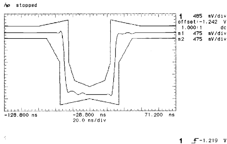
Figure 3-7 8 Mb/s Isolated Negative Pulse
