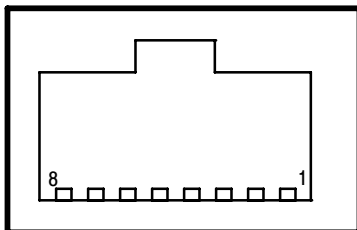
Figure 1- 1: Ethernet pinout
