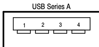
Figure 1-2: USB Host pinout
