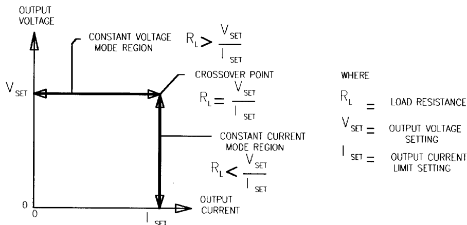
Figure 3.5-1 Operating Modes
