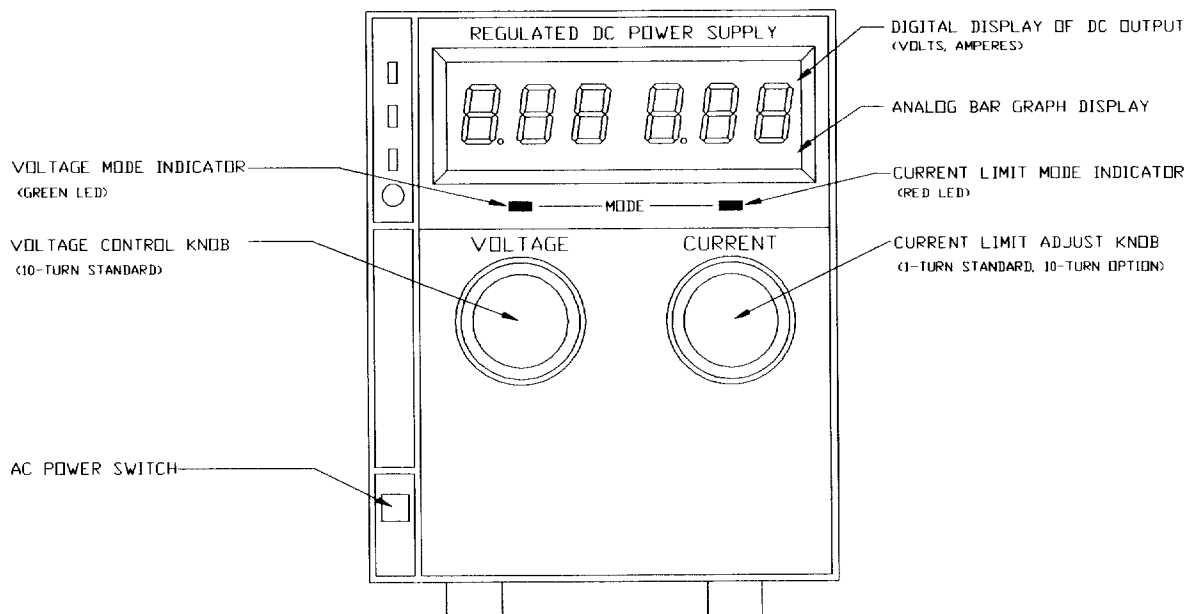
Figure 2.1-1 HPD Series Supply Front Panel
