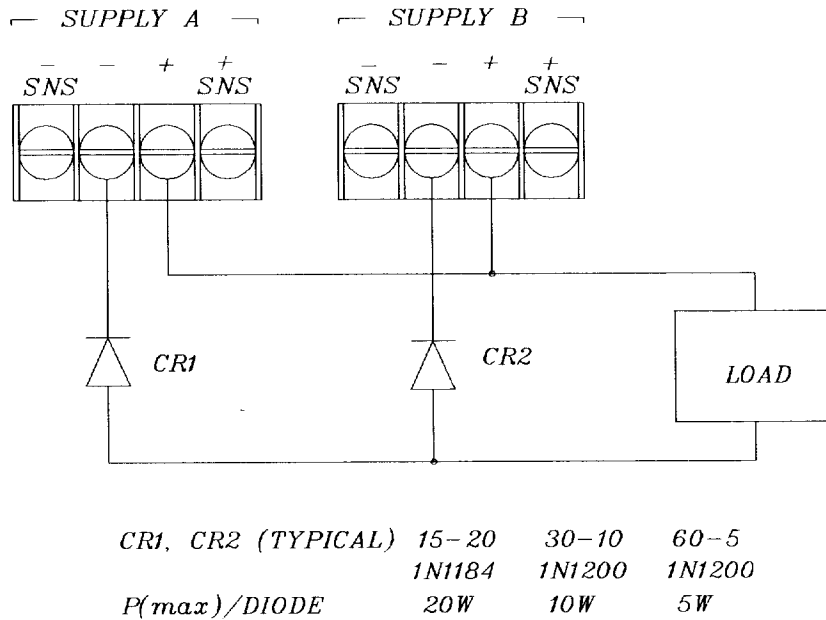
Figure 3.6-2 Parallel Operation with OVP-equipped Units
