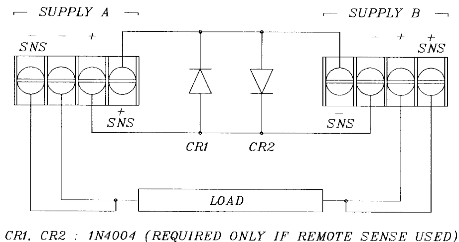
Figure 3.6-1 Series Operation with and without OVP
