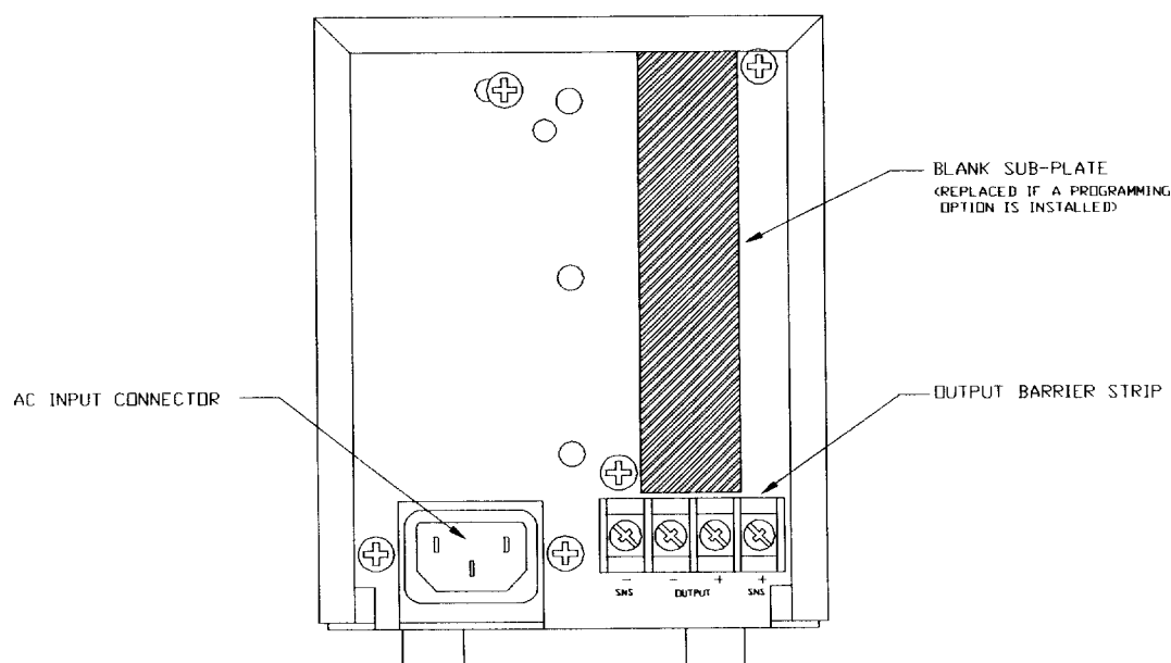
Figure 2.1-2 HPD Series Supply Rear Panel
