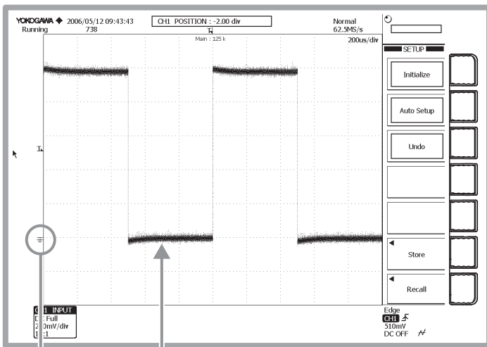
Lowering the vertical position allows the entire amplitude of the waveform to be displayed. The ground level mark is also moved.
