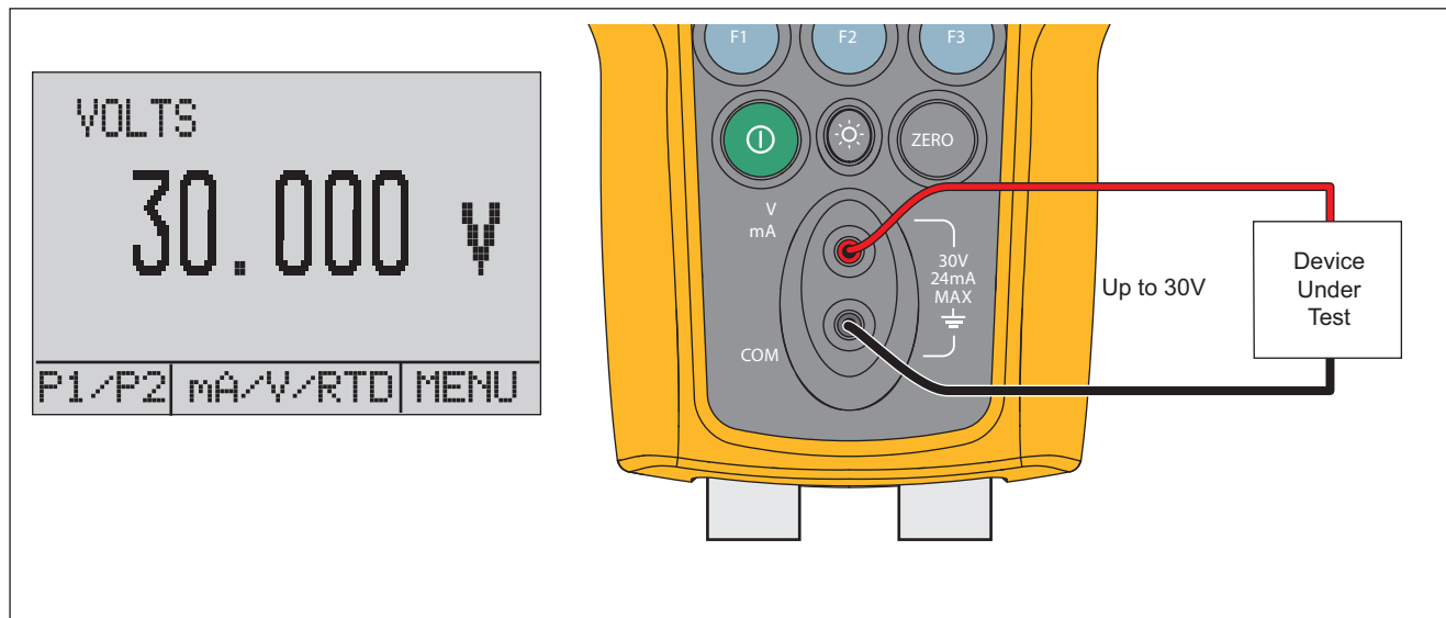
Figure 7. Voltage Measurement
